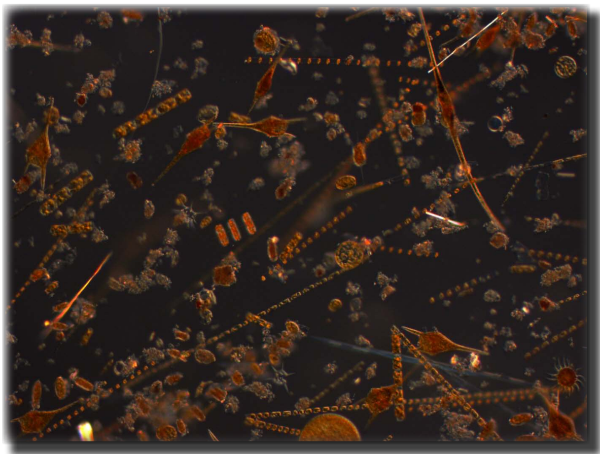
Fig.1 The spring bloom had already started in the southern part of the Kattegat area at the time of the January cruise.
