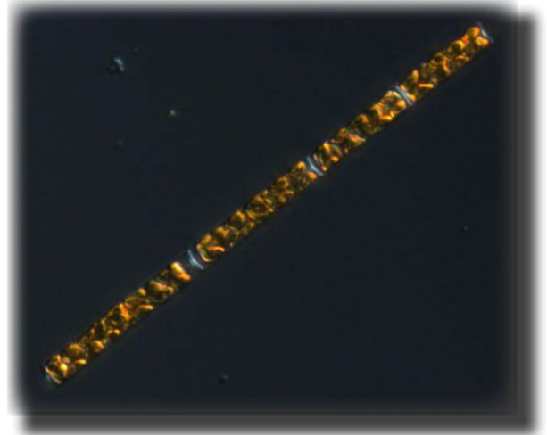
Fig.3 The spring bloom had not started in the northern part of the Kattegat and the diatom species Leptocylindrus danicus was rather alone in the sample from N14.
