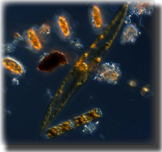
Fig.2. The beautiful phyto-benthic diatom cf. Gyrosigma sp. visited the pelagic part of the station Anholt E.
