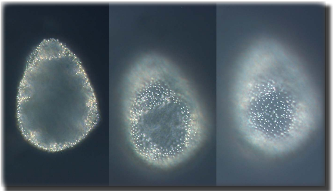
Fig.4 Very few cells were found in the Baltic Sea. This cyanobacterial colony, cf. Aphanocapsa sp., was found in BCSIII, the South East Baltic Sea.
