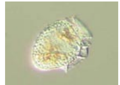
Dinophysis acuminata
