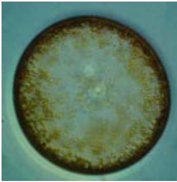
Coscinodiscus sp.
