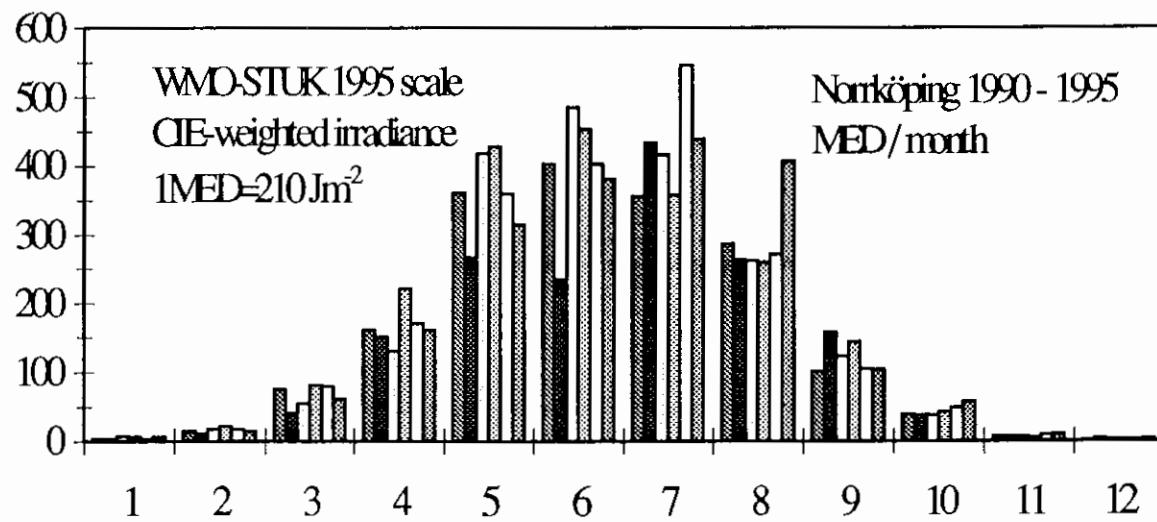
Figure 6.6 Monthly values from the station in Norrköping. The individual years are consecutively presented by different shaded bars, where 1991 has the darkest shade. Unit: MED/month. MED= Minimum Erythemal Dose corresponding to 210 \text{ Jm}^{-2} CIE-weighted irradiance, WMO-STUK 1995 scale
