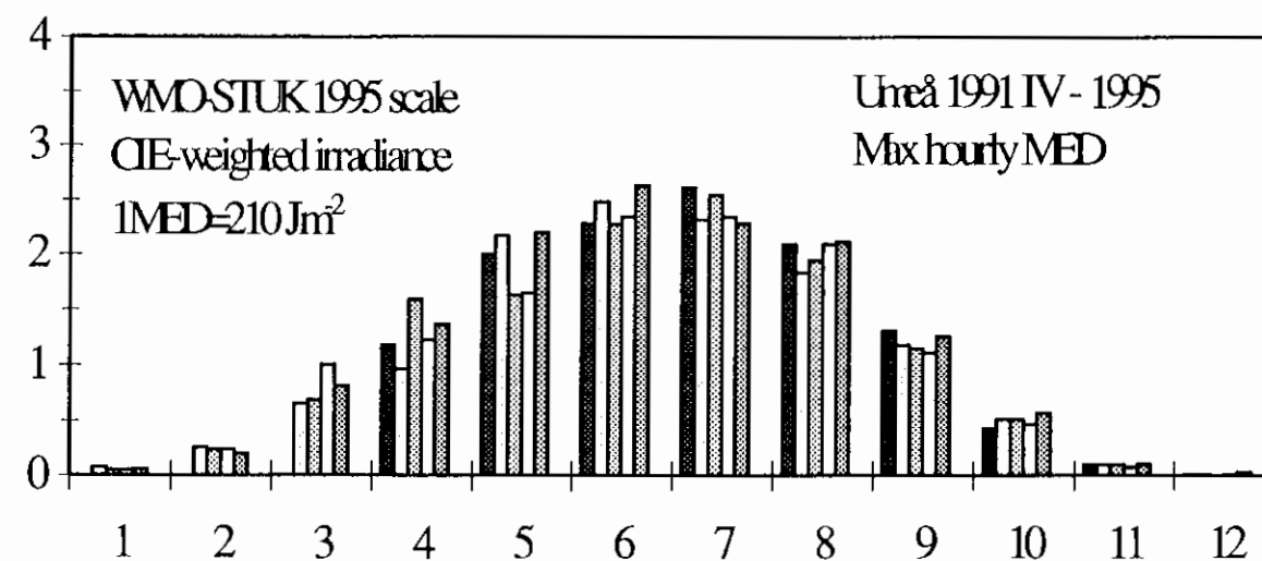
Figure 6.14 The maximum hourly value of each month of each year from the station in Umeå. Data of individual years are consecutively presented by different shaded bars, where 1991 has the darkest shade. Unit: Max MED/hour. MED= Minimum Erythemat Dose corresponding to 210 \text{ Jm}^{-2} CIE-weighted irradiance, WMO-STUK 1995 scale.
