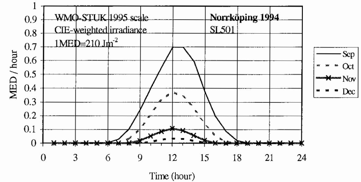
Figure 6.24 Average hourly values of the months September to December of 1994 from the station in Norrköping recorded by Solar Light Model 501 #922. Data of individual months are presented by different lines. Unit: MED/hour. MED= Minimum Erythemal Dose corresponding to 210 \text{ Jm}^{-2} CIE-weighted irradiance, WMO-STUK 1995 scale.
