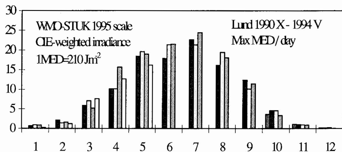
Figure 6.12 The maximum daily value of each month of each year from the station in Lund. Data of individual years are consecutively presented by different shaded bars, where 1991 has the darkest shade. Unit: Max MED/day. MED= Minimum Erythemat Dose corresponding to 210 \text{ Jm}^{-2} CIE-weighted irradiance, WMO-STUK 1995 scale.
