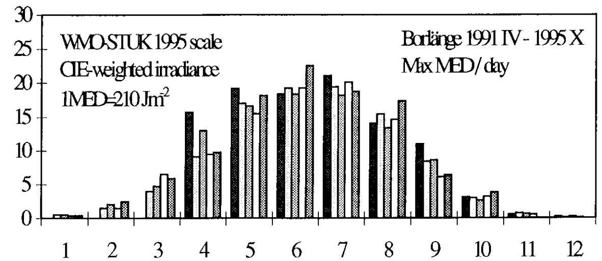
Figure 6.10 The maximum daily value of each month of each year from the station in Borlänge. Data of individual years are consecutively presented by different shaded bars, where 1991 has the darkest shade. Unit: Max MED/day. MED= Minimum Erythemal Dose corresponding to 210 \text{ Jm}^{-2} CIE-weighted irradiance, WMO-STUK 1995 scale.
