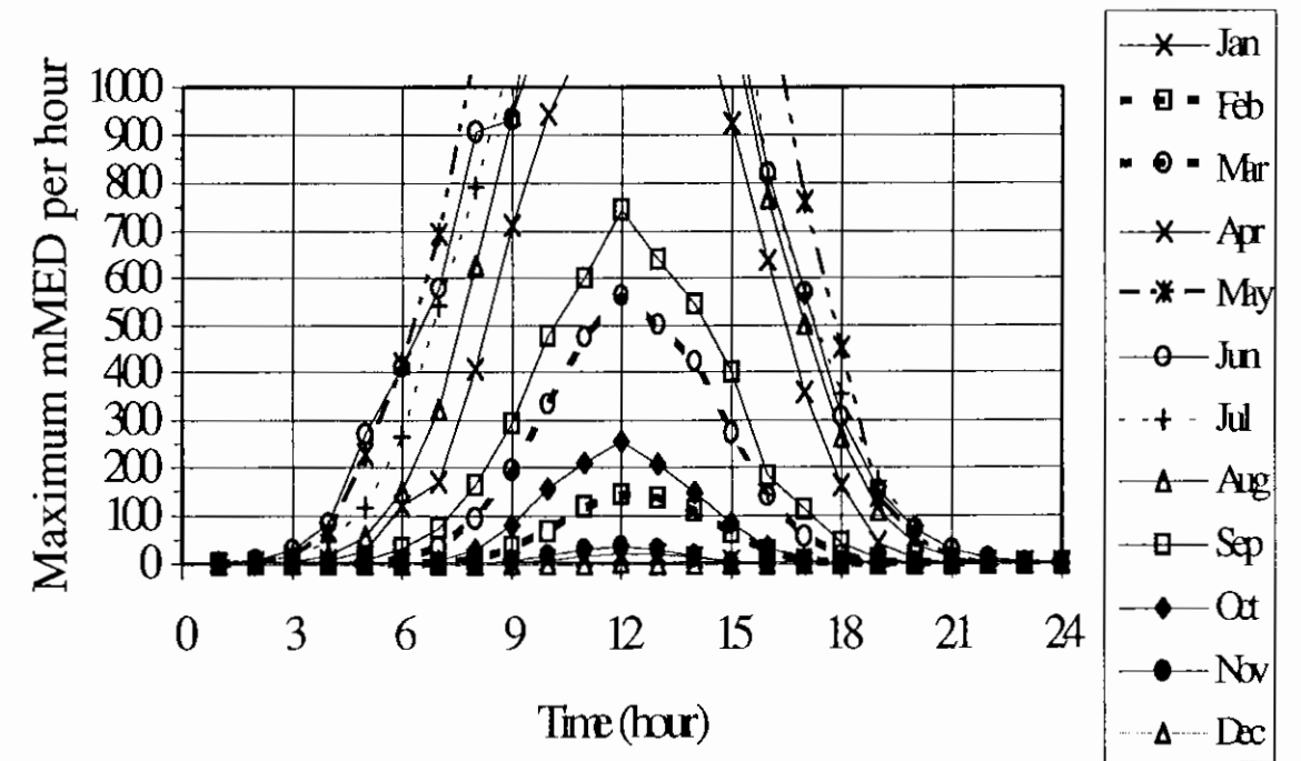
Figure 6.21 Enlargement of the lower part of Figure 6.20. Maximum hourly values of each month during 1991 from the station in Kiruna. Data of individual months are presented by different lines and symbols. Unit: mMED/hour. MED= Minimum Erythemal Dose corresponding to 210 \text{ Jm}^{-2} CIE-weighted irradiance, WMO-STUK 1995 scale.
