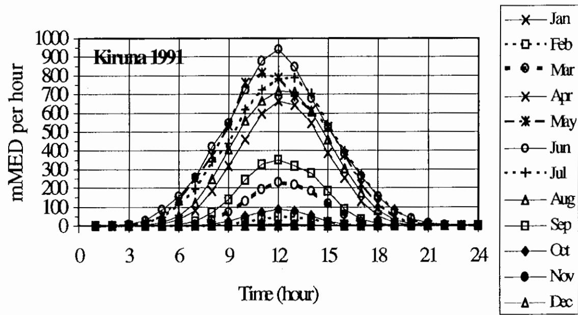
Figure 6.18 Average hourly values of each month during 1991 from the station in Kiruna. Data of individual months are presented by different lines and symbols. Unit: mMED/hour. MED= Minimum Erythemal Dose corresponding to 210 \text{ Jm}^{-2} CIE-weighted irradiance, WMO-STUK 1995 scale.
