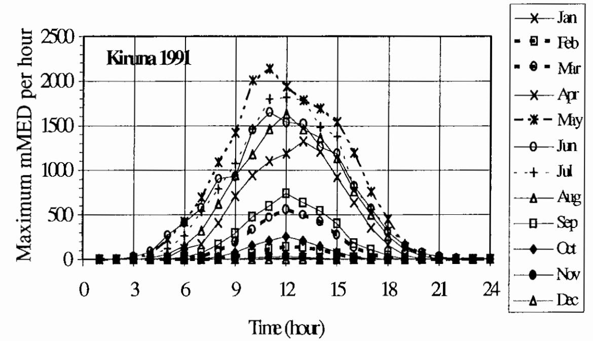
Figure 6.20 Maximum hourly values of each month during 1991 from the station in Kiruna. Data of individual months are presented by different lines and symbols. Unit: mMED/hour. MED= Minimum Erythemal Dose corresponding to 210 \text{ Jm}^{-2} CIE-weighted irradiance, WMO-STUK 1995 scale.
