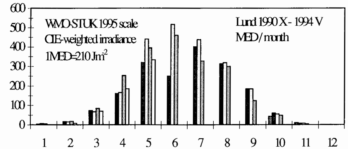
Figure 6.7 Monthly values from the station in Lund. The individual years are consecutively presented by different shaded bars, where 1991 has the darkest shade. Unit: MED/month. MED= Minimum Erythemal Dose corresponding to 210 \text{ Jm}^{-2} CIE-weighted irradiance, WMO-STUK 1995 scale
