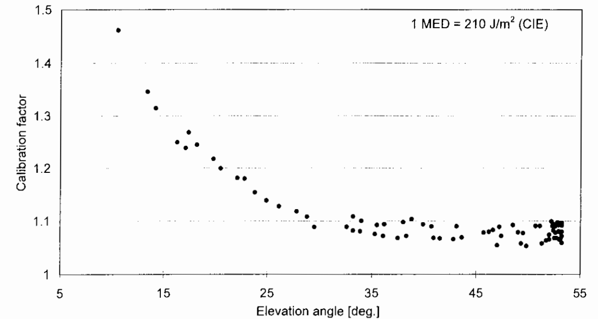
Figure 3.1.2 The calibration factor of Solar Light Model 501 #922 as measured at the WMO-STUK 1995 intercomparison in Helsinki. The reference data are cosine corrected, K. Leszczynski pers.comm.
