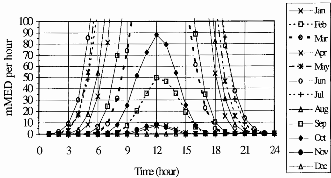
Figure 6.19 Enlargement of the lower part of Figure 6.18. Average hourly values of each month during 1991 from the station in Kiruna. Data of individual months are presented by different lines and symbols. Unit: mMED/hour. MED= Minimum Erythemal Dose corresponding to 210 \text{ Jm}^{-2} CIE-weighted irradiance, WMO-STUK 1995 scale.
