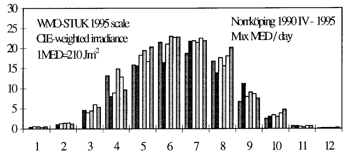
Figure 6.11 The maximum daily value of each month of each year from the station in Norrköping. Data of individual years are consecutively presented by different shaded bars, where 1991 has the darkest shade. Unit: Max MED/day. MED= Minimum Erythemal Dose corresponding to 210 \text{ Jm}^{-2} CIE-weighted irradiance, WMO-STUK 1995 scale.
