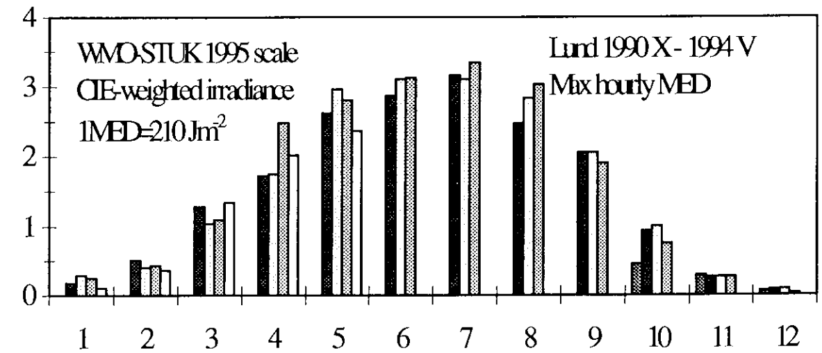
Figure 6.17 The maximum hourly value of each month of each year from the station in Lund. Data of individual years are consecutively presented by different shaded bars, where 1991 has the darkest shade. Unit: Max MED/hour. MED= Minimum Erythemat Dose corresponding to 210 Jm -2 CIE-weighted irradiance, WMO-STUK 1995 scale.
