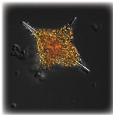
Dictyocha fibula
