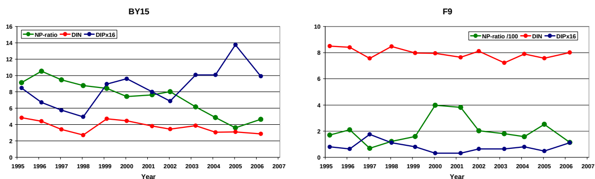
Figure 7. Left: The maximum observed surface layer (10 m) DIN to DIP ratio (green) in early spring and corresponding DIP (x16) (mmolPm -3 ) (blue) and DIN (mmolNm -3 ) (red) values at the Gotland Deep station BY15 (Left). Right: The minimum observed surface layer (10 m) DIN to DIP ratio (divided by 100) in early spring and corresponding DIP (x16) (mmolPm -3 ) and DIN (mmolNm -3 ) values at the Bothnian Bay station F9.
