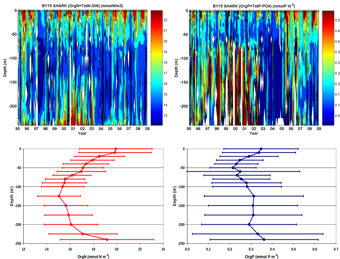
Figure 1. Upper: Observations (mmol m -3 ) of organic nitrogen (left) and phosphorus (right), defined as total N (P) – inorganic N (P), respectively, at the Gotland Deep station BY15 during the period 1995-2008 (data from SHARK). White areas lack observations. The upper black tic marks indicate dates of observations. Lower: Corresponding mean values of organic nitrogen (left) and phosphorus (right) (mmol N m -3 ) and ±1 standard deviation given by error bars.
