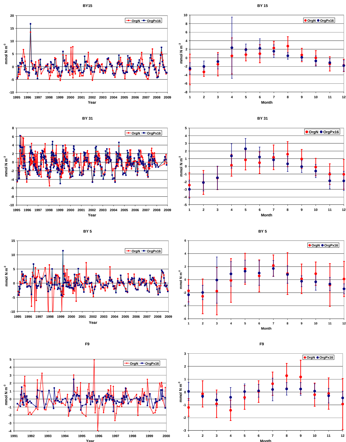
Figure 4. Annual anomaly variations (Left) of OrgN (mmol N m -3 ) (red) and the corresponding estimate of OrgN based on the Redfield model, OrgN=OrgP x 16, (blue). The right panel show the corresponding monthly means and \pm 1 standard deviation. The stations listed from above and down are BY15, BY31, BY5 and F9.
