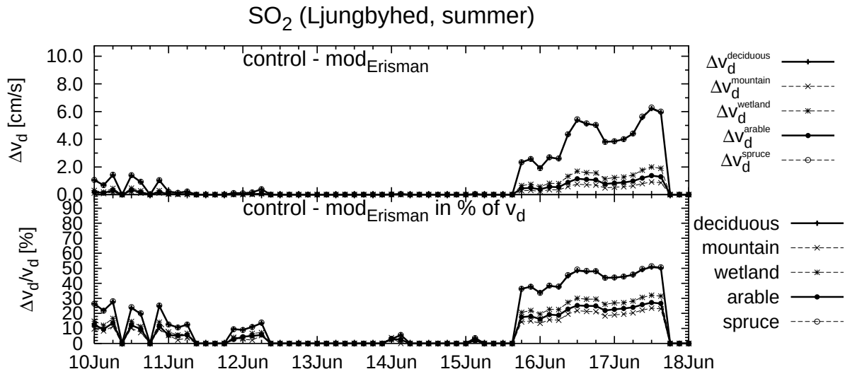
Figure 15: Same as Figure 13, but for the differences between the control run (original Erismann scheme) and the run with a lower limit of r_{\text{ext}} = 10 \text{ sm}^{-1} for \text{SO}_2 (modified Erismann scheme).
