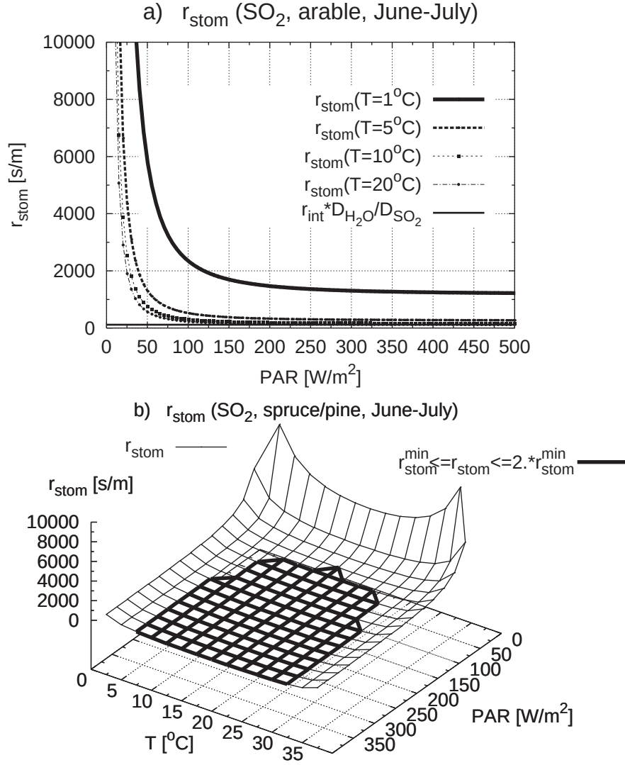
Figure 6. Computation of the stomata resistance after Wesley (1989). a) Variation of r_{\text{stom}} with photosynthetically active radiation PAR for different near surface temperatures T , assuming an internal resistance r_{\text{int}} = 60 \text{ s/m} (June-July, arable). b) Three-dimensional display of the variation of r_{\text{stom}} with T and PAR for spruce/pine ( r_{\text{int}} = 130 \text{ s/m} ). The thick lines indicate the area with r_{\text{stom}}^{\text{min}} \leq r_{\text{stom}} \leq 2 \cdot r_{\text{stom}}^{\text{min}} where r_{\text{stom}}^{\text{min}} = r_{\text{int}} \cdot D_{\text{H}_2\text{O}} / D_{\text{SO}_2} . Note that the variation of r_{\text{stom}} with temperature is symmetric about an optimum temperature of T = 20^\circ \text{C} .
