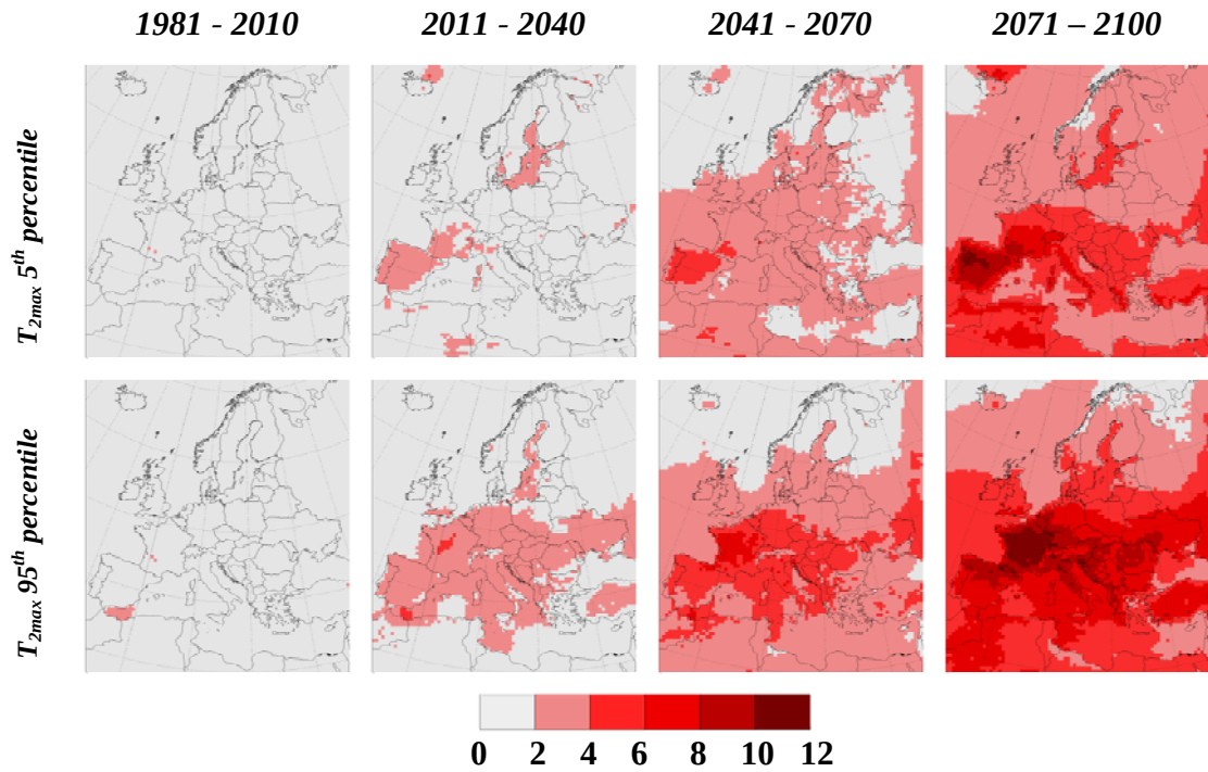
Figure 37. Change in summer T_{2max} extremes in RCA3ECHAM4A2. Units are ^{\circ}\text{C} .
