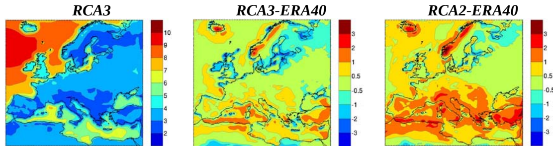
Figure 22. The annual mean 10 m level wind speed according to RCA3 and the corresponding differences between RCA3/RCA2 and ERA40. Units are \text{m s}^{-1} .
