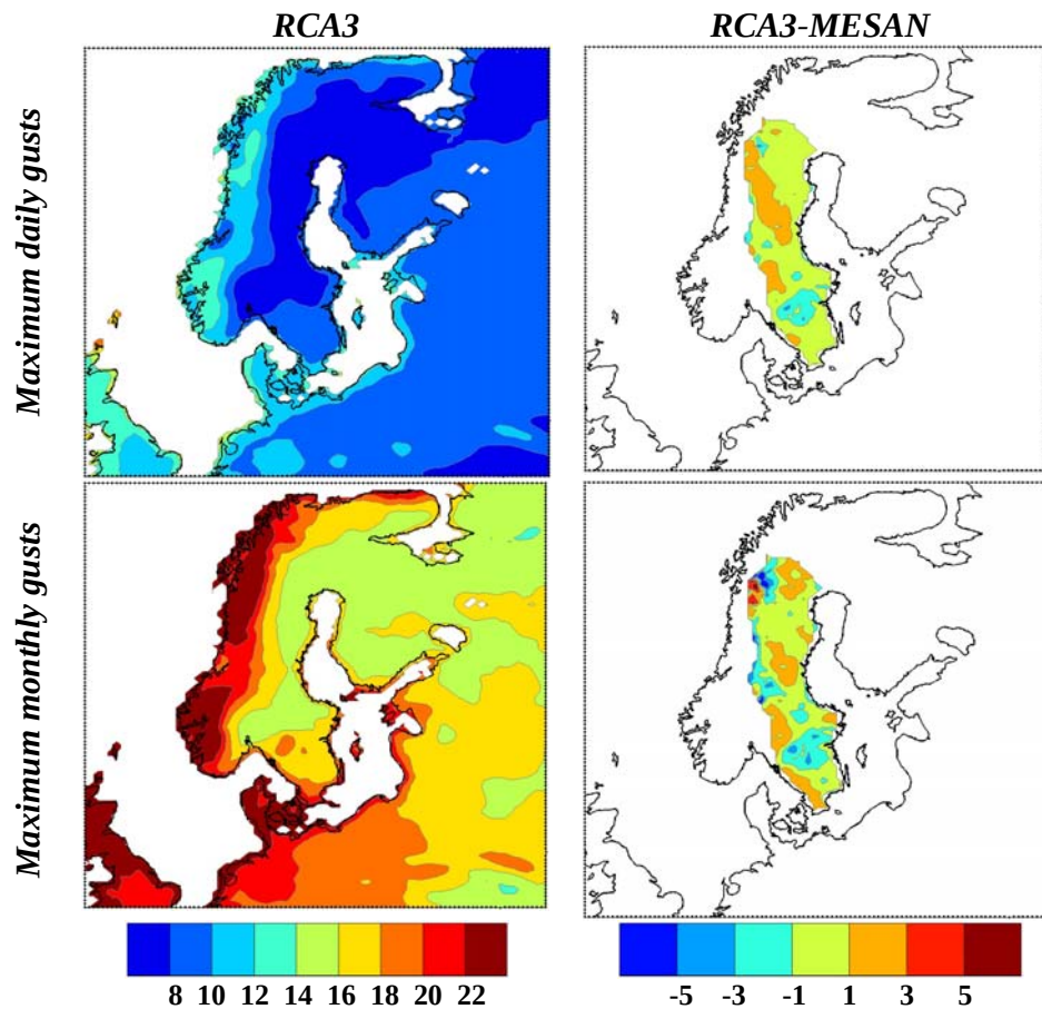
Figure 23. The winter (DJF) maximum daily gusts (top) and maximum monthly gusts (bottom) ( \text{m s}^{-1} ) as mean values over the period 1999-2004 according to RCA3 and the difference between RCA3 and MESAN. Units are \text{m s}^{-1} .
