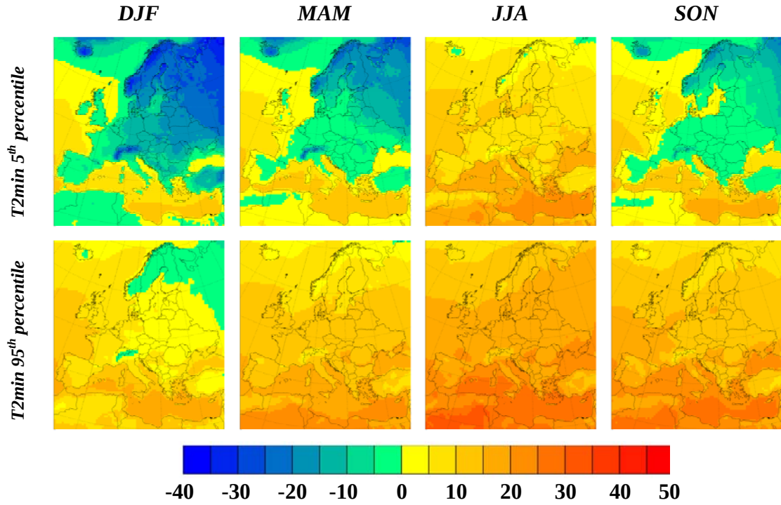
Figure 13. Same as Figure 12 but for daily T_{2min} . Units are ^{\circ}\text{C} .
