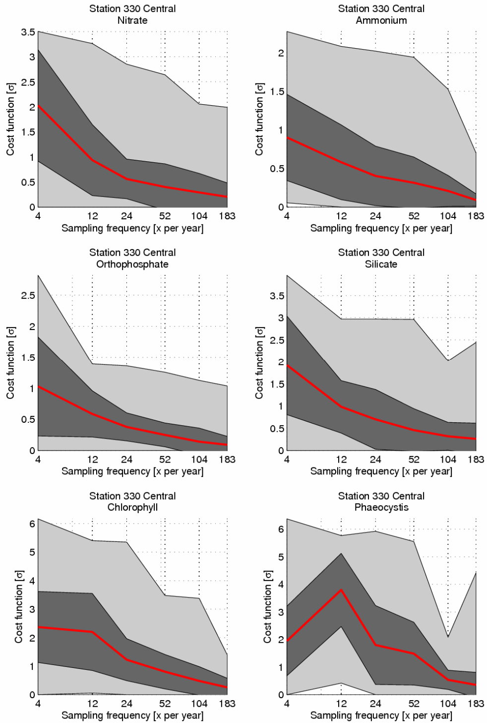
Figure 17 Effect of different sampling strategies on estimates of the maximum concentration (central waters). Light grey indicates the entire range of estimates. Dark grey is the standard deviation of the estimate quality. Red is the mean quality (after 5 tests per sampling frequency, repeated for 10 years of data)
