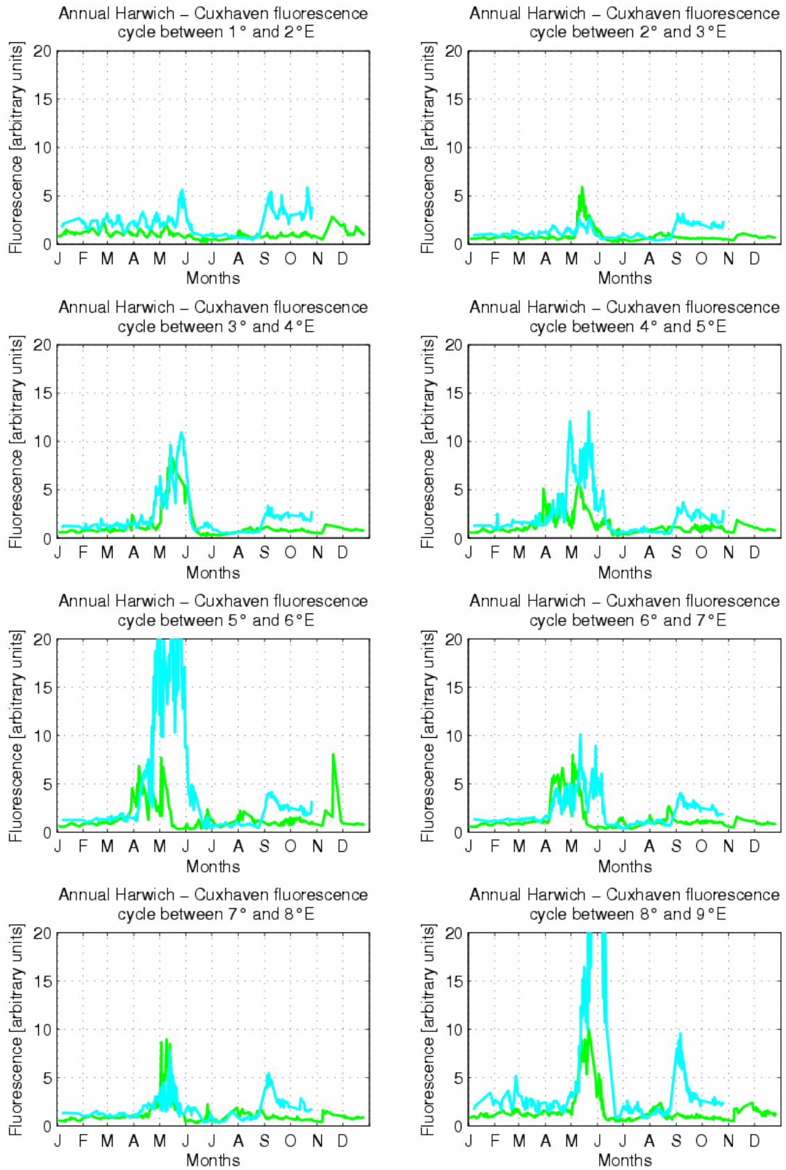
Figure 5 Annual cycles of chlorophyll a fluorescence from the GKSS ferrybox, 2004 & 2005
