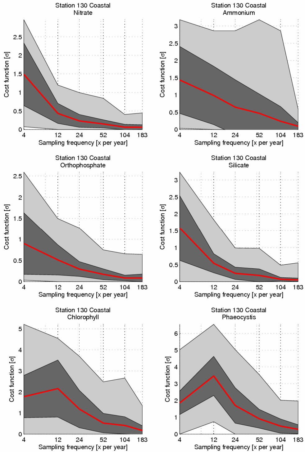
Figure 16 Effect of different sampling strategies on estimates of the maximum concentration (coastal waters). Light grey indicates the entire range of estimates. Dark grey is the standard deviation of the estimate quality. Red is the mean quality (after 5 tests per sampling frequency, repeated for 10 years of data)
