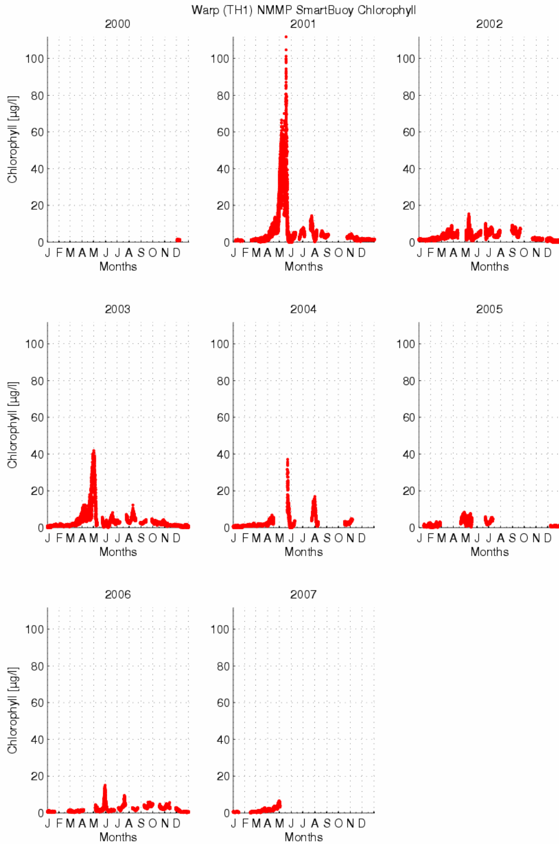
Figure 4 Annual cycles of chlorophyll a concentration, from the CEFAS Smartbuoy at Warp. Data are Crown Copyright.
