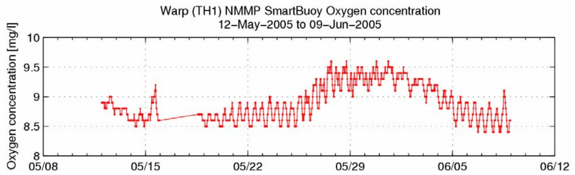
Figure 7 Part of the oxygen time series from Warp, showing the tidal influence. Data are Crown Copyright.
