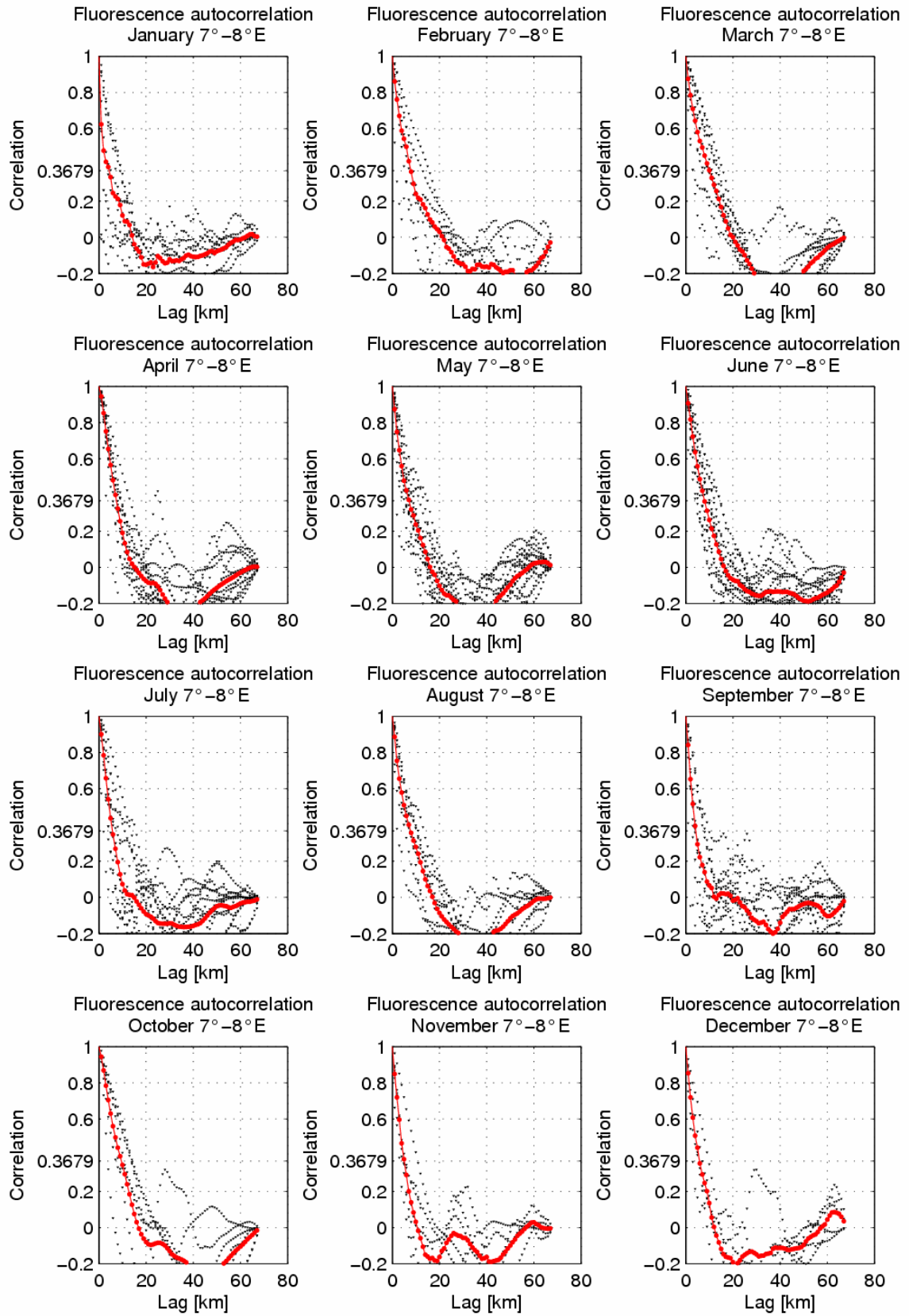
Figure 20 Autocorrelation of chlorophyll fluorescence from GKSS Ferrybox, between 7 & 8°E, January to December
