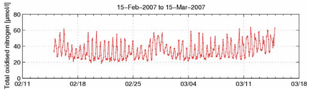
Figure 3 Time series of total oxidised nitrogen, showing the tidal influence on the observations. Data are Crown Copyright
