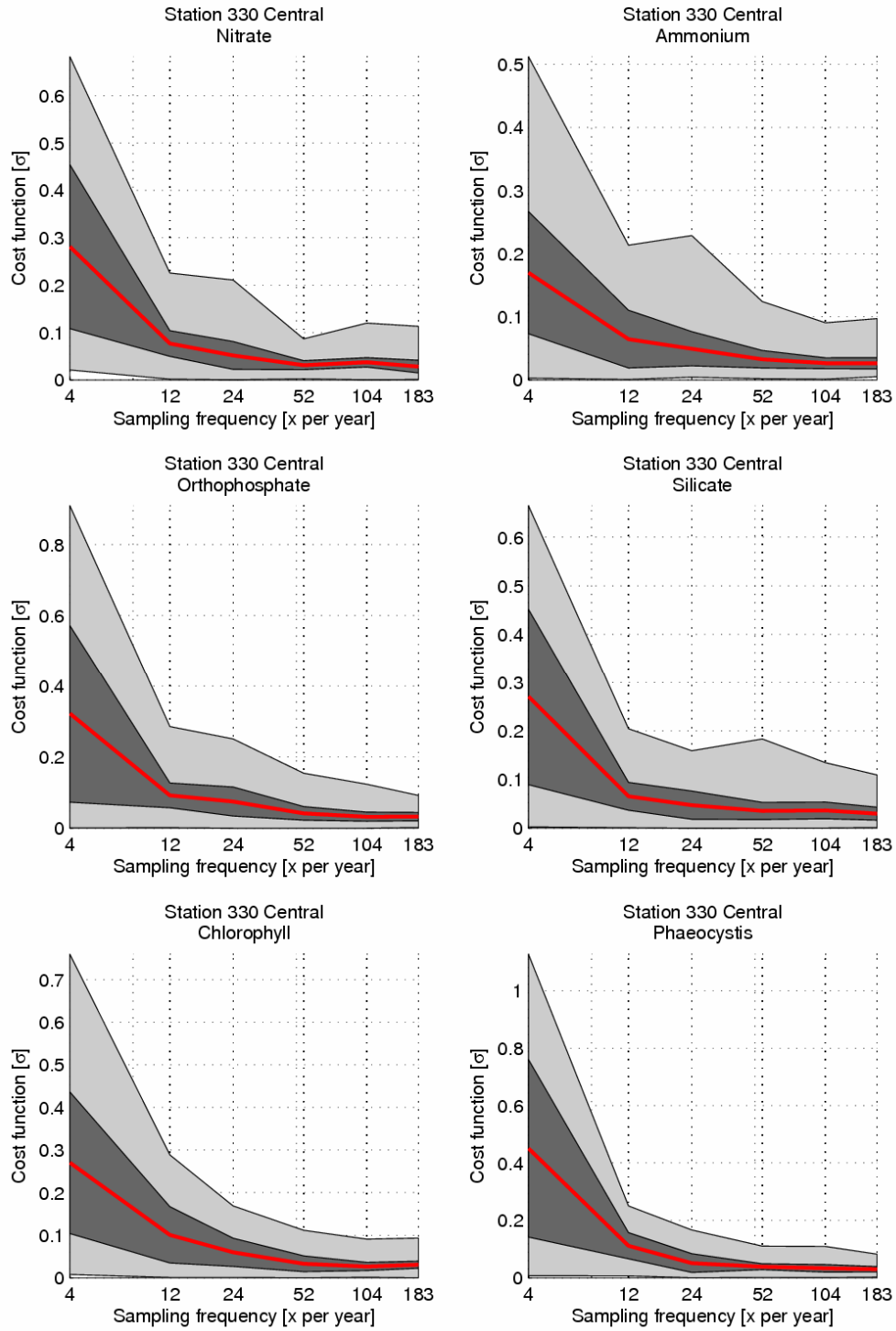
Figure 14 Effect of different sampling strategies on estimates of the mean (Central waters). Light grey indicates the entire range of estimates. Dark grey is the standard deviation of the estimate quality. Red is the mean quality (after 5 tests per sampling frequency, repeated for 10 years of data)
