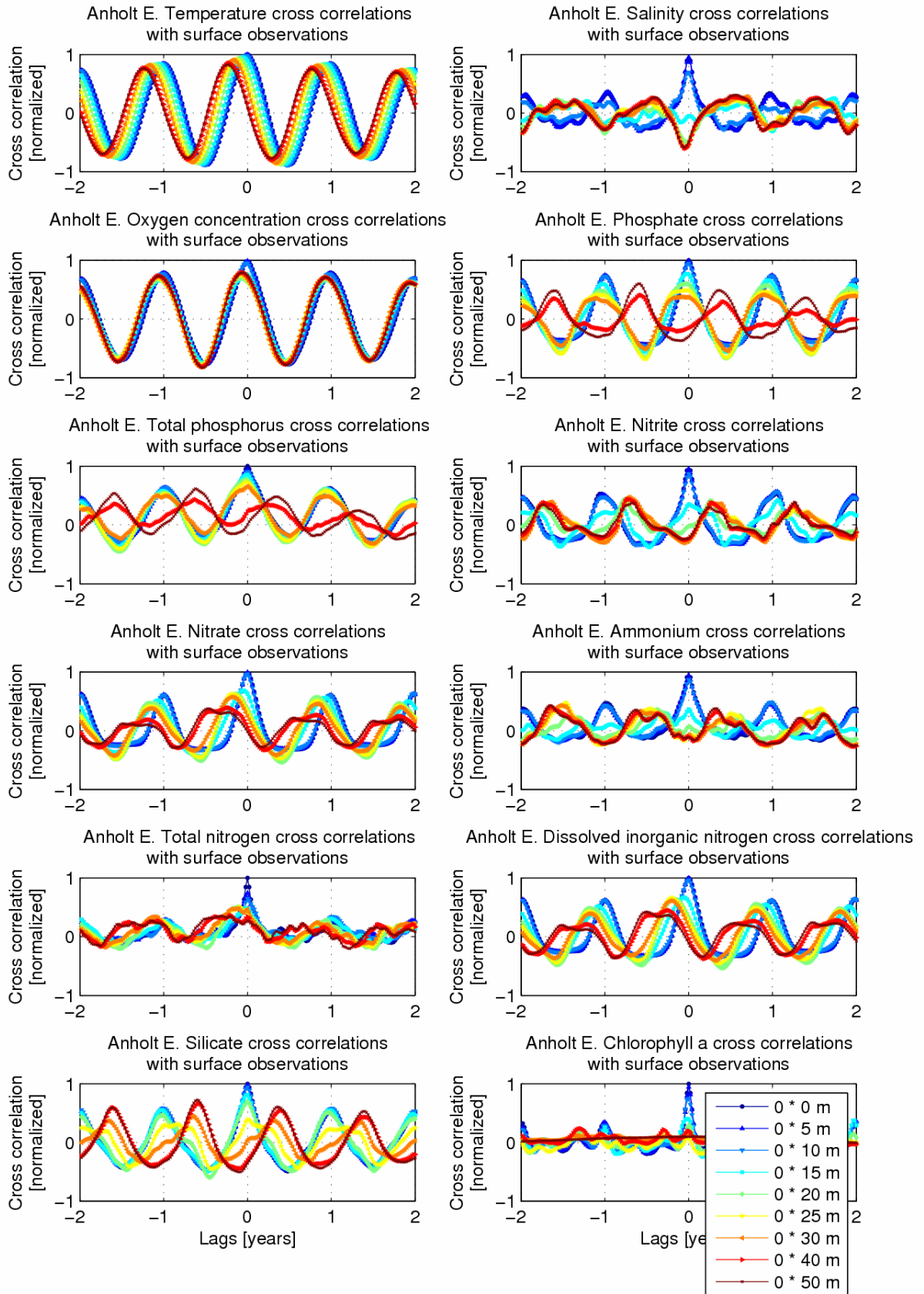
Figure 19 Cross correlations between surface data and data from standard depths, at Anholt E. in the southern Kattegat
