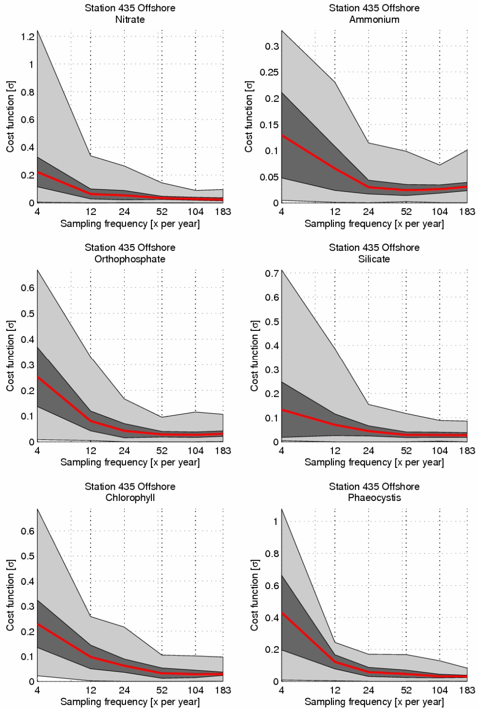
Figure 15 Effect of different sampling strategies on estimates of the mean (offshore waters). Light grey indicates the entire range of estimates. Dark grey is the standard deviation of the estimate quality. Red is the mean quality (after 5 tests per sampling frequency, repeated for 10 years of data)
