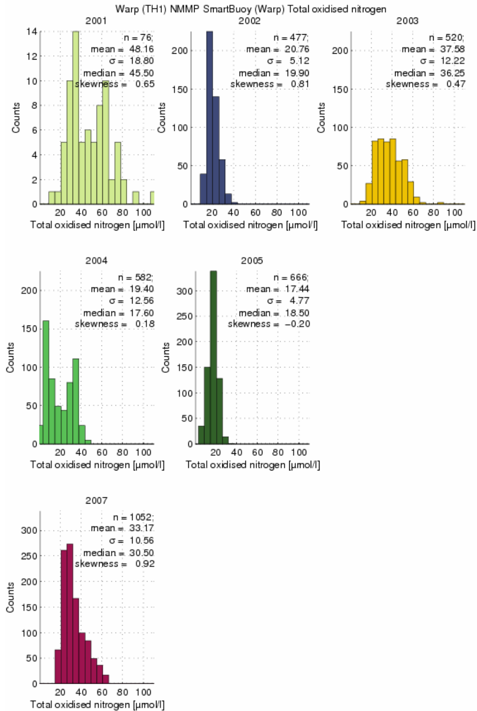
Figure 11 Distribution of winter Total Oxidised Nitrogen at Warp
