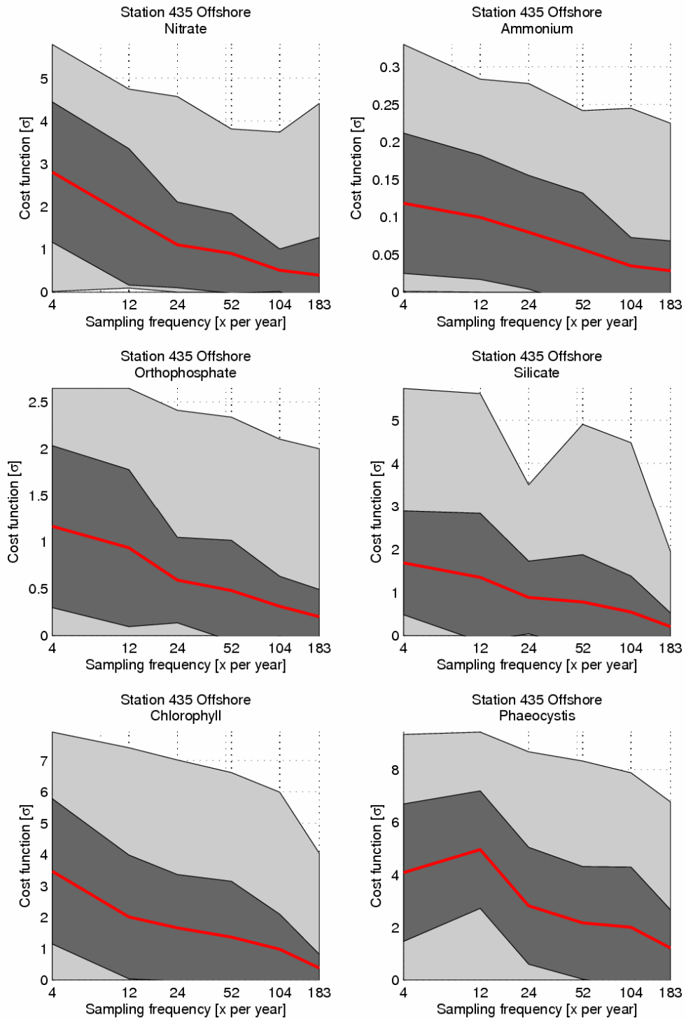
Figure 18 Effect of different sampling strategies on estimates of the maximum concentration (offshore waters). Light grey indicates the entire range of estimates. Dark grey is the standard deviation of the estimate quality. Red is the mean quality (after 5 tests per sampling frequency, repeated for 10 years of data)
