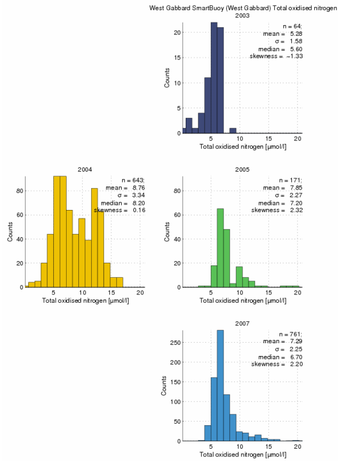
Figure 10 Distributions of Total Oxidised Nitrogen during winter at West Gabbard
