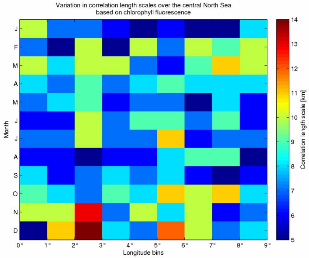
Figure 21 Summary of variation in correlation lengths by longitude and month, based on GKSS ferrybox chlorophyll
