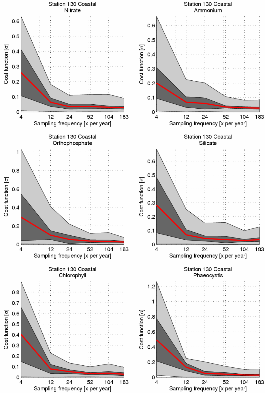
Figure 13 Effect of different sampling strategies on estimates of the mean (Coastal waters). Light grey indicates the entire range of estimates. Dark grey is the standard deviation of the estimate quality. Red is the mean quality (after 5 tests per sampling frequency, repeated for 10 years of data)
