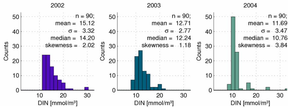
Figure 9 Distributions of offshore winter DIN 2002 - 2004. Belgian data
