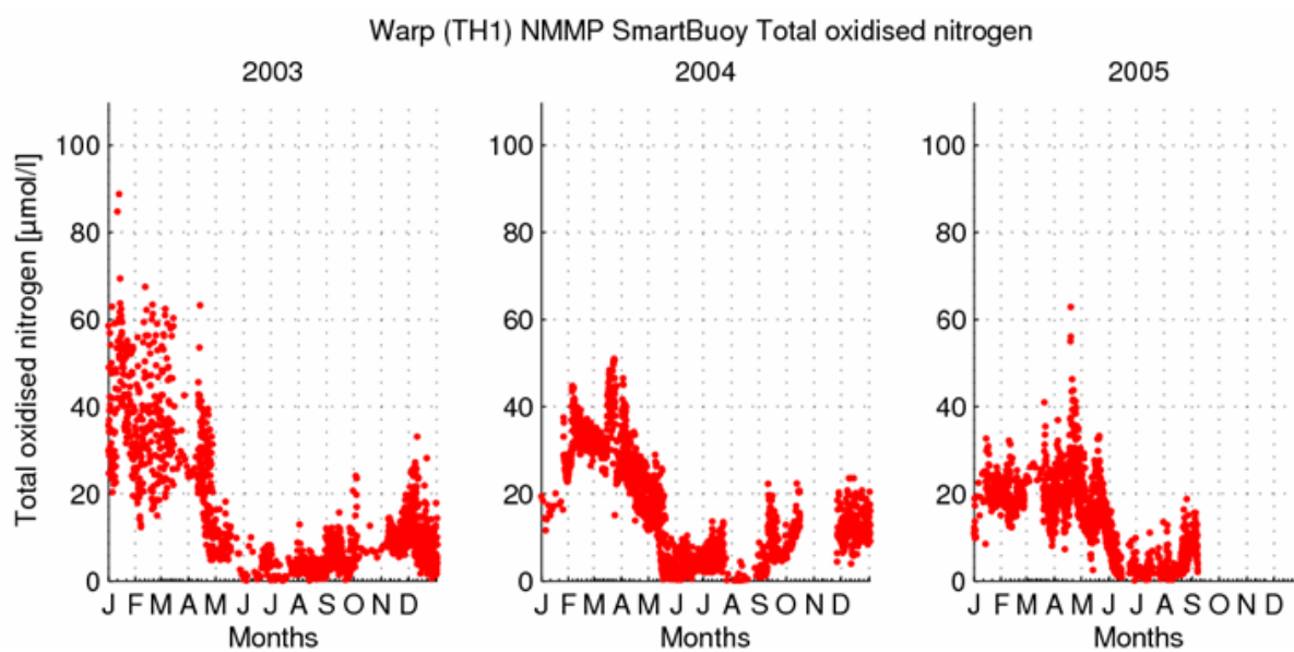
Figure 2 Annual cycles of total oxidised nitrogen ( \Sigma nitrite + nitrate) observed by the CEFAS Smartbuoy at Warp. These data are Crown Copyright.
