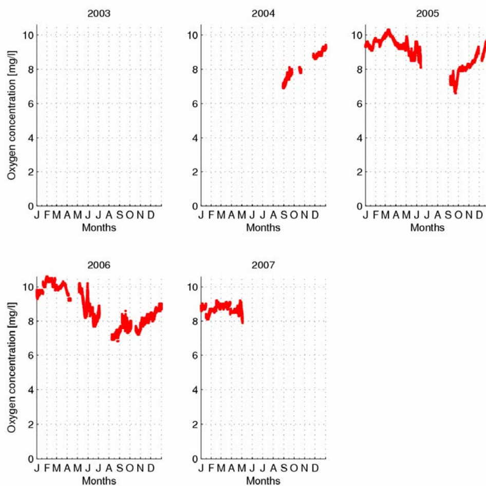
Figure 6 Annual cycles of oxygen at 1 m depth, from CEFAS Smartbuoy at Warp. These data are Crown Copyright.
