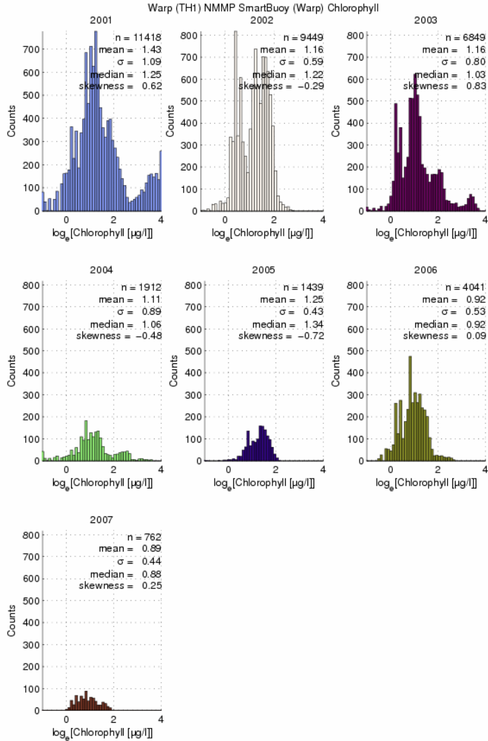
Figure 12 Distribution of the \log_e chlorophyll concentrations from Warp
