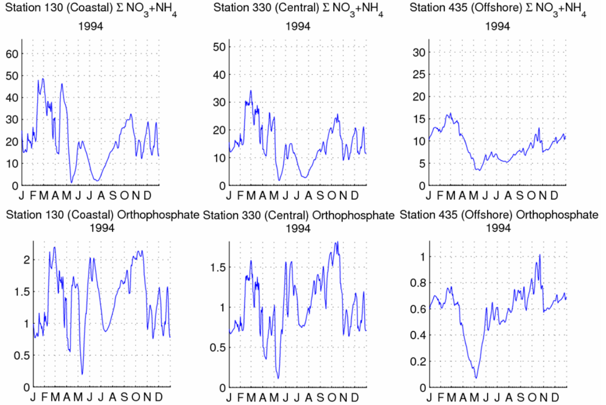
Figure 1 Nutrient cycles (the sum of nitrate and ammonium and DIP) for coastal, central and offshore Belgian waters, 1994. Concentration units are \text{mmol/m}^3
