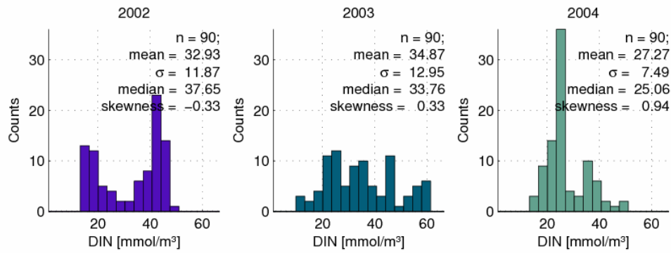
Figure 8 Distributions of winter inshore DIN concentrations, 2002 - 2004. Belgian data
