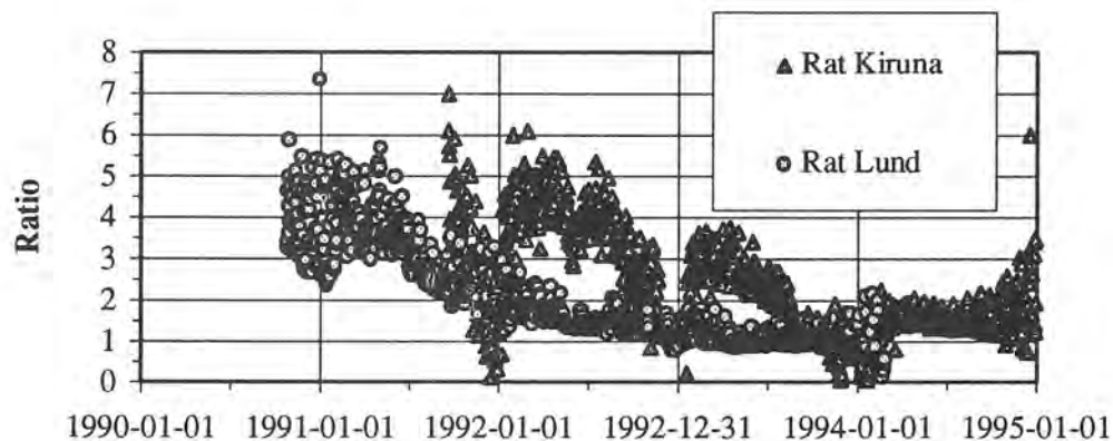
Figure 3.2.1 Ratio of daily values of Solar Light Model 500 UV-A Meter over global radiation recorded in Kiruna and Lund as a function of the time. Plotted to illustrate the decrease of the responsivity of the UV-A meters.
