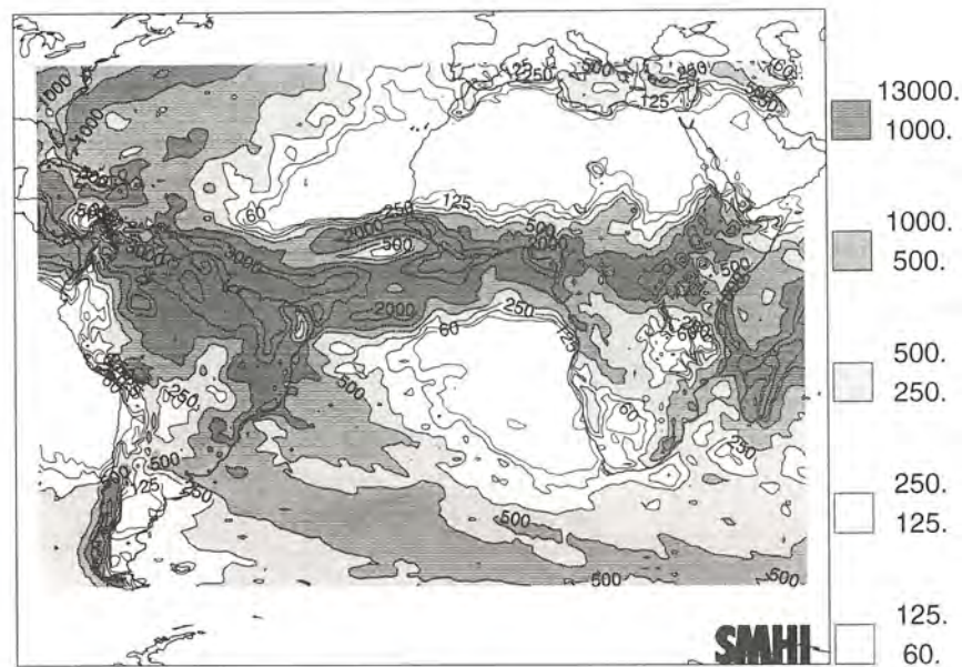
Fig. 4. Accumulated precipitation from used ECMWF weather data, and scaled to represent annual precipitation ( \text{mm yr}^{-1} ).
