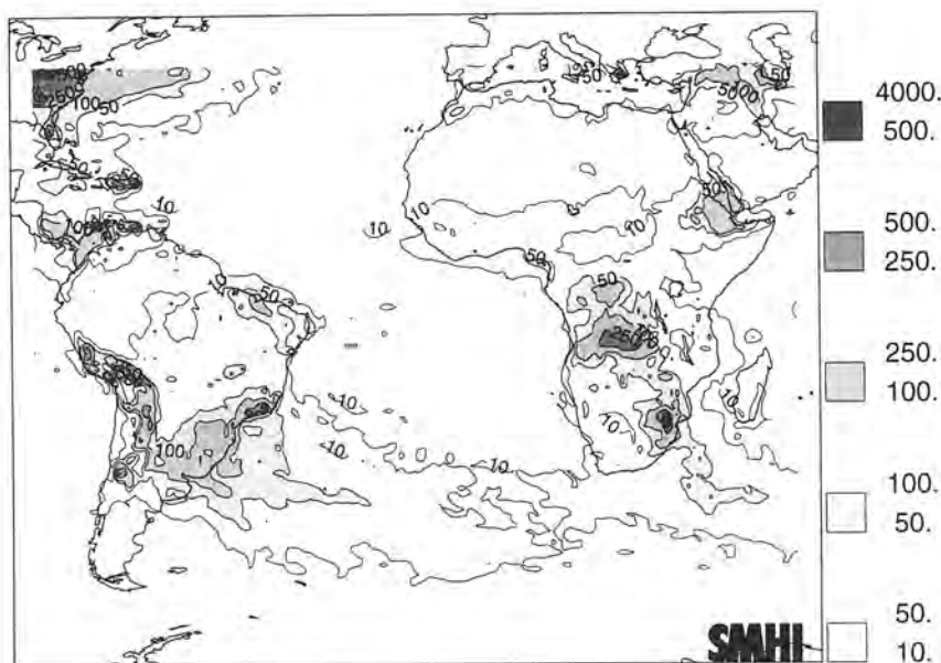
Fig. 10. Annual wet deposition of sulfur in \text{mg S m}^{-2}
