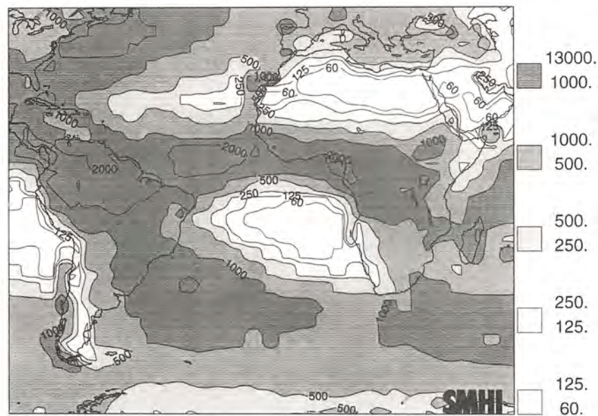
Fig. 5. Annual precipitation estimates for 1988 (Rudolf, 1993)
