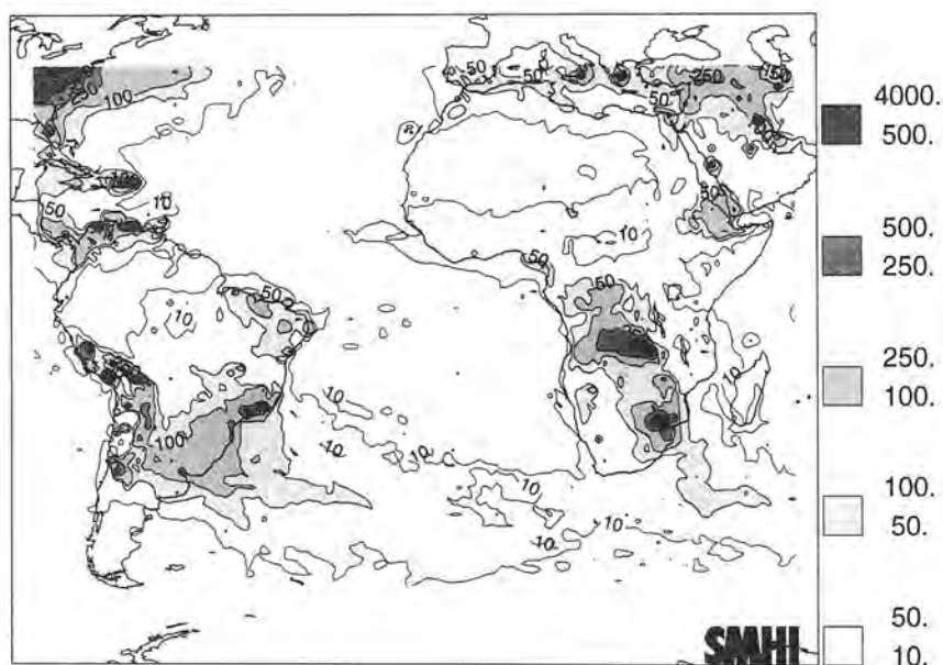
Fig. 11. Annual total deposition of sulfur in \text{mg S m}^{-2}
