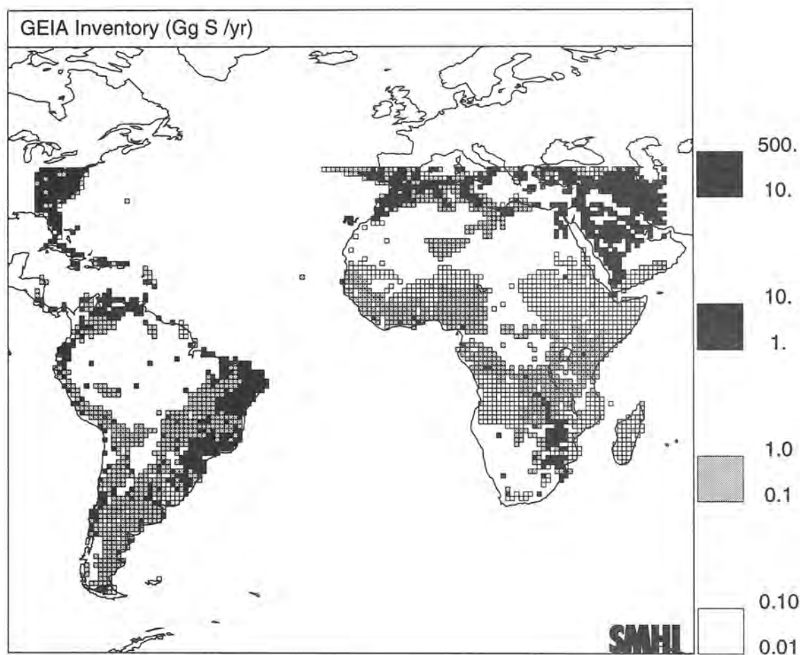
Fig. 2. Anthropogenic emissions used on 1^\circ \times 1^\circ resolution ( \text{Gg S yr}^{-1} ). Based on the GEIA inventory (Benkowitz, 1993).
