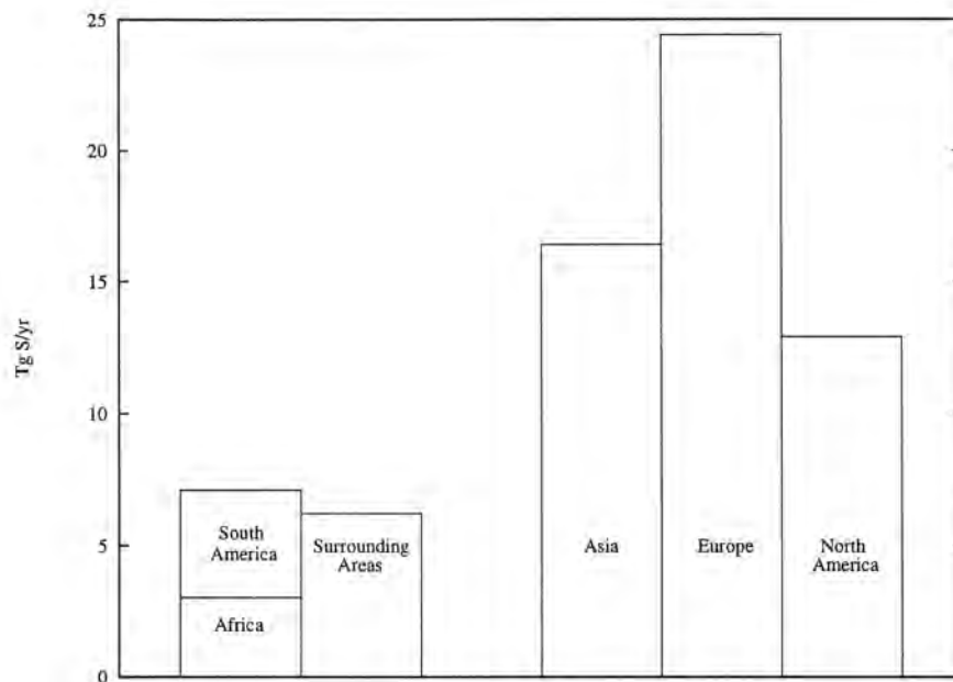
Fig. 3. Emission budgets for Africa and South America and surrounding areas (S-E USA, Mediterranean area, Middle East and Saudi Arabia) used in the simulations. For comparison emissions for Asia shown (50 °E - 160 °E, 30 °S - 50 °N), Europe and North America is shown. Based on the GEIA inventory (Benkovitz, 1993).
