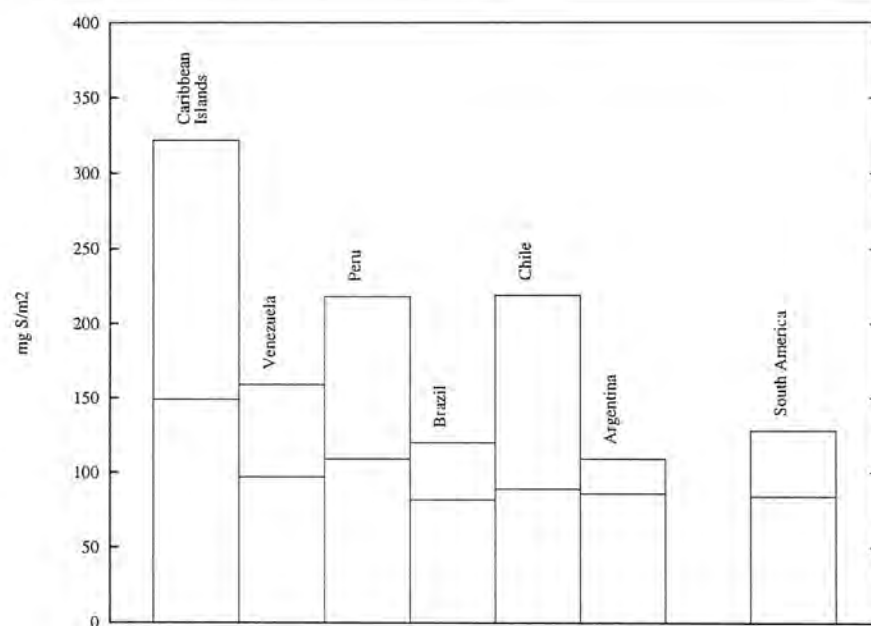
Fig. 7. Box diagram of the mean deposition for a sample of countries in South America, together with the areal mean deposition for the whole continent (the rightmost box) in \text{mg S m}^{-2} . Each box is divided into two parts denoting wet deposition (bottom) and dry deposition (top). Note the different scale from previous figure.
