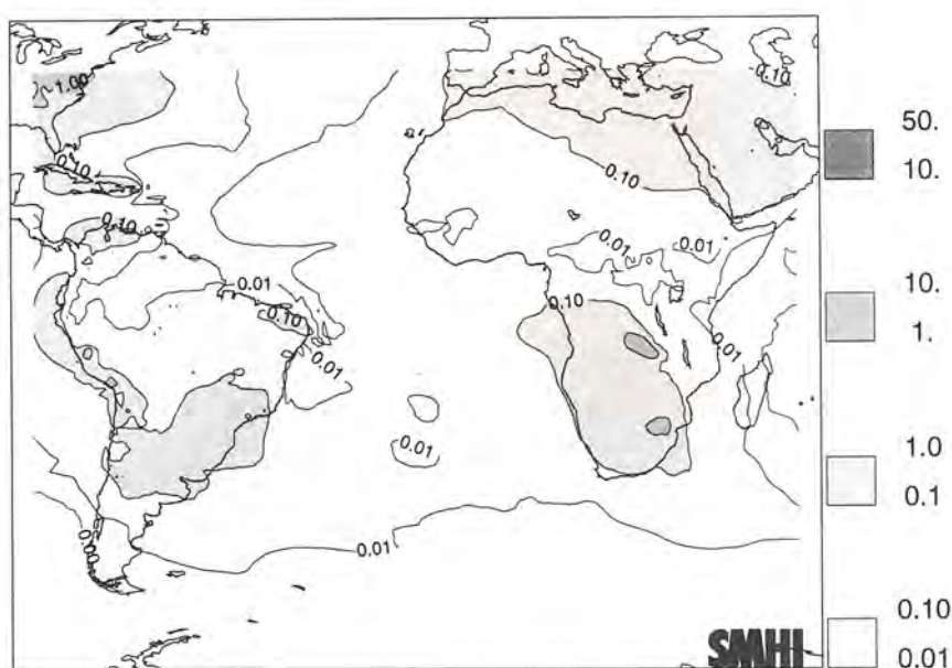
Fig. 9. Annual mean concentration of \text{SO}_4^{2-} in \mu\text{g S m}^{-3} .
