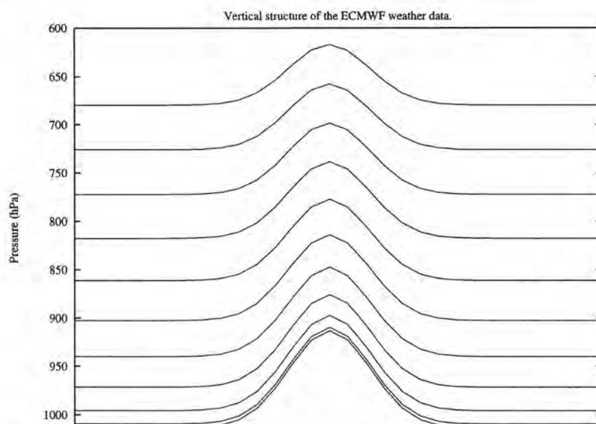
Fig. 1. Approximate heights to various model levels as defined by the ECMWF input weather data. Heights are given as pressure levels (hPa). The lowest contour assumes the ground surface.
