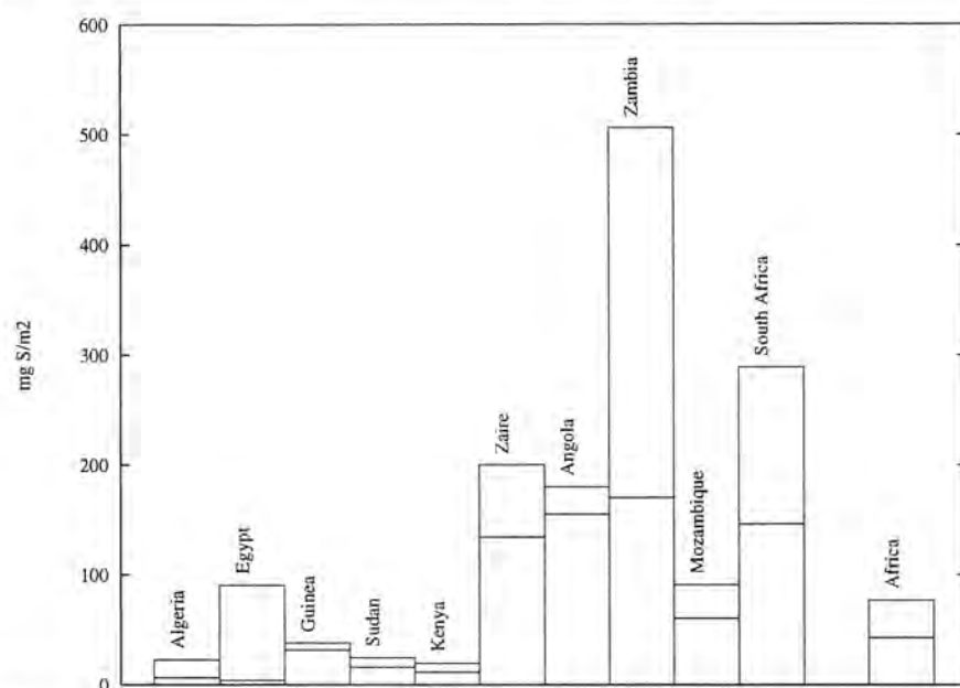
Fig. 6. Box diagram of the areal mean deposition for a sample of countries in Africa, together with the areal mean deposition for the whole continent (the rightmost box) in \text{mg S m}^{-2} . Each box is divided into two parts denoting wet deposition (bottom) and dry deposition (top).
