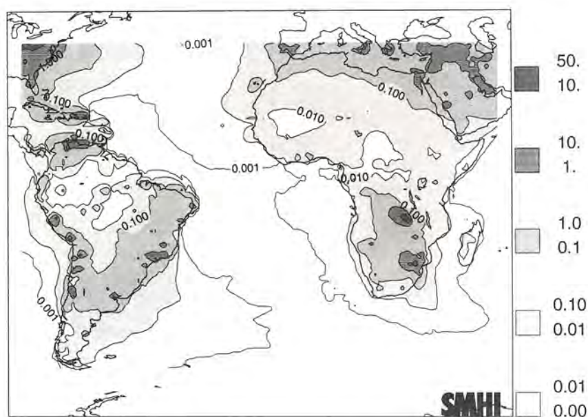
Fig. 8. Annual mean concentration of \text{SO}_2 in \mu\text{g S m}^{-3} .
