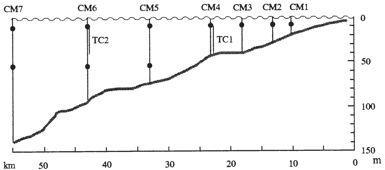
Figure 3.2. The moorings at the Rauma transect.
