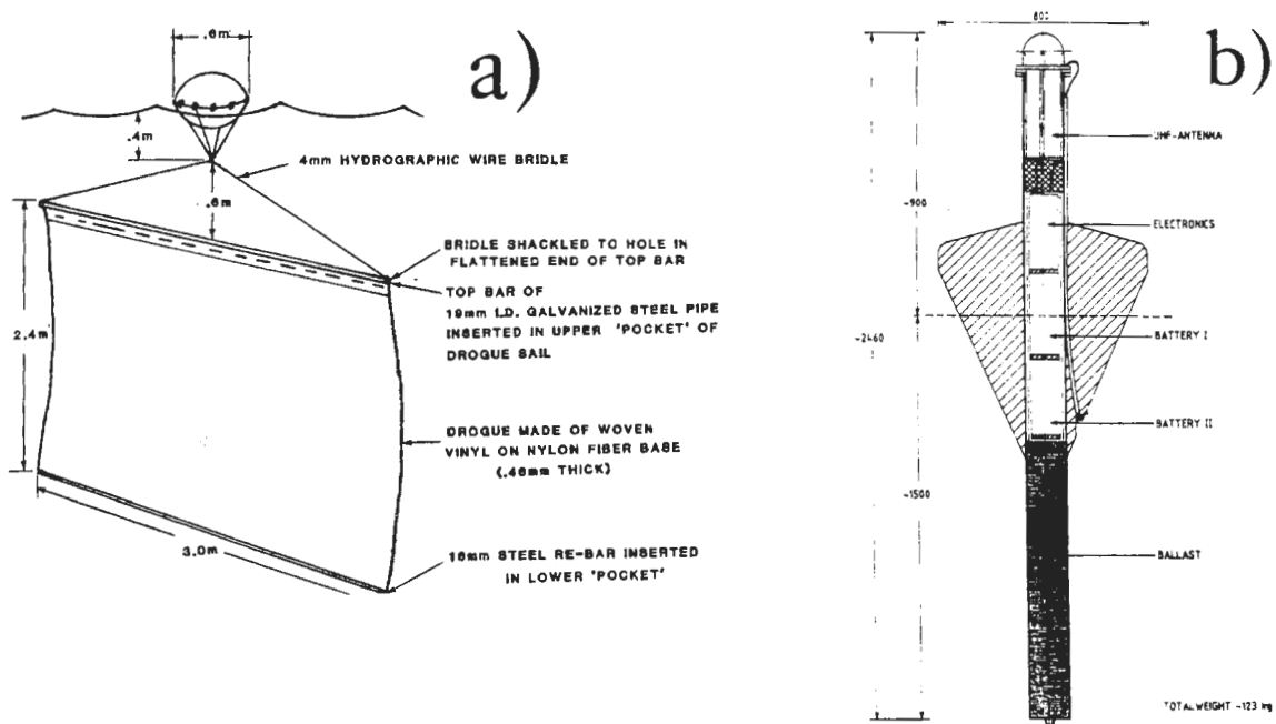
Figure 5.2. Overall sketch of the buoy types used (in different scale). The drogue for the Norwegian buoy in b) is the same as for a).
