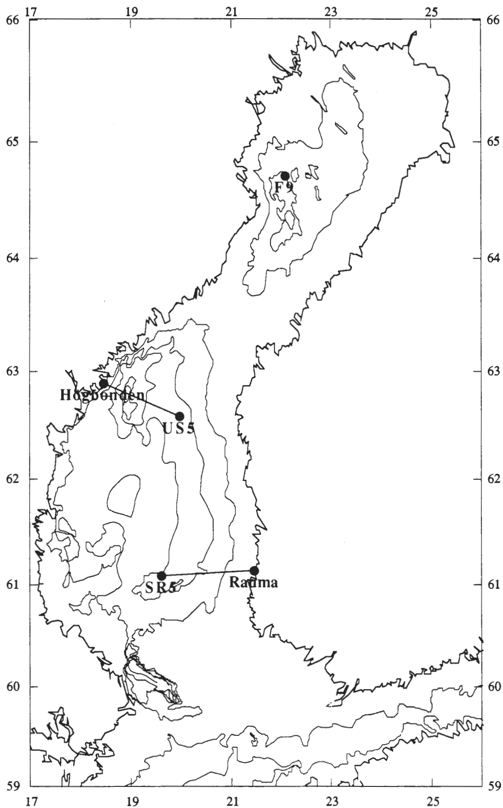
Figure 4.1. Chart of the Gulf of Bothnia with measurement transects for current meter moorings.
