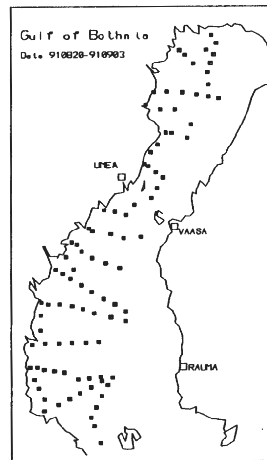
Figure 7.3. Hydrographical stations visited by the R/V Argos, August - September 1991.
