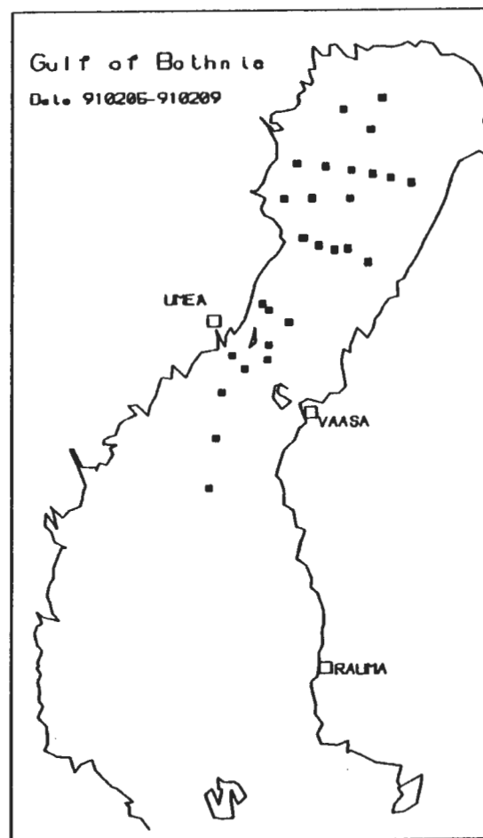
Figure 7.5. Hydrographical stations visited by the ice- breaker Ymer, February 1991.
