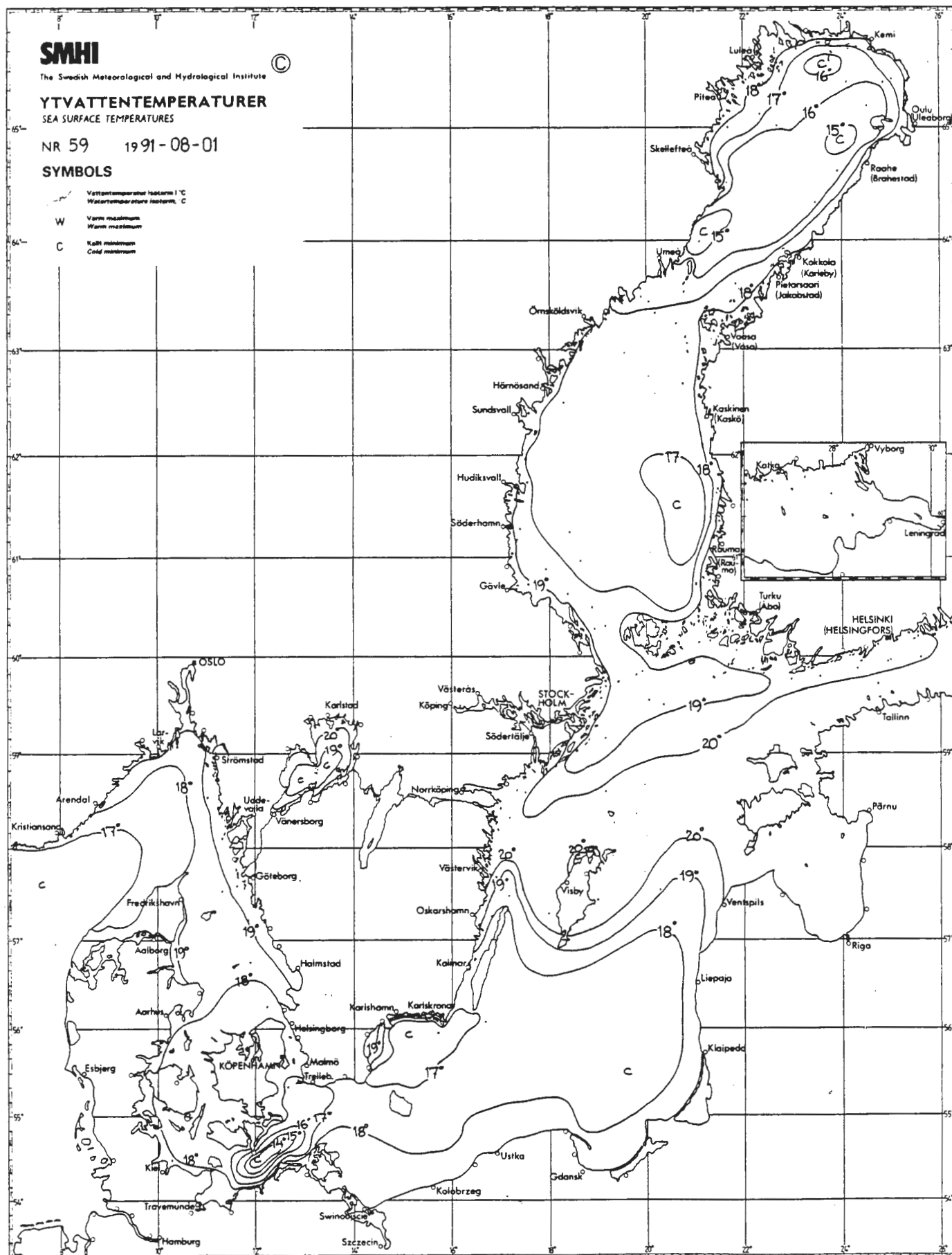
Figure 9.7. Typical sea surface temperature during the end of the summer of 1991, observed on August 1, 1991.
