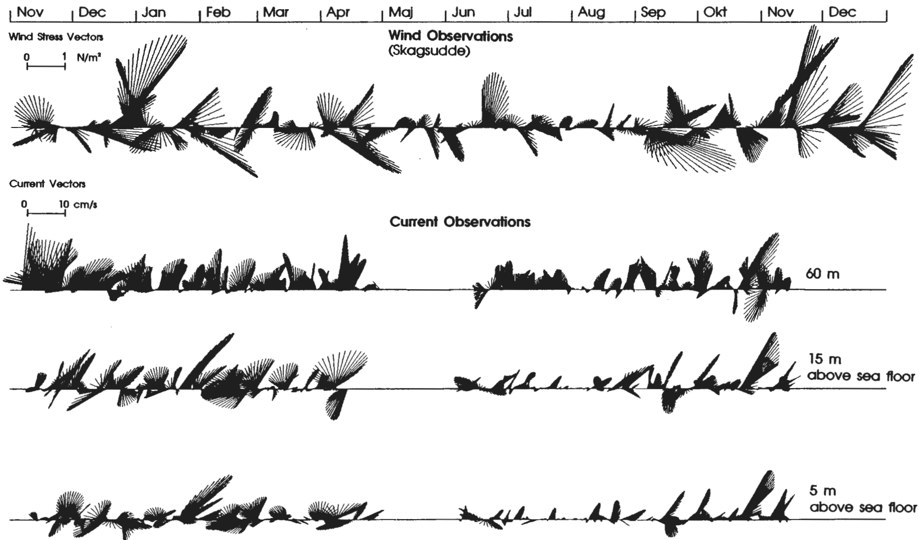
Figure 2.9b. Time series vector plots of wind and current data of the Open Sea station in the Bothnian Sea, US5B. The data have been filtered with a low-pass filter with 18 to 24 hour cutoff.
