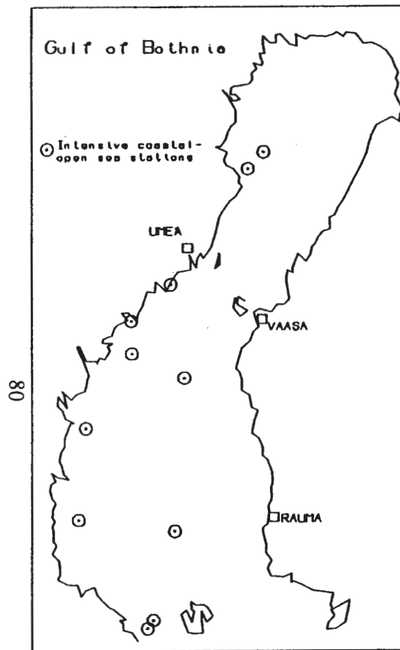
Figure 7.7. Hydrographical stations which were visited more than 10 times during 1991, i.e. intensive stations.
