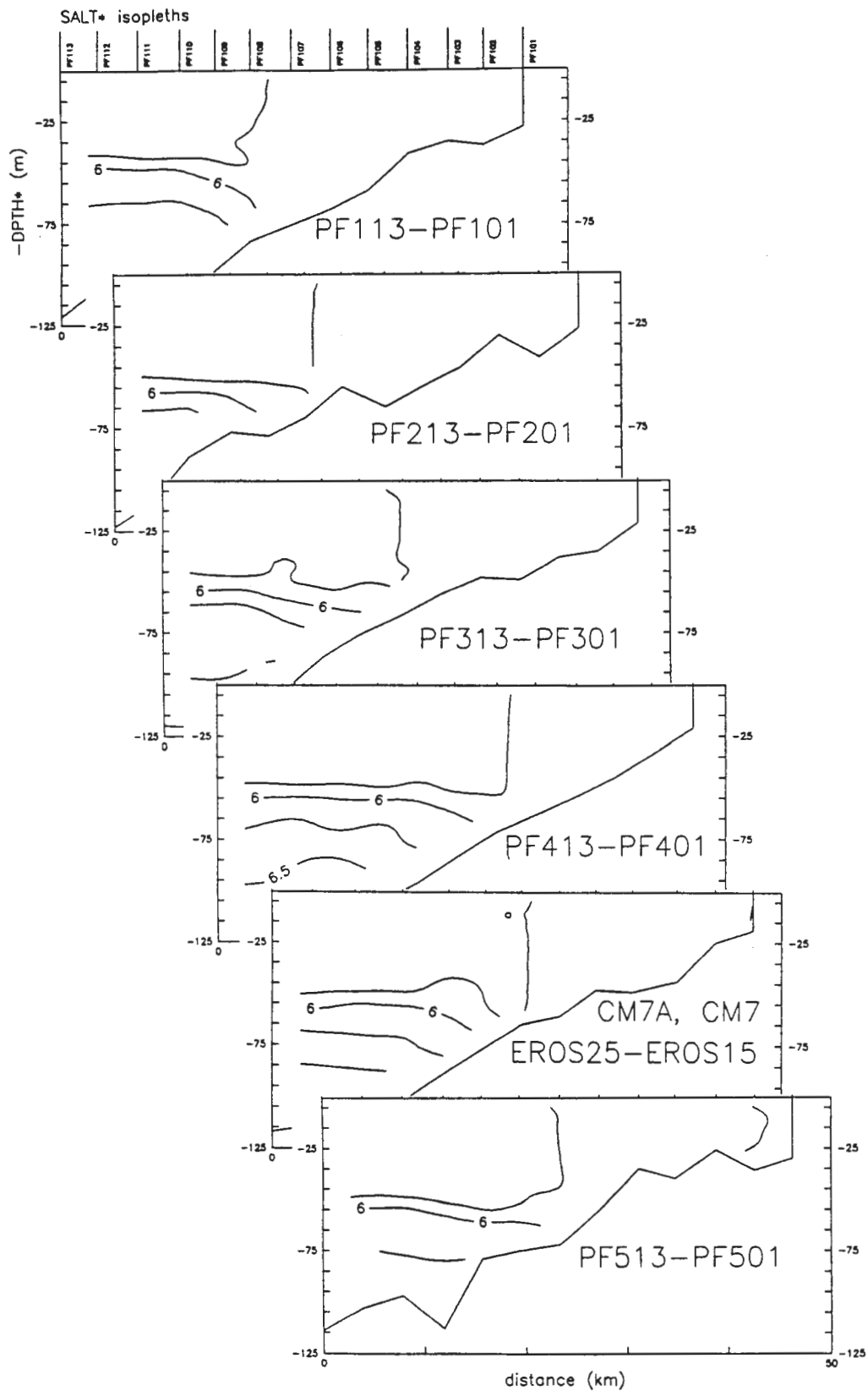
Figure 8.8. Salinity distribution in the coastal grid near the Finnish coast, November, 1991.
