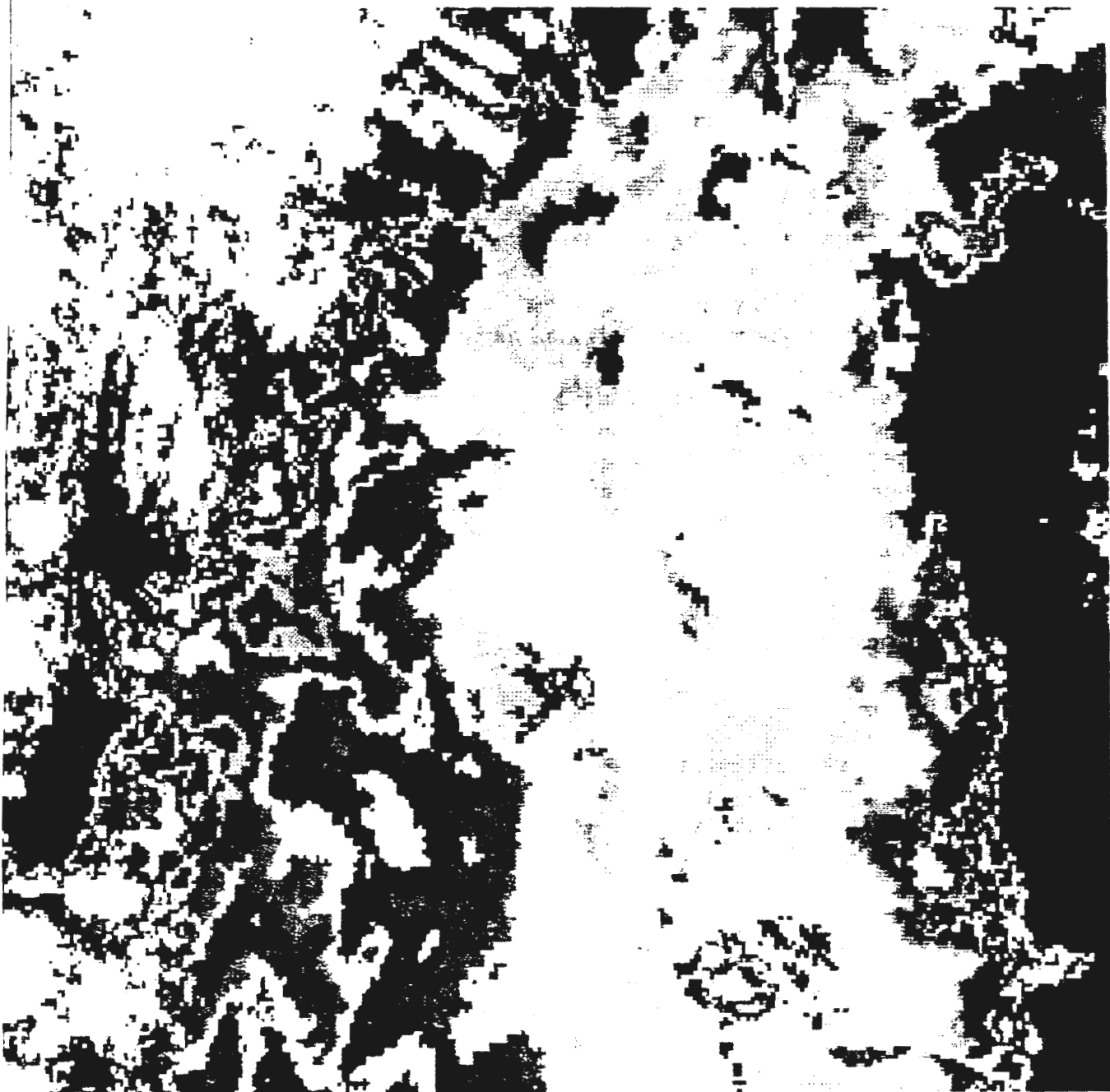
Figure 6.4. High resolution brightness temperature image from August 14, covering the northern part of the Bothnian Sea.
