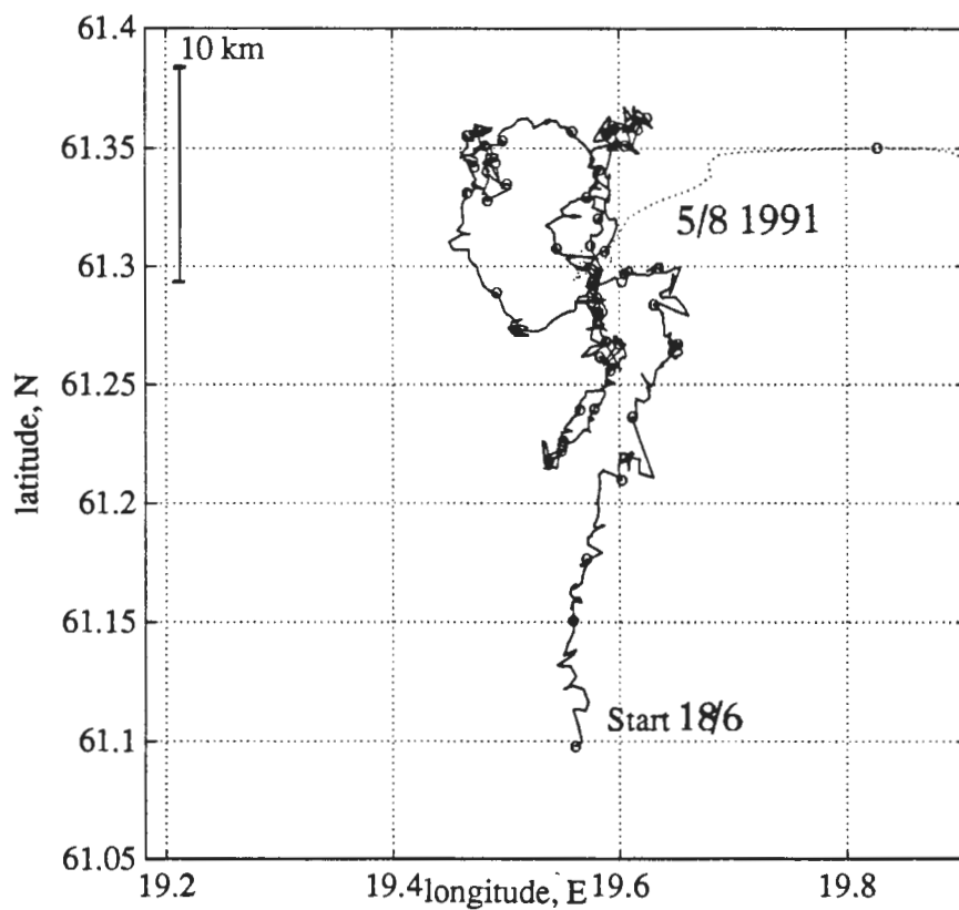
Figure 5.10. Trajectory of the deep water experiment. Most of the drift at the end of the experiment after August 5 (dotted line) was scaled out of the figure. Positions with daily intervals are given as circles.
