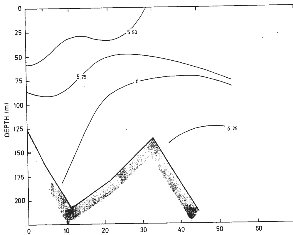
Figure 7.36. Salinity distribution along the US section, August.
