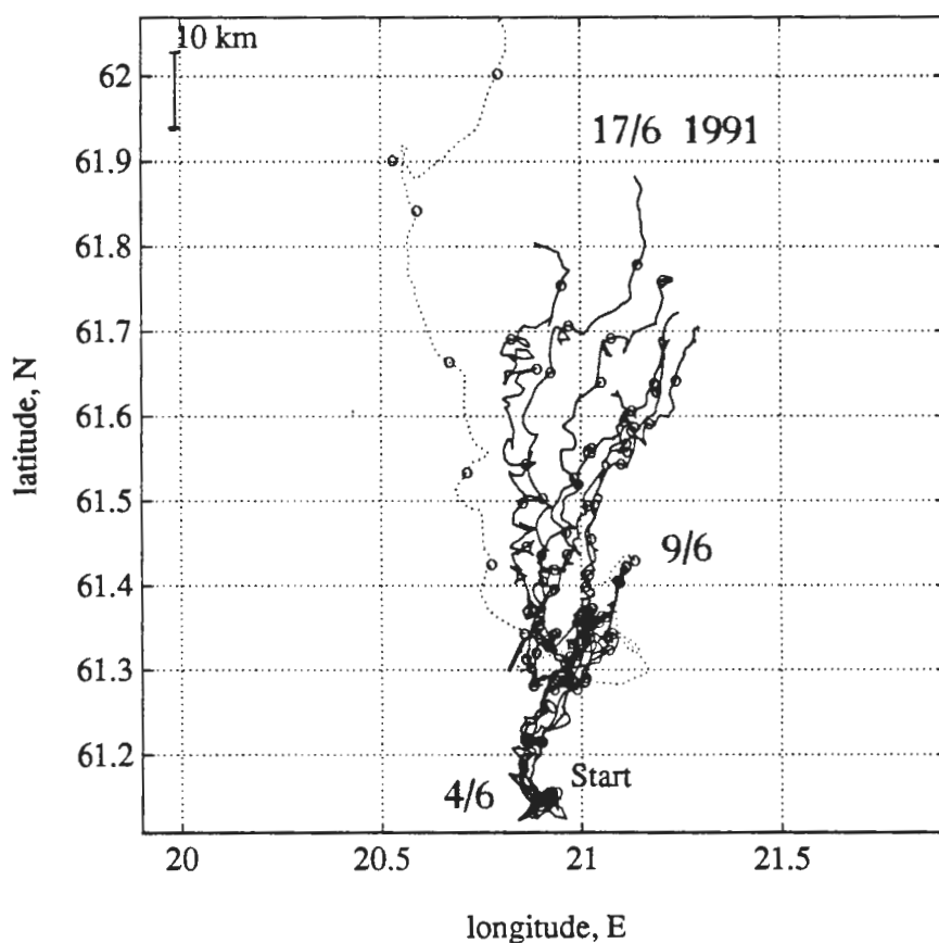
Figure 5.6. Drifter trajectories for the Cluster Experiment 1; positions with daily intervals are given as circles. Dotted line indicates suspectable data. The scale is given in the figure.
