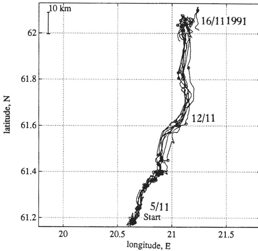
Figure 5.7. Drifter trajectories for the Cluster Experiment 2; positions with daily intervals are given as circles.
