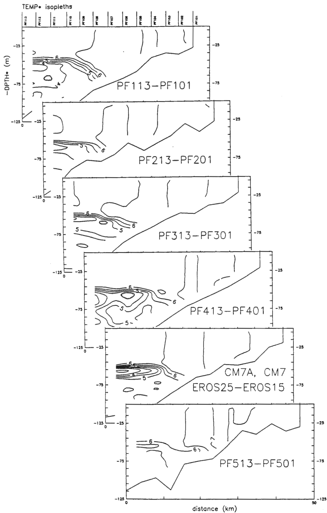
Figure 8.7. Temperature distribution in the coastal grid near the Finnish coast, November, 1991.
