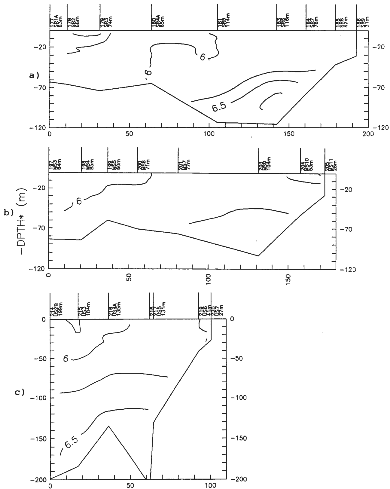
Figure 8.6. Salinity distribution along a) US section, b) MS section and c) SR section, June, 1991.
