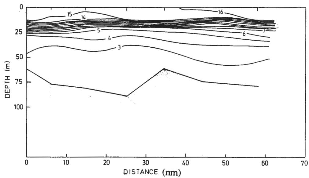
Figure 7.27. Temperature distribution along the MS section, August.
