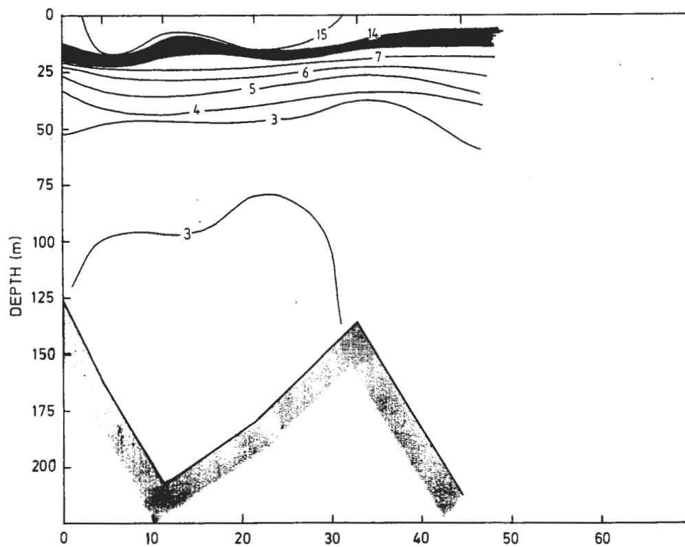
Figure 7.32. Temperature distribution along the US section, May - June.
