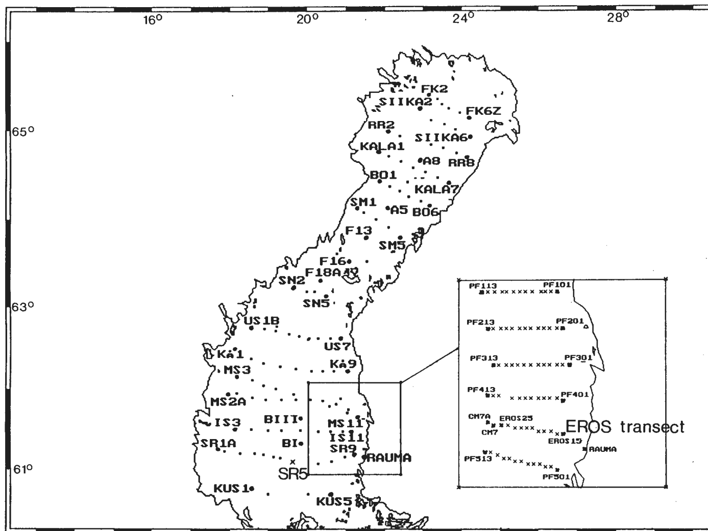
Figure 8.1. Finnish CTD stations during the GB-91 Year. The first and last station name of the transect presented. The coastal grid is shown in the small picture.
