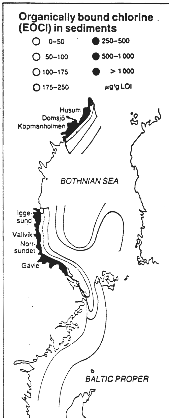
Figure 1.1. Organically bound chlorine (EOCI) in sediments. (From Håkansson et al., 1988, Swedish Environ. Prot. Agency, Report 3522.)
