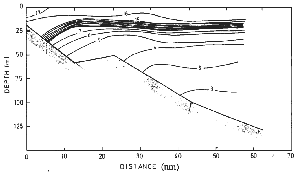
Figure 7.21. Temperature distribution along the GBY1 section, August.
