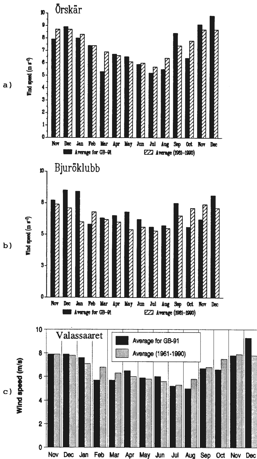
Figure 9.4. Monthly average wind speed from a) the Örskär, b) the Bjuröklubb and c) the Valassaaret stations during the GB-91 compared to the 30-year period.
