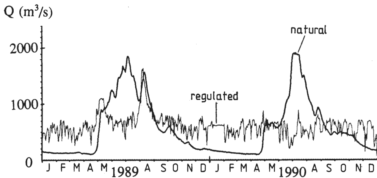
Figure 9.11. Example of the influence of regulation on the flow in the River Luleälven at Boden (24 488 km 2 ) near the outlet into the Baltic Sea. Thick curve: Reconstructed natural. Thin curve: Recorded regulated.
