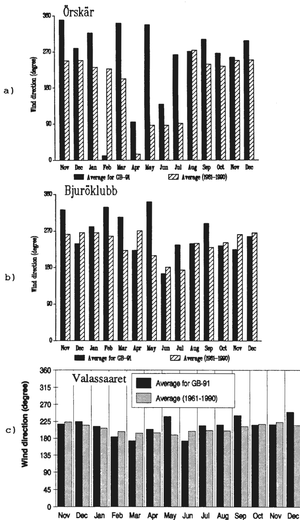
Figure 9.5. Monthly average wind direction from a) the Örskär, b) the Bjuröklubb and c) the Valassaaret stations during the GB-91 compared to the 30-year period.
