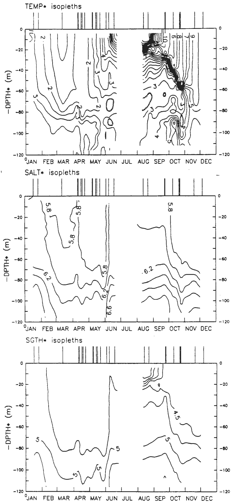
Figure 8.2. Seasonal (upper) temperature, (middle) salinity and (lower) density variation at SR5 in the southern Bothnian Sea. The observation dates are marked with a vertical line on the top of the picture.
