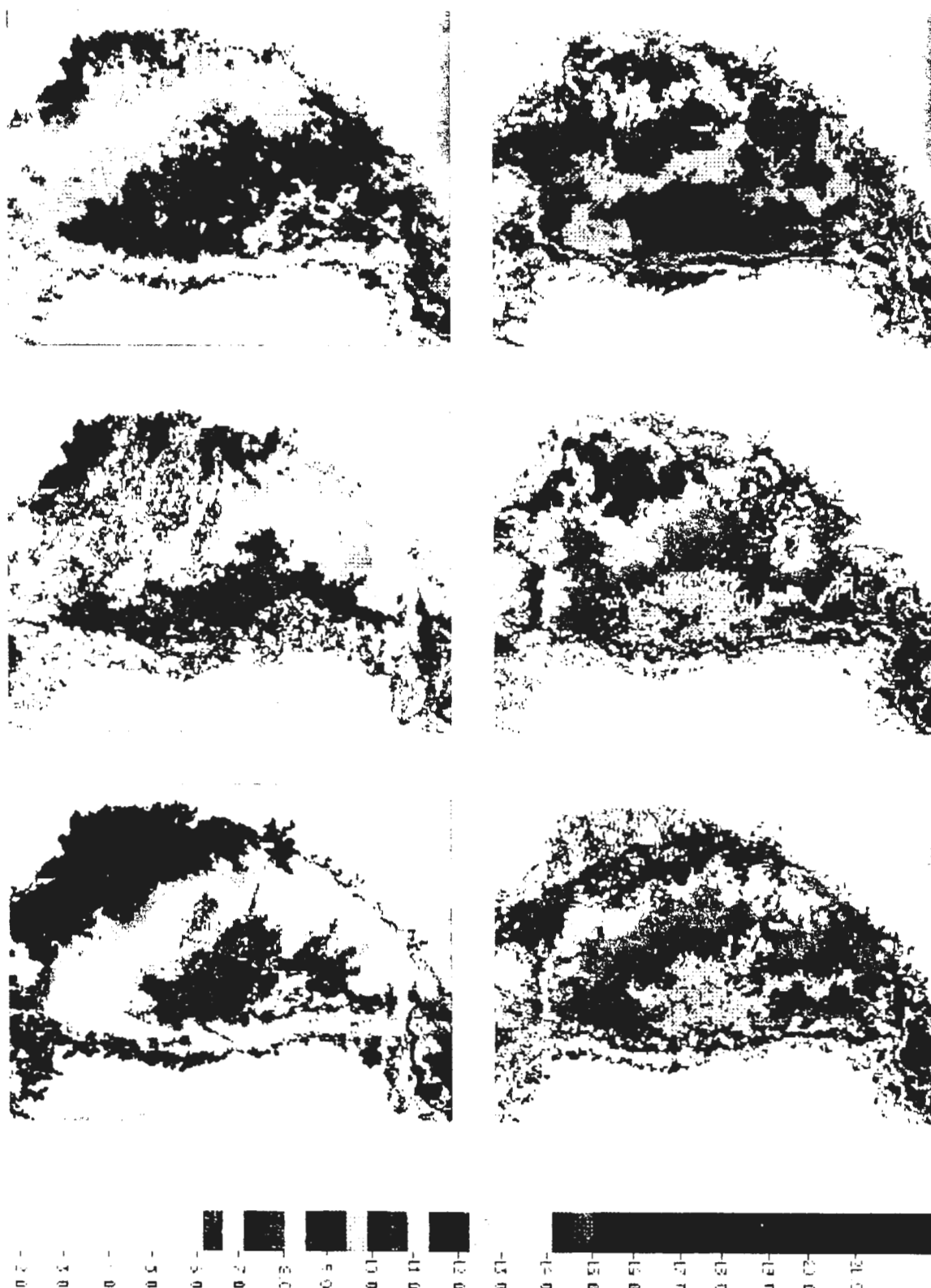
Figure 6.3. Time series of brightness temperature images from July 3 to 8, 1991.
