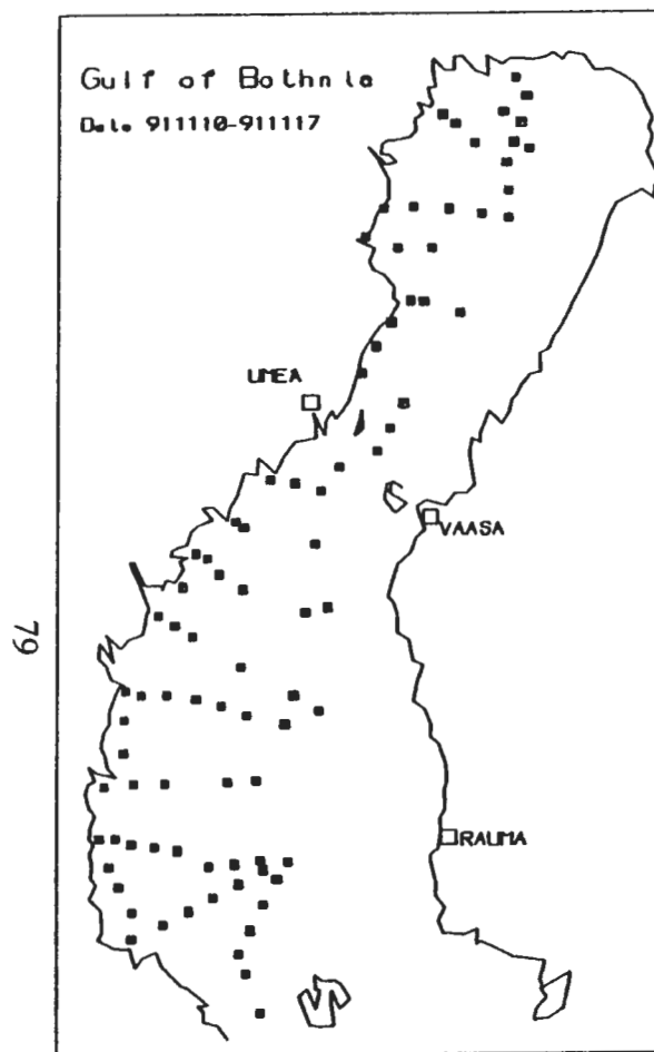
Figure 7.4. Hydrographical stations visited by the R/V Argos, November 1991.
