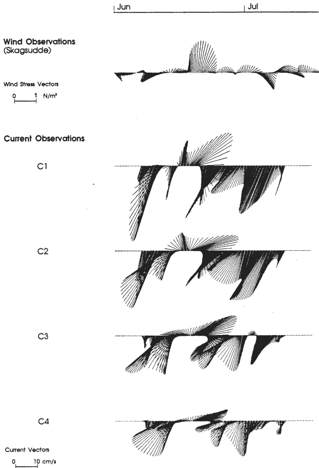
Figure 2.5. Time series vector plots of wind and current meter data of the Högbonden transect. The data have been filtered with a low-pass filter with 18 to 24 hour cutoff.
