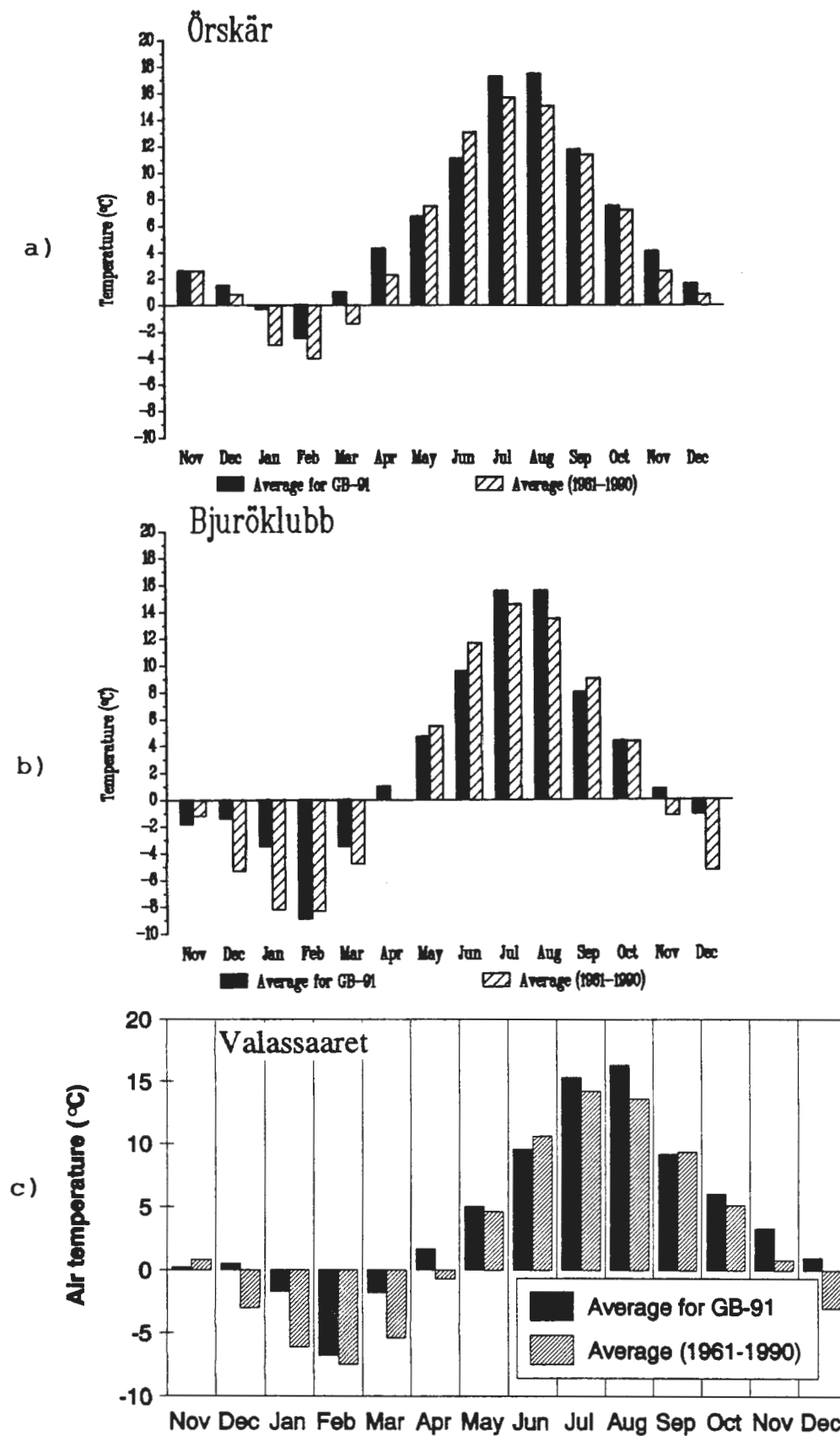
Figure 9.3. Monthly average temperature from a) the Örskär, b) the Bjuröklubb and c) the Valassaaret stations during the Gulf of Bothnia Year compared to the 30-year period covering the years 1961 to 1990.
