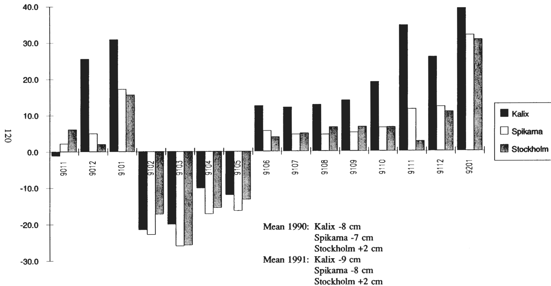
Figure 9.8a. Monthly deviation in centimetres from average water-level (during the GB-91 from the Swedish water-level stations: Kalix, Spikarna and Stockholm).
