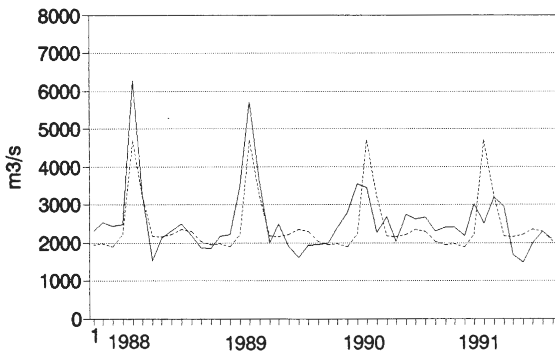
Figure 9.9b. Monthly runoff from Sweden to the Bothnian Sea 1988-91 ( — ) compared with monthly runoff from the period 1961-90 (---).
