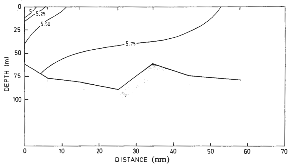
Figure 7.29. Salinity distribution along the MS section, May - June.
