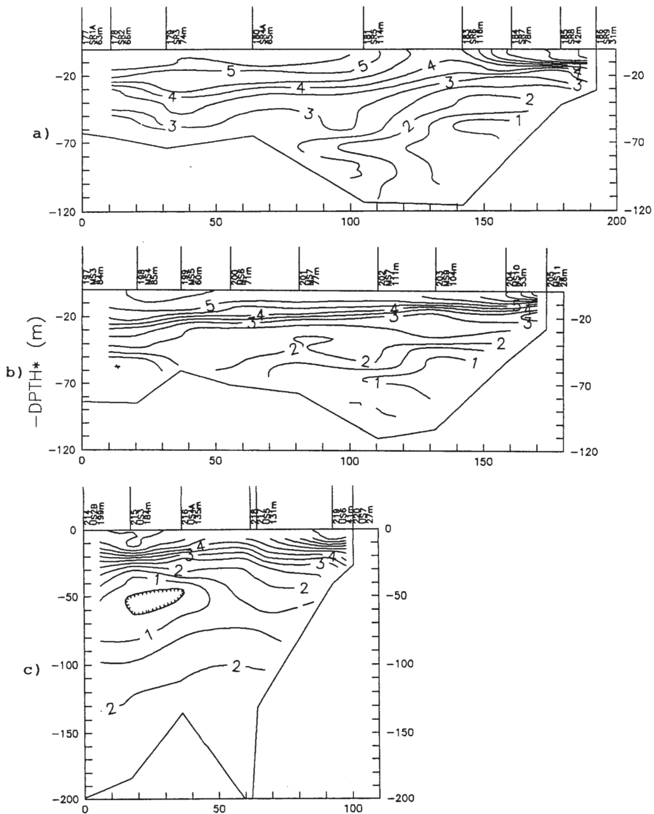
Figure 8.5. Temperature distribution along a) US section, b) MS section and c) SR section, June, 1991.
