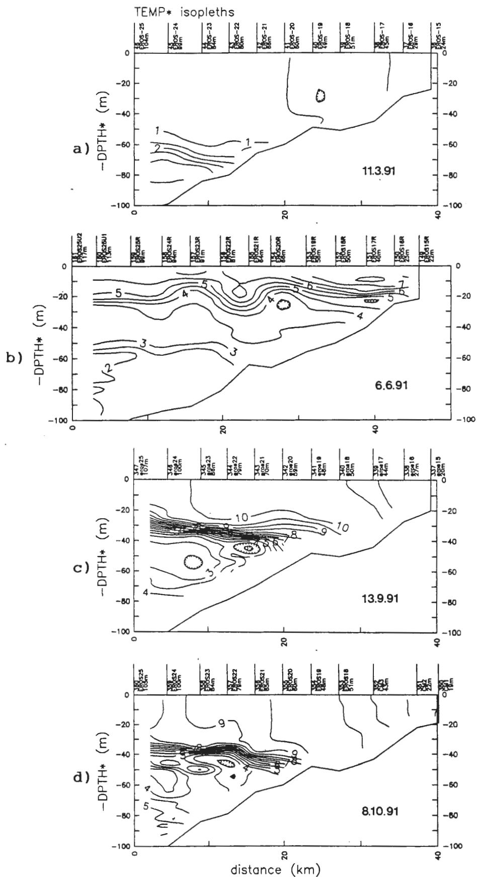
Figure 8.3. Temperature distribution along the EROS transect outside Rauma. a) 11.3.1991, b) 6.6.1991, c) 13.9.1991 and d) 8.10.1991.
