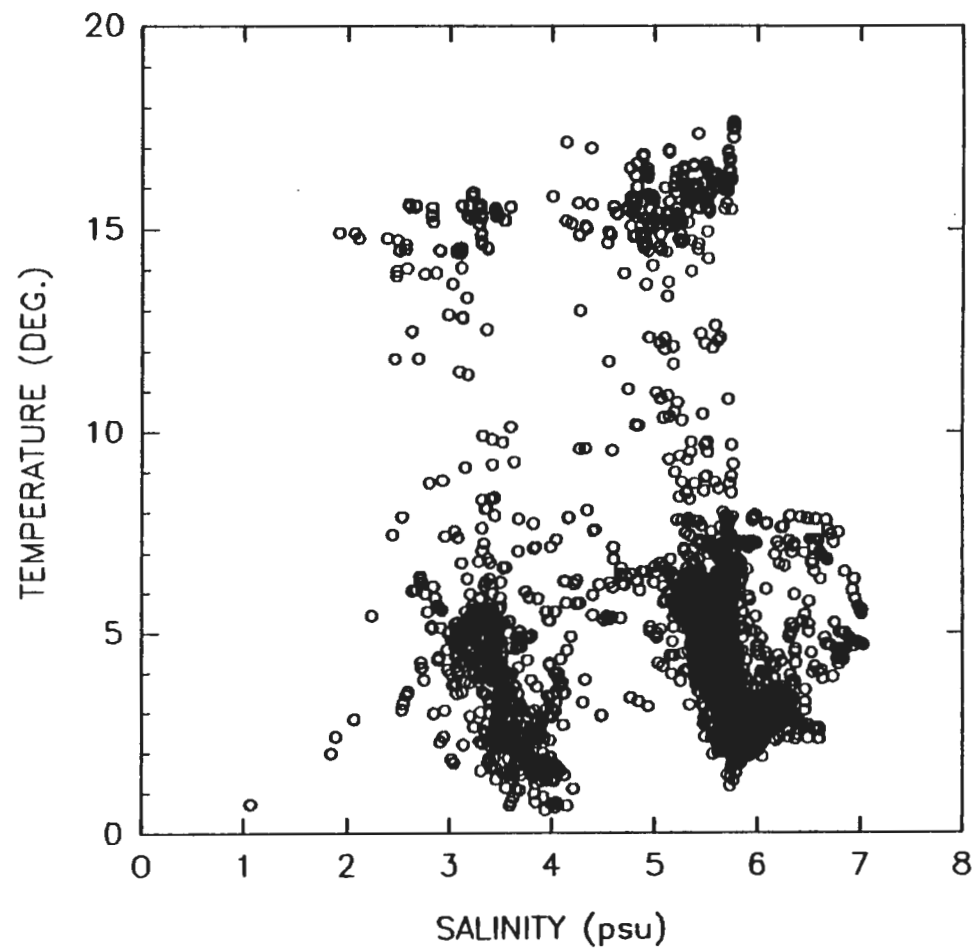
Figure 7.8. Temperature/salinity diagram showing the results from all four expeditions with the R/V Argos.
