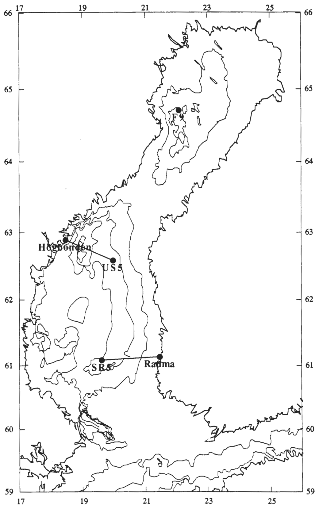
Figure 1.2. Geographical sites of the GB-91 Physical transport experiments in the Gulf of Bothnia, showing transects of current meter mooring stations ( — ) and dedicated deep-water investigations at stations SR5, US5 and F9. Depth contour resolution is 50 m.
