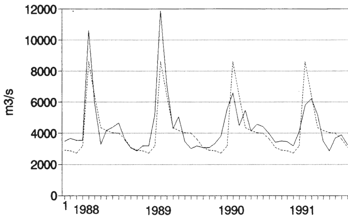
Figure 9.9c. Monthly runoff from Sweden to the Gulf of Bothnia 1988-91 ( — ) compared with monthly runoff from the period 1961-90 (---).
