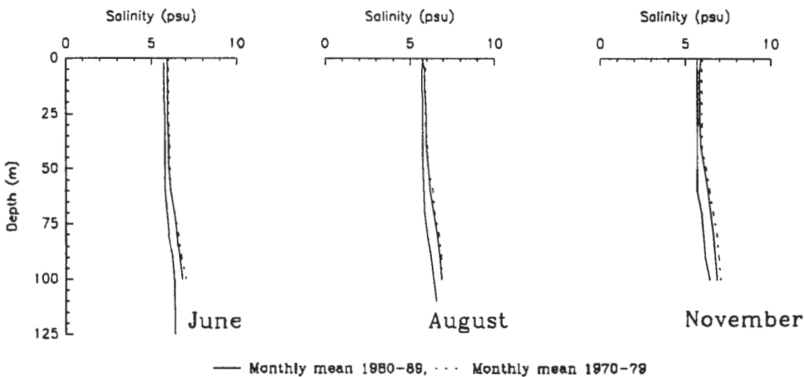
Figure 7.43. Salinity profiles, measured and mean, in the central part of the Bothnian Sea.
