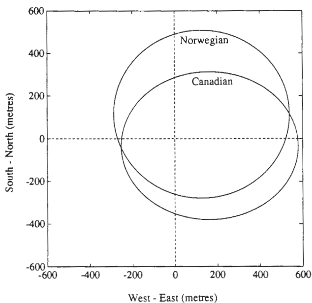
Figure 5.5. Standard deviations of the location accuracy during a test period in a fixed place. Different Argos-location classes are not separated and values are calculated as overall averages for the Canadian and Norwegian buoys. The figure is centered in the mean coordinates of the locations of the best accuracy class. (This was found to be within 120 m from the location given by the GPS-location system.)
