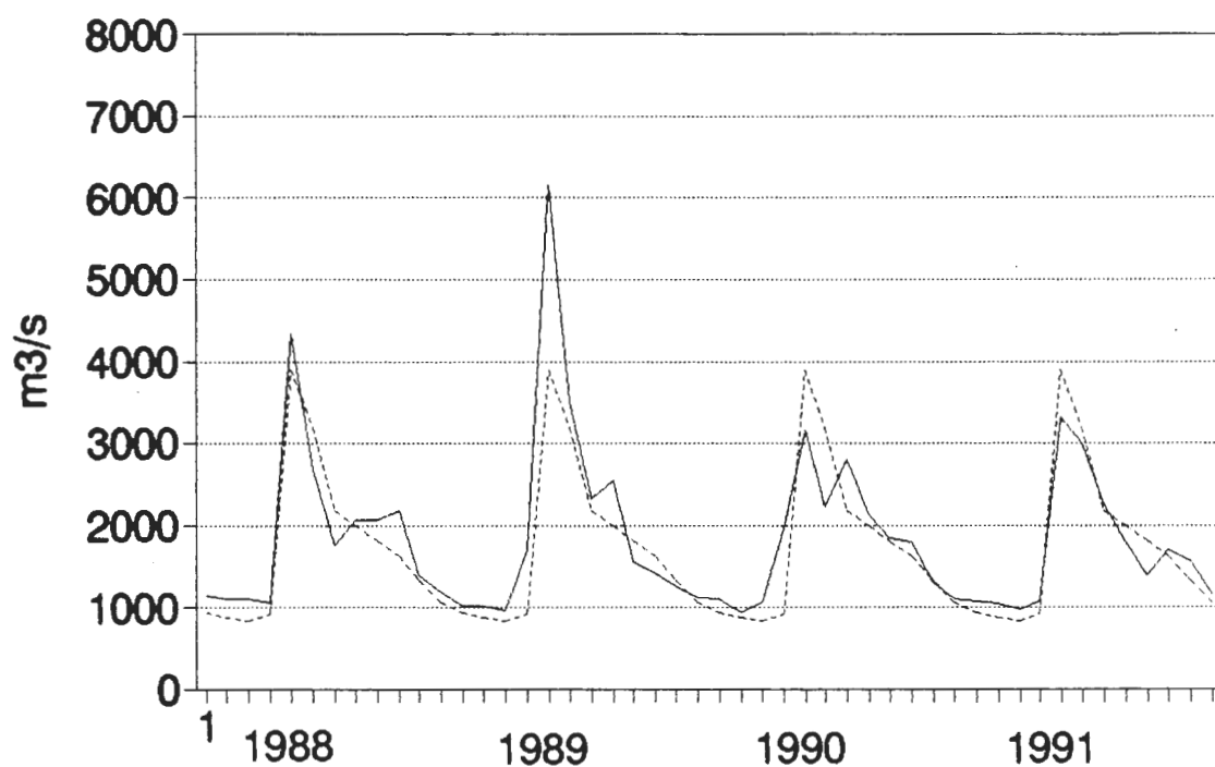
Figure 9.9a. Monthly runoff from Sweden to the Bay of Bothnia 1988-91 ( — ) compared with monthly runoff from the period 1961-90 (---).
