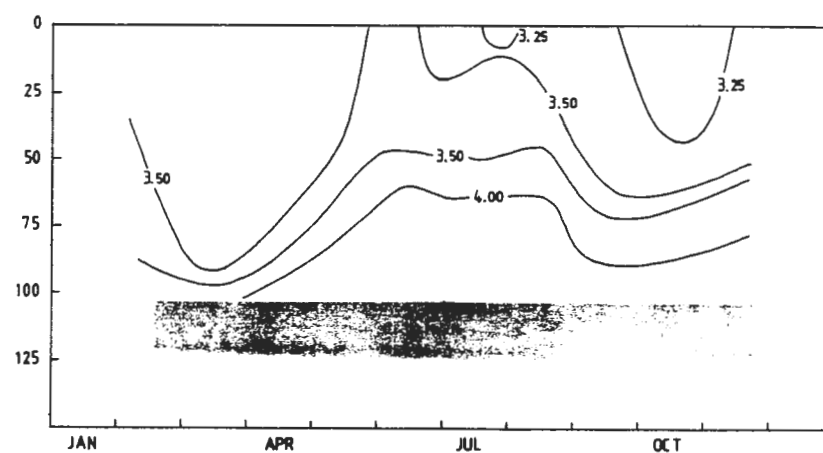
Figure 7.12. Seasonal salinity variation at F9 in the Bothnian Bay.
