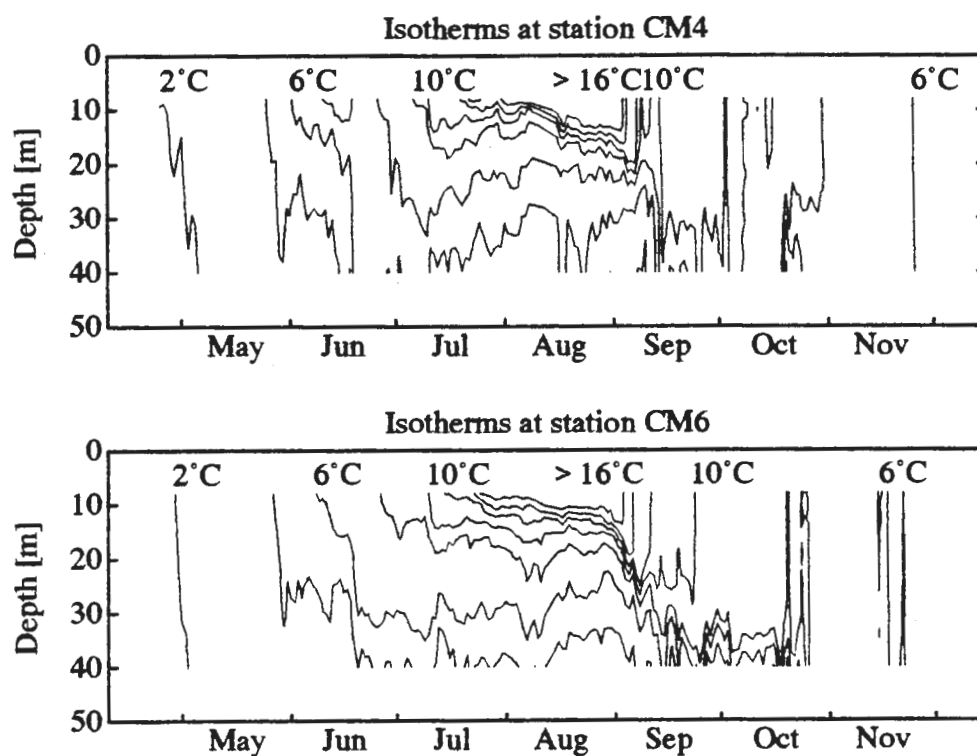
Figure 3.5. Daily mean isotherm depths at the thermistor chain stations CM4 and CM6.
