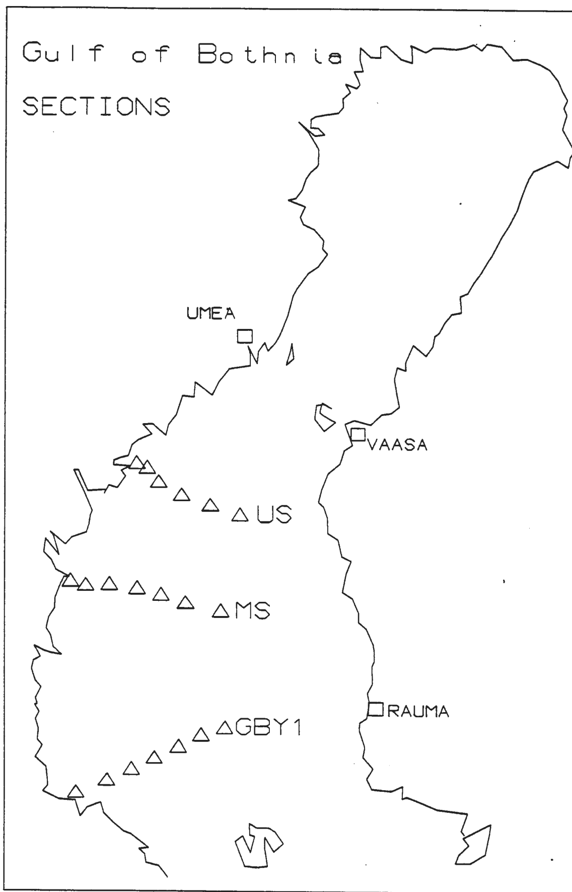
Figure 7.19. Key map showing the different sections.
