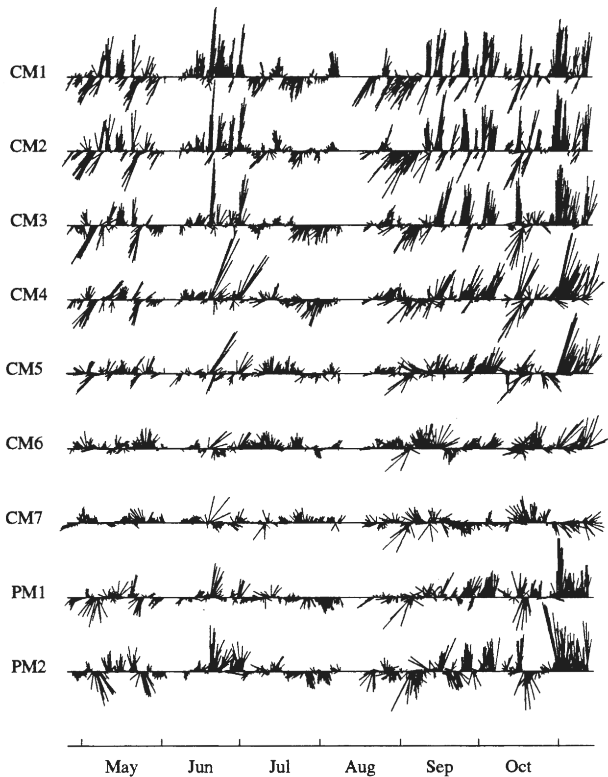
Figure 3.8. Graham-filtered current vectors plotted with 6 hours intervals at 8 m depth on the coastal transect (stations CM1 - CM7) and stations PM1 and PM2. The figure clearly shows the episodic nature of the currents.
