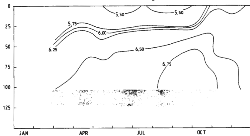
Figure 7.10. Seasonal salinity variation at Singö in the southern part of the Bothnian Sea.
