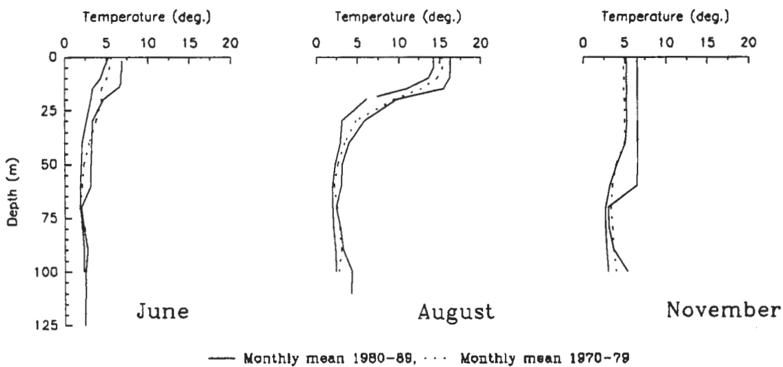
Figure 7.42. Temperature profiles, measured and mean, in the central part of the Bothnian Sea.
