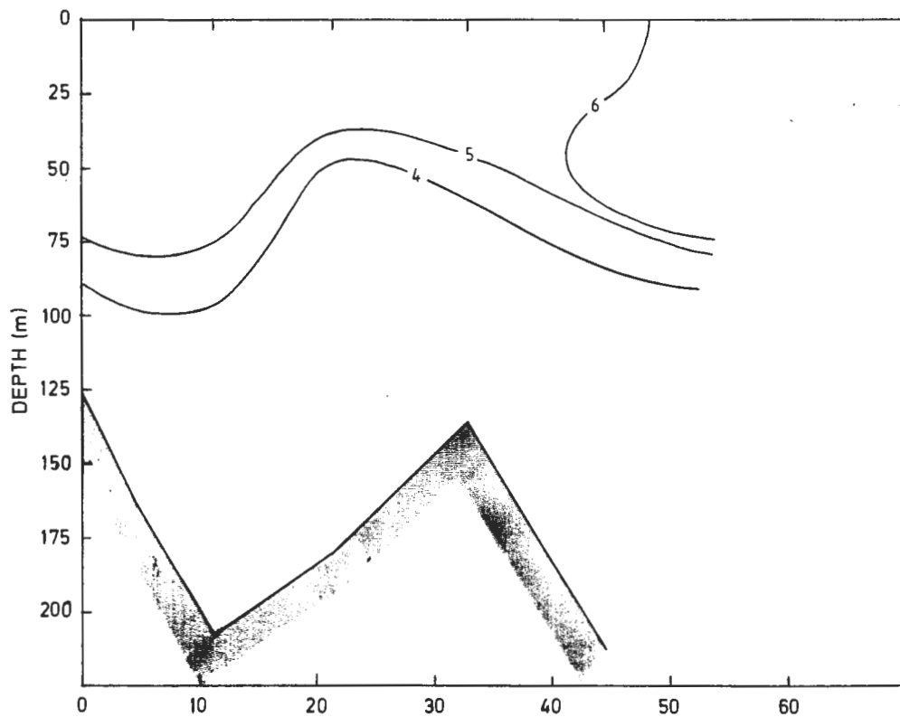
Figure 7.34. Temperature distribution along the US section, November.
