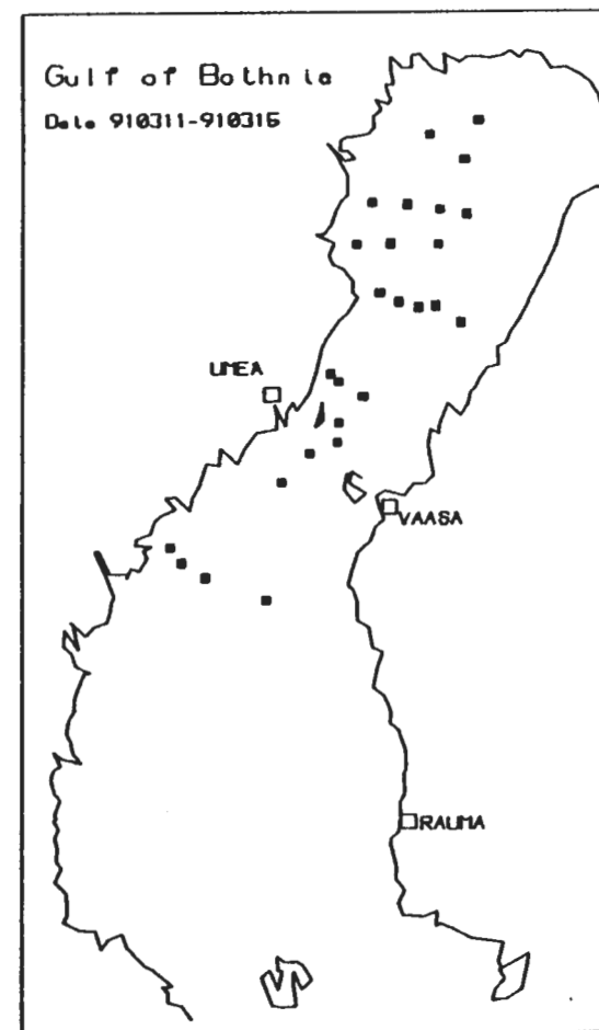
Figure 7.6. Hydrographical stations visited by the ice- breaker Ymer, March 1991.
