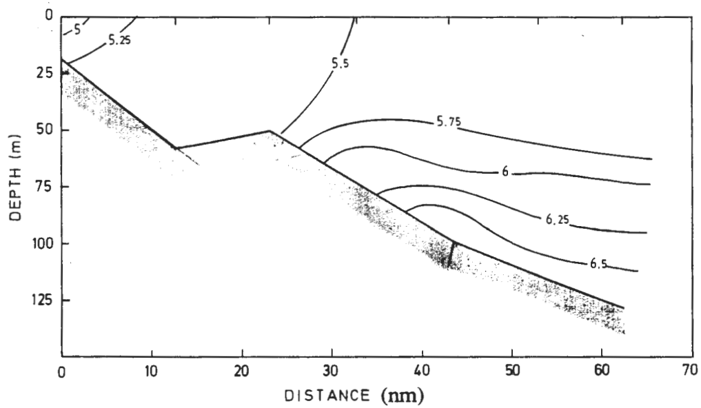
Figure 7.25. Salinity distribution along the GBY1 section, November.
