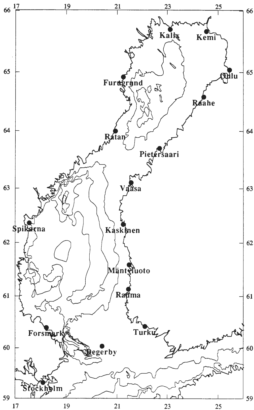
Figure 9.2. The water-level stations in the area.
