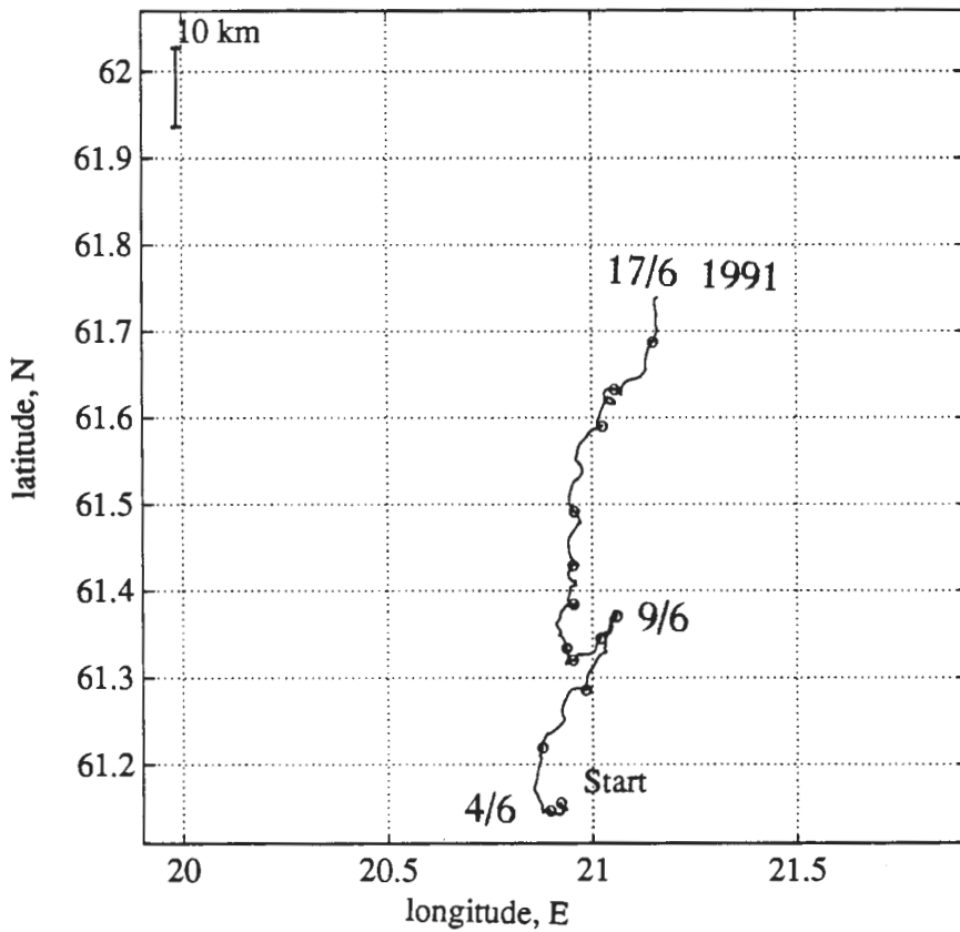
Figure 5.8. Centroid (center of population) trajectory for the Cluster Experiment 1; daily positions are given as circles.
