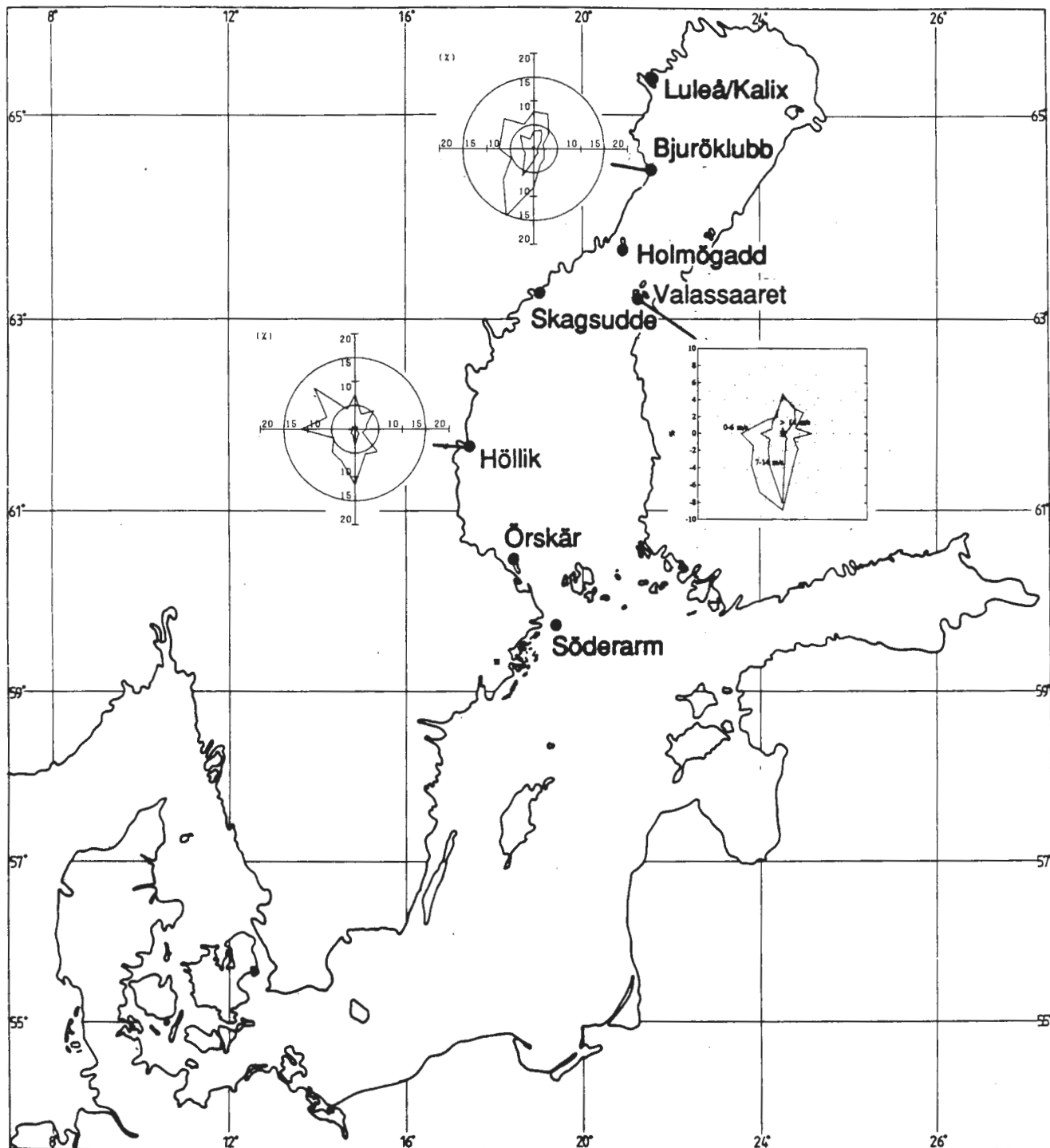
Figure 9.1. Weather stations in the Gulf of Bothnia. The observed parameters are wind, temperature, relative evaporation and cloudiness. The stations Luleå/Kalix, Bjuröklubb and Holmögdad also observe air pressure. The wind roses from the weather stations Bjuröklubb, Höllik and Valassaaret (22.4. - 22.11.) illustrate the distribution of wind speed directions. The directions are towards the wind. Here the magnitudes are below 7 m/s, between 7 and 14 m/s and above 14 m/s.
