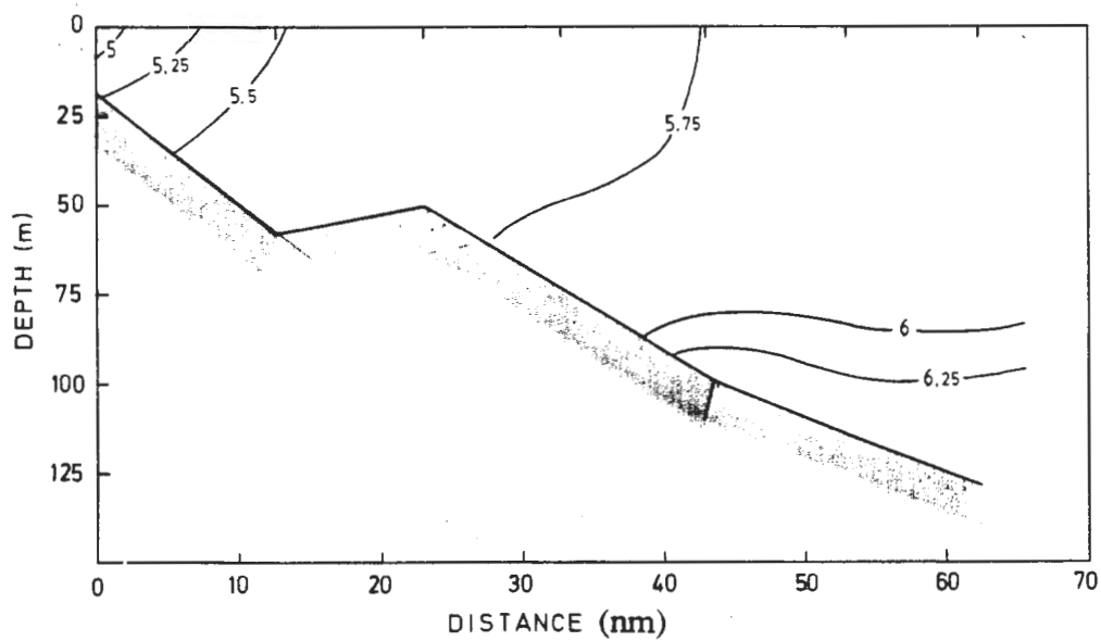
Figure 7.23. Salinity distribution along the GBY1 section, May - June.
