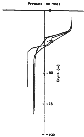
Figure 7.38. Examples of how the vertical structure of the first mode P_1 varies with depth. The scale on the ordinate is arbitrary.
