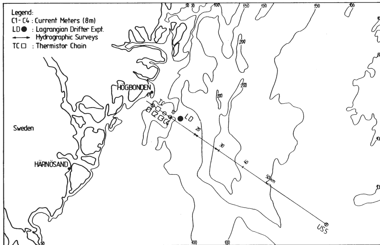
Figure 2.1. Bathymetric chart of the area where the Swedish Coastal Transect Experiment was carried out.
