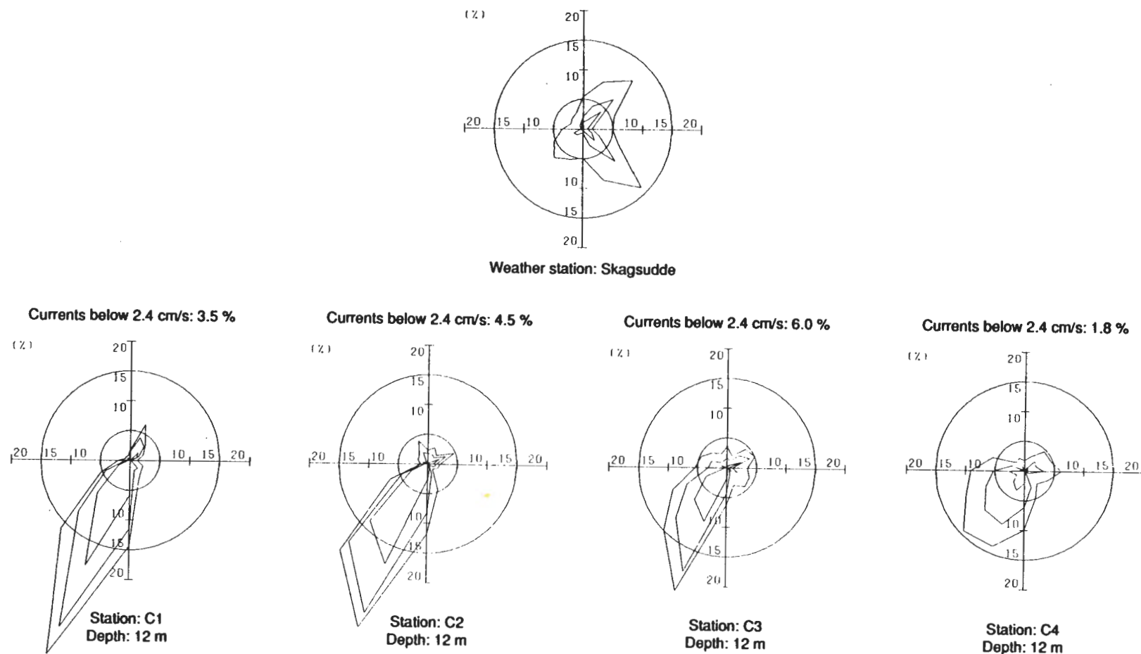
Figure 2.4. Current roses of filtered data from Högbonden Transect, illustrating the distribution of current directions with velocities below 7 cm/s, between 7 and 14 cm/s and above 14 cm/s, respectively. The percentage of currents below 2.4 cm/s is also given for the different current meters, which is the lower limit of the Sensor Data current meters. The wind rose is from the nearest weather station, Skagsudde. It illustrates the distribution of wind stress directions. The direction is with the wind. Here the magnitudes are below 0.07 \text{ N/m}^2 , between 0.07 and 0.14 \text{ N/m}^2 and above 0.14 \text{ N/m}^2 .
