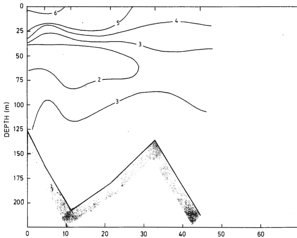
Figure 7.32. Temperature distribution along the US section, May - June.
