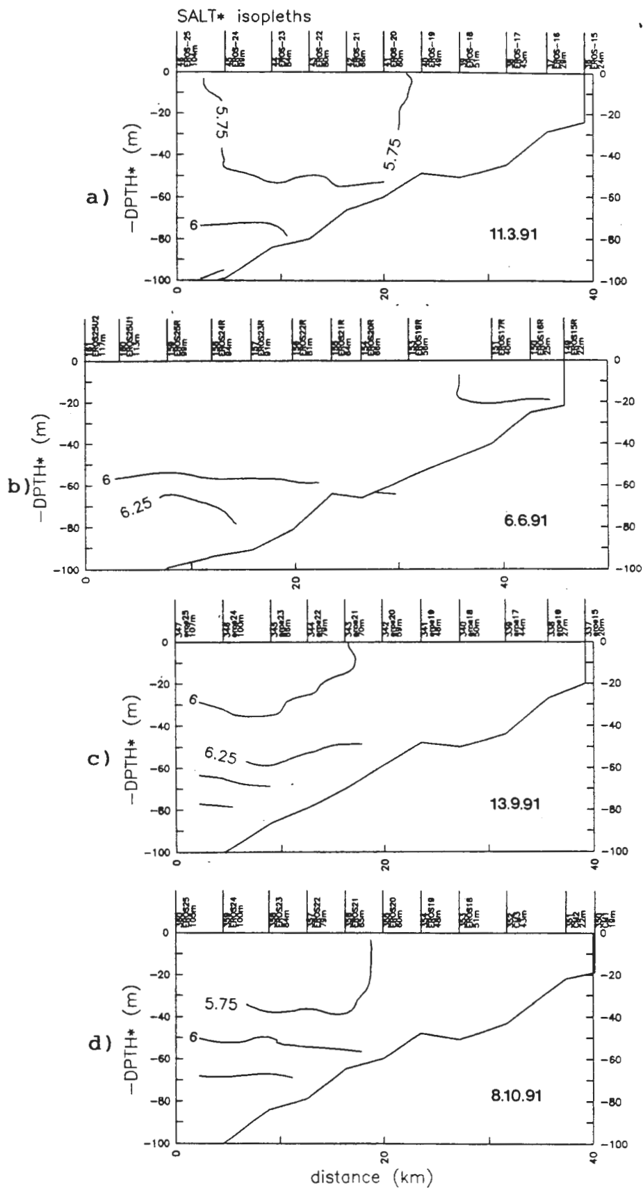
Figure 8.4. Salinity distribution along the EROS transect outside Rauma. a) 11.3.1991, b) 6.6.1991, c) 13.9.1991 and d) 8.10.1991.
