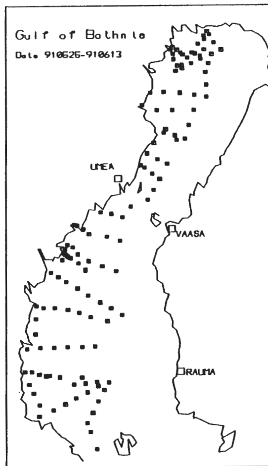
Figure 7.2. Hydrographical stations visited by the R/V Argos, May - June 1991.
