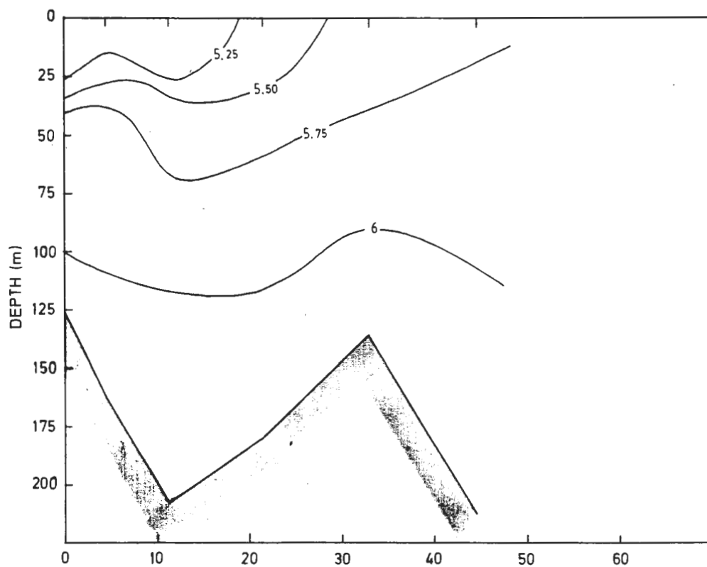
Figure 7.34. Temperature distribution along the US section, November.
