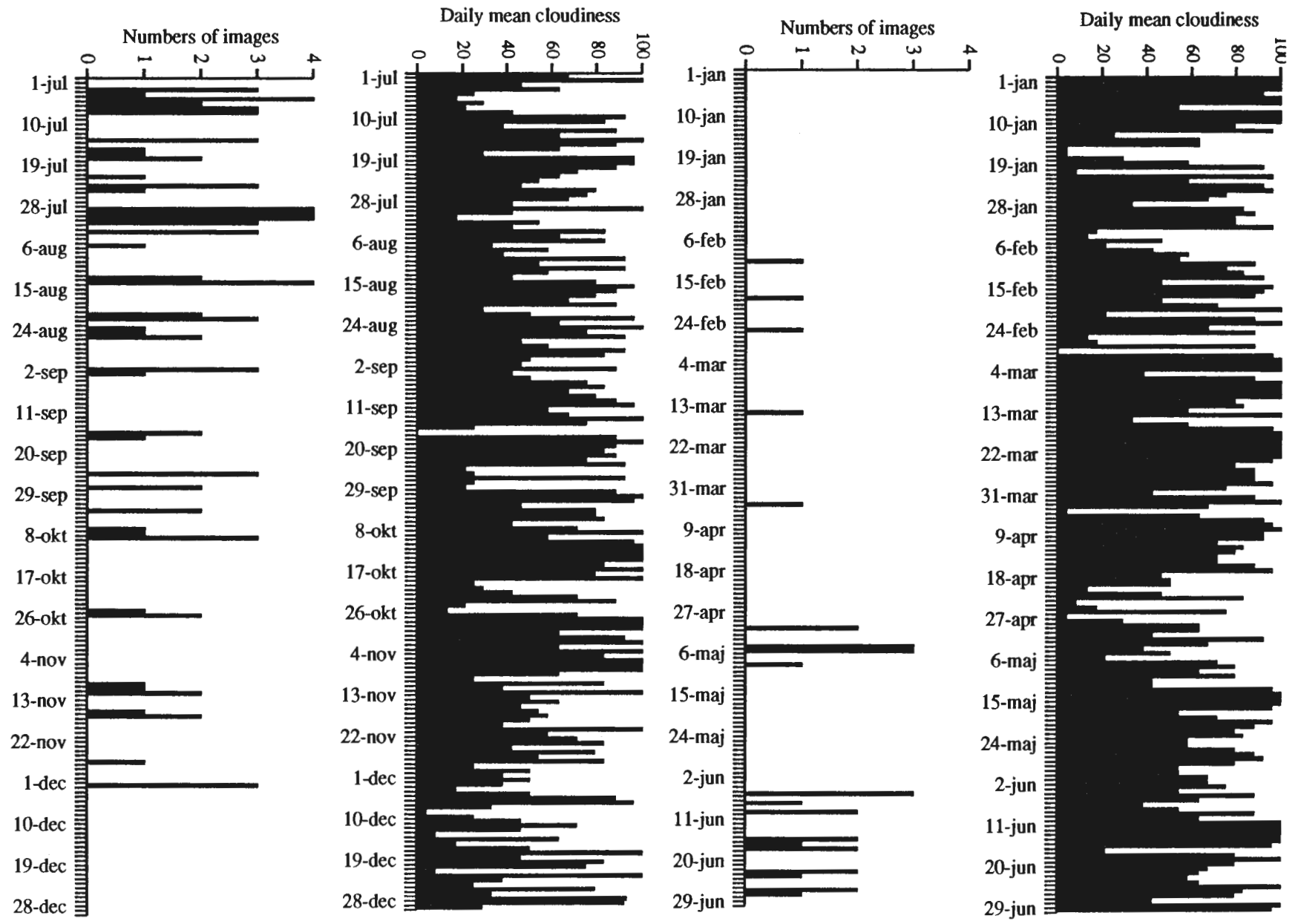
Figure 6.1. Achieved images and daily mean cloudiness at Skagsvade weather station, 1991.
