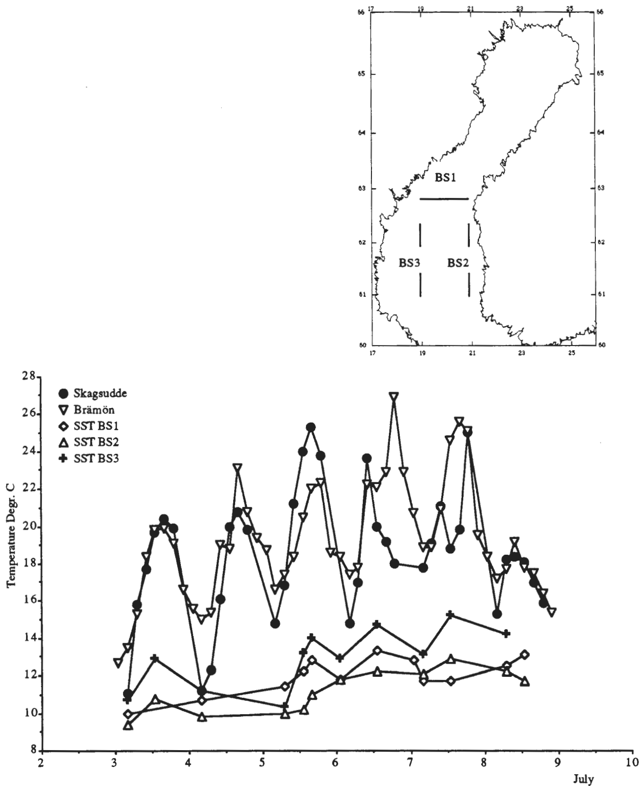
Figure 6.2. Air temperature from two coastal stations and sea surface brightness temperatures from three line sections in the images, covering the Bothnian Sea.
