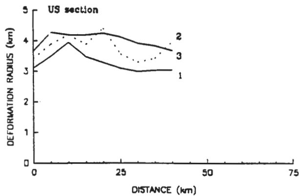
Figure 7.41. The deformation radius as a function of distance from the coast at section US. The numbers refer to the expeditions in May (1), August (2) and November (3).
