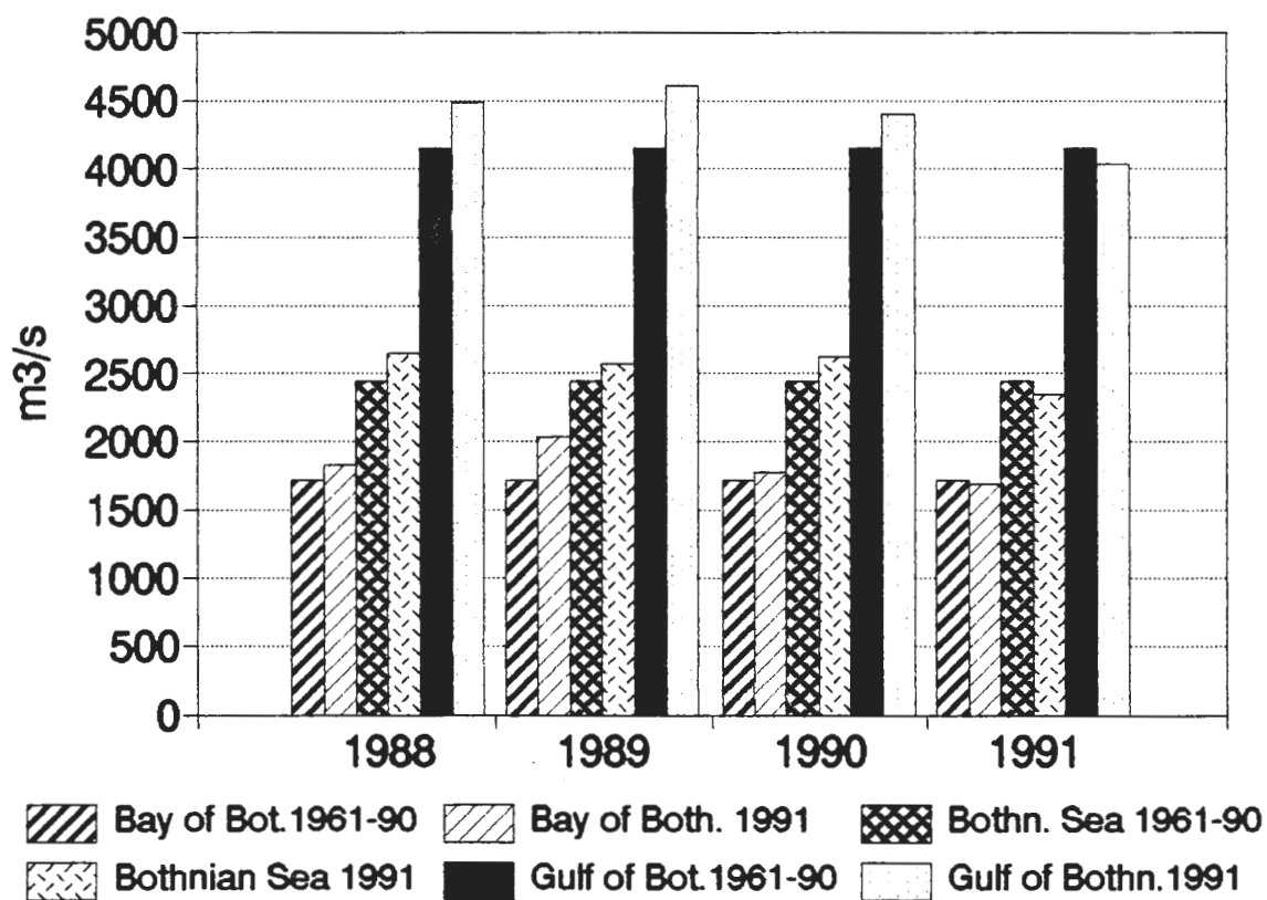
Figure 9.9d. Annual means of runoff to the Gulf of Bothnia from Sweden.
