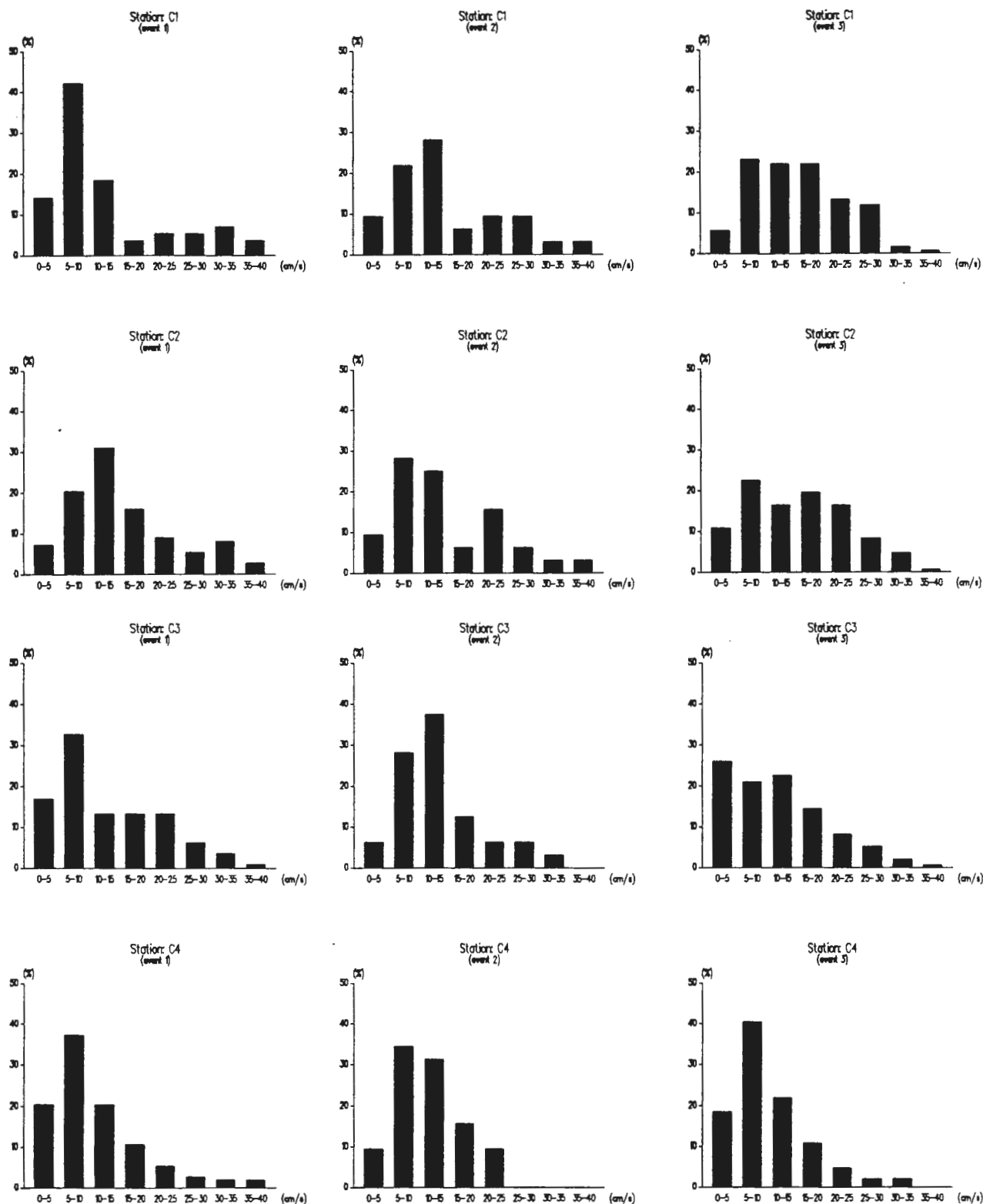
Figure 2.10. Distribution of current velocity during the Coastal Transect Experiment. The experiment is divided into three separating events, where the first event covers the period from the start of the experiment to June 15, the second event from June 16 to June 19, and the last event covers the period from June 20 until the end of the experiment, July 17.
