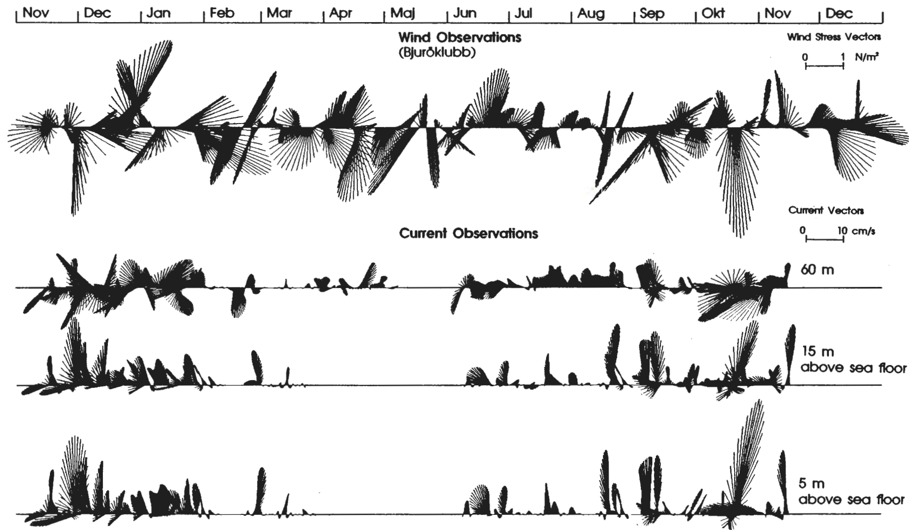
Figure 2.9a. Time series vector plots of wind and current data of the Open Sea station in the Bothnian Bay, F9. The data have been filtered with a low-pass filter with 18 to 24 hour cutoff.
