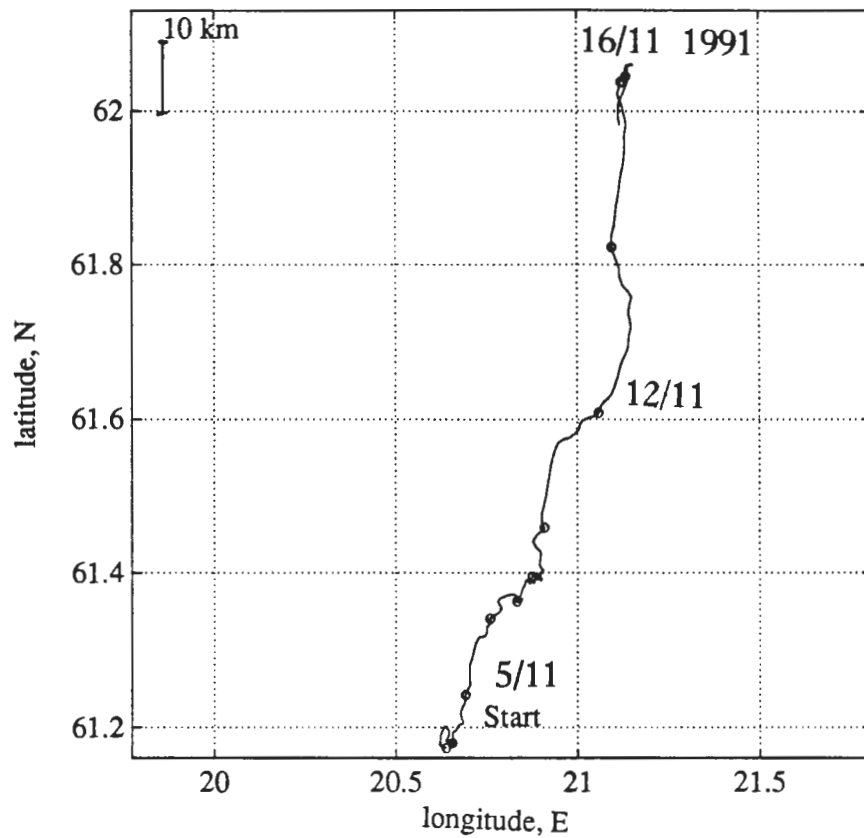
Figure 5.9. Centroid (center of population) trajectory for the Cluster Experiment 2.
