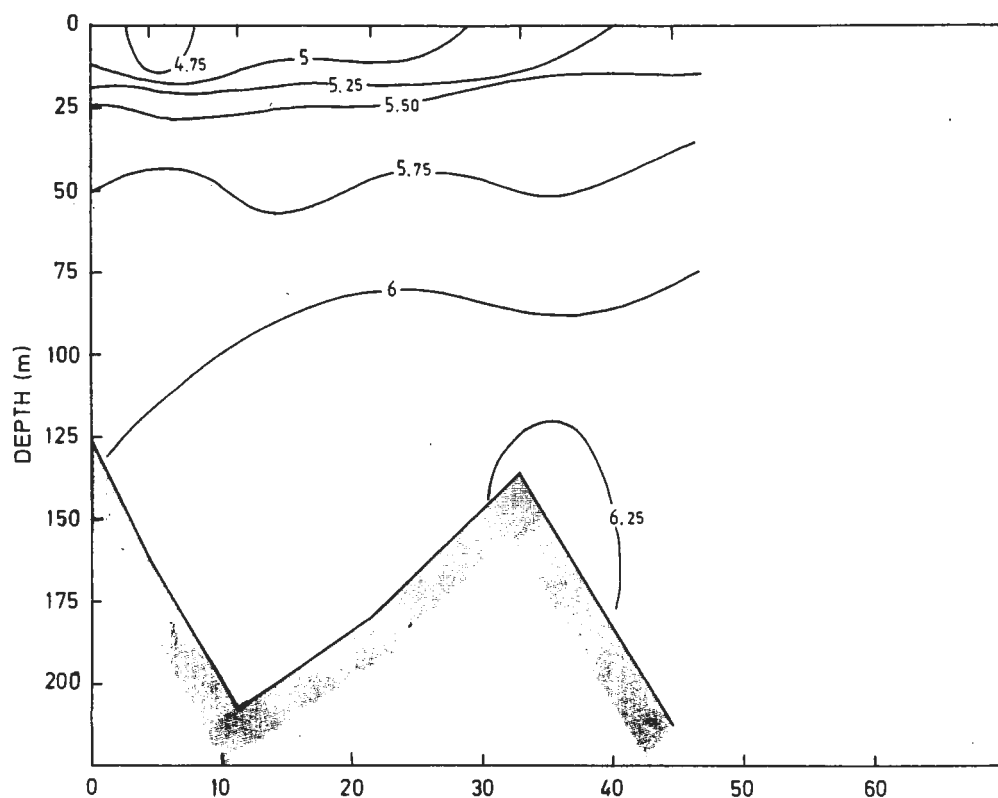
Figure 7.36. Salinity distribution along the US section, August.
