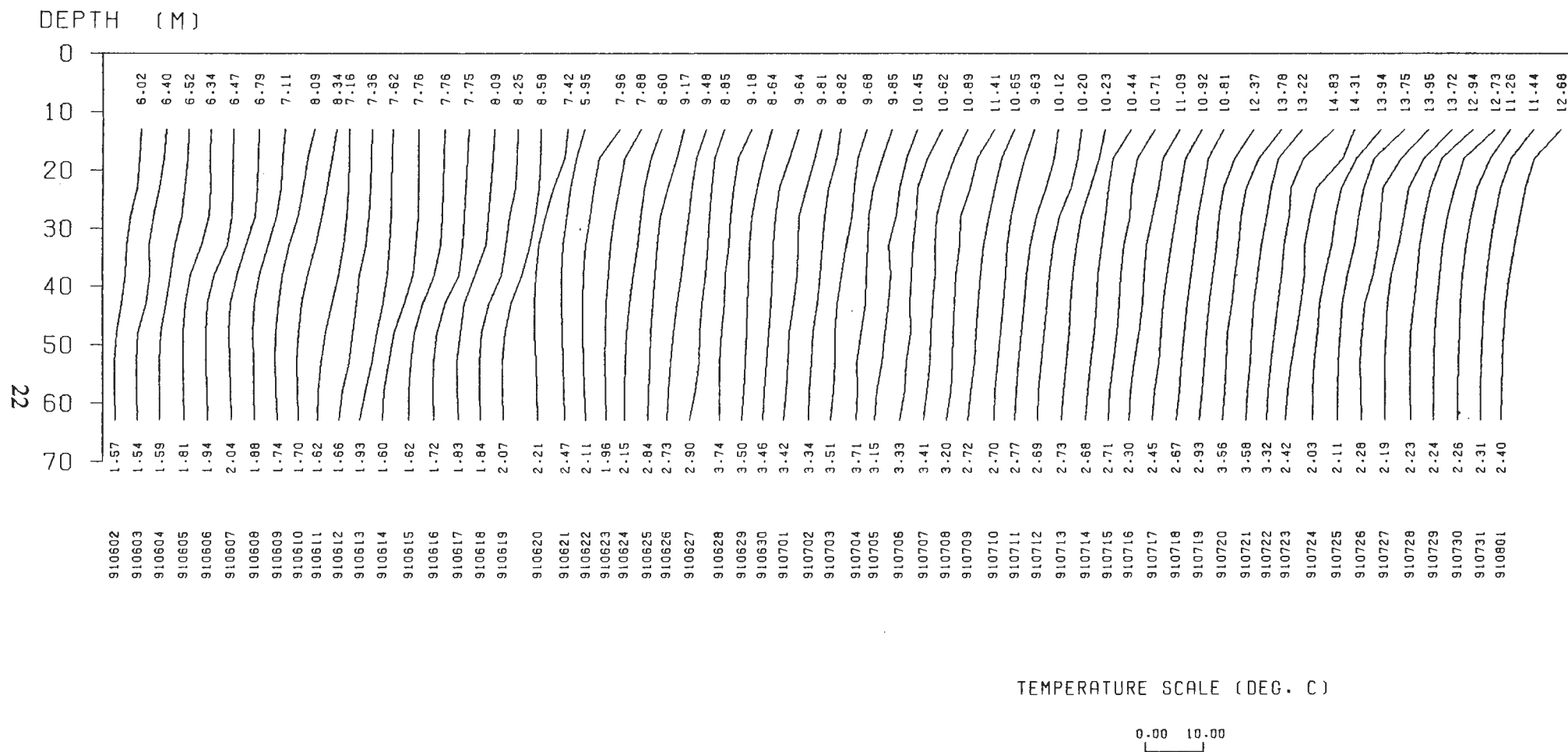
Figure 2.6. Daily average temperature profiles of the thermistor chain at station C2. The thermistors were placed between 13 and 63 m depth, and 5 m apart.
