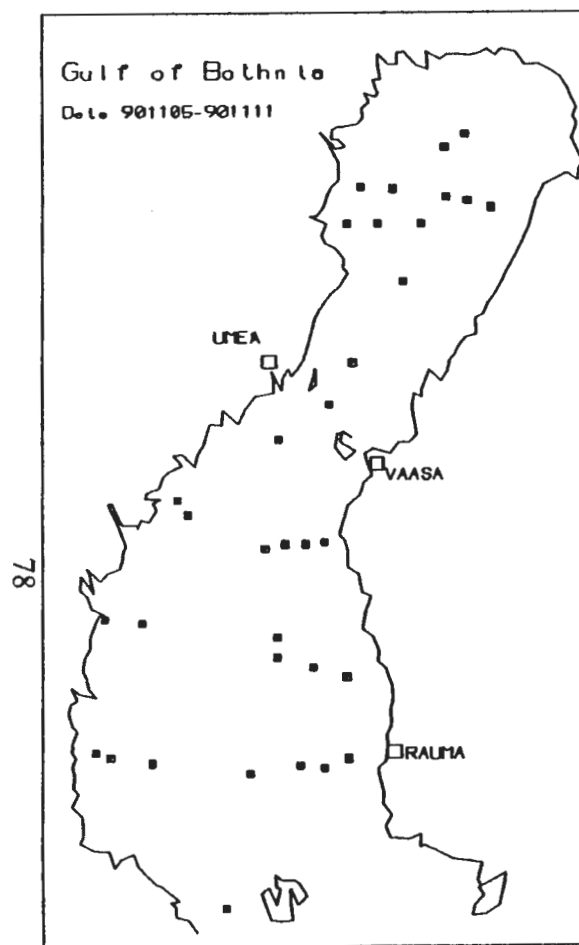
Figure 7.1. Hydrographical stations visited by the R/V Argos, November 1990.
