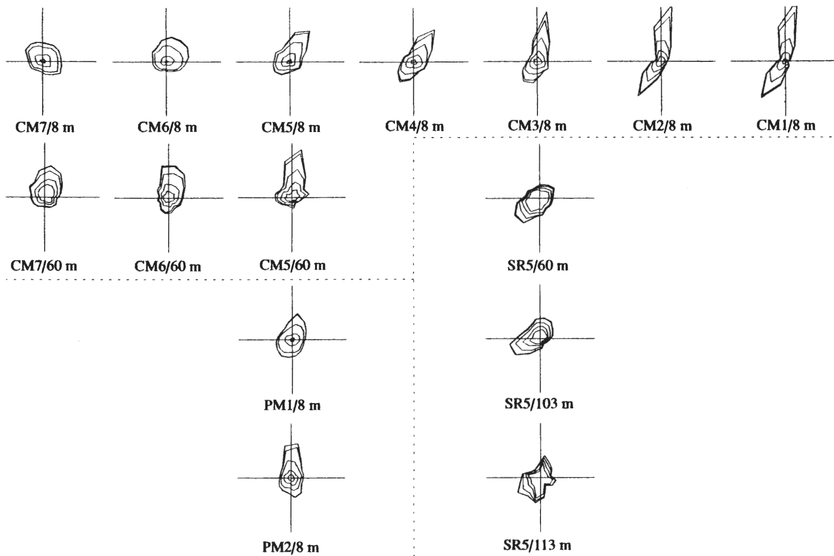
Figure 3.7. Schematic current roses from the Finnish current meters, illustrating the distribution of the current directions in different speed classes.
