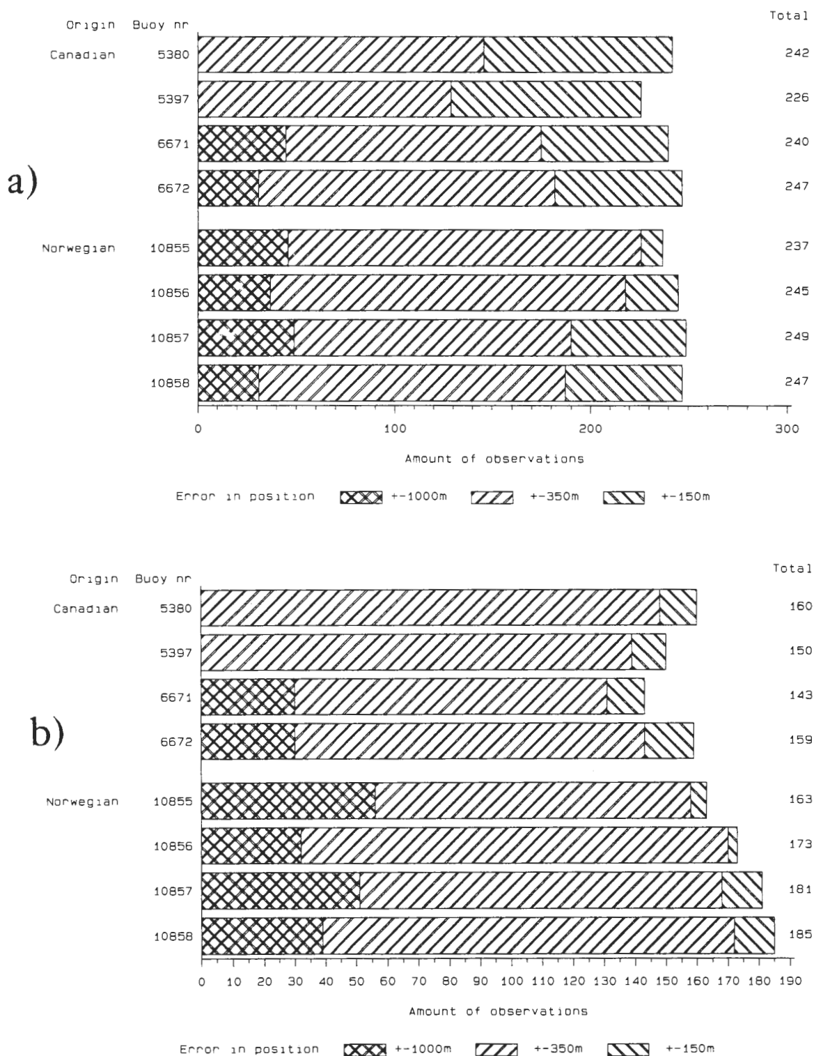
Figure 5.4. Location accuracy given as the distribution of location classes of the Argos system for the drifters used in the Finnish drifter experiment. a) gives the results for Cluster 1 and b) those for Cluster 2, respectively.
