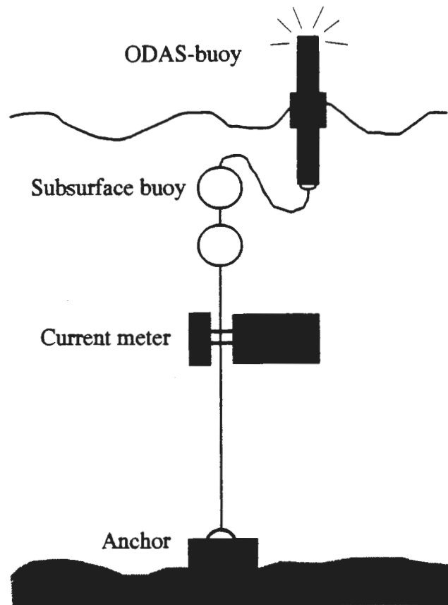
Figure 3.3. Schematic figure of mooring system.
