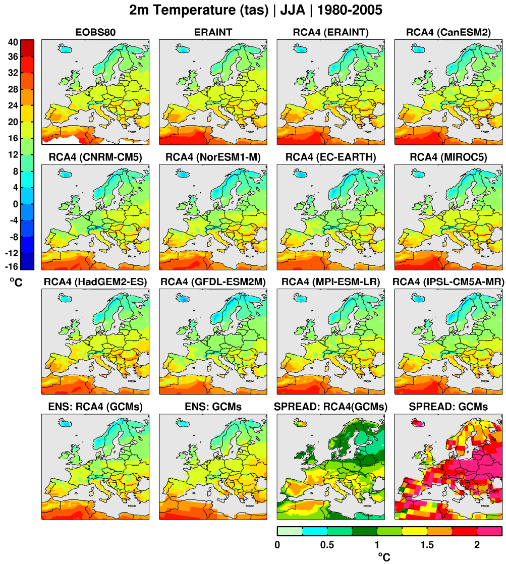
Figure A4. Summer (June – August) temperature (°C) in the recent past climate, 1980-2005, according to E-OBS, ERAINT, RCA4 forced with ERAINT and RCA4 forced with 9 different GCMs (rows 1-3). Bottom row: ensemble mean in RCA4 forced by GCMs, ensemble mean in GCMs, spread between members in the RCA4 GCM ensemble and spread in the GCM ensemble given as standard deviation.
