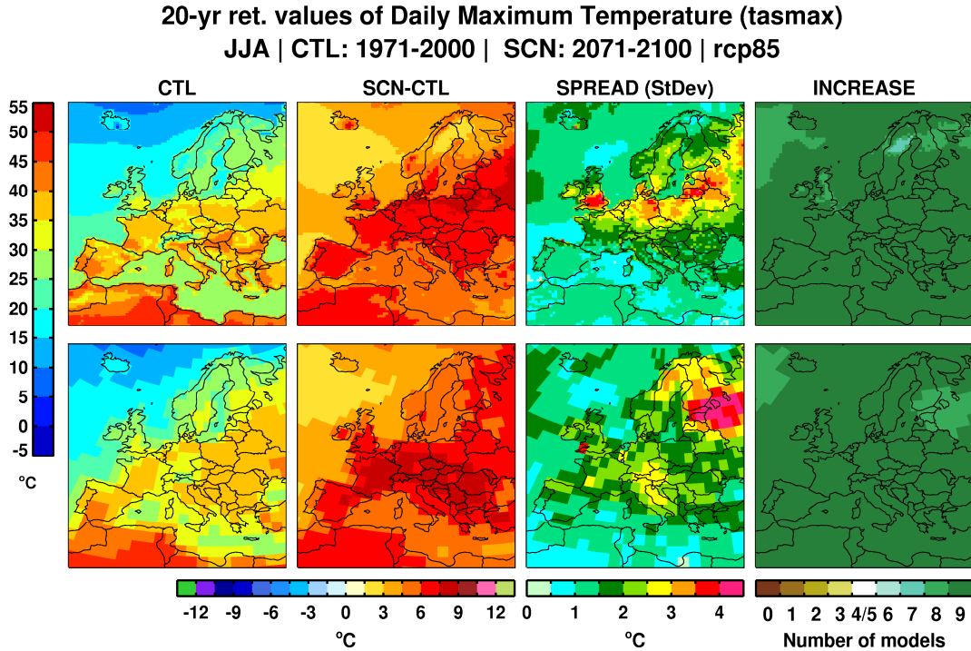
Figure 26. Ensemble mean summer (June – August) 20-year return values for daily maximum temperatures in the control period 1971-2000 (left). The three other columns show changes between the period 2071-2100 under the RCP 8.5 scenario as compared to the control period for the return levels (second from left), the standard deviation calculated from the nine ensemble members (third from left) and number of models that simulate an increase (rightmost). The upper row shows conditions in RCA4 and the lower the corresponding fields taken directly from the underlying GCMs.
