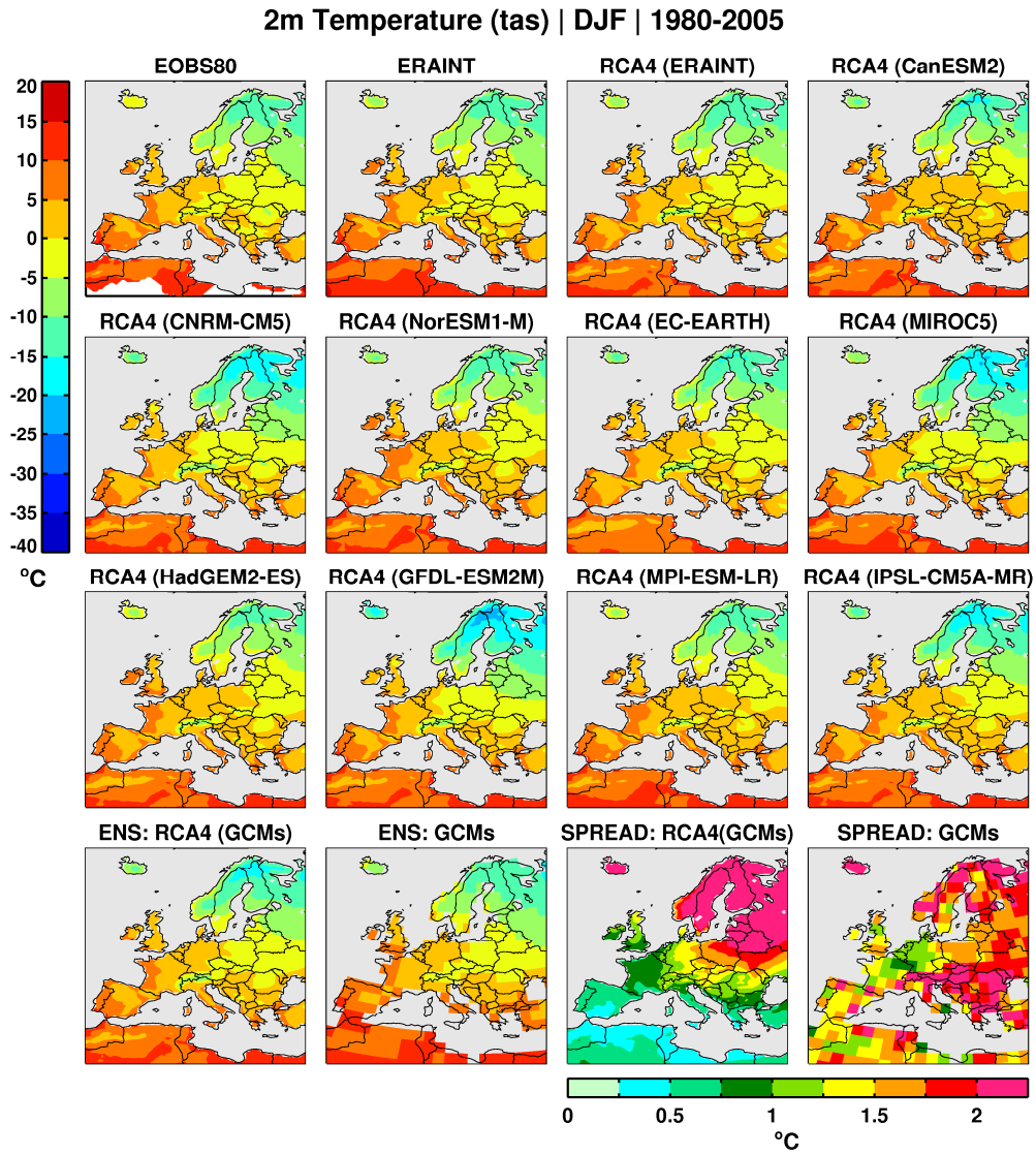
Figure A3. Winter (December – February) temperature (°C) in the recent past climate, 1980-2005, according to E-OBS, ERAINT, RCA4 forced with ERAINT and RCA4 forced with 9 different GCMs (rows 1-3). Bottom row: ensemble mean in RCA4 forced by GCMs, ensemble mean in GCMs, spread between members in the RCA4 GCM ensemble and spread in the GCM ensemble given as standard deviation.
