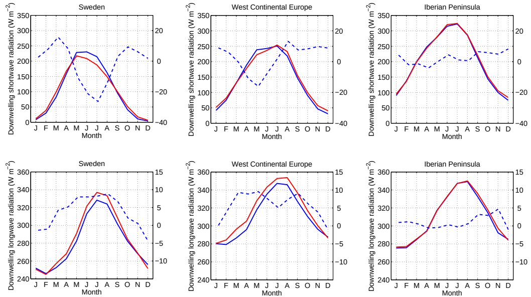
Figure 9. Annual cycles of incoming short wave radiation (top row, W/m^2 ) and incoming long wave radiation (bottom row, W/m^2 ) in RCA (red) and ERAINT (blue); Sweden (left), West Continental Europe (middle) and the Iberian Peninsula (right). Differences RCA4 – observation/reanalysis are represented by dashed lines on the right hand y-axis.
