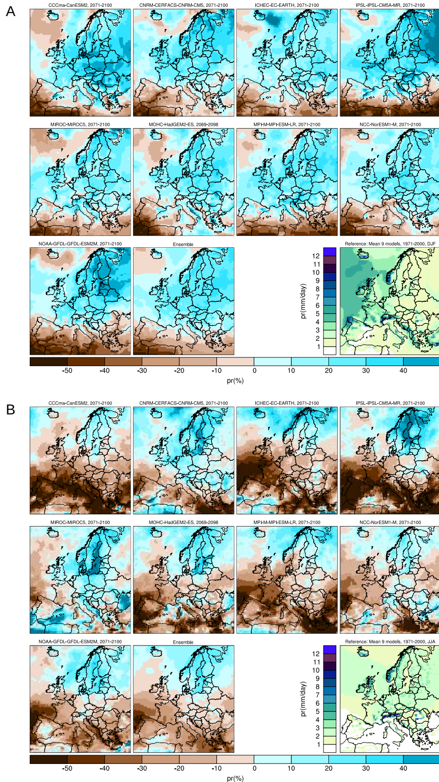
Figure A12. Difference in precipitation (%) 2071-2100 compared to 1971-2000 in RCA4 forced with 9 different GCMs and the RCA4 ensemble mean according to RCP 8.5. The ensemble mean of the absolute precipitation (mm/day), 1971-2000, is shown in the bottom right corner. A) winter (December – February), B) summer (June – August).
