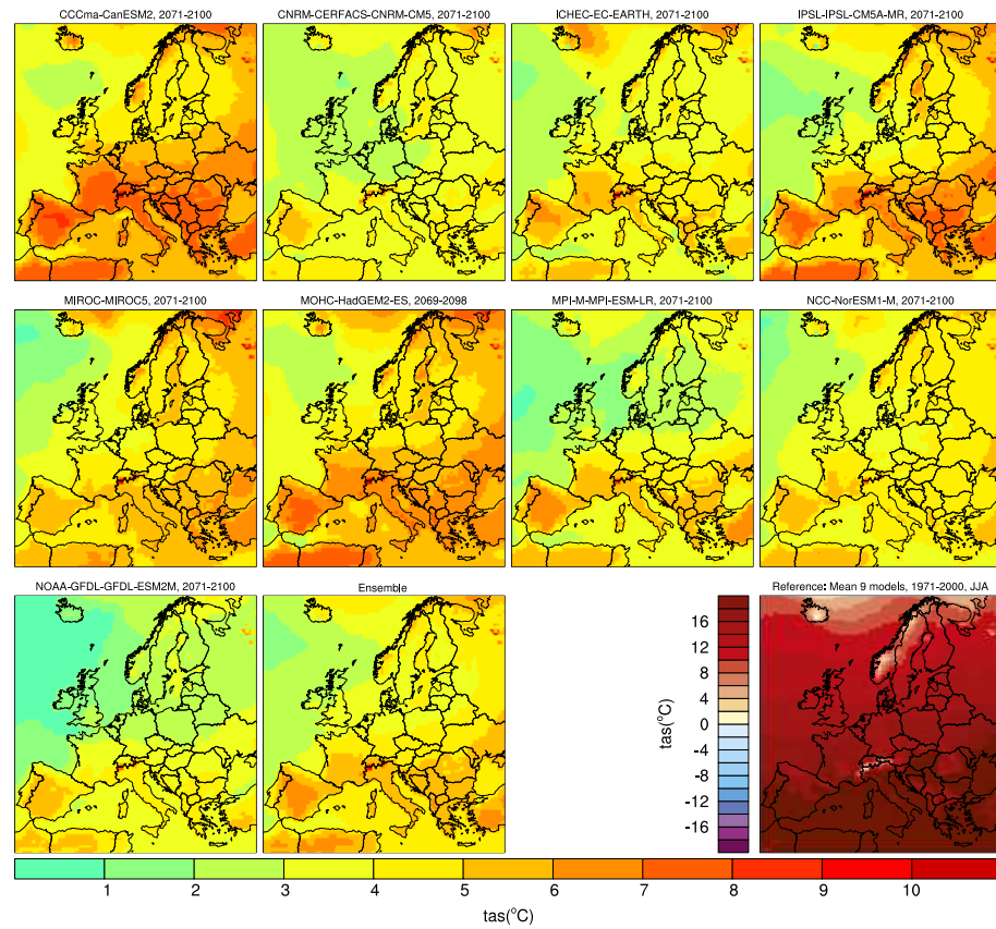
Figure A7. Difference in temperature (°C) 2071–2100 compared to 1971–2000 in RCA4 forced with 9 different GCMs and the RCA4 ensemble mean according to RCP 8.5. The ensemble mean of the absolute temperature (°C), 1971–2000, is shown in the bottom right corner. A: winter (December – February), B: summer (June – August).
