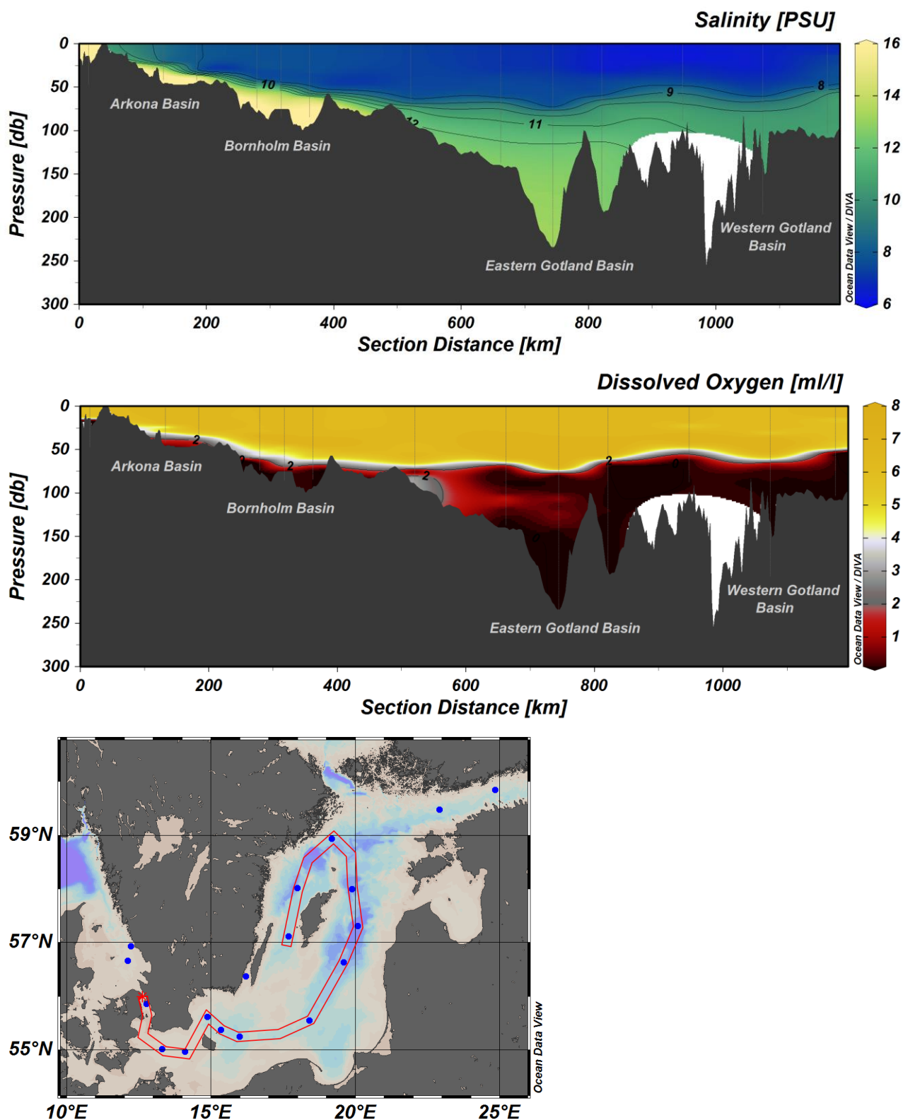
Figure 2. Transect showing dissolved oxygen and salinity from the Sound, through the Baltic Proper, to the Western Gotland Basin. Grey lines mark the positions that the plots are based on and below is a map showing these positions.
