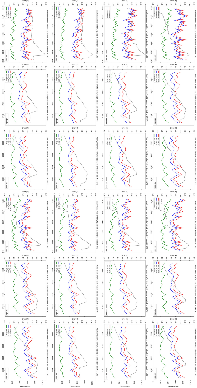
Figure 2: Yearly mean of RMSE and thenumber of observations for each hour of the T2m analysis
