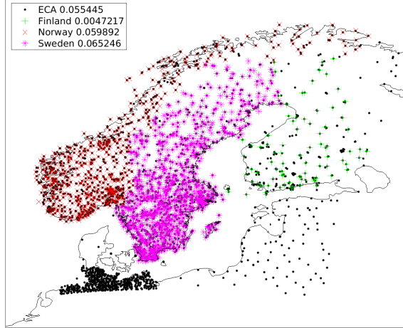
Precip observations for month 1970-07. Legend gives number of observations.
