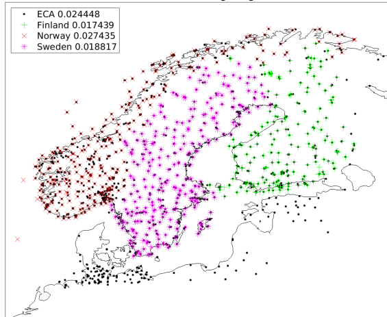
T2mmax observations for month 2015-07. Legend gives number of observations
