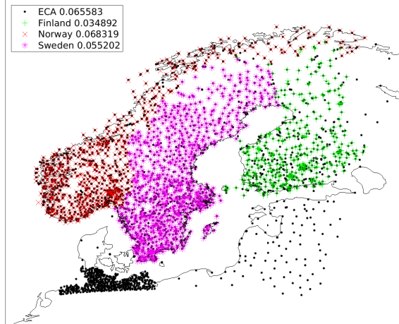
Precip observations for month 1990-07. Legend gives number of observations.
