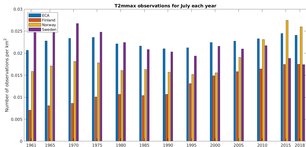
Figure 6: As Figure 5 but also with the numbers from each year-month map showed in a bar plot.
