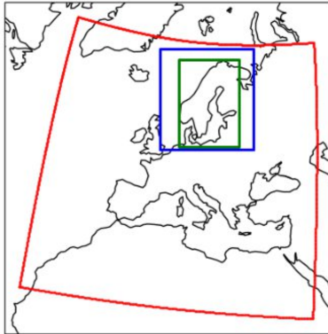
Model areas. Red: UERRA, Blue: MEPS, Green: SweGridClim
