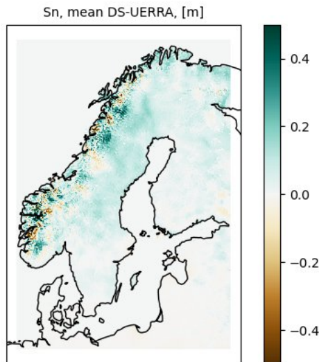
Figure 6.5 Mean differences between downscaled Sn and the original UERRA fields. The color scale was limited to \pm 0.5 m to reveal more details.
