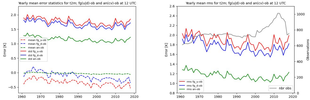
Figure 6.17 Error statistics for T2m at 12 UTC. Left: bias (dashed lines) and standard deviations (solid lines). Right: RMSE and number of observations. Red: UERRA, blue: downscaled, green: analysis.
