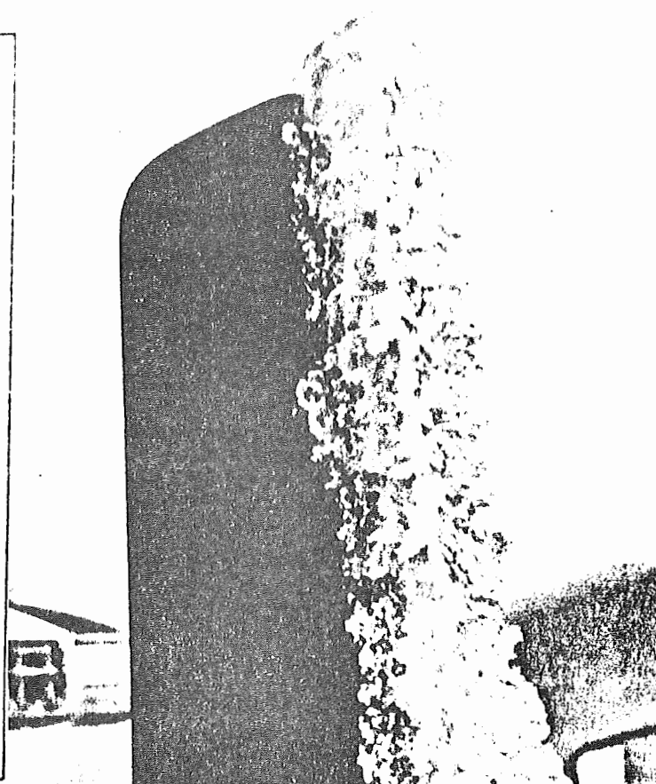
A radio mast about twelve inches high, loaded with drag-causing ice. Things like this can't be deiced. The more of these "ice catchers" on an airplane, the less time one can stay in ice—deicer-equipped or no. (ESSA photo)
