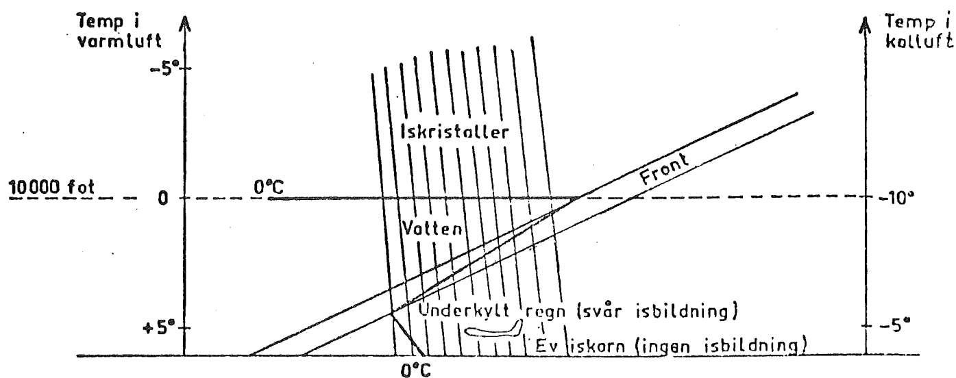
Fig 6: Underkyllt regn.
