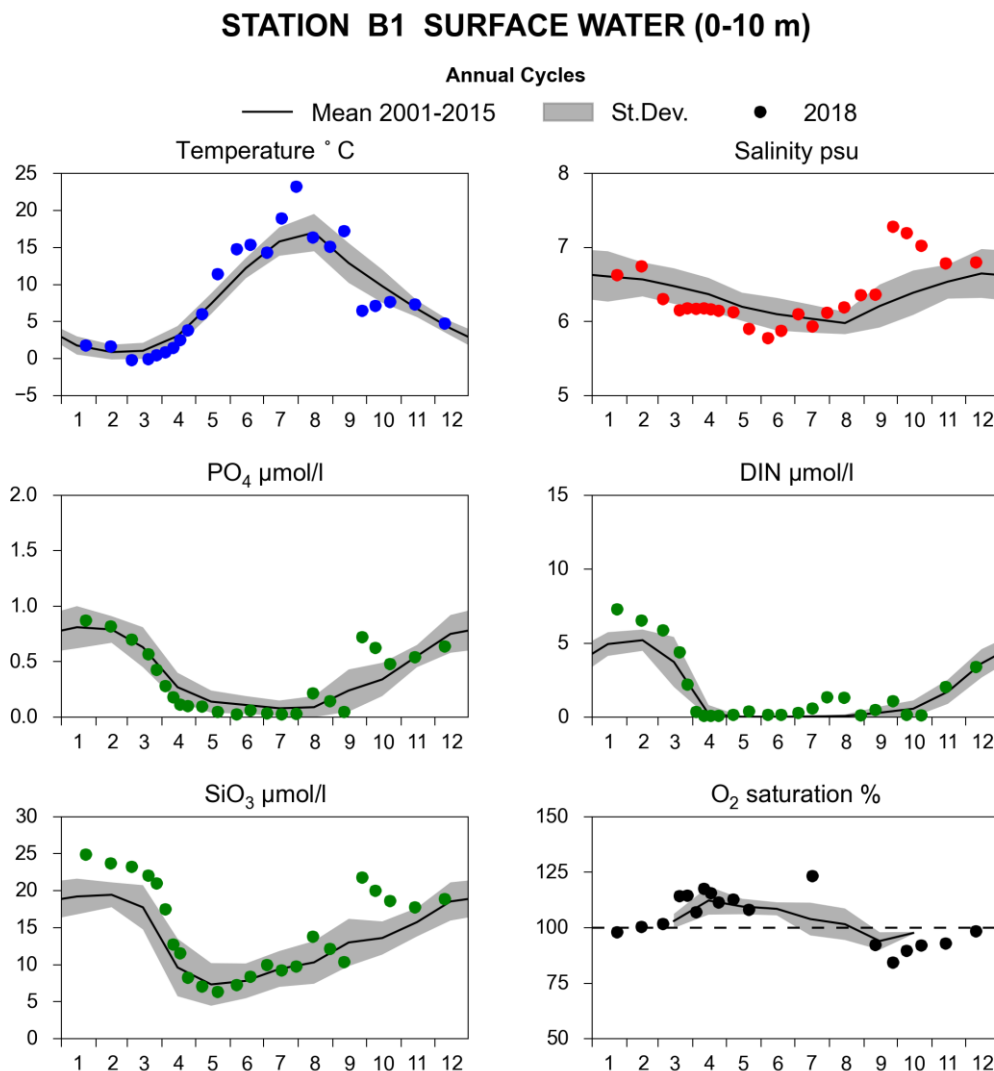
Figure 15 Surface temperature (blue), salinity (red), nutrients (green: DIP, DIN and silicate) and oxygen saturation (black) at the coastal station B1 in 2018. Oxygen data from the surface is missing from most visits during summer due to difficulties with calibration of the sensor for warm waters.
