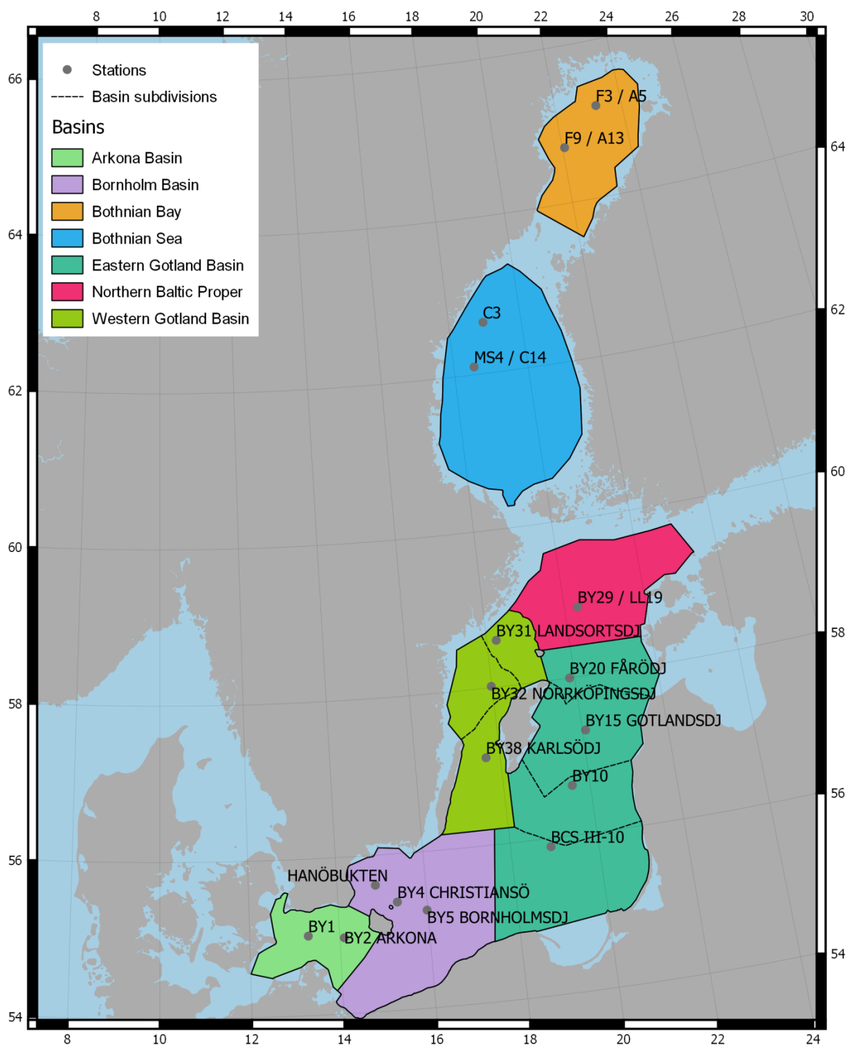
Figure 1 Basin subdivisions used for calculating hypsography and then basin content of sub-basins. The major basins shown in different colours are the HELCOM basin division revised in 2018. The previous basin division placed the station BY31 in the Northern Baltic Proper. The dashed lines showing the sub-basins were drawn to follow the bathymetry to get a smaller basin that the individual monitoring station better represents.
