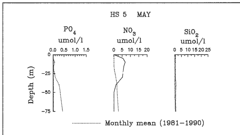
Figure 3.1.2 Nutrient profiles from the station HS5 in southern Skagerrak, together with mean profiles for May, for the period 1981-1990.
