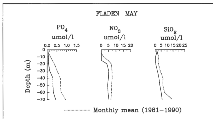
Figure 3.2.3 Nutrient profiles from the station Fladen in northern Kattegat, together with mean profiles for May, for the period 1981-1990.
