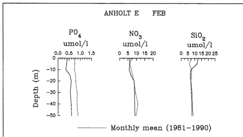
Figure 3.2.2 Nutrient profiles from the station Anholt E in central Kattegat, together with mean profiles for February, for the period 1981-1990.
