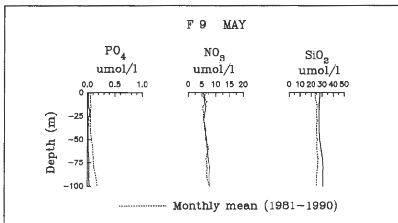
Figure 3.4.2 Nutrient profiles from the station F9 in the Bothnian Bay together with mean profiles for May for the period 1981-1990.
