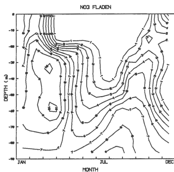
Figure 3.2.13 Isopleths showing the depth distribution of temperature, salinity, oxygen, \text{PO}_4 and \text{NO}_3 as a function of time during the year for the station Fladen in northern Kattegat.
