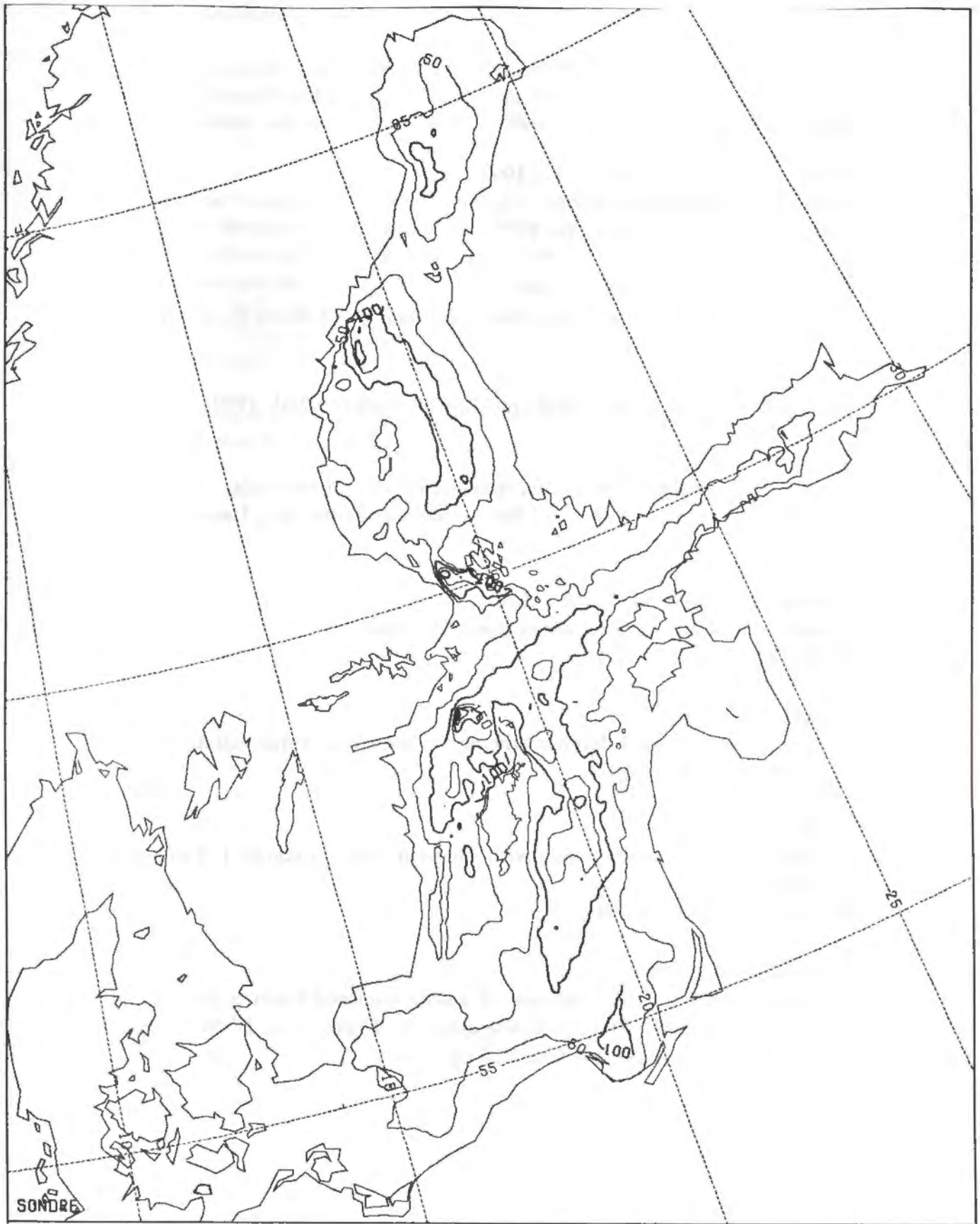
Figure 3. Depths for the Baltic Sea model. Isolines are shown for every 50 m.
