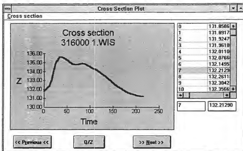
Figure 16. Calculated water level hydrograph for the cross section at km 316 in Vistula river.
