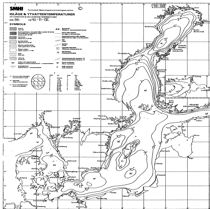
Figure 23: Modelled sea surface temperature (in °C) from November 2, 1992, compared with the corresponding sst chart published by SMHI.
