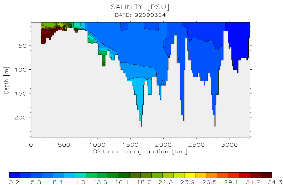
Figure 20: Salinity section (in PSU) through the whole Baltic Sea from Kattegat to Bothnian Bay from May 18 and September 3, 1992. The same colour bars are used.
