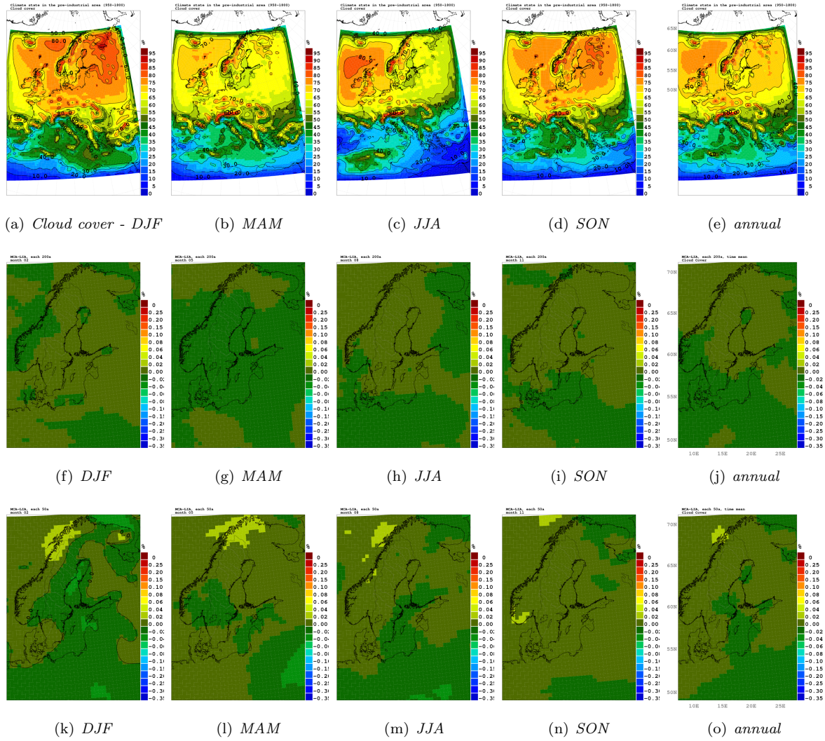
Figure 21. Same as Fig. 16 only for cloud cover.
