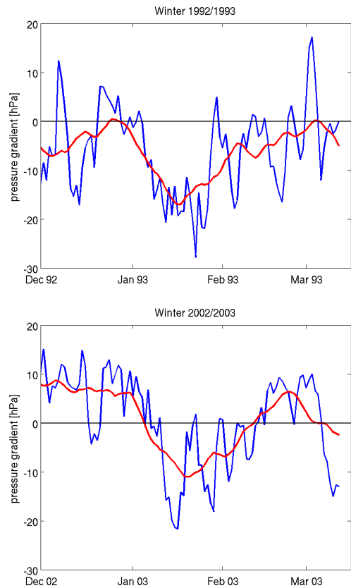
Figure 2. SLP differences [hPa] between Oksøy (Norway) and De Bilt (Netherlands). Blue lines indicate daily values. Red lines show the 20 day running mean. Figures are for the major inflows in January 1993 (top) and January 2003 (bottom).
