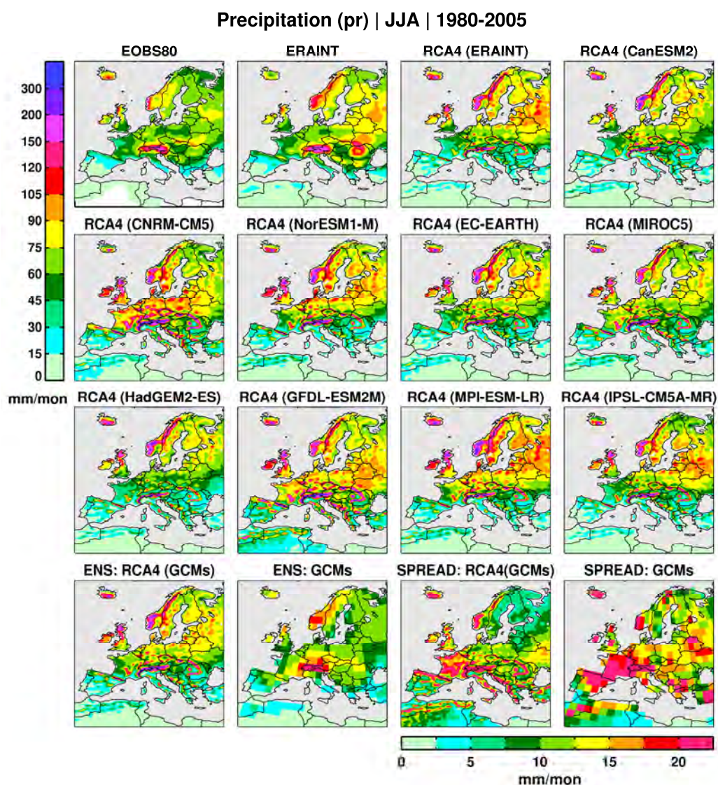
Figure A6. Summer (June – August) precipitation (mm/mon) in the recent past climate, 1980–2005, according to E-OBS, ERAINT, RCA4 forced with ERAINT and RCA4 forced with 9 different GCMs (rows 1–3). Bottom row: ensemble mean in RCA4 forced by GCMs, ensemble mean in GCMs, spread between members in the RCA4 GCM ensemble and spread in the GCM ensemble given as standard deviation.
