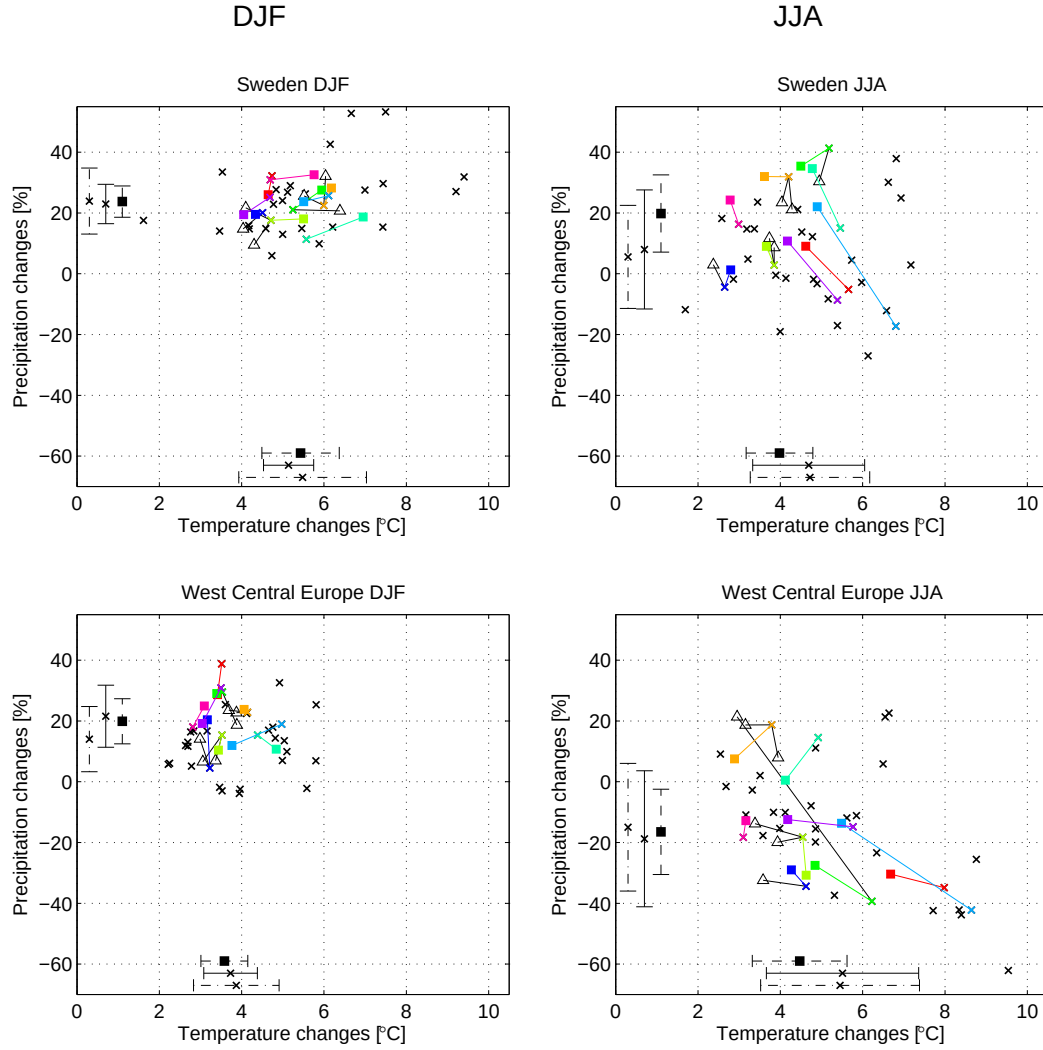
Figure 29. Temperature (°C) and precipitation (%) changes 2071-2100 compared with 1971-2000 for winter (DJF, left column) and summer (JJA, right column); Sweden (top row) and West Central Europe (bottom row). Filled squares represent RCA4 simulations, connected by a line to the corresponding GCM (cross of the same colour as the square). Black crosses represent other CMIP5 GCMs. Triangles indicate simulations with other RCMs than RCA4. Mean values and \pm 1 standard deviations are shown along the x-axis for temperature and the y-axis for precipitation for: the full GCM ensemble (represented by crosses for mean values and dash dotted line for \pm 1 standard deviation), the ensemble of GCMs used by RCA4 (crosses and full lines) and the RCA4 ensemble (filled squares and dashed lines).
