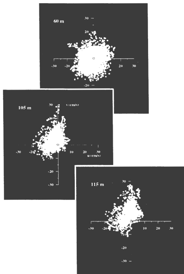
Figure 7. u -components vs v -components from the station F9 during the first observation period. The direction of the transports at 60 m depth are highly fluctuating, while they near the bottom tends to follow the local bathymetry. The velocities are occasionally extremely high near the bottom.
