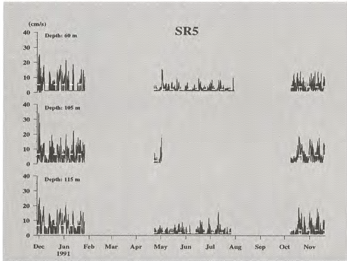
Figure 6. Current speed from the station SR5 during the Open Sea Experiment. The average speed for every period and observation depth is marked with a white dashed line. Corresponding speeds from the stations US5B and F9 are found in Appendix C5 - C6
