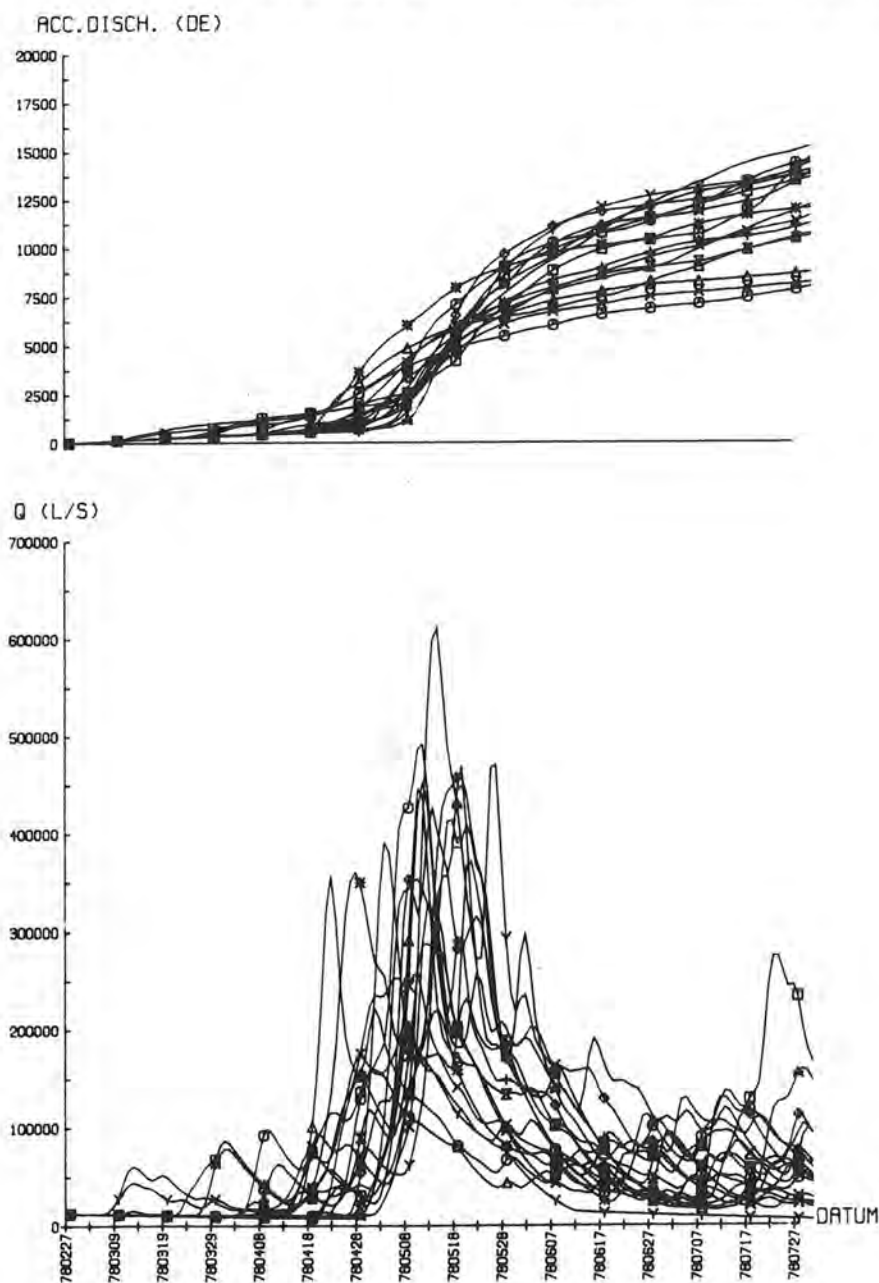
Figure 7. Example of a long range hydrological forecast by the HBV model. The lower graphs show alternative discharge simulations and can be used to judge the risk for flooding. The upper graphs show the corresponding cumulative values and are useful for reservoir operation. (Trängslet basin, 4 483 km 2 .)
