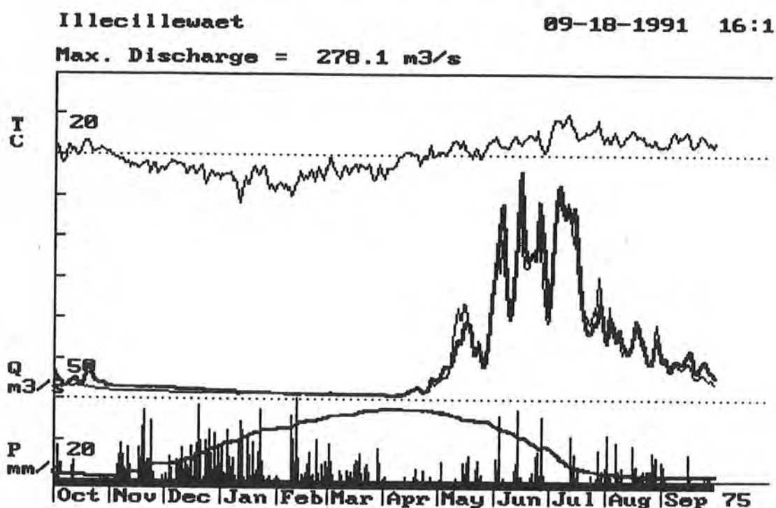
Figure 14e. Example of simulation by the HBV model in Canada for the Illecillewaet basin in the Rocky Mountains for the hydrological year of 1974-75. The basin size is 1 155 km 2 and the model is divided into two submodels.
