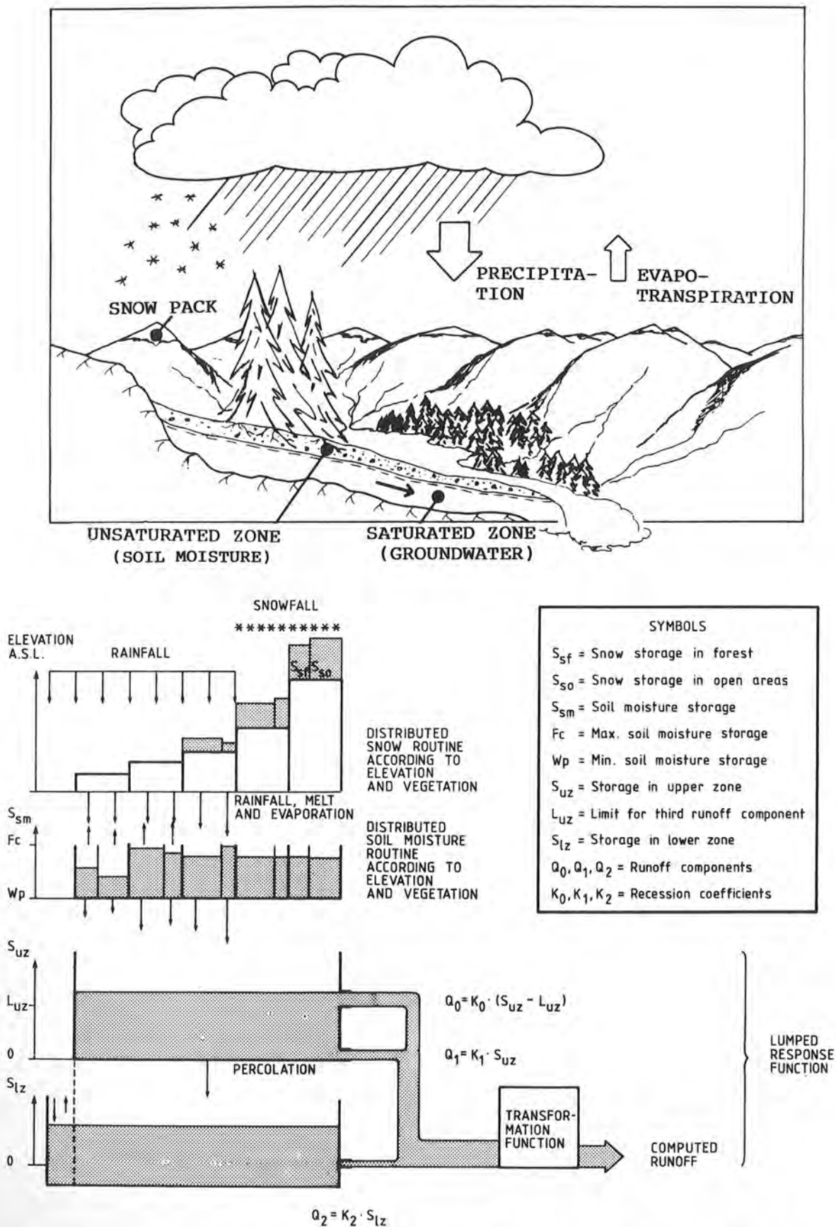
Figure 2. The general structure of the SMHI version of the HBV model when applied to one subbasin.
