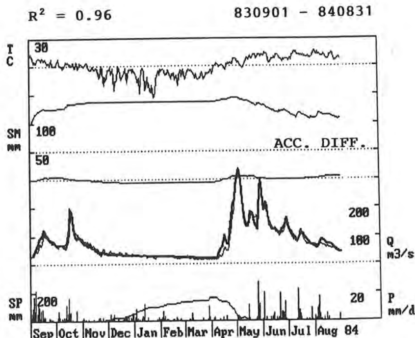
Figure 6. Example of graphical presentation of output from a good model simulation in the Höljes basin in 1983-84. T = air temperature, SM = soil moisture, Q = runoff (thin line = observed, thick line = computed), SP = snowpack, P = precipitation.
