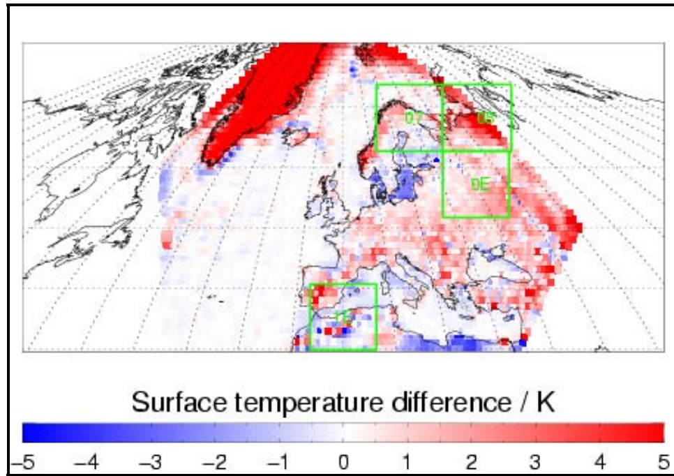
Figure 6. Monthly bias of surface temperature between the HIRLAM and ECMWF NWP analyses, calculated on a 1^\circ resolution. Data shown is for May 2005. The green squares show the sub-regions used for further studies in satellite resolution.
