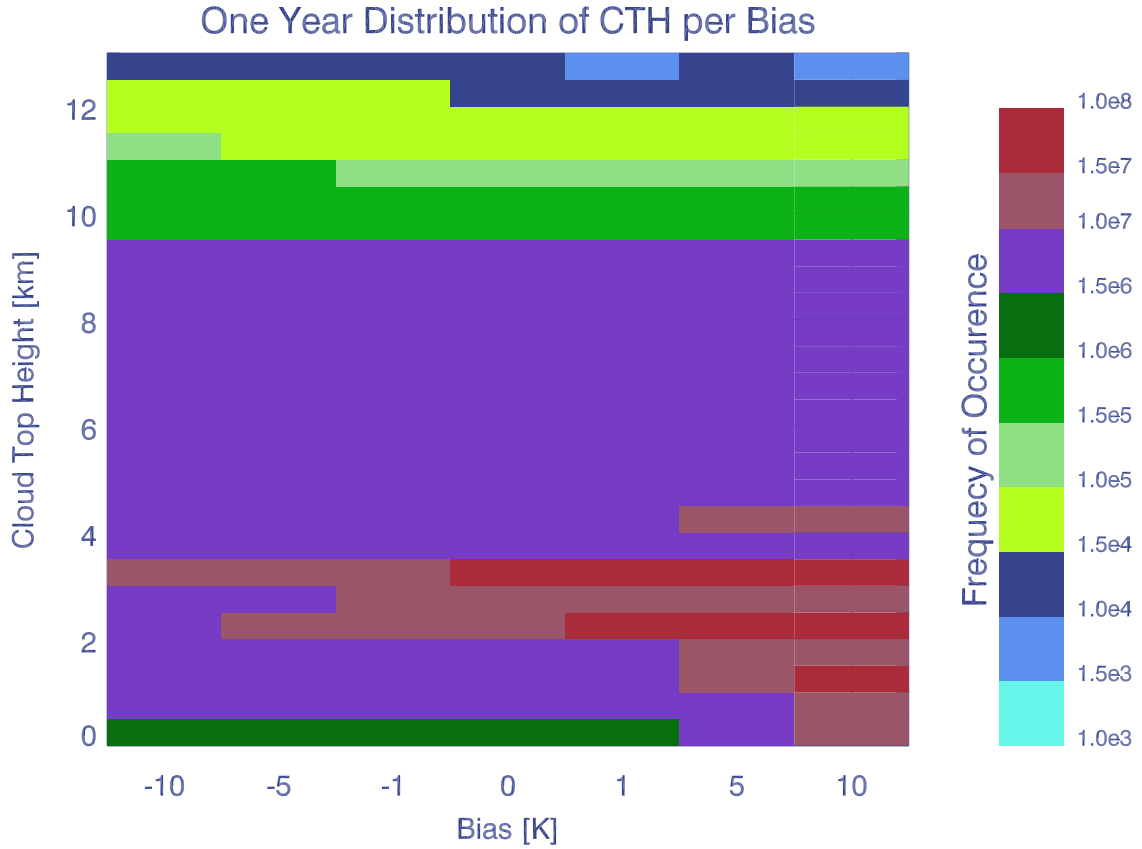
Figure 4. Absolute frequency (i.e., number of pixels) of cloud top height categories (in bins of 500 m vertical resolution) as a function of surface temperature perturbation (bias) value.
