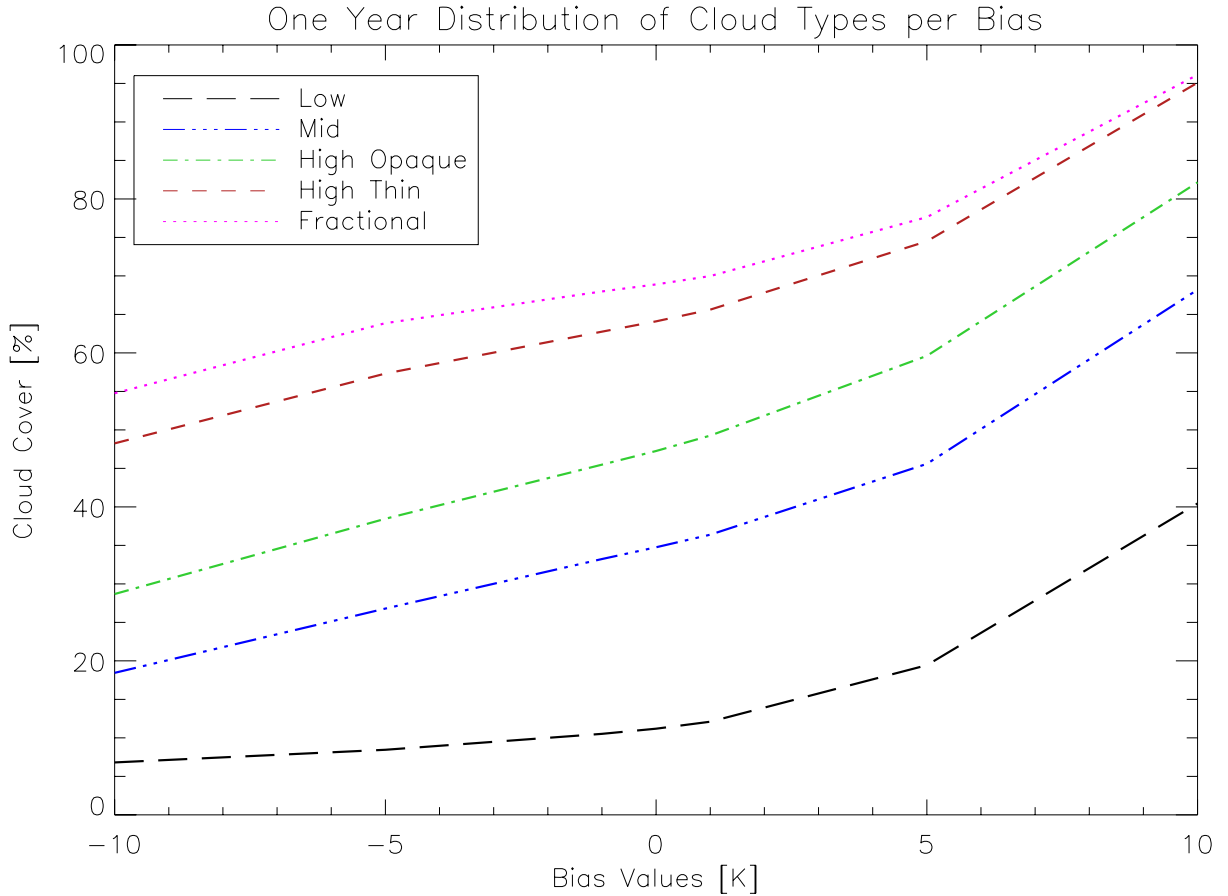
Figure 3. Accumulated contributions to the total area mean cloud cover from five sub-groups of clouds as a function of surface temperature perturbation (bias) value. Notice that curves show contributions that are subsequently added; first for Low, then added in the order Mid, High Opaque, High Thin and Fractional, which means that the curve for Fractional shows the final total area mean cloud cover.
