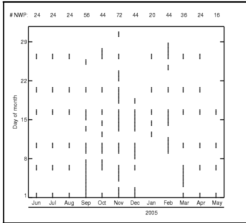
Figure 5. Temporal coverage of the NWP datasets available for this work. Each dot represents one NWP analysis. The numbers on top give the total number of datasets per month (out of possible 124).
