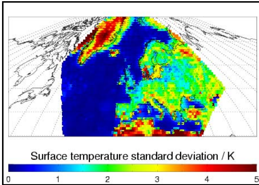
Figure 7. Monthly standard deviation of surface temperature difference between the HIRLAM and ECMWF NWP analysis, calculated on a 1^\circ grid resolution. Data shown is for May 2005.
