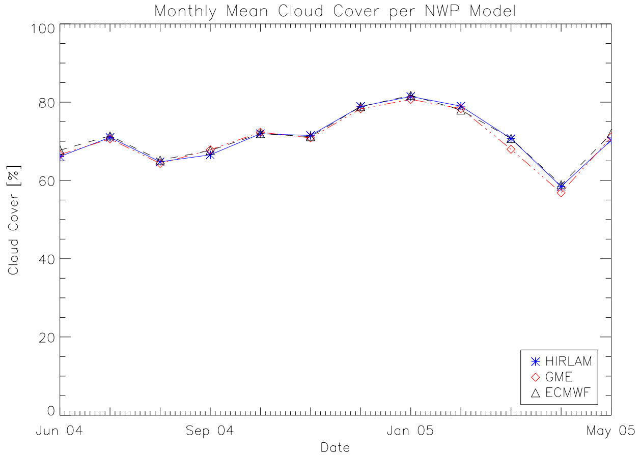
Figure 10. Time-series of PPS-derived monthly mean cloud cover over the Baltrad1km are for each NWP model used as background information for the PPS cloud software.
