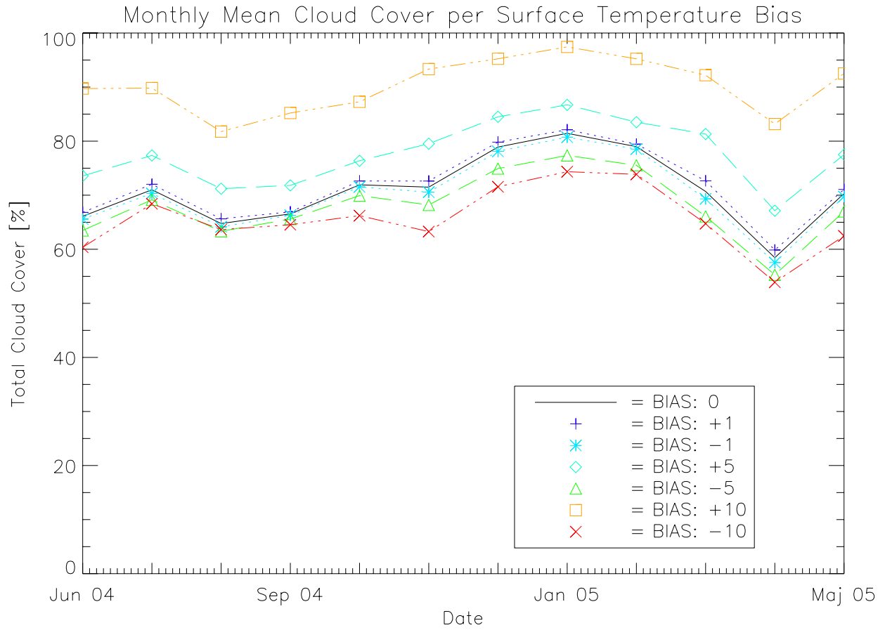
Figure 2. Time-series of monthly mean cloud cover for each value of the surface temperature perturbation (bias).
