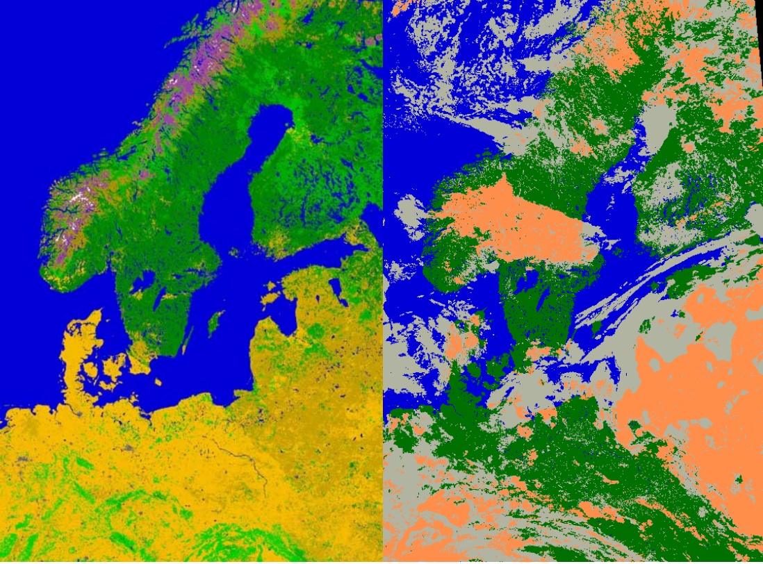
Figure 1. Overview of the Baltrad1km area ( left , colours corresponding to different USGS land use categories) and a corresponding PPS Cloud mask product ( right , opaque clouds in orange and thin clouds in grey) over this area from April 16 2005 at 20:52 UTC.
