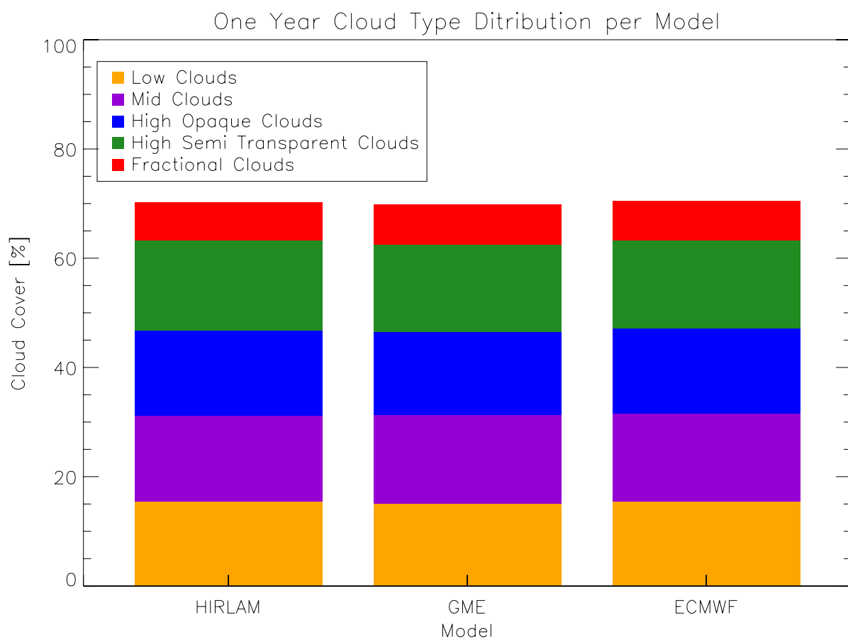
Figure 11. Accumulated total contributions to the total cloud cover from five cloud type categories over the Baltrad1km in the period June 2004 to May 2005 for each NWP model.
