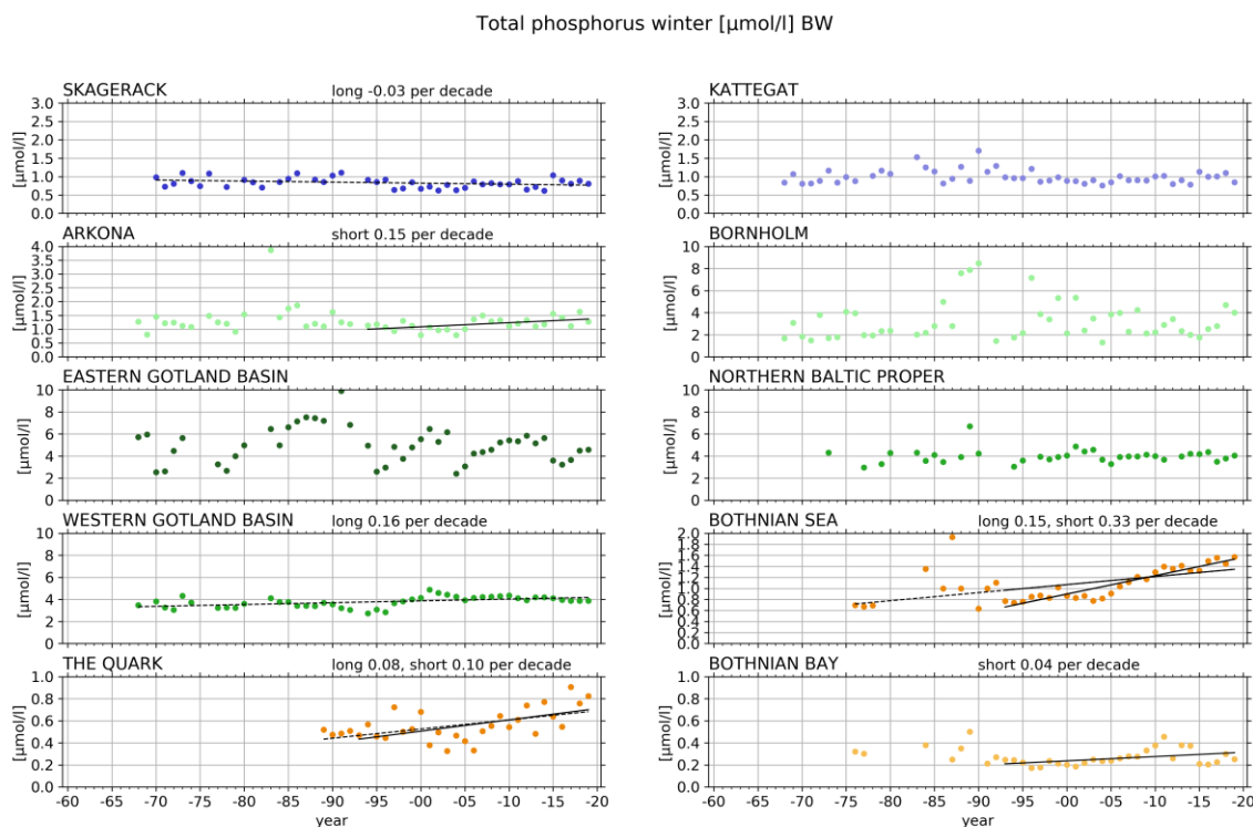
Figure 34. Winter mean concentration of total phosphorus in the bottom water, the Skagerrack and the Kattegat in blue, the Baltic Proper in green and the Gulf of Bothnia in orange. A line is shown when the p-value of the slope is \leq 0.05 , dashed line are shown for the longer time series.
