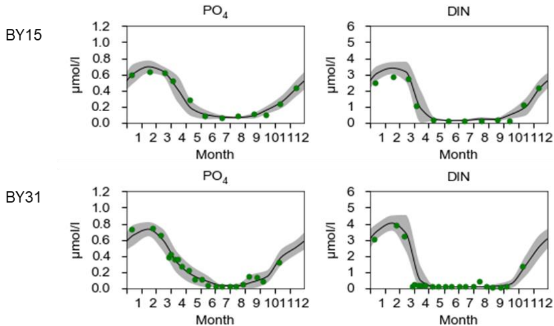
Figure 15. Surface mean (0-10 m) of phosphate (left) and dissolved inorganic nitrogen (right) at two stations in the Baltic Proper, BY15 in the Eastern Gotland Basin (top) and BY31 in the Western Gotland Basin (bottom). The decrease in dissolved inorganic nitrogen in spring shows variation in the time of the spring bloom.
