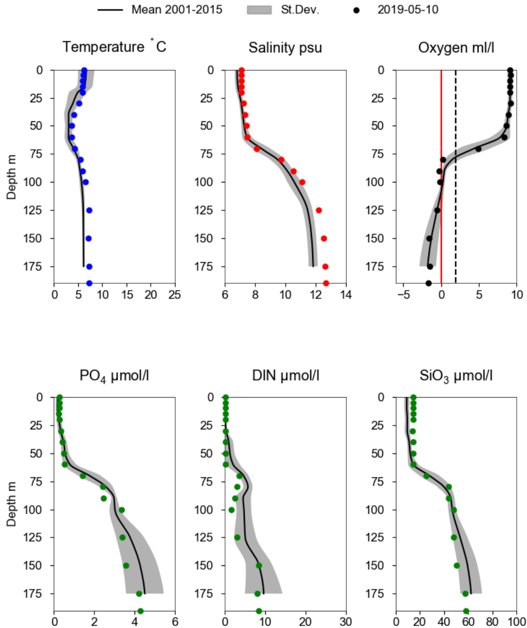
Figure 16. Vertical profiles from station BY20, Fårödjupet in the Eastern Gotland Basin in May 2019. Parameters shown in the top panel, from left to right are; temperature (blue), salinity (red), oxygen (black) and nutrients (green).. In the bottom panel, from left to right; phosphate, dissolved inorganic nitrogen and silicate. The vertical lines in the top, right panel show the limit for zero oxygen (red) and 2 ml/l (black dashed) oxygen concentration, negative values represent hydrogen sulphide recalculated to equivalent oxygen concentration.
