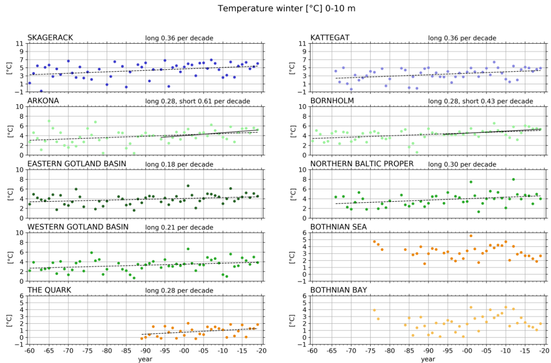
Figure 25. Winter mean values and trends for surface temperature, the Skagerrak and the Kattegat in blue, the Baltic Proper in green and the Gulf of Bothnia in orange. There are significant trends in all basins except the Gulf of Bothnia. A line is shown when the p-value of the slope is \leq 0.05 , dashed line are shown for the longer time series and solid line for the post-1994 time series.
