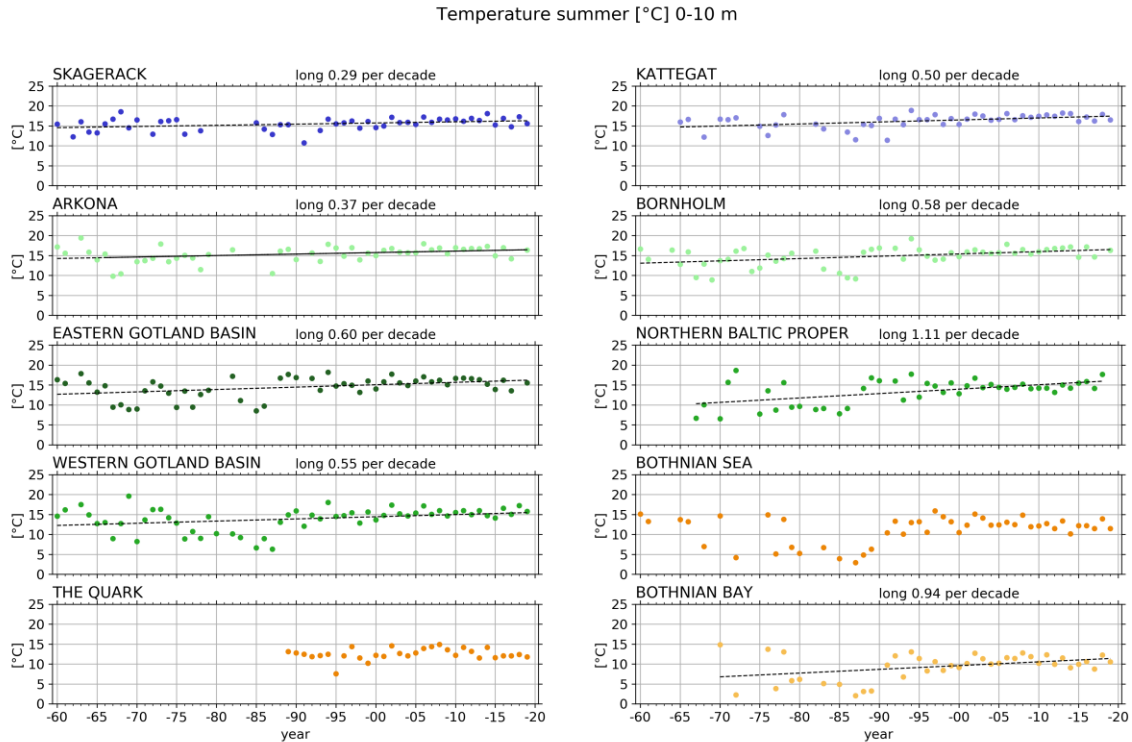
Figure 26. Summer mean values and trends for surface temperature, the Skagerrak and the Kattegat in blue, the Baltic Proper in green and the Gulf of Bothnia in orange. There are significant trends in all basins except the Bothnian Sea and the Quark. A line is shown when the p-value of the slope is \leq 0.05 , dashed line are shown for the longer time series and solid line for the post-1994 time series.
