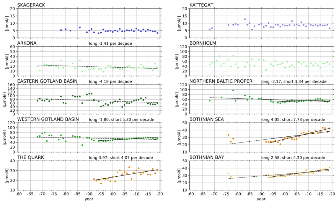
Figure 36. Winter mean concentration of dissolved silica in the bottom water, the Skagerrak and the Kattegat in blue, the Baltic Proper in green and the Gulf of Bothnia in orange. A line is shown when the p-value of the slope is \leq 0.05 , dashed line are shown for the longer time series.
