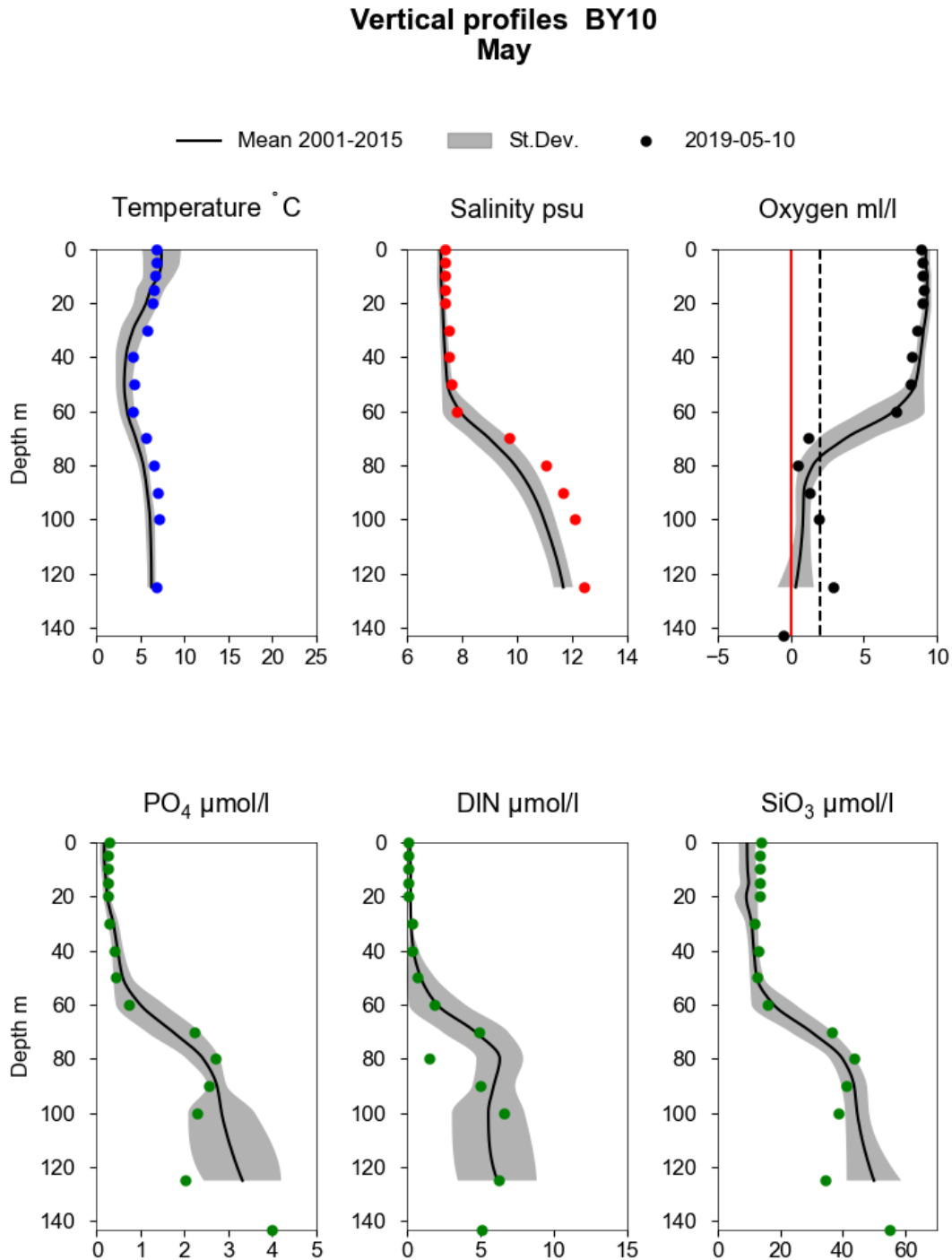
Figure 17. Vertical profiles from station BY10 in the Eastern Gotland Basin in May 2019. Parameters are temperature (blue), salinity (red), oxygen (black) and nutrients (green) in bottom row from left to right; phosphate, dissolved inorganic nitrogen and silicate. Traces of an inflow from the Kattegat can be seen in increase salinity and oxygen below 80 m. Associated with this are also changes in nutrient concentration. The vertical lines in the top, right panel show the limit for zero oxygen (red) and 2 ml/l (black dashed) oxygen concentration, negative values represent hydrogen sulphide recalculated to equivalent oxygen concentration.
