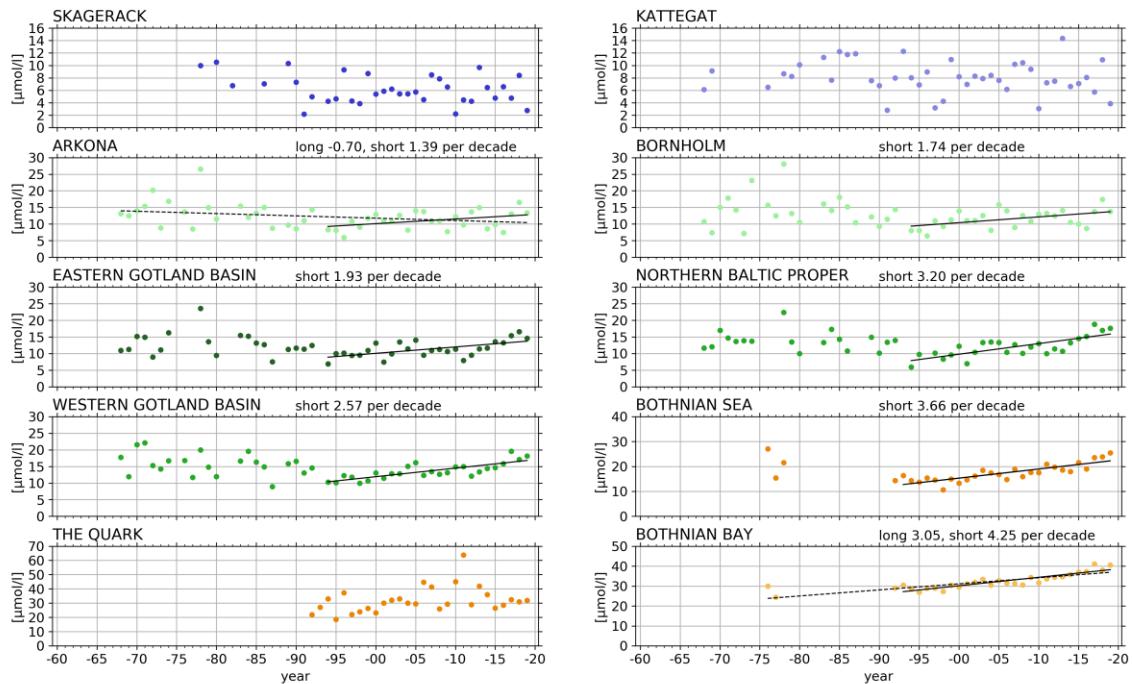
Figure 35. Winter mean concentration of dissolved silica in the surface water, the Skagerrak and the Kattegat in blue, the Baltic Proper in green and the Gulf of Bothnia in orange. A line is shown when the p-value of the slope is \leq 0.05 , dashed line are shown for the longer time series.
