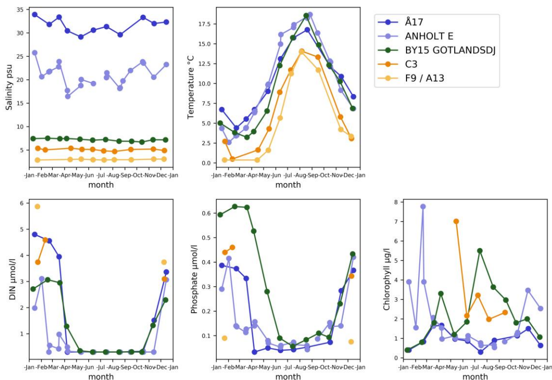
Figure 4. Selection of parameters from the different sea areas around Sweden: the Skagerrak (Å17), the Kattegat (Anholt E), the Baltic Proper (BY15), the Bothnian Sea (C3), the Bothnian Bay (F9/A13). All parameters are mean values of surface water (0-10 m).
