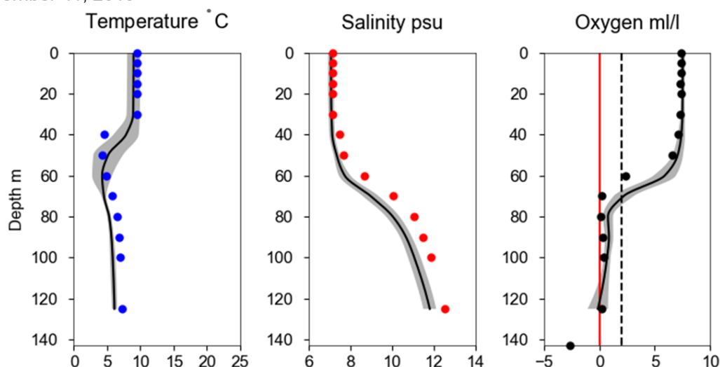
Figure 14. Temperature (blue), salinity (red) and oxygen (black) profiles from station BY10, top panel is from October 15 th 2019 and bottom panel from November 11 th 2019. The vertical lines in the right panel show the limit for zero oxygen (red) and 2 ml/l (black dashed) oxygen concentration, negative values represent hydrogen sulphide recalculated to equivalent oxygen concentration. The salinity had increased between the two observations which indicate inflowing water originating from the more saline Kattegat.
