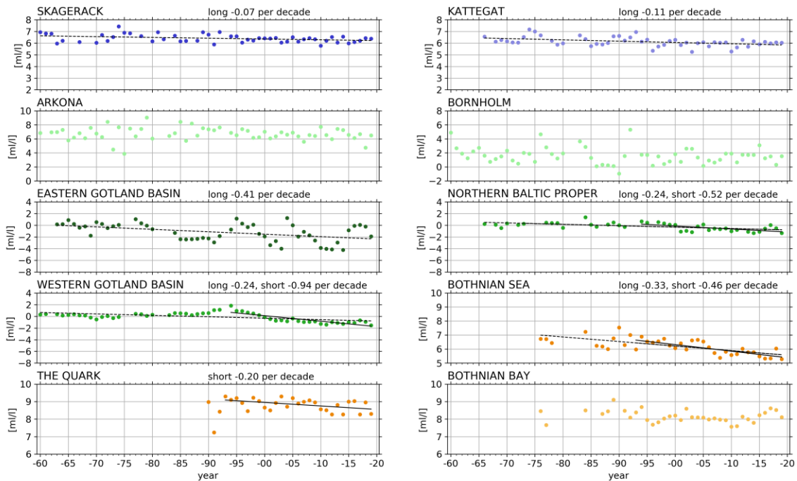
Figure 30. Winter mean oxygen in the bottom water, the Skagerrak and the Kattegat in blue, the Baltic Proper in green and the Gulf of Bothnia in orange. A line is shown when the p-value of the slope is \leq 0.05 , dashed line are shown for the longer time series.
