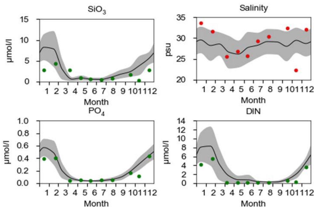
Figure 8. Surface concentrations of inorganic nutrients (green) and salinity (red) at station Å13 in Skagerrak. Unusually low salinity in November together with low nutrient concentrations.
