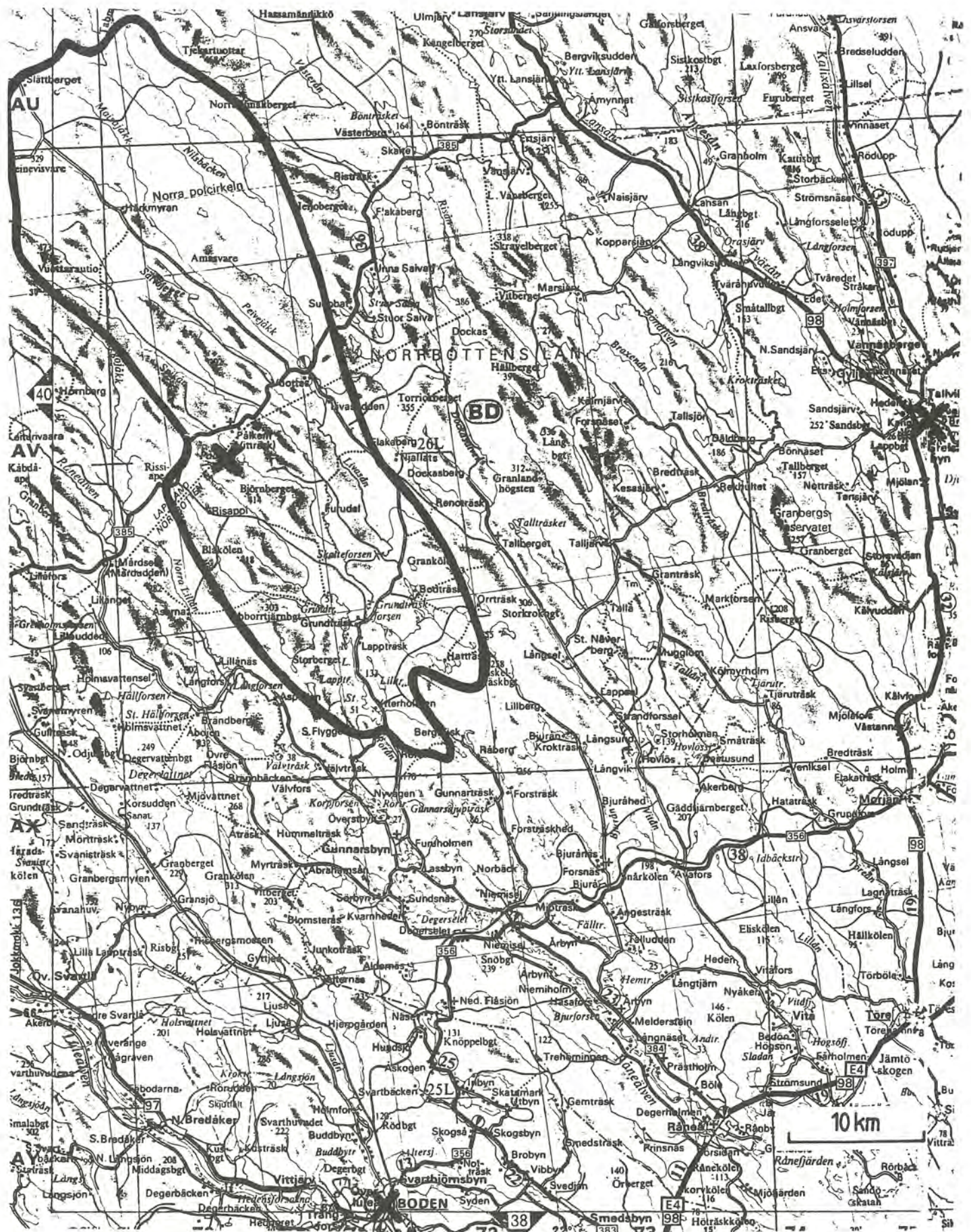
Figure 5 Detailed map showing the representative area of Lappträsket. The synoptic stations of Pålchem (within the area), Boden and Överkalix are marked by crosses.
