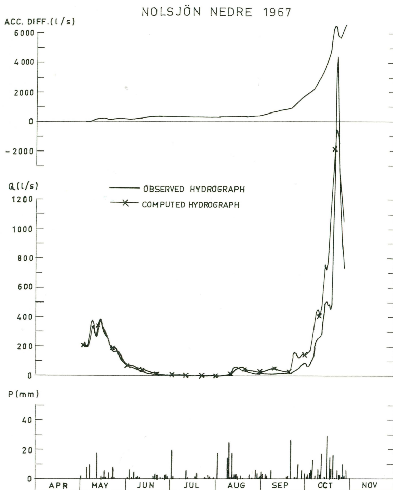
Fig. 8. Simulated year in the Nolsjön catchment.
