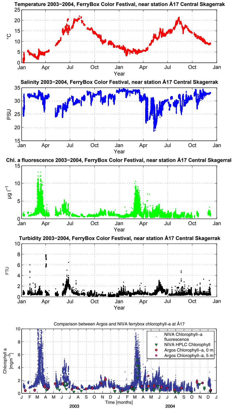
Figure 48. Data from station Å17 in the Skagerrak. In the bottom graph a comparison between chl. a fluorescence from FerryBox-system, water sampling from FerryBox and water sampling from R/V Argos is made. Chl. a from waters samples was analysed after filtering and extraction. Chl. a was analysed using HPLC from the FerryBox samples and using a fluorometric method for the samples from R/V Argos.
