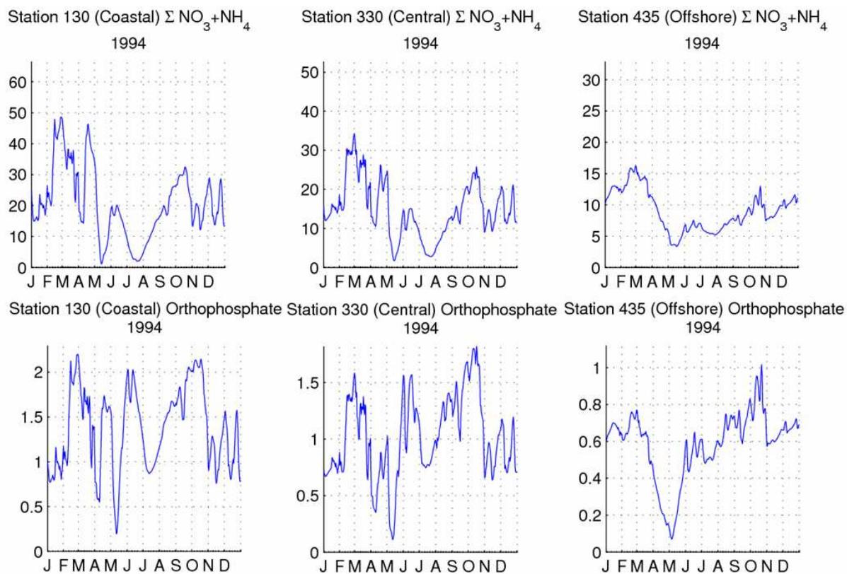
Figure 1 Nutrient cycles (the sum of nitrate and ammonium and DIP) for coastal, central and offshore Belgian waters, 1994. Concentration units are mmol/m 3
