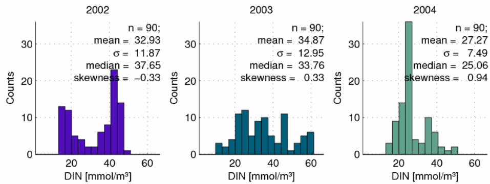
Figure 8 Distributions of winter inshore DIN concentrations, 2002 - 2004. Belgian data
