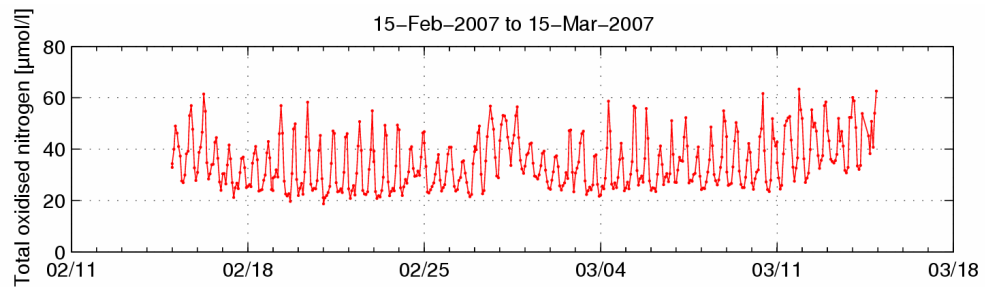
Figure 3 Time series of total oxidised nitrogen, showing the tidal influence on the observations. Data are Crown Copyright
