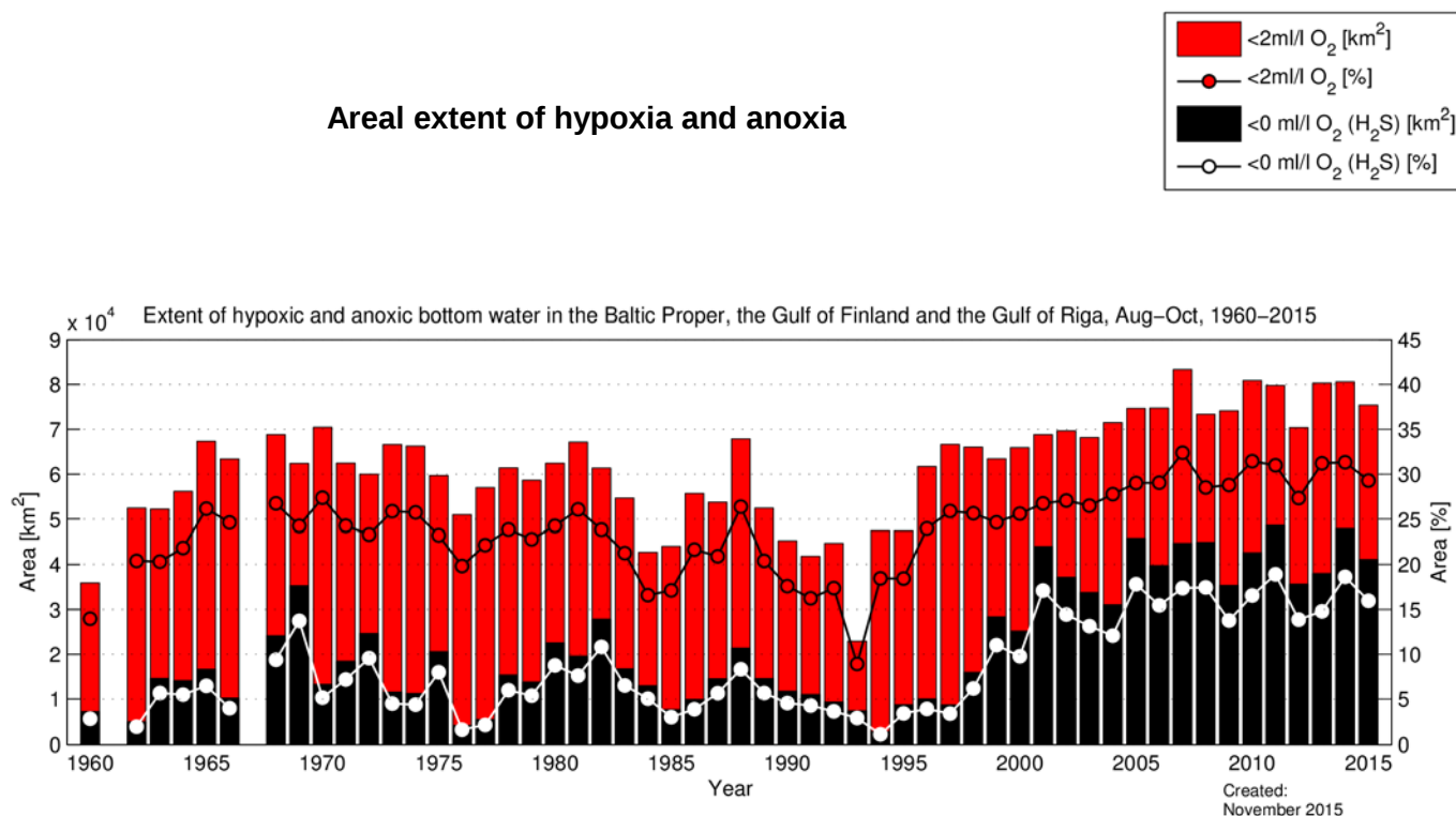
Figure 2. Areal extent of anoxic and hypoxic conditions in the Baltic Proper, Gulf of Finland and Gulf of Riga. Results from 1961 and 1967 have been removed due to lack of data from the deep basins.
