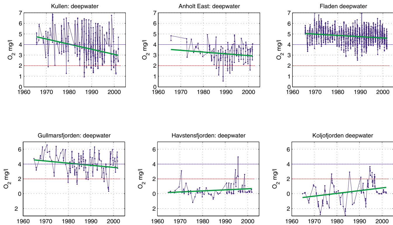
Fig. 2.3.3: Time series of deepwater oxygen levels from Kattegat( Kullen, Anholt, Fladen) and from Skagerrak (Gullmarensfjorden, Koljöfjorden, Havstensfjorden). (cf. Fig. 2.1.1) in offshore Kattegat and inshore Skagerrak.
