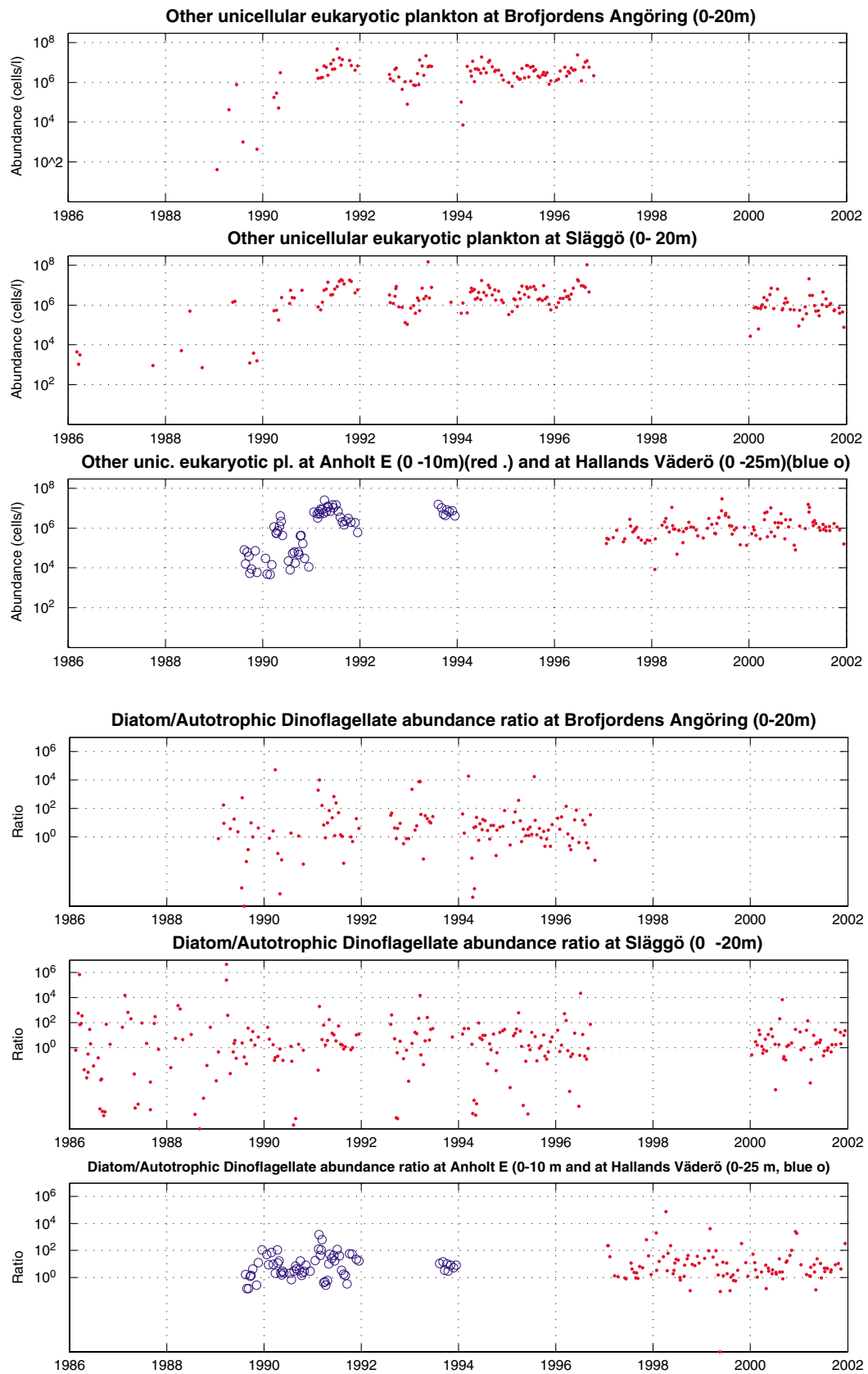
Figure 2.2.13. The abundance of other unicellular eukaryotic plankton (upper panel) and the ratio of the abundance of diatoms/abundance of autotrophic dinoflagellates (lower panel) at four stations in the Skagerrak-Kattegat.
