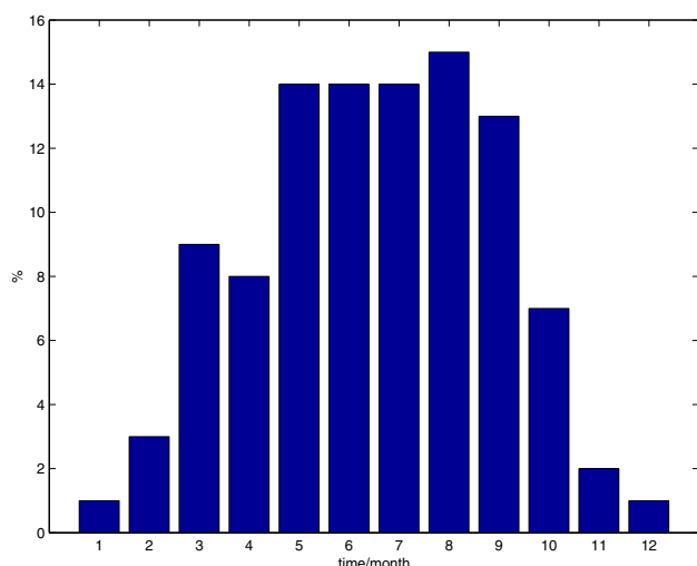
Fig. 2.2.4 The monthly contribution to the annual production.
