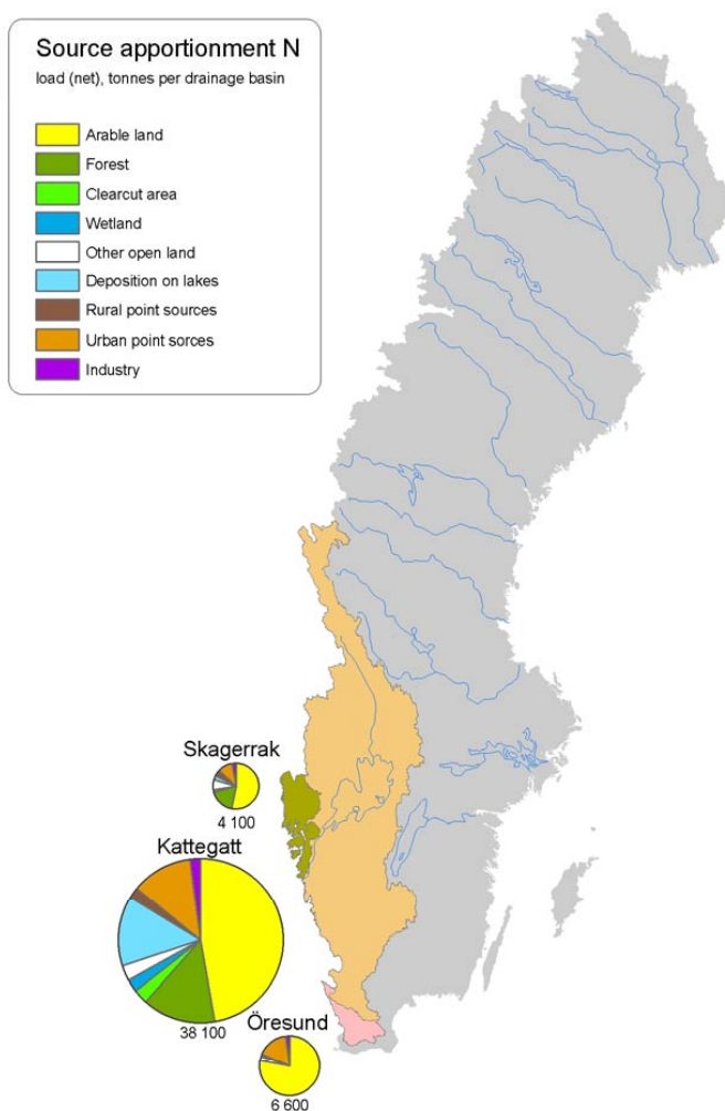
Fig. 2.1.3: Source apportionment for nitrogen net load including point sources that goes direct to the sea. Period 1985-1999.
