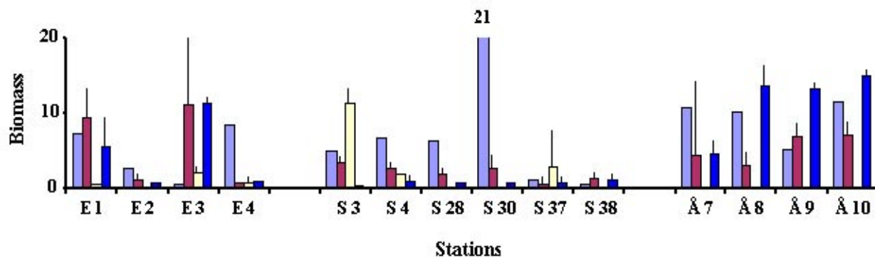
Fig. 2.3.5. Macrofaunal biomass (g wet weight m -2 ) at stations in the Ellösfjord (E), Stigfjord (S) and Åbyfjord (Å) for the years 1976, 1986 (Josefson & Rosenberg, 1988), 1997/98 and 2001 (Rosenberg unpublished), where the first bar is year 1976, etc.
