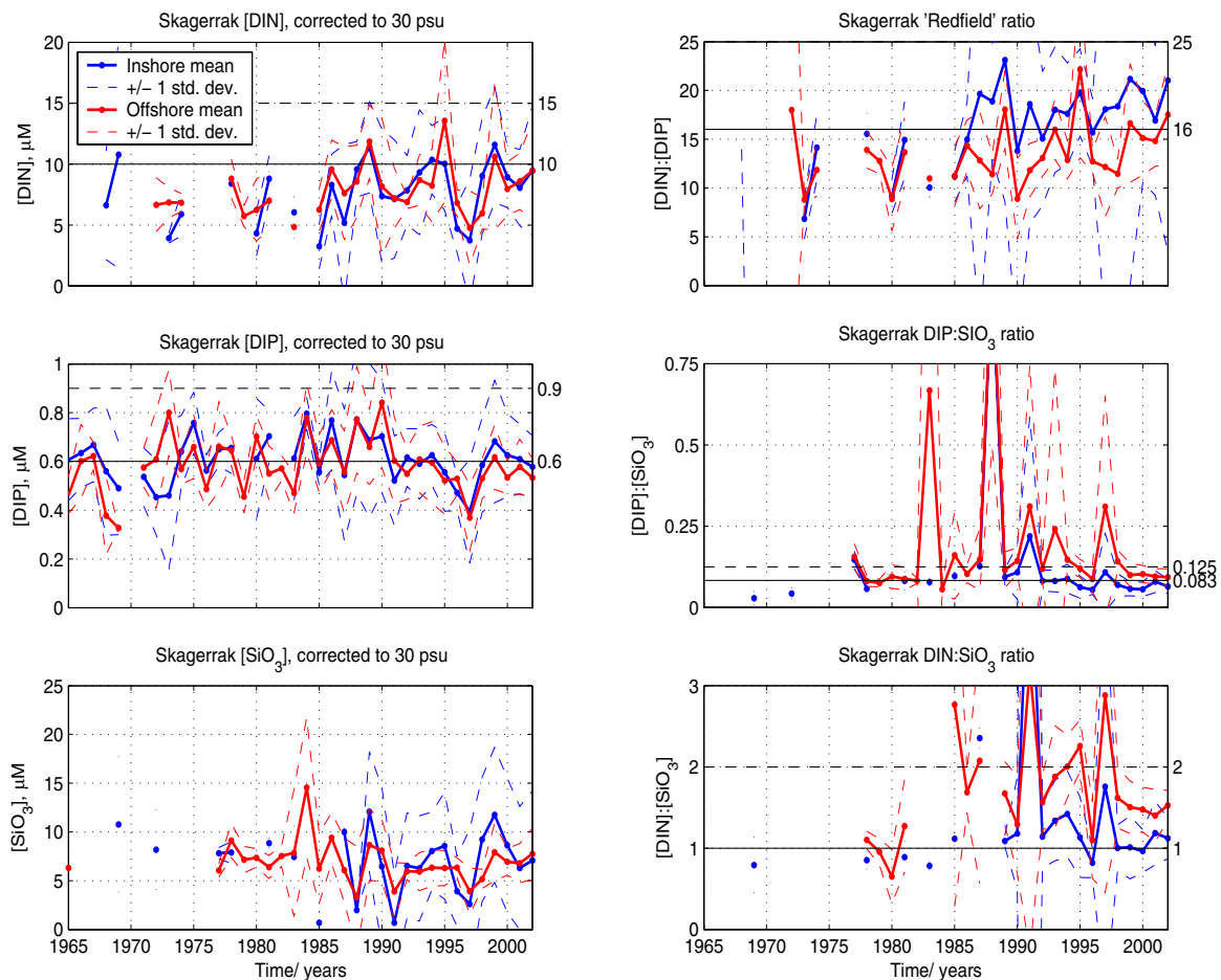
Fig. 2.1.6b: Time series of average nutrient concentrations and nutrient rations, including one standard deviation, of Skagerrak offshore (red dots) and inshore (blue dots) waters. Background value given by solid line and critical value given by dashed line.
