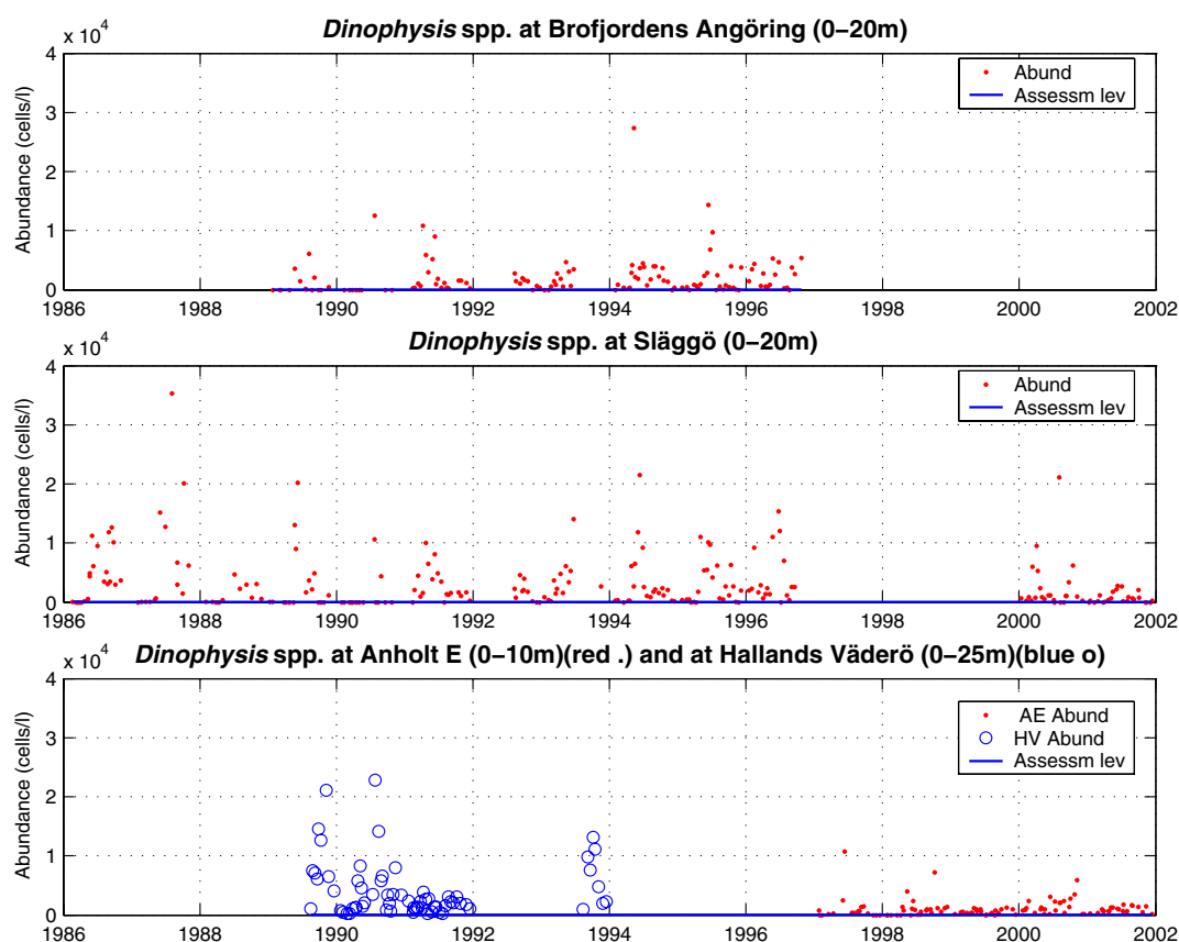
Figure 2.2.9. The abundance of Dinophysis spp. at four stations in the Skagerrak-Kattegat, OSPAR assesment level is 100 cells l -1 .
