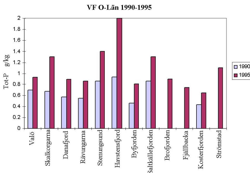
Fig. 2.3.11: The concentration of total phosphorous (g/kg dw) in the surficial sediment at 12 resampled stations along the Bohus Coast in 1990 and 1995, respectively (From Cato 1997b).
