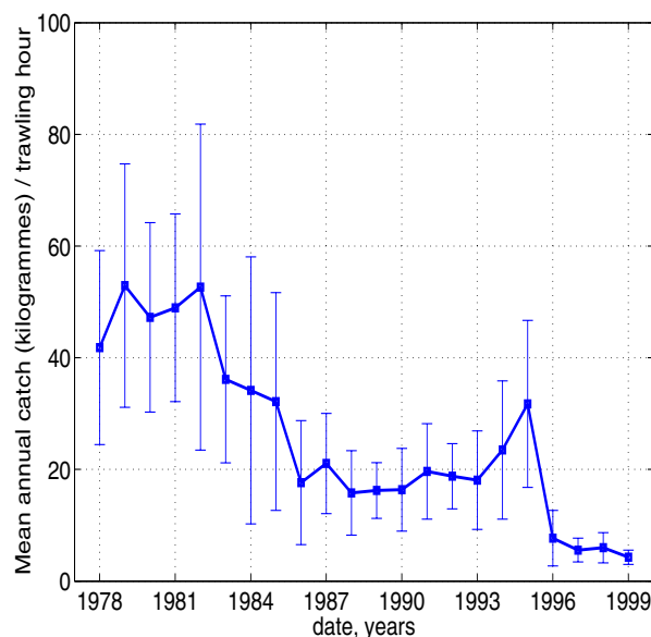
Fig. 2.3.6: A time series of mean annual catch per trawl hour in Skagerrak and Kattegat.
