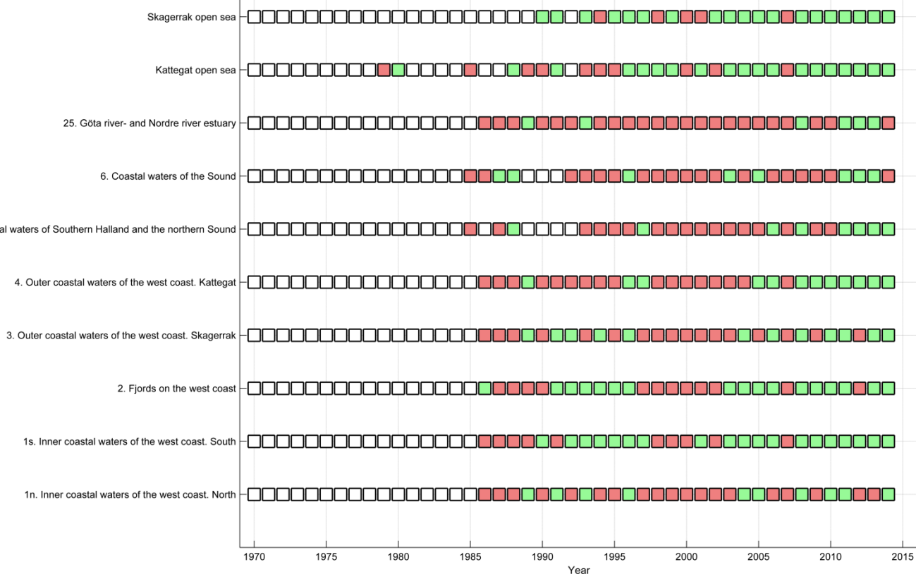
Classification of Secchi (m) in summer
