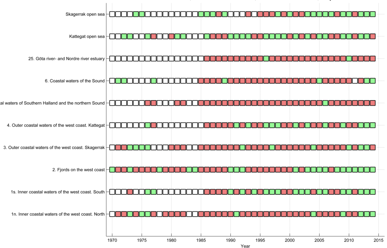
Classification of Secchi (m) in summer
