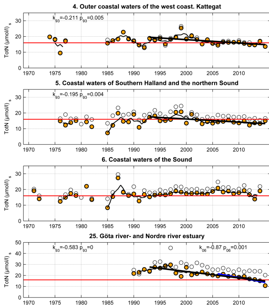
Figure 24. Time series of mean summer Tot-N in coastal water.
