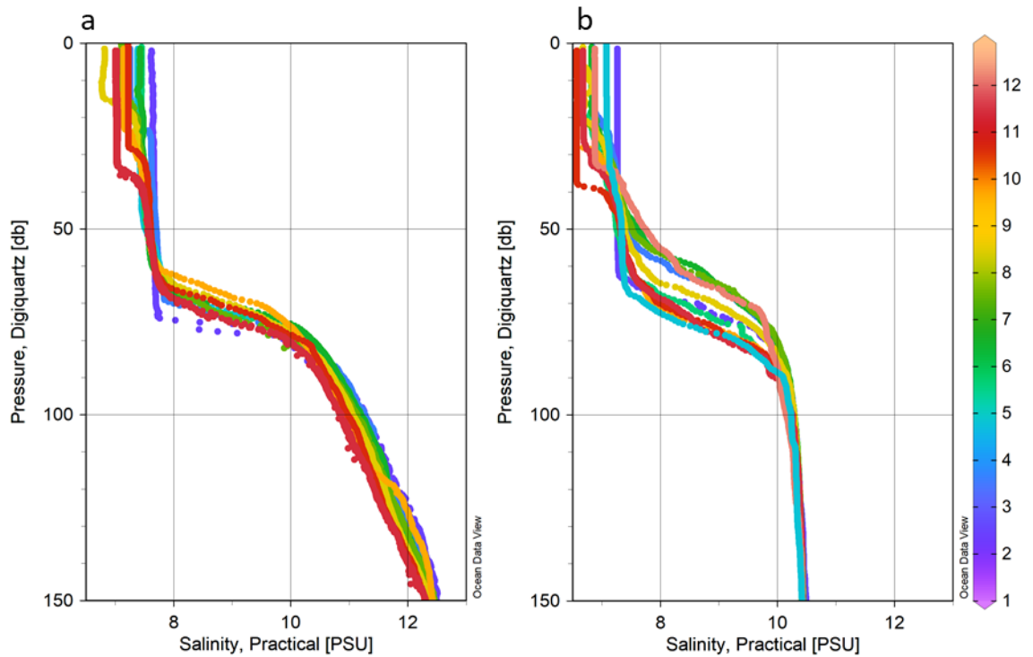
Figure 16 Profiles of salinity at a) BY15 Gotland deep and b) BY32 Norrköping deep from 2022. The figure shows the more variable halocline depth in the Westerns Gotland Basin (b) compared to the Eastern Gotland Basin (a).
