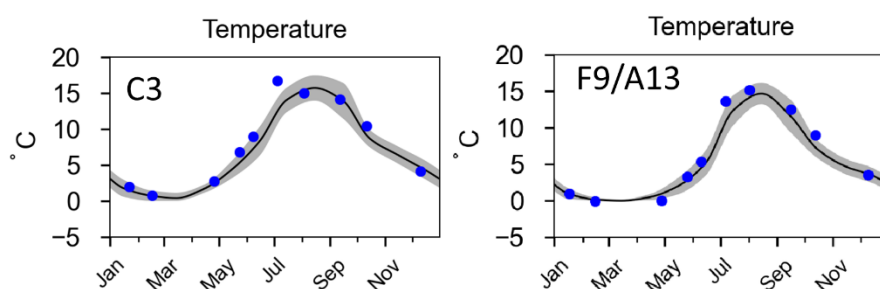
Figure 28. The temperature in the sea surface, 0-10 m, during 2022 at the stations C3 (left) in the Bothnian Sea and F9/A13 (right) in the Bothnian Bay. Monthly measurements (dots) during 2022 are shown in relation to average value for the period 1991-2020 (black line) and \pm 1 standard deviation (grey area).
