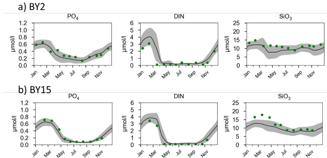
Figure 21. Concentrations of nutrients in the surface water (0-10 m) at stations BY2 in the Arkona Basin (a) and BY15 in the Eastern Gotland Basin (b). To the left: phosphate, middle: dissolved inorganic nitrogen (DIN) and to the right: silicate. Monthly measurements (dots) during 2022 are shown in relation to average value for the period 1991-2020 (black line) and \pm 1 standard deviation (grey area).
