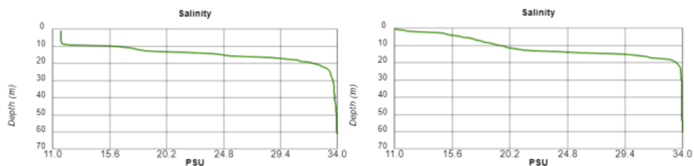
Figure 13. The salinity at station Anholt E in Kattegat. Left 2022-04-21, right 2022-04-26.
