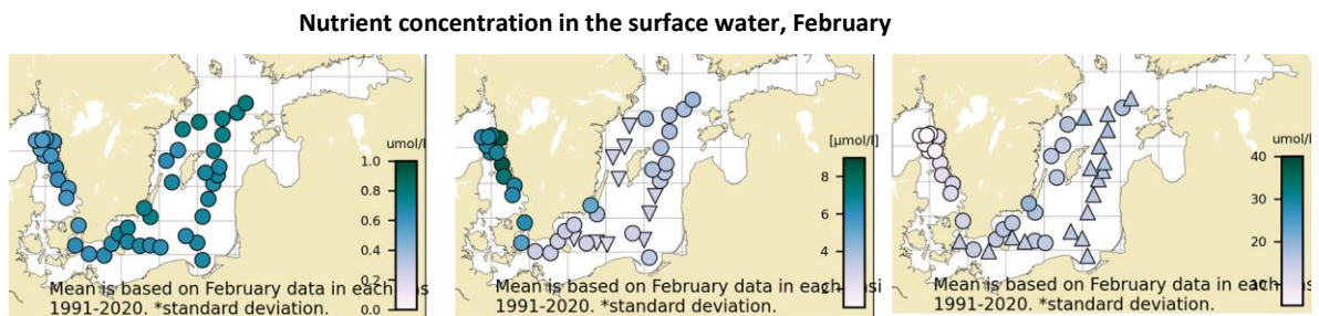
Figure 20. Maps showing the concentration of phosphate (a), dissolved inorganic nitrogen (b) and silicate (c) in February 2022. Circles represent values within \pm 1 standard deviation, upwards and downwards pointing triangles represent values that are above/below \pm 1 standard deviation.
