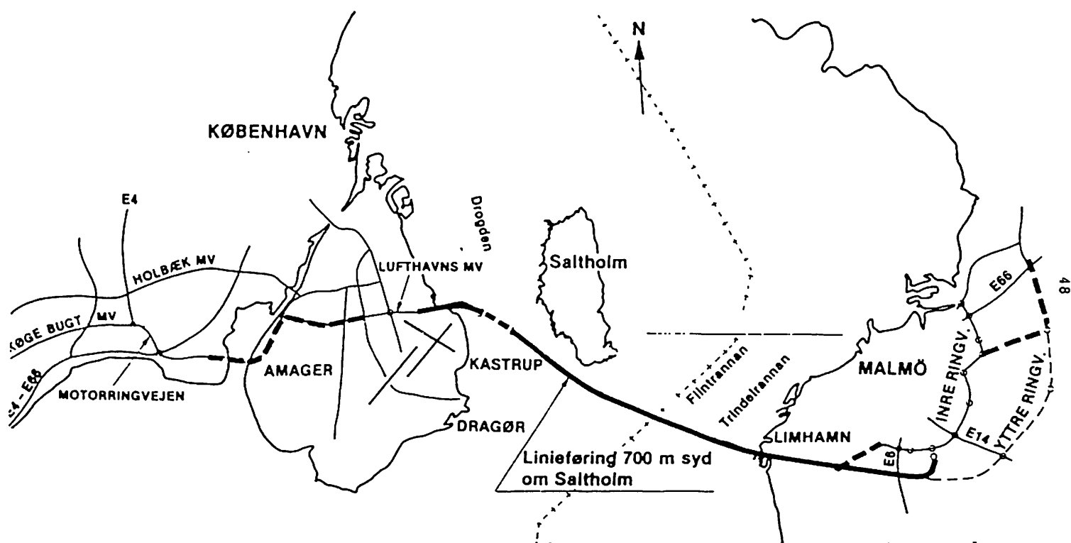
Figure 1. Bridge / tunnel position
