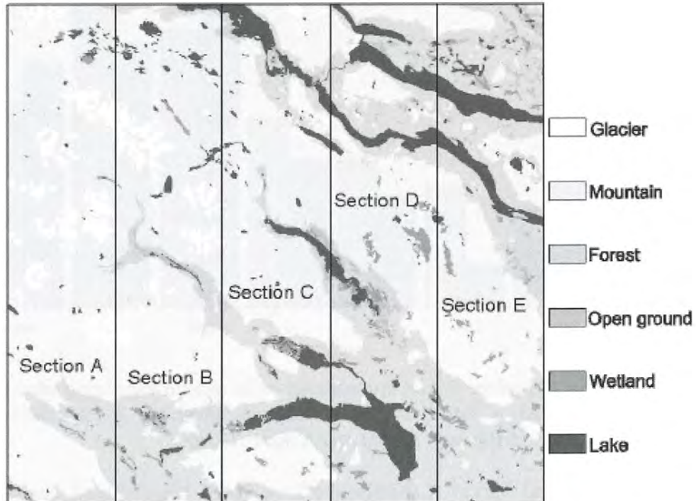
Figure 3 Land cover within the investigated area. Five sections used as sub-divisions for limiting the area for analyses are also marked (sections A-E).
