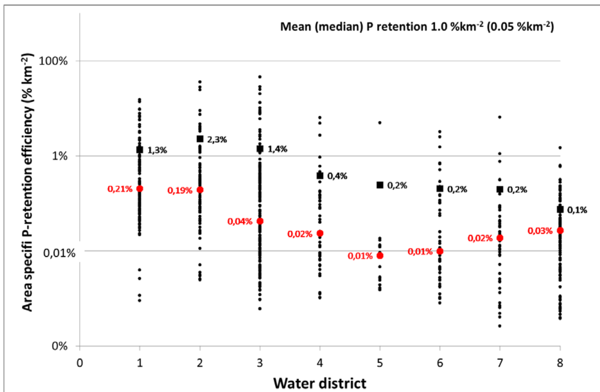
Figure 11. Area-specific phosphorus retention efficiency (R/A) (% km -2 ) of phosphorus in 653 sub-basins of the SCM model. The results are presented for eight different water districts (see Fig. 9). Mean values are shown by black squares and black numbers while the median numbers are shown by red circles and numbers. The mean and median values for all basins are shown in the upper right corner. Note the logarithmic scale on the vertical axes.
