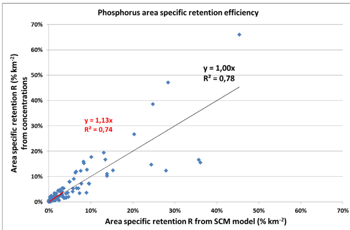
Figure 13. Best linear fit for area-specific phosphorus retention efficiency ( R/A ) calculated from theoretical model including information from the sediment and water column concentrations (Eq.4 and Eq.6 combined) and compared to SCM model results ( R/A ). Best fit for P on all data (653 sub basins) was obtained with \text{Blr(P)}=0.04 \text{ yr}^{-1} . The linear trend for a sub set (613 sub basins) of the data is shown by the red line and the red text.
