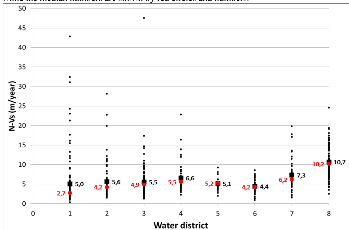
Figure 10. Similar as Fig. 9 but for nitrogen.
