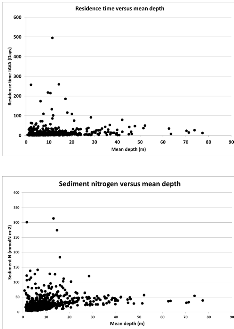
Figure A2. The relation between mean depth and IAVA residence time (days) in the 653 sub-basins of the SCM model is shown in the upper plot. The relation between sediment nitrogen concentrations (mmol N m -2 ) and mean depth is shown in the lower plot.
