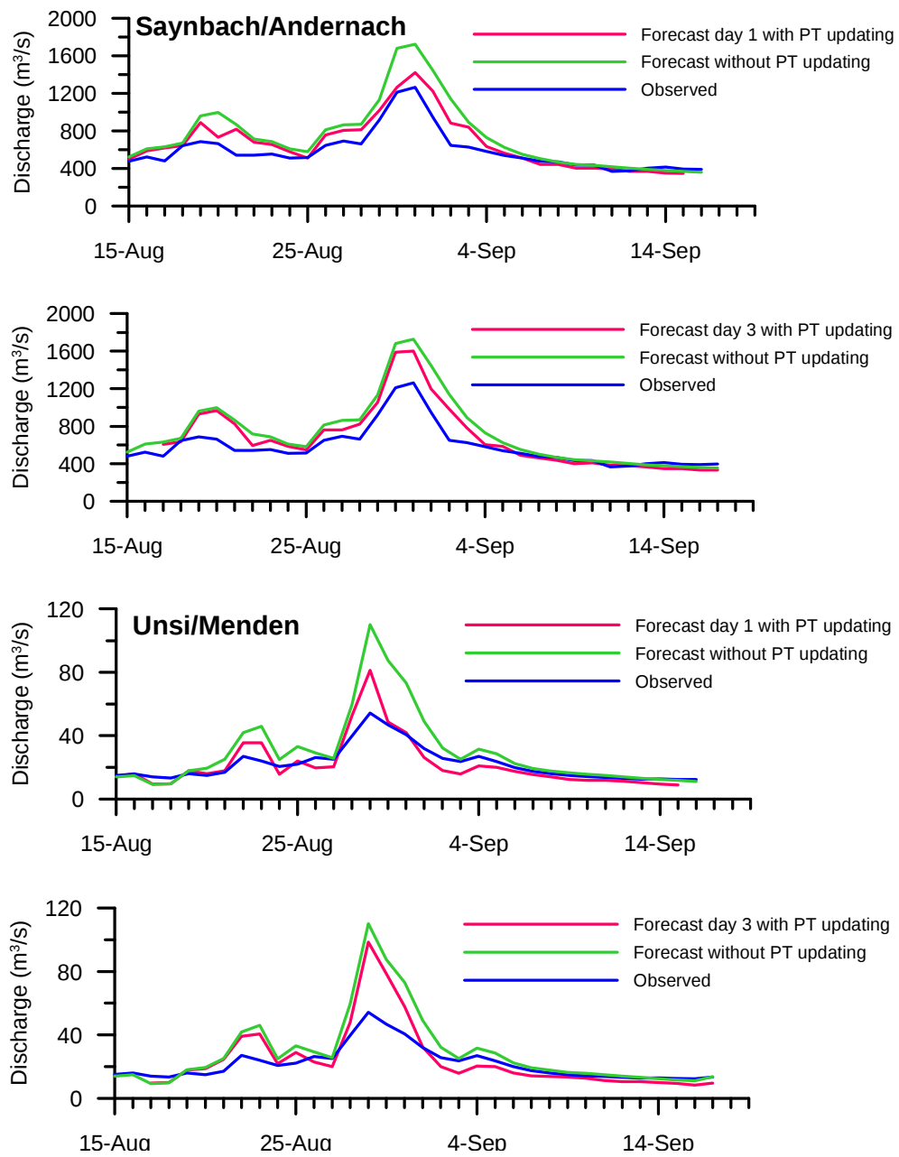
Figure 30. Forecast evaluation graphs for low flow period 2006. Forecasts were made once a day five days ahead. The red and green lines show the forecasted discharge for the first and third day of each forecast (31). No data were available for Main in this period
