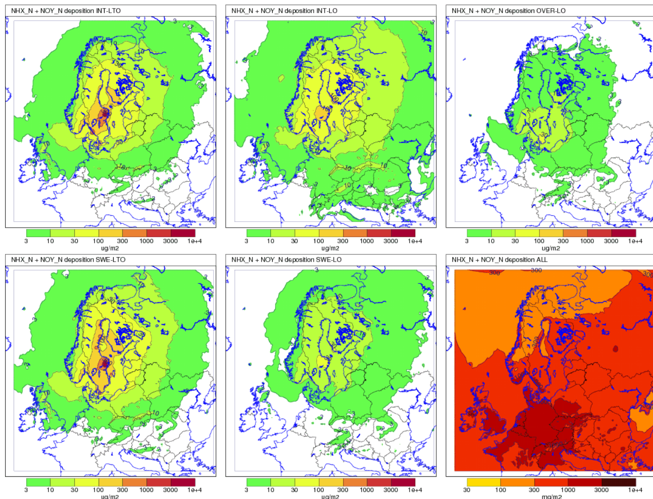
Figure 5: Yearly mean deposition of oxidised and reduced nitrogen for year 2012-2014.
