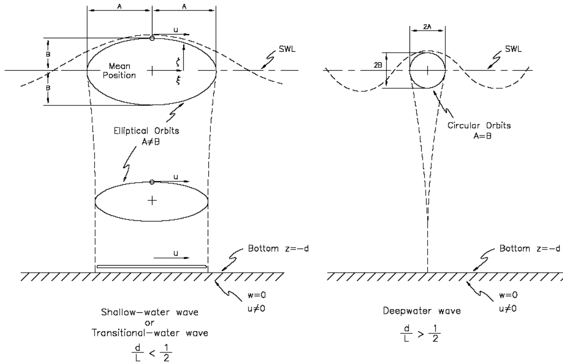
Figure 14 Water movements under waves in intermediate/shallow (left) and deep (water) respectively (from Coastal Engineering Manual, Part II, Chapter 1)
