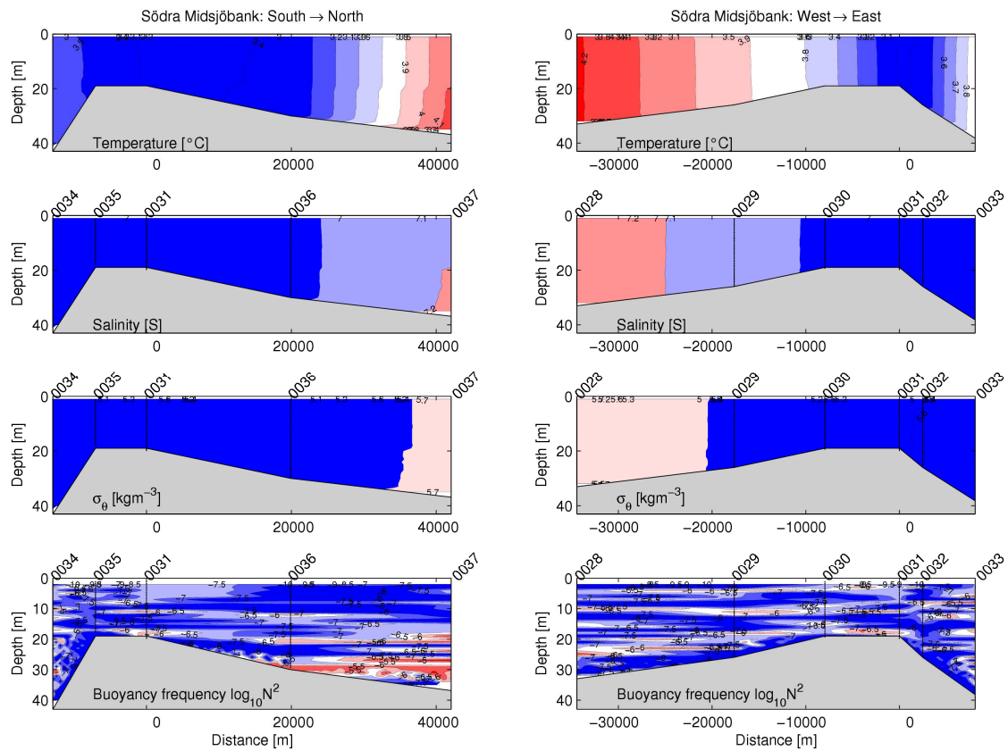
Figure 62 Gridded hydrographic parameters over Södra Midsjöbank
