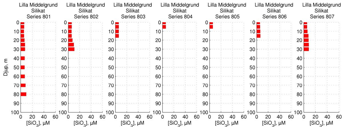
Figure 28 Silicate concentrations across Lilla Middelgrund
