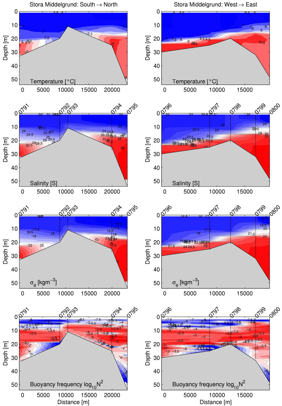
Figure 38 Gridded hydrographic parameters across Stora Middelgrund
