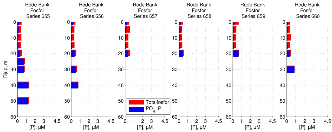
Figure 34 Phosphorus concentrations across Röde Bank
