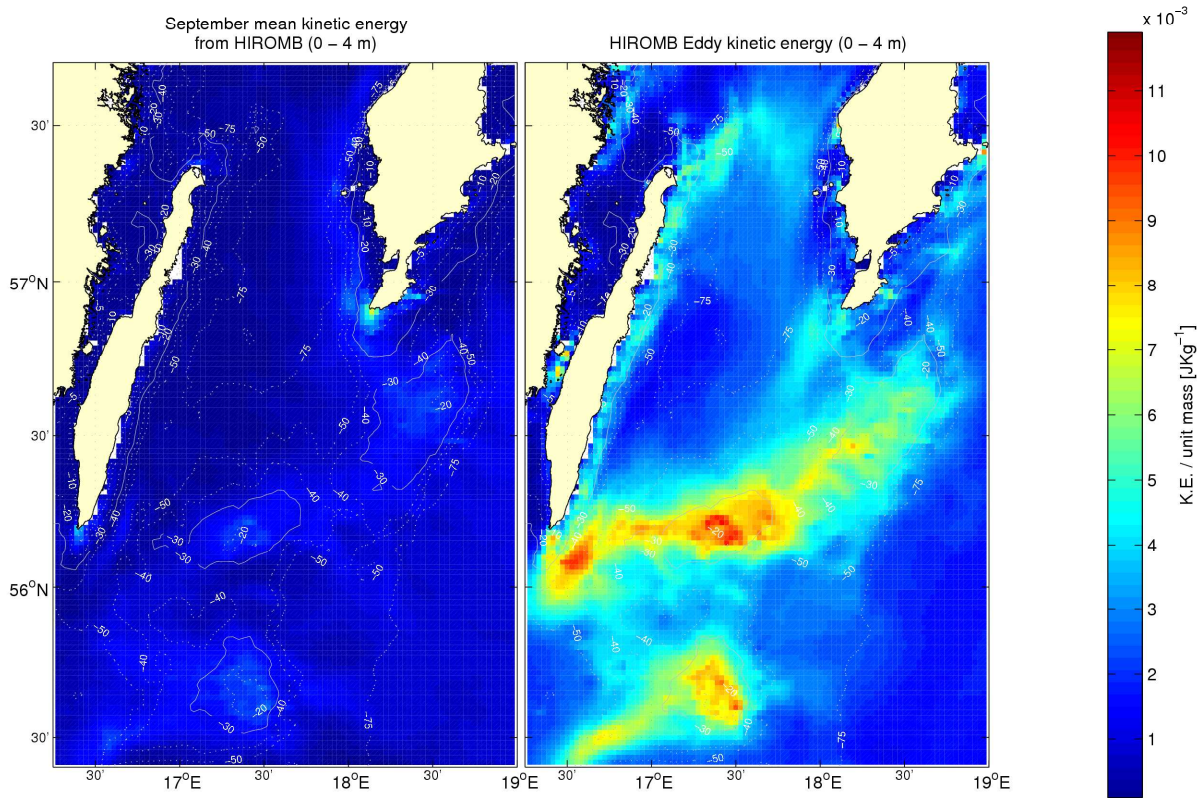
Figure 12 Mean (left) and eddy (right) kinetic energy (per unit mass) from HIROMB surface data, September 2004. The bathymetry is indicated by the grey contours.
