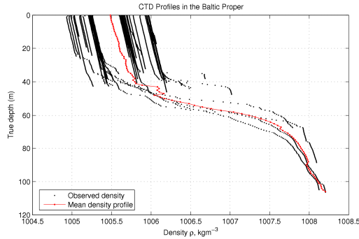
Figure 6 Observed & mean density profiles around the Baltic Banks
