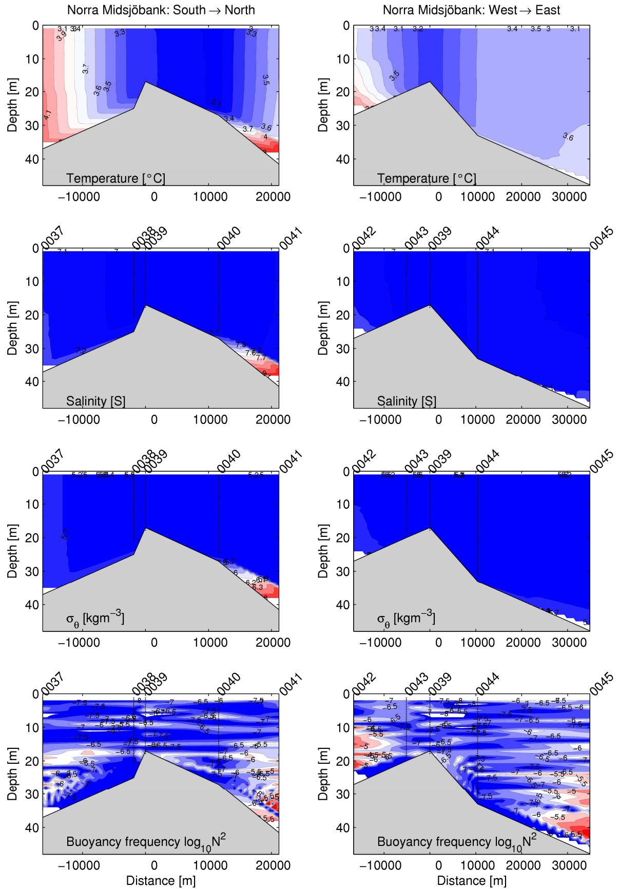
Figure 70 Gridded hydrographic parameters across Norra Midsjöbank
