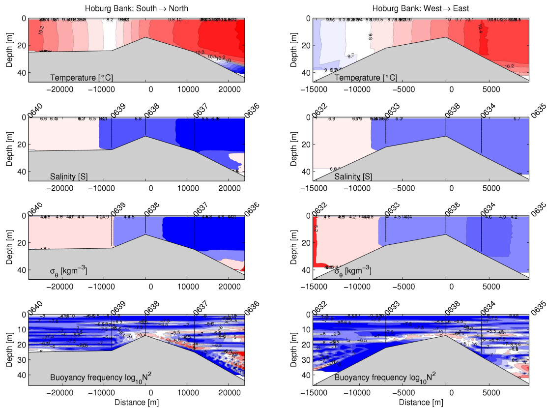
Figure 78 Gridded hydrographic parameters across the Hoburg Bank
