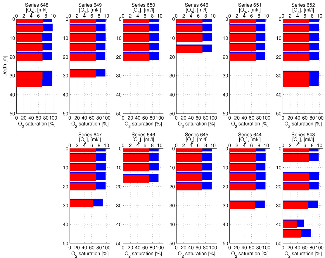
Figure 52 Oxygen concentrations and saturation in the vicinity of Kriegers Flak
