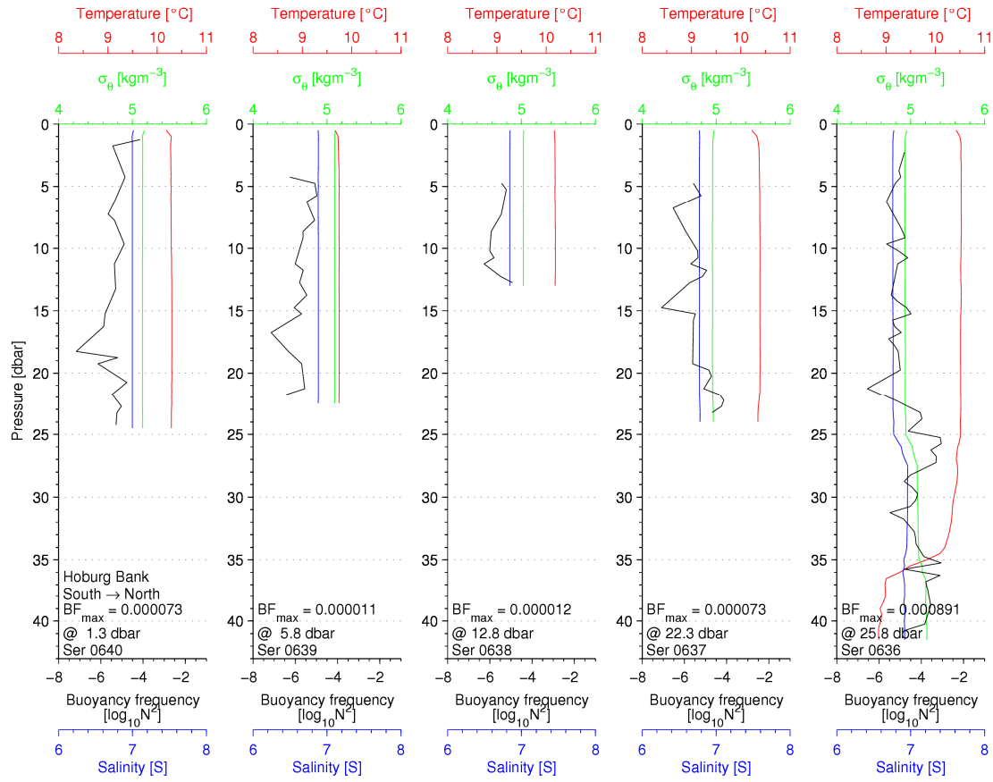
Figure 79 CTD profiles from south to north across Hoburg Bank
