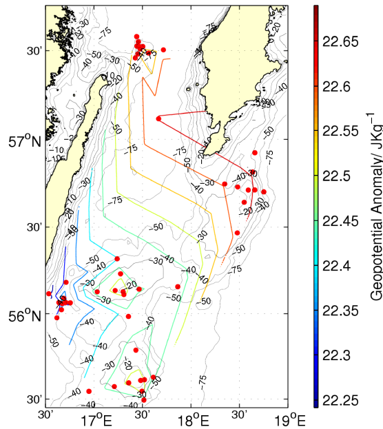
Figure 7 Estimate of the geopotential anomaly in the southern West Gotland Basin
