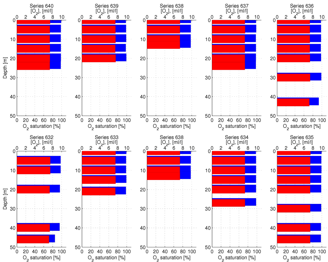
Figure 84 Oxygen concentrations (red) and saturation (blue) over the Hoburg Bank
