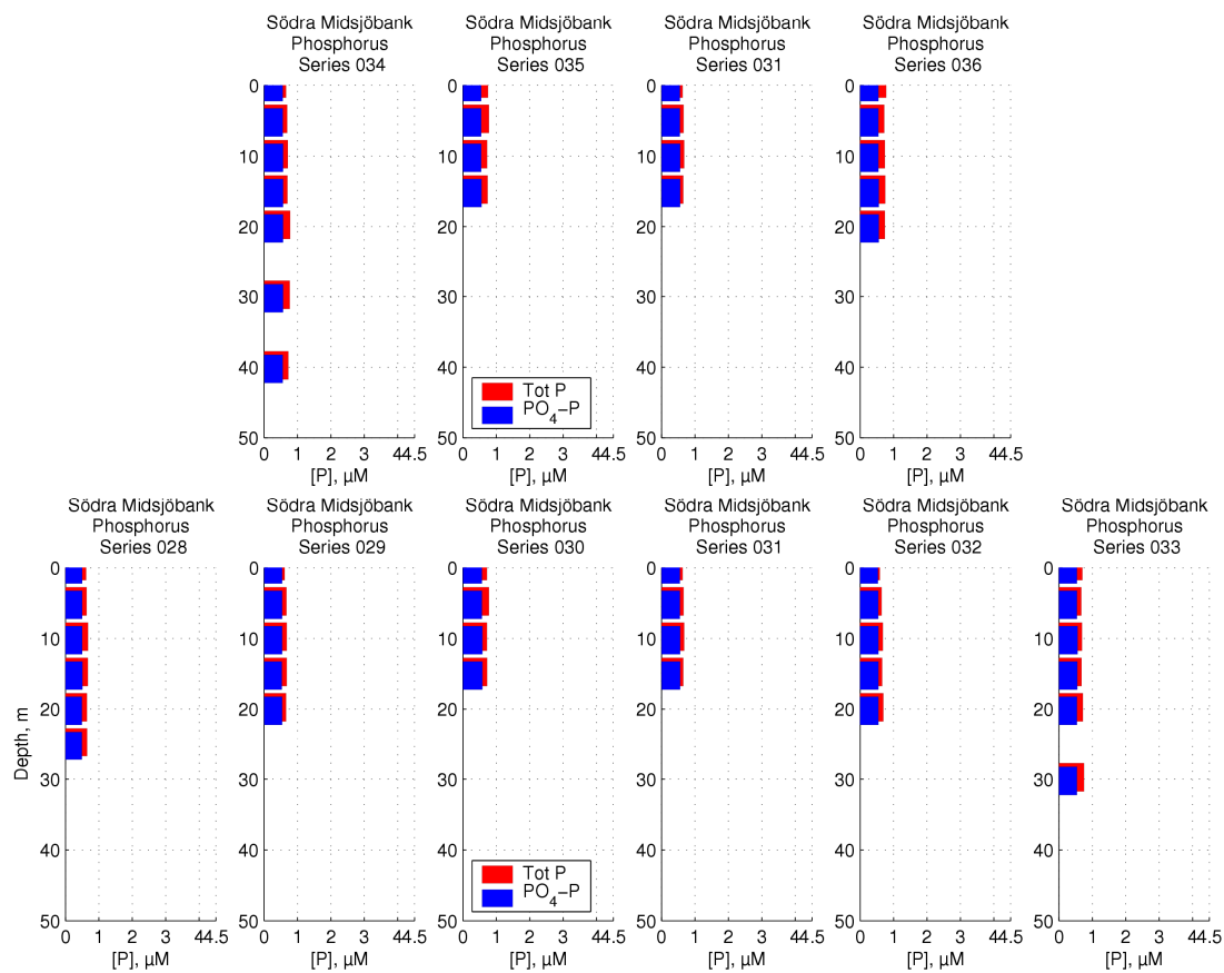
Figure 66 Phosphorus concentrations over Södra Midsjöbanken
