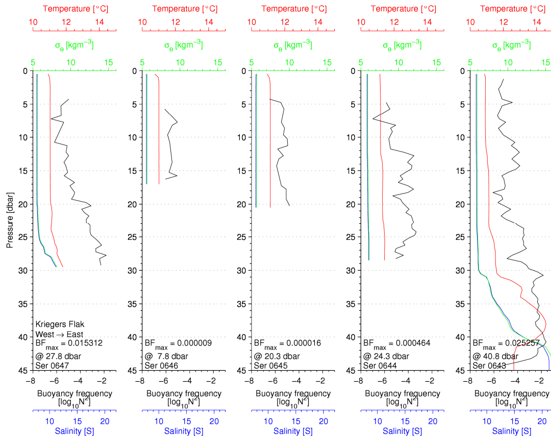
Figure 48 CTD profiles along the west – east transect over Kriegers Flak
