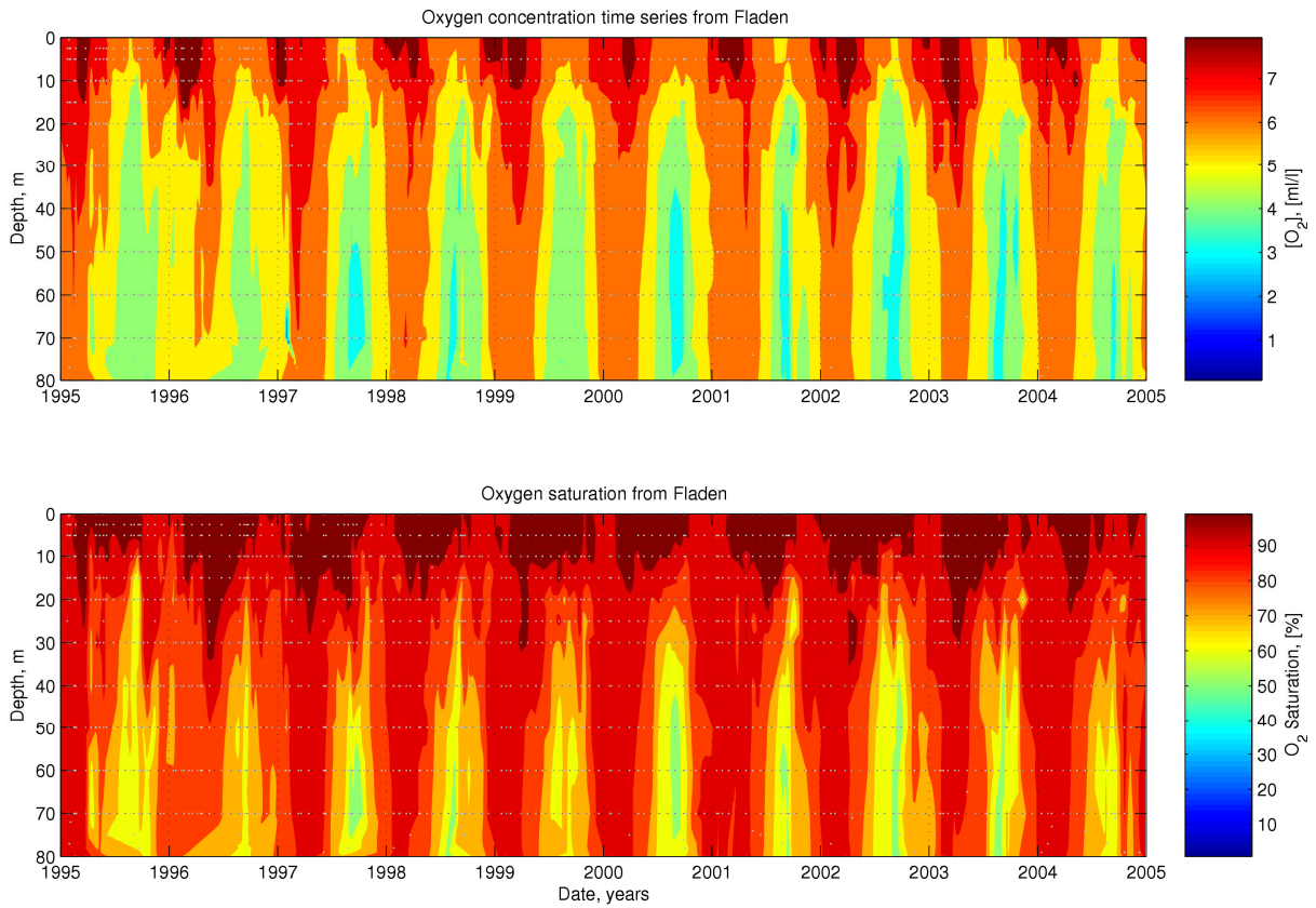
Figure 10 Time series of oxygen concentration and saturation from Fladen
