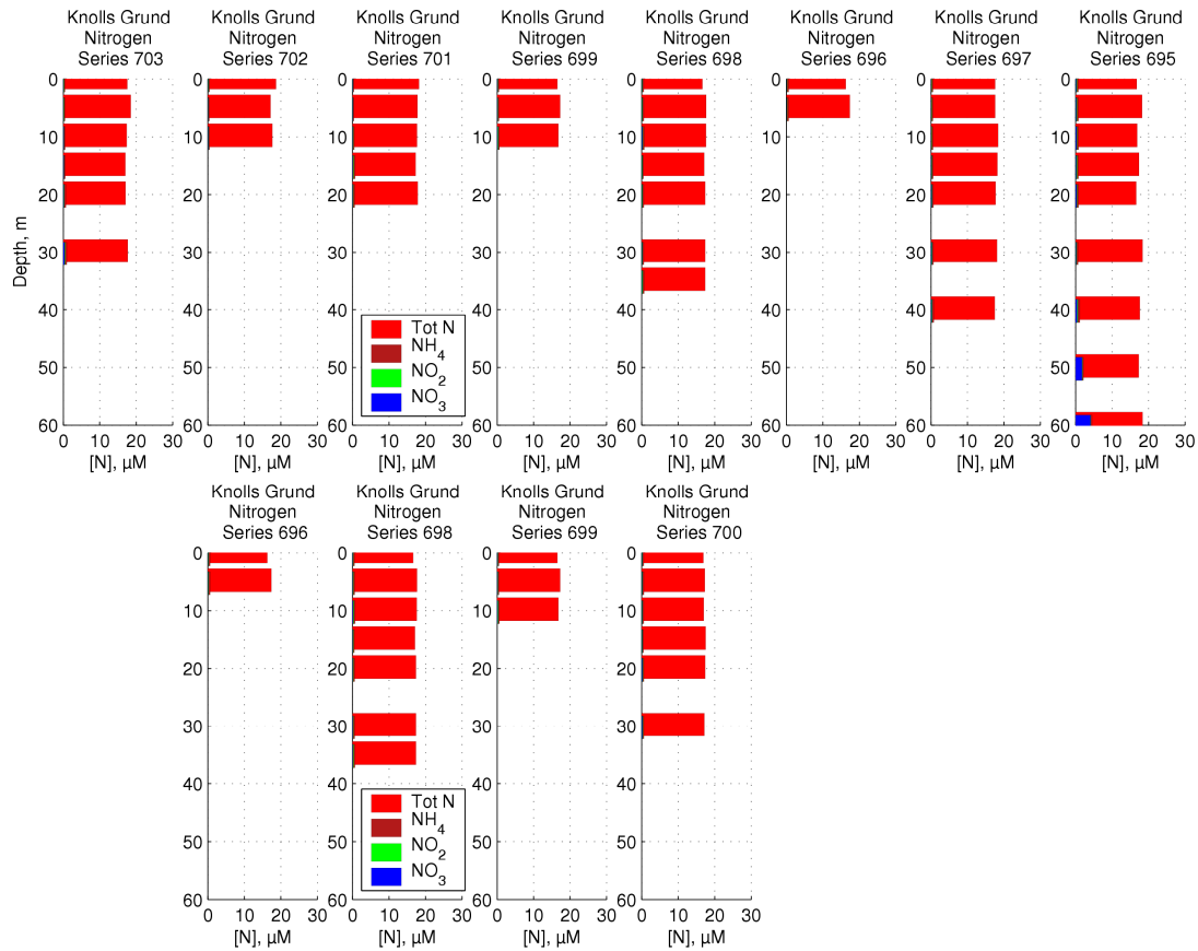
Figure 89 Nitrogen concentrations over Knolls Grund
