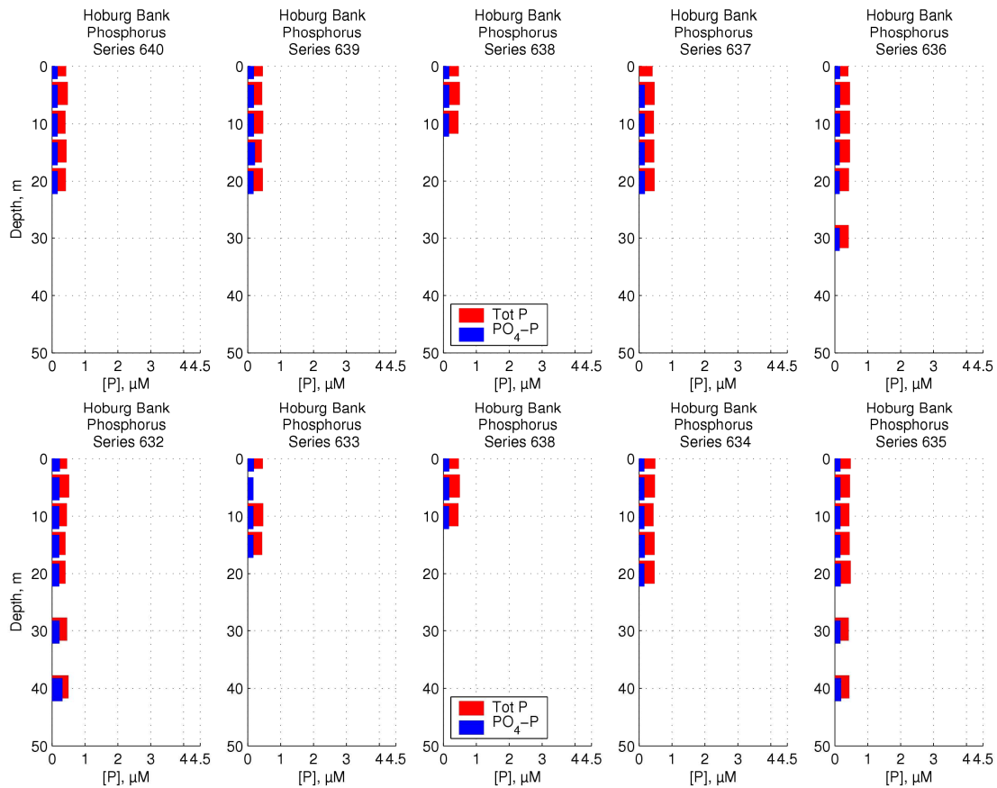
Figure 82 Phosphorus concentrations over the Hoburg Bank
