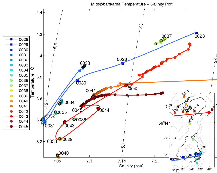
Figure 5 Temperature Salinity diagram over both the Midsjö banks.
