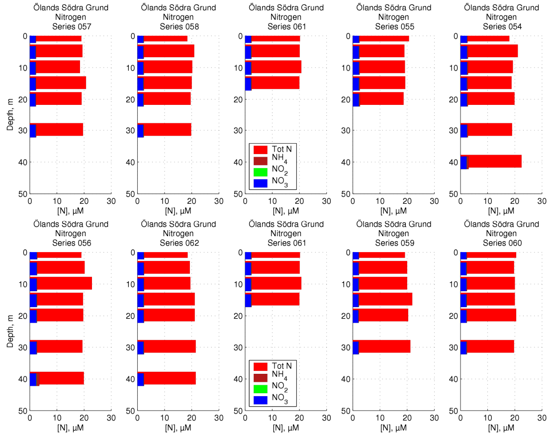
Figure 57 Nitrogen concentrations around Ölands Södra Grund
