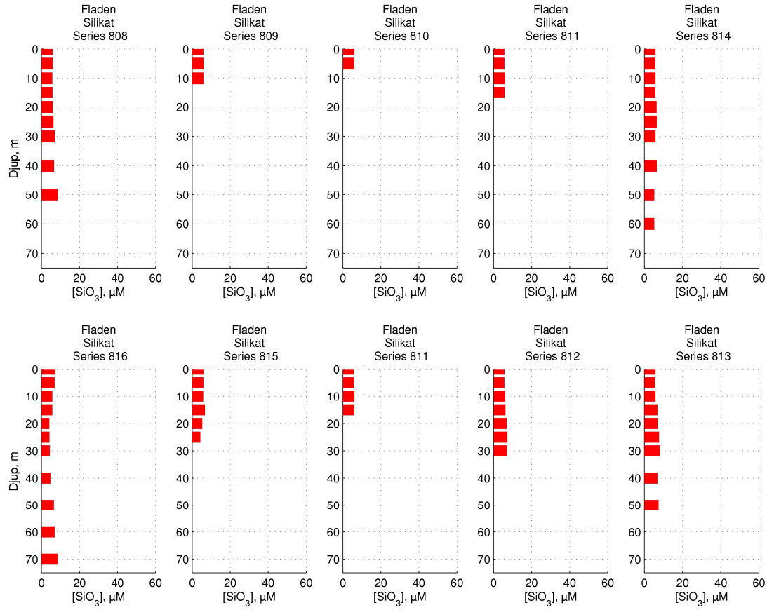
Figure 21 Silicate concentrations across Fladen
