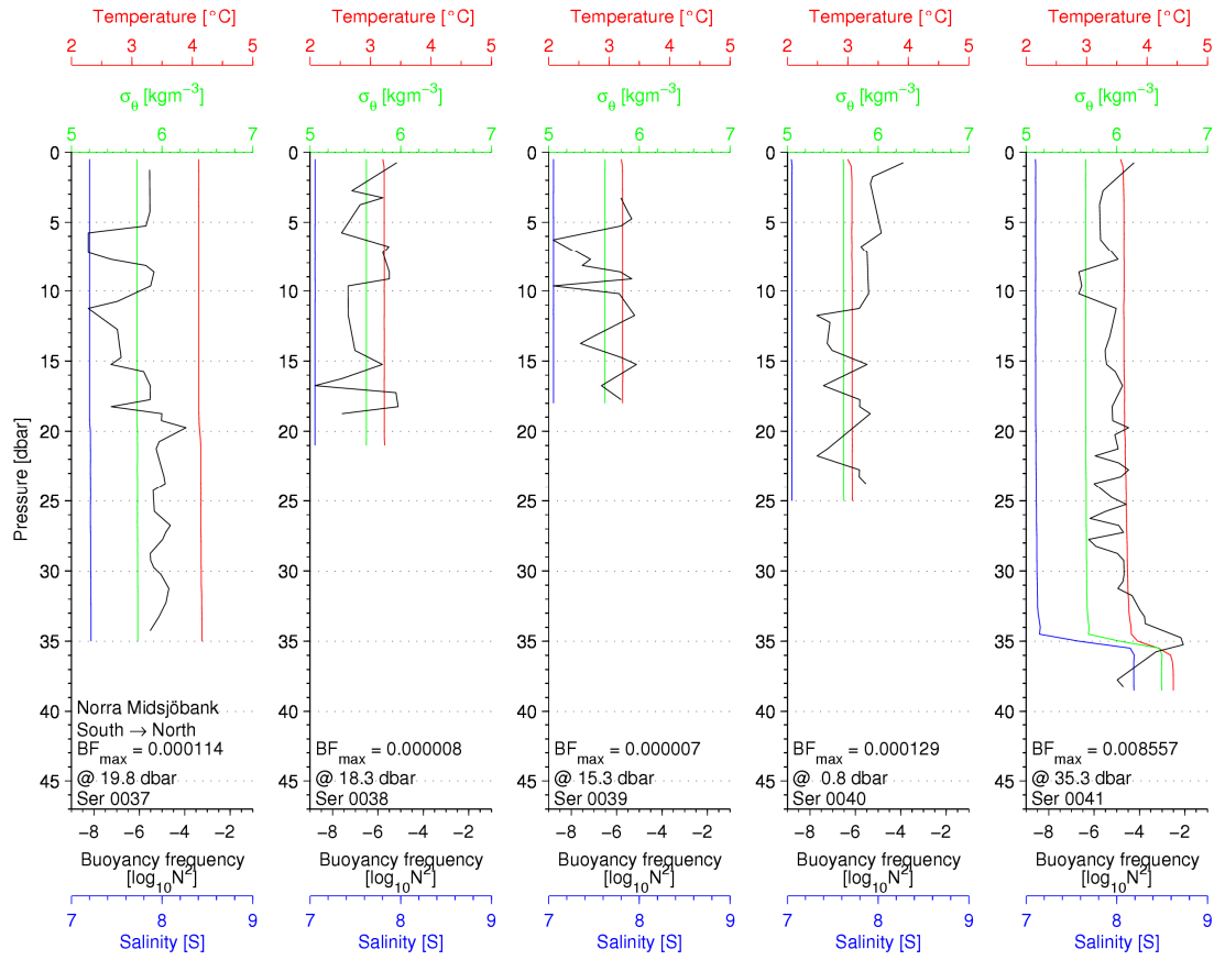
Figure 71 CTD profiles from south to north across Norra Midsjöbank
