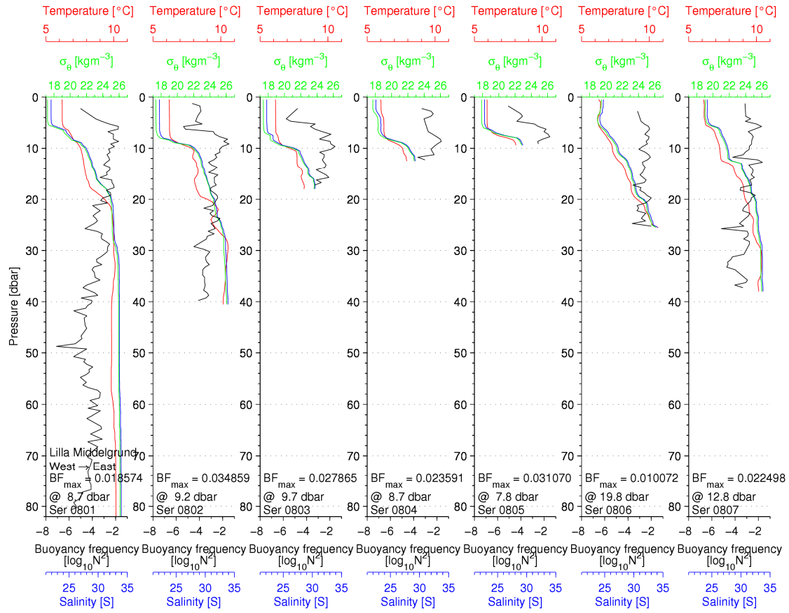
Figure 25 Temperature, salinity and buoyancy frequency profiles across Lilla Middelgrund.
