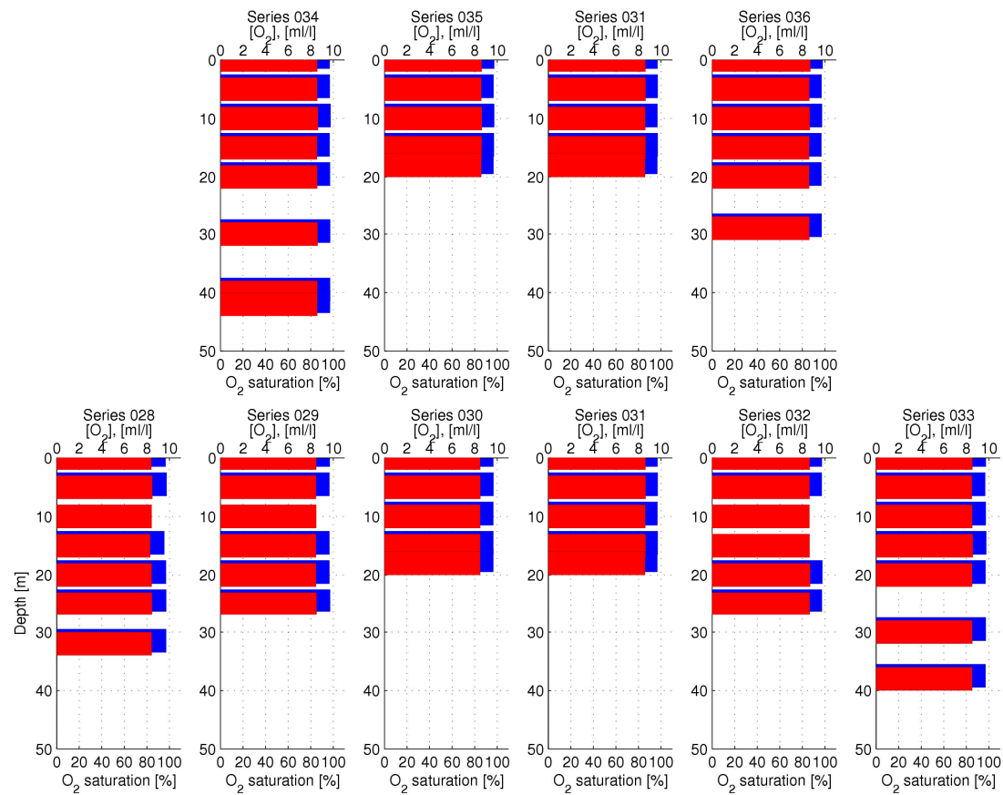
Figure 68 Oxygen concentrations (red) and saturation (blue) across Södra Midsjöbanken
