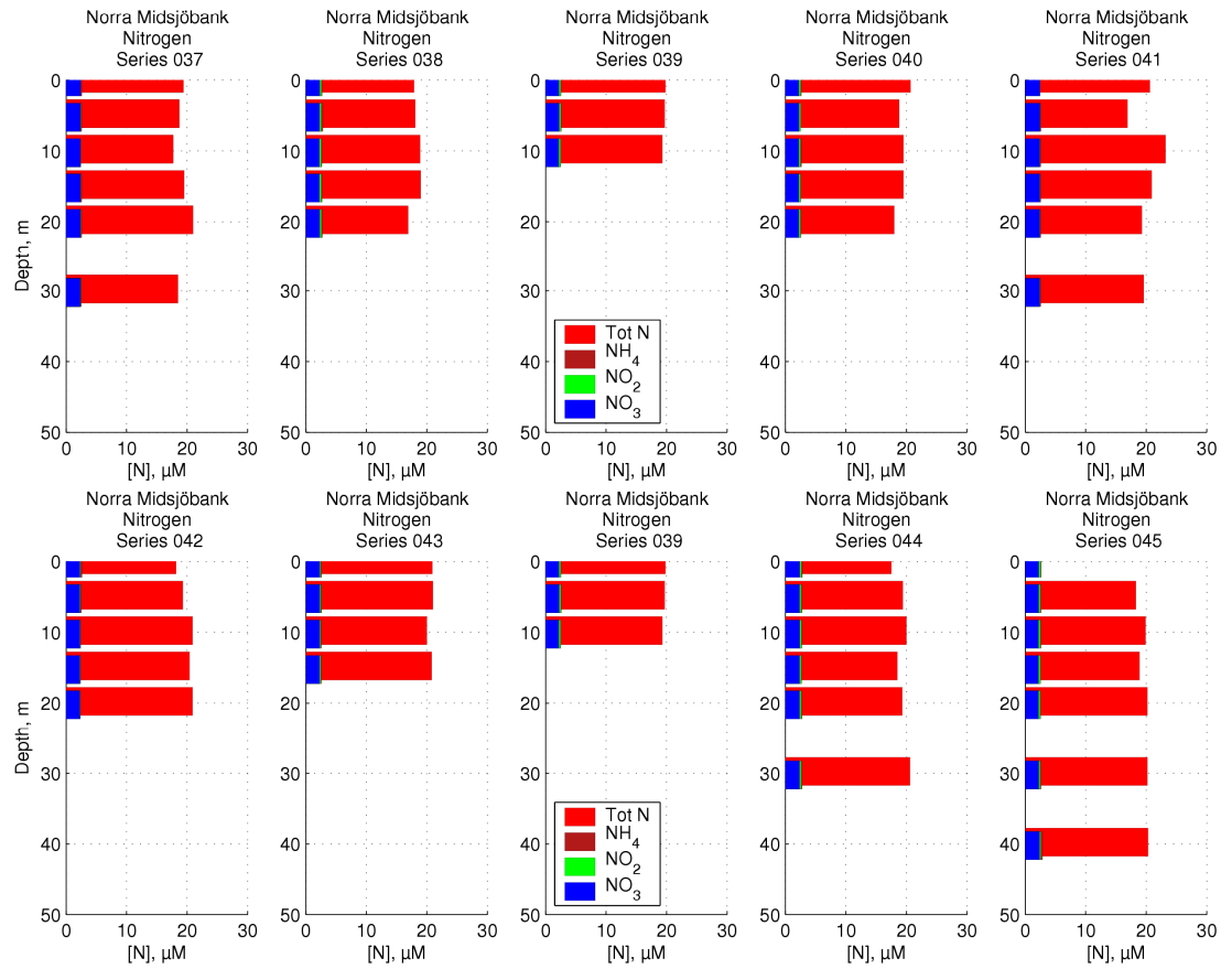
Figure 73 Nitrogen concentrations over Norra Midsjöbank
