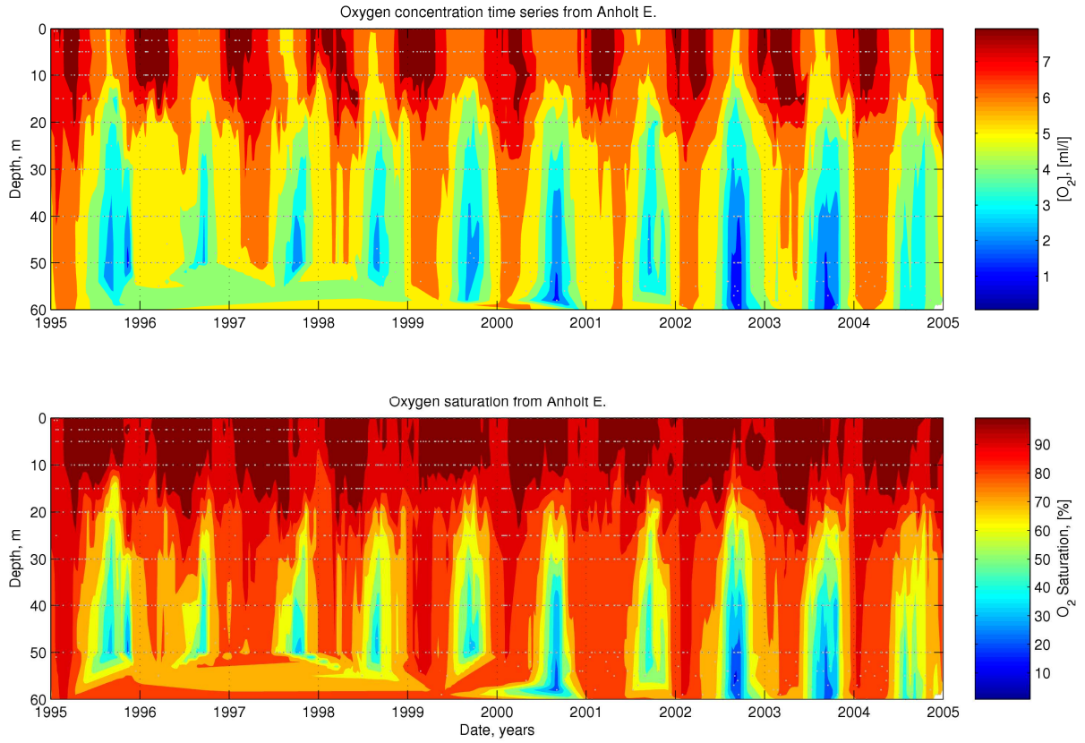
Figure 9 Time series of oxygen concentration and saturation from Anholt E.
