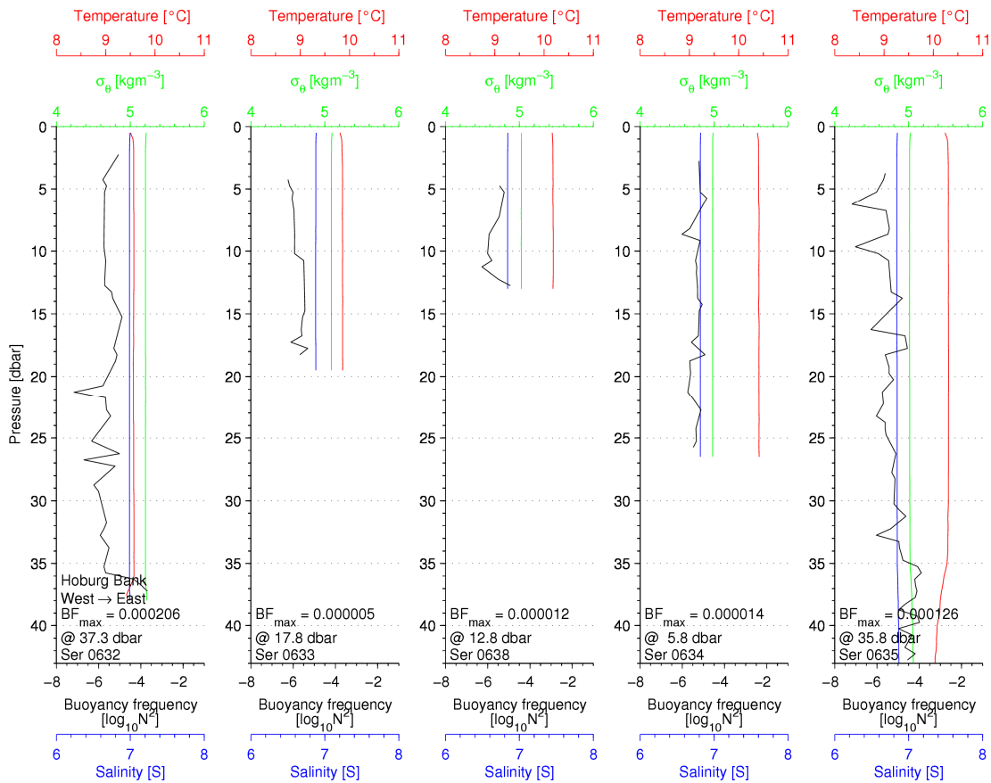
Figure 80 CTD profiles from west to east across Hoburg Bank
