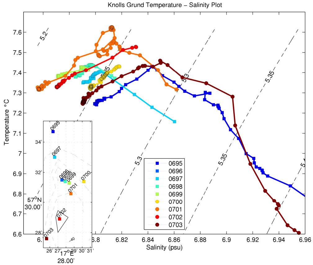
Figure 85 Temperature – salinity plot for Knolls Grund
