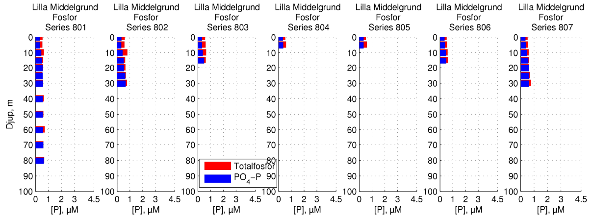
Figure 27 Phosphorus concentrations across Lilla Middelgrund
