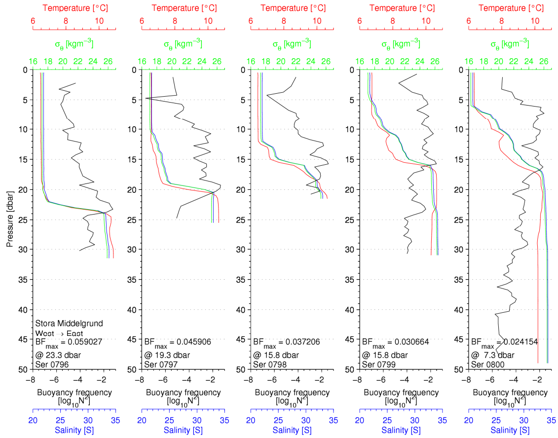
Figure 40 CTD profiles across Stora Middelgrund from west to east
