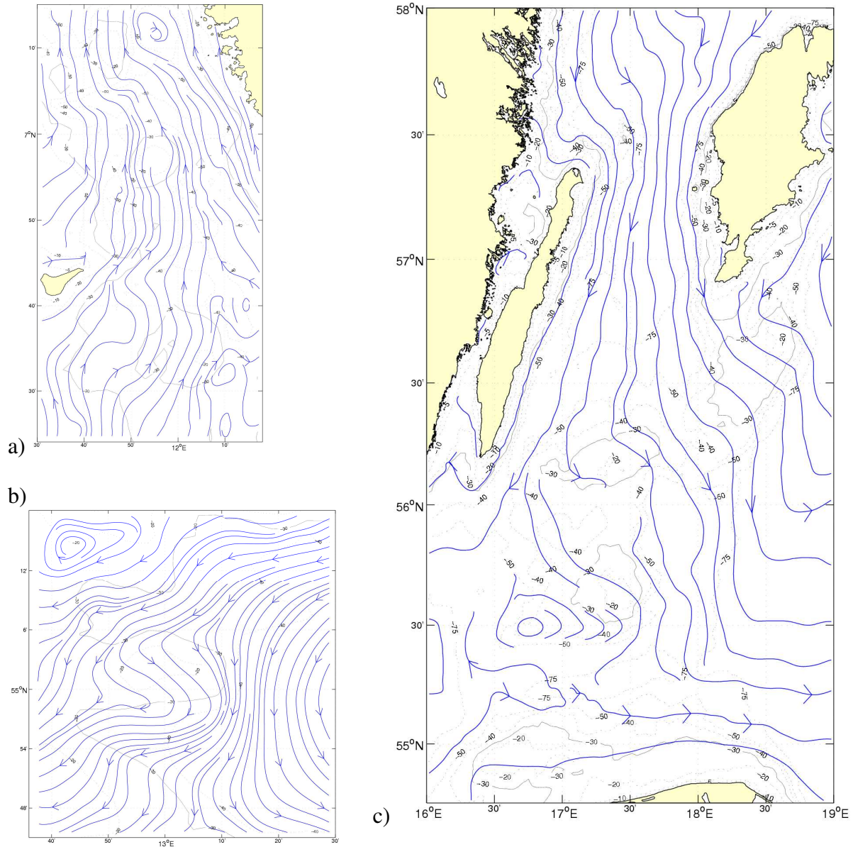
Figure 11 Annual mean, depth integrated (0 – 40 metres) stream function from HIROMB, showing the large scale circulation for the Kattegat (a), Kriegers Flak (b) and Baltic Proper banks (c). Depth contours are shown in grey.
