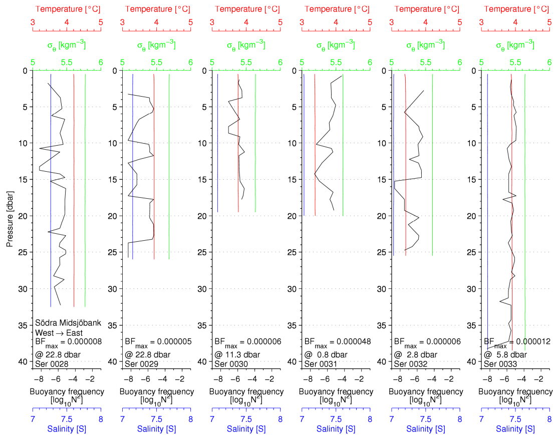
Figure 64 CTD profiles from west - east transect over Södra Midsjöbank
