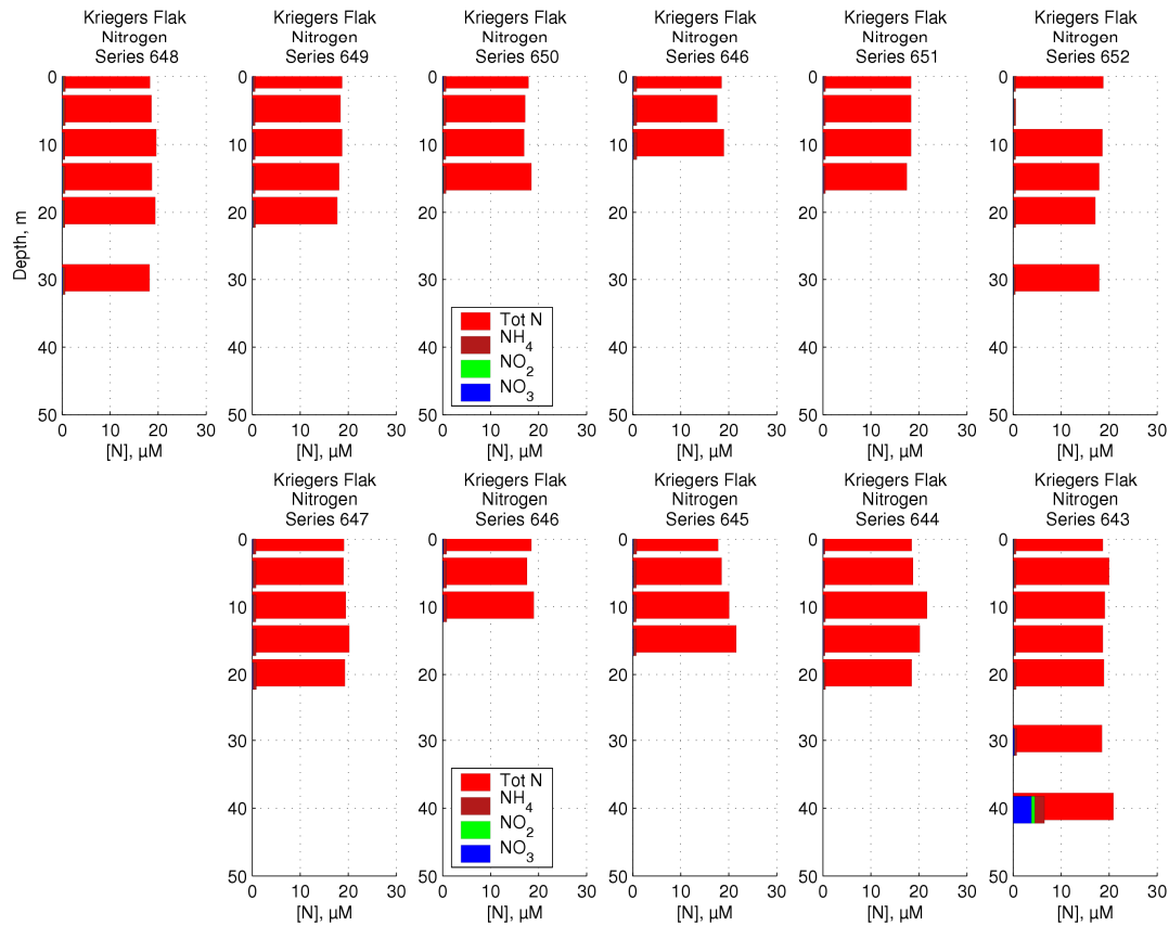
Figure 49 Nitrogen concentrations around Kriegers Flak
