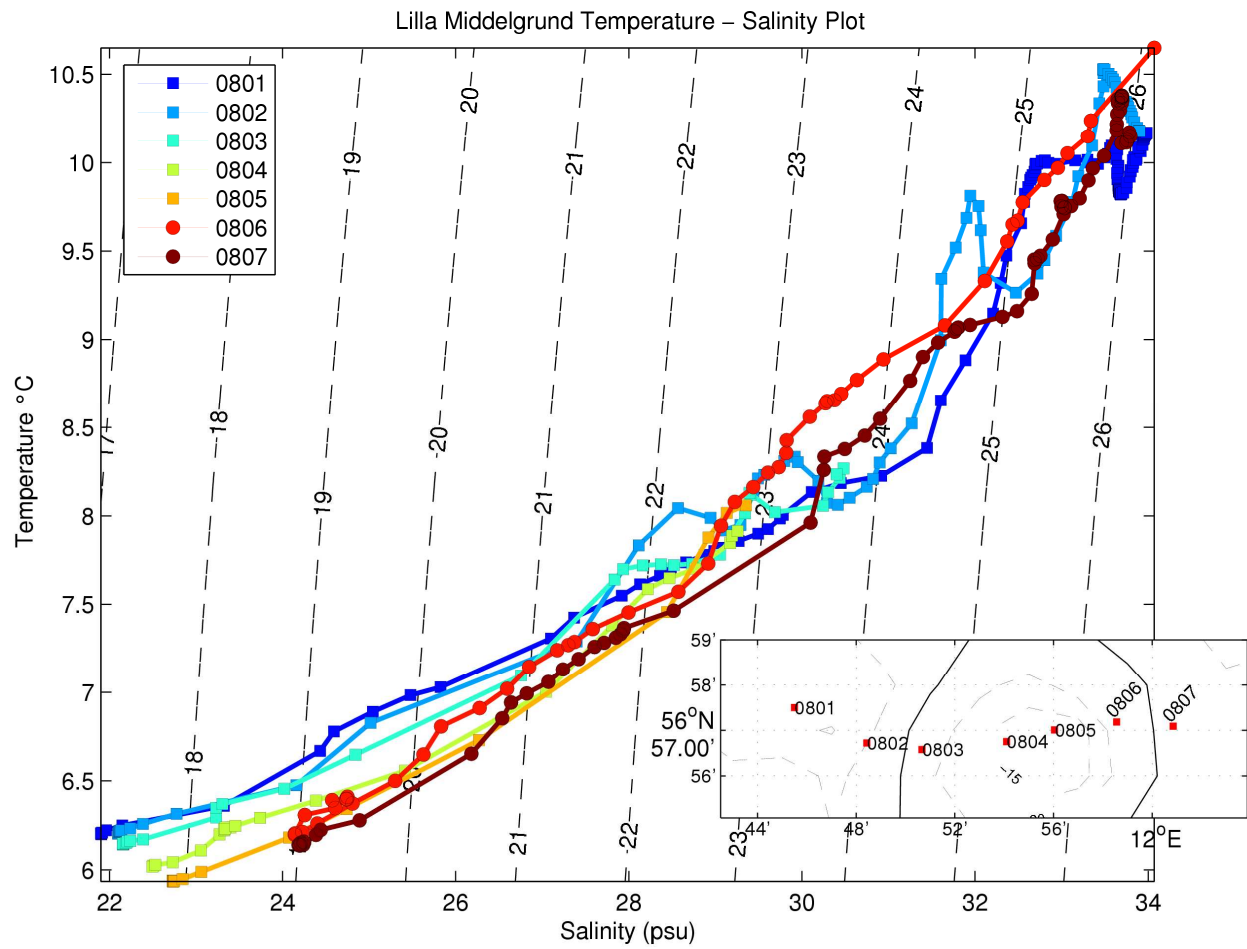
Figure 23 Temperature - salinity plot over Lilla Middelgrund
