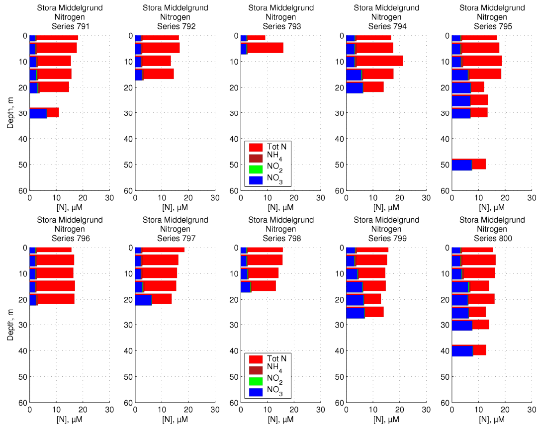
Figure 41 Stora Middelgrund nitrogen concentrations
