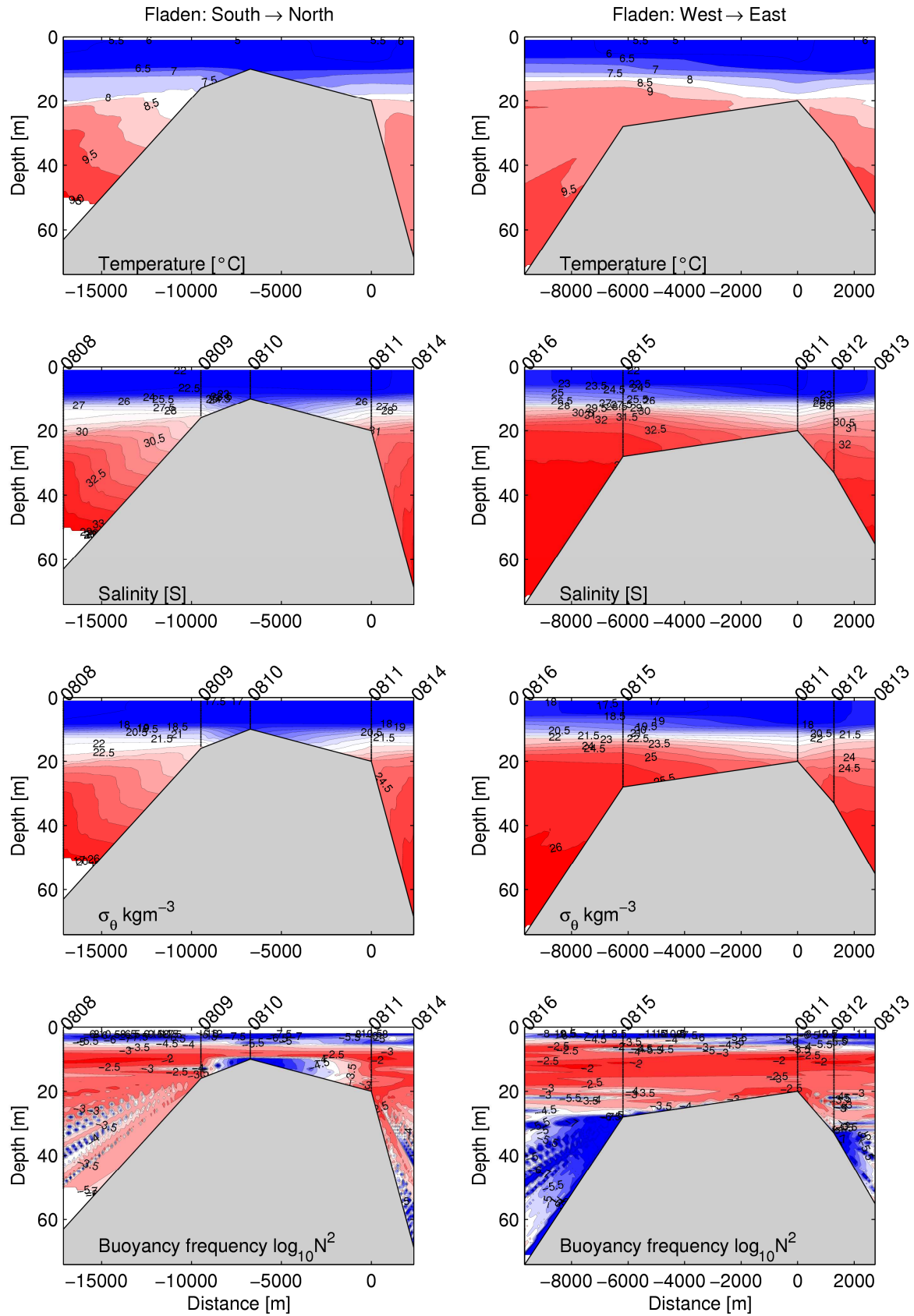
Figure 16 Gridded hydrographic properties over Fladen
