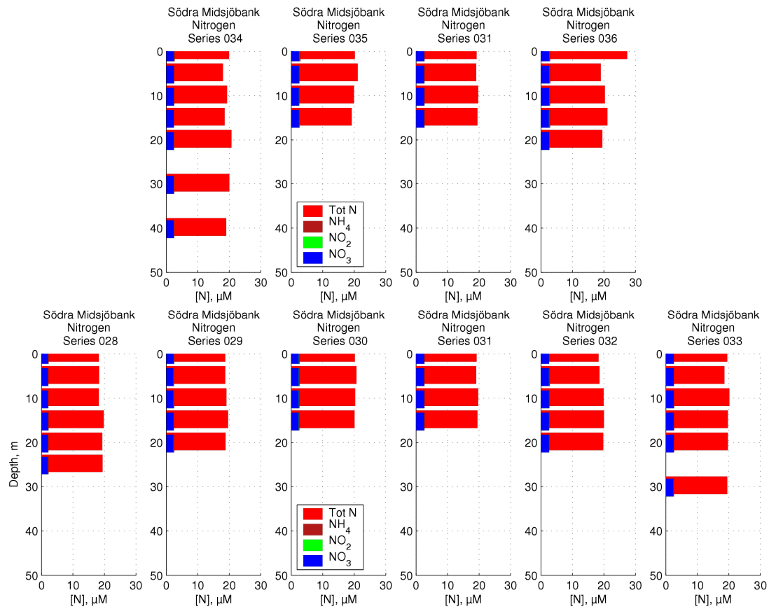
Figure 65 Nitrogen concentrations over Södra Midsjöbanken
