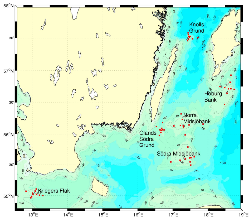
Figure 2 Sampling stations over banks in the Baltic Proper: October 2003 – December 2004
