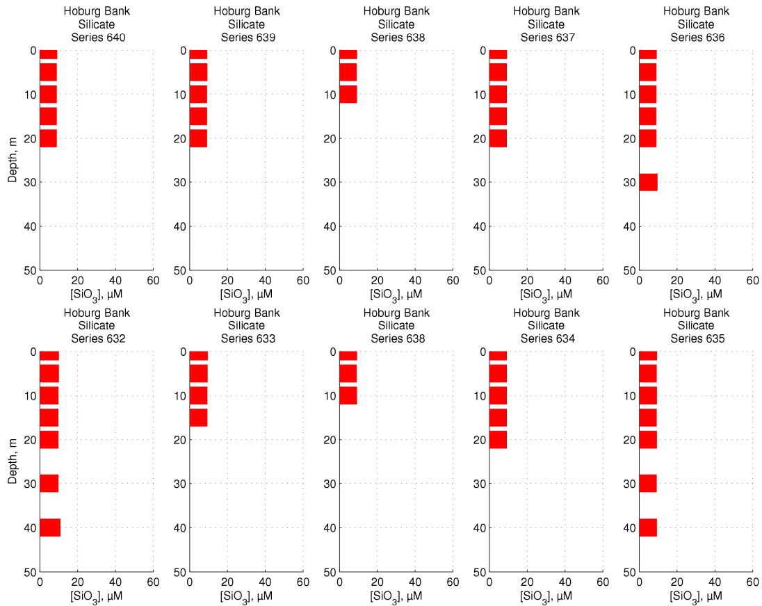
Figure 83 Silicate concentrations over the Hoburg Bank
