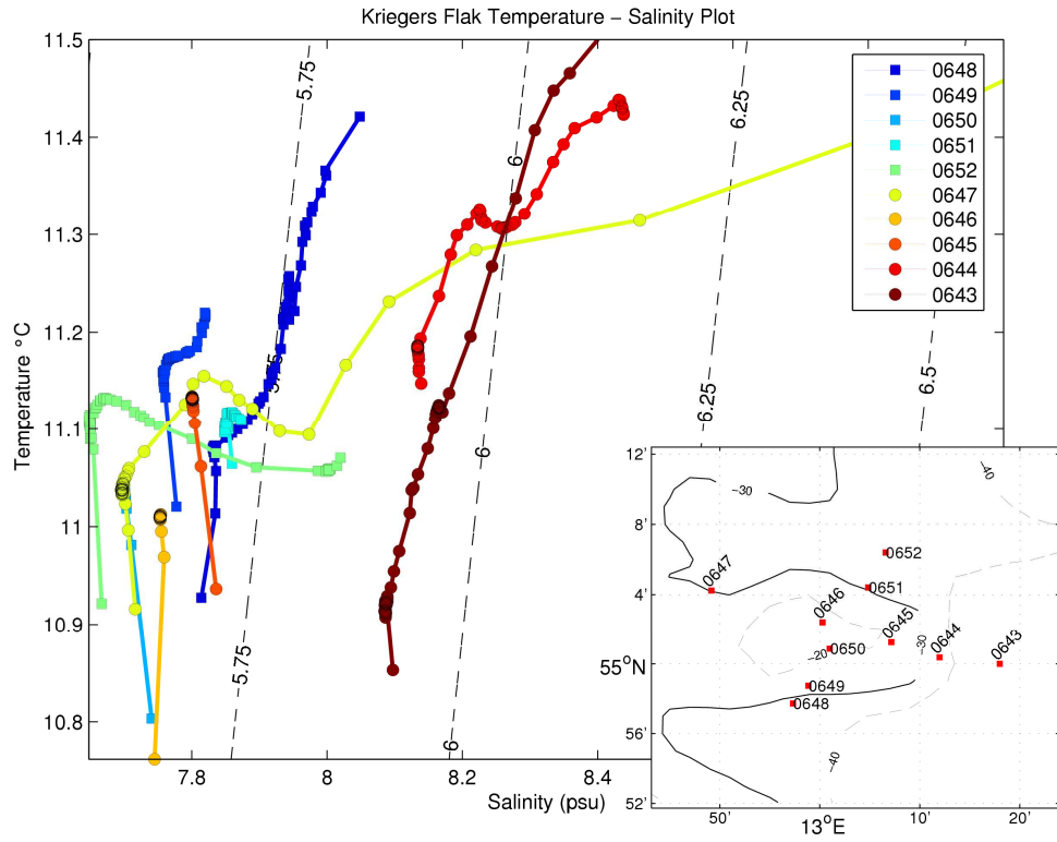
Figure 45 Kriegers Flak (enlarged) temperature and salinity plot
