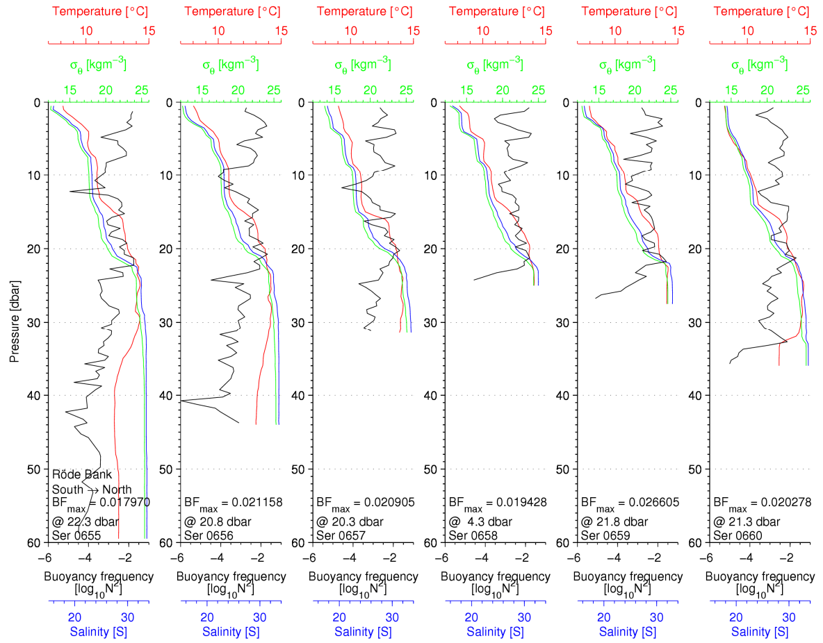
Figure 32 CTD profiles measured over Röde Bank
