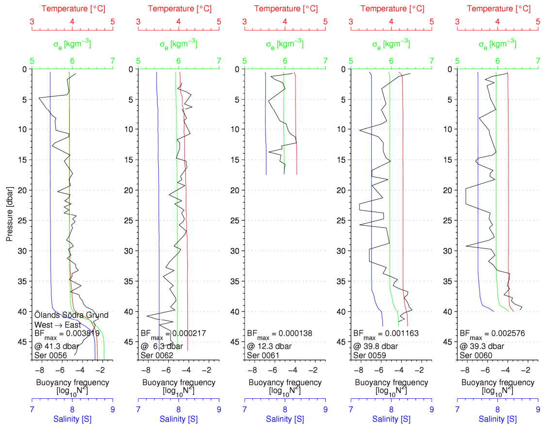
Figure 56 CTD profiles from west – east across Ölands Södra Grund
