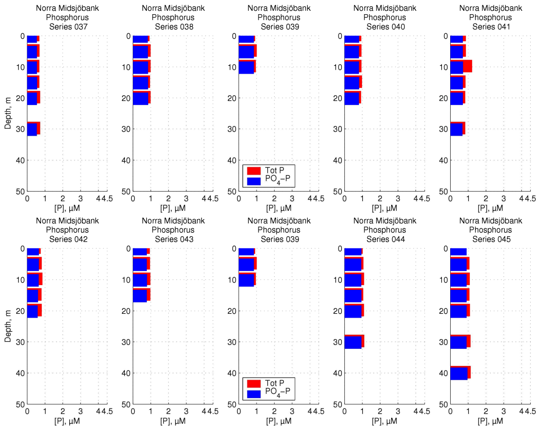
Figure 74 Phosphorus concentrations over Norra Midsjöbank
