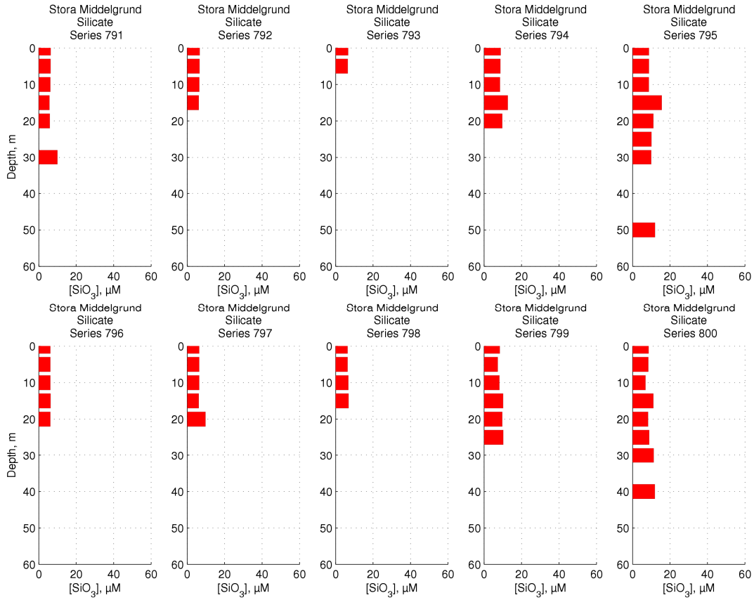
Figure 43 Stora Middelgrund silicate concentrations
