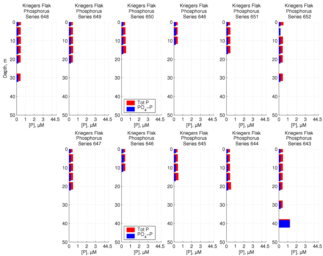
Figure 50 Phosphorus concentrations around Kriegers Flak
