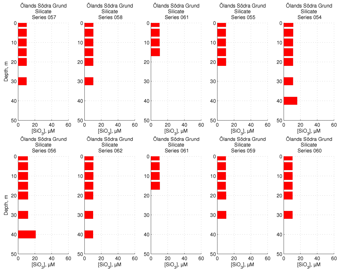
Figure 59 Silicate concentrations around Ölands Södra Grund
