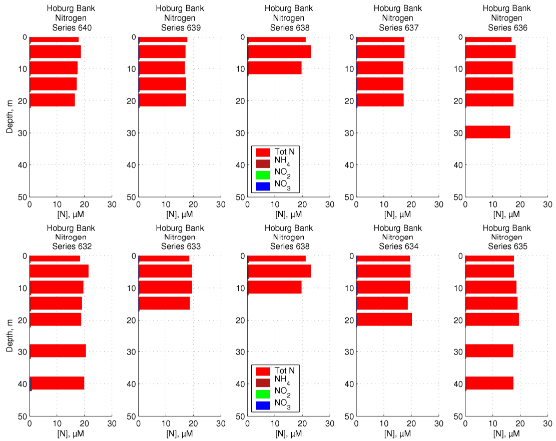
Figure 81 Nitrogen concentrations over the Hoburg Bank
