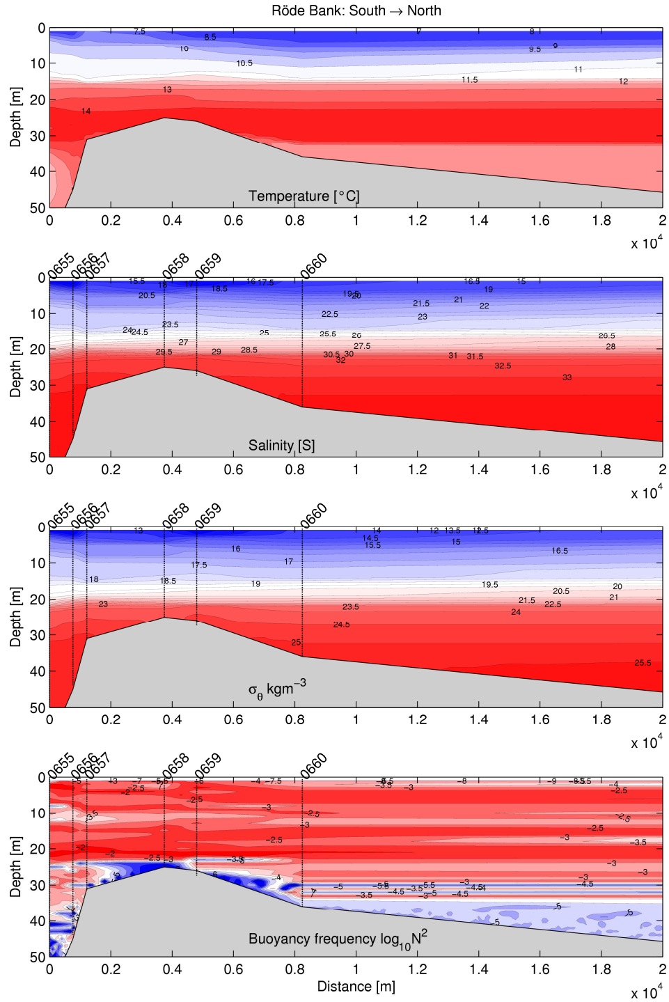
Figure 31 Hydrography over Röde Bank, gridded from south to north.
