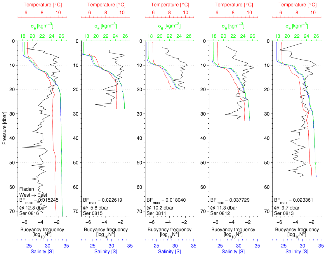
Figure 18 CTD profiles from the west – east transect across Fladen
