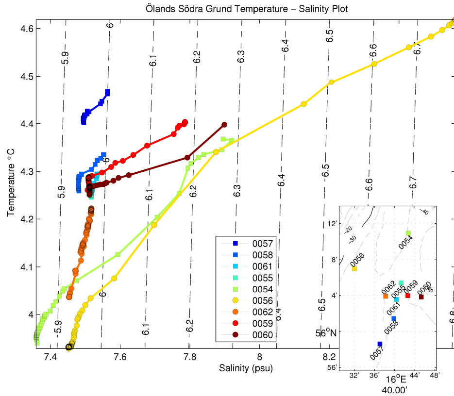
Figure 53 Ölands Södra Grund temperature – salinity relationship
