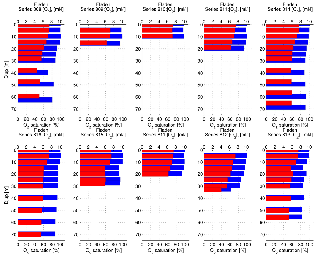
Figure 22 Oxygen concentrations (red) and saturation (blue) across Fladen
