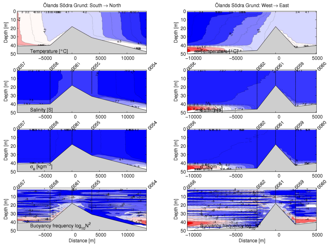
Figure 54 Gridded hydrographic parameters across Ölands Södra Grund.
