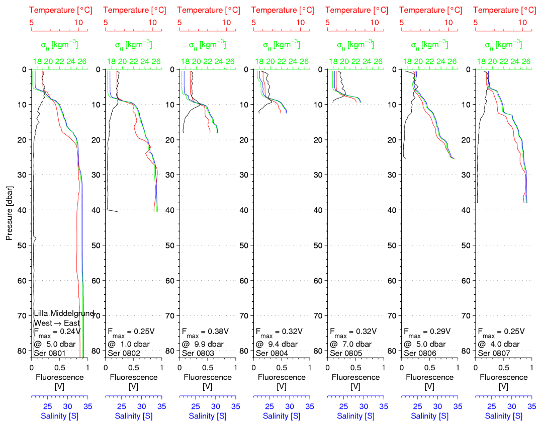
Figure 3 Temperature, salinity and fluorimeter profiles across Lilla Middelgrund.
