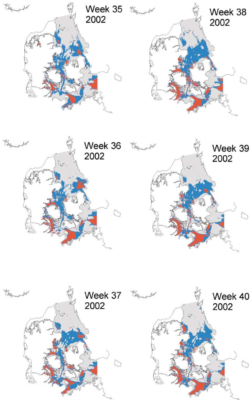
Figure 8 Maximum extent of the 2002 Oxygen Depletion (from Ærtjeberg et al, 2003)
