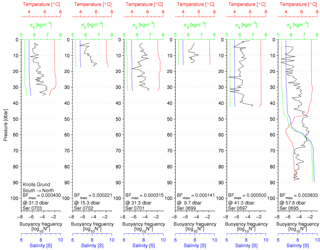
Figure 87 CTD profiles along the south – north transect along Knolls Grund
