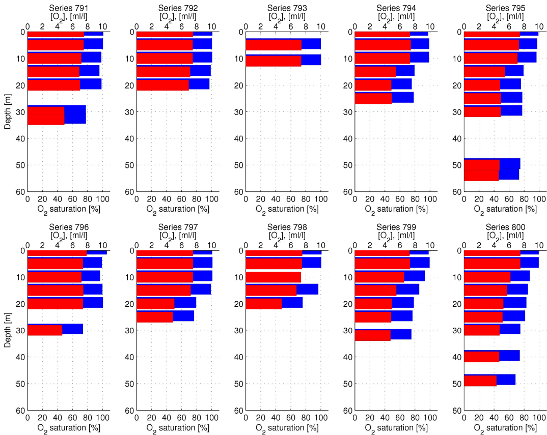
Figure 44 Stora Middelgrund oxygen concentration (red) and saturation (blue)
