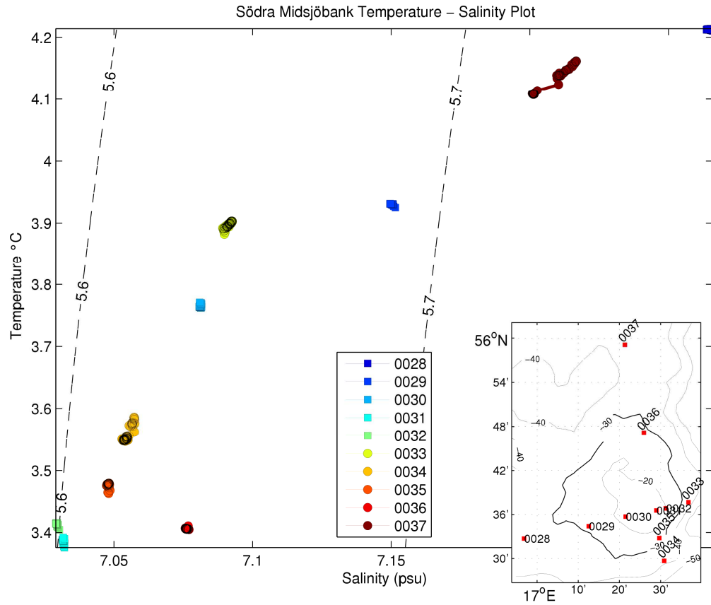
Figure 61 Temperature – salinity plot across Södra Midsjöbank
