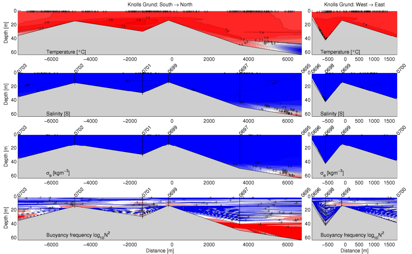
Figure 86 Hydrographic parameters gridded across Knolls Grund
