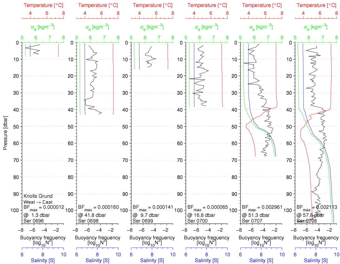
Figure 88 CTD profiles from west – east across Knolls Grund (For comparison, profiles 0707 and 0708 show conditions further out in the West Gotland Basin)
