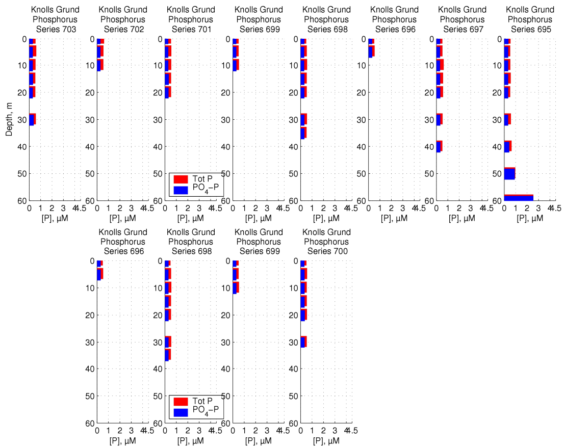
Figure 90 Phosphorus concentrations over Knolls Grund
