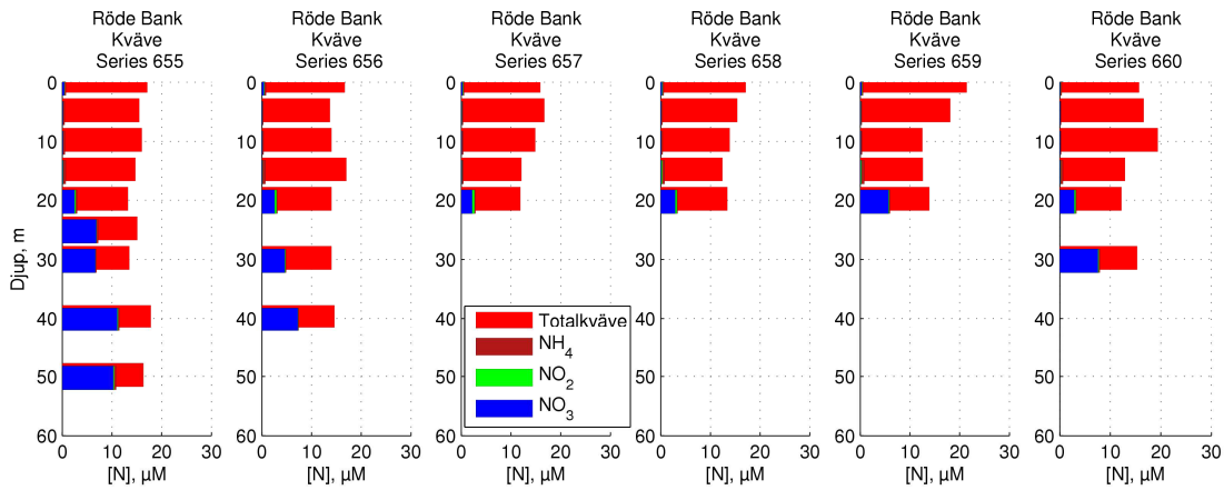
Figure 33 Nitrogen concentrations across Röde Bank
