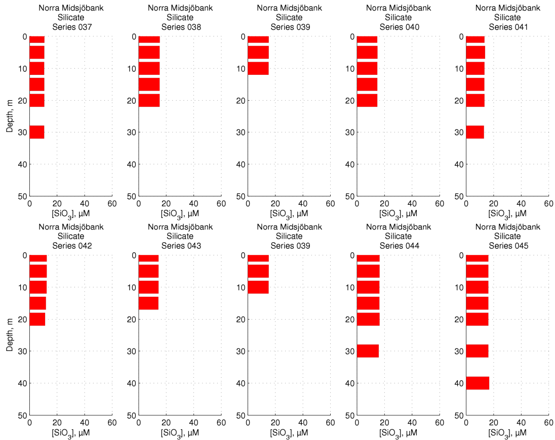
Figure 75 Silicate concentrations across Norra Midsjöbank
