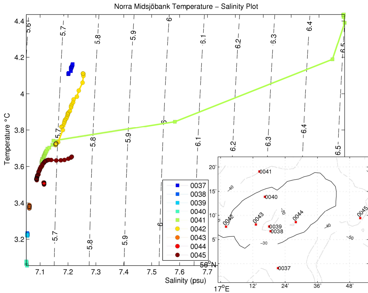
Figure 69 Temperature – salinity diagram for Norra Midsjöbank
