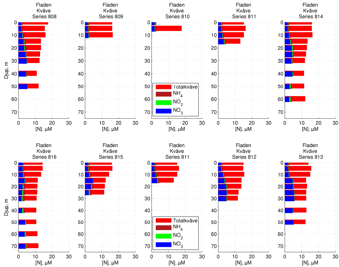
Figure 19 Nitrogen concentrations across Fladen
