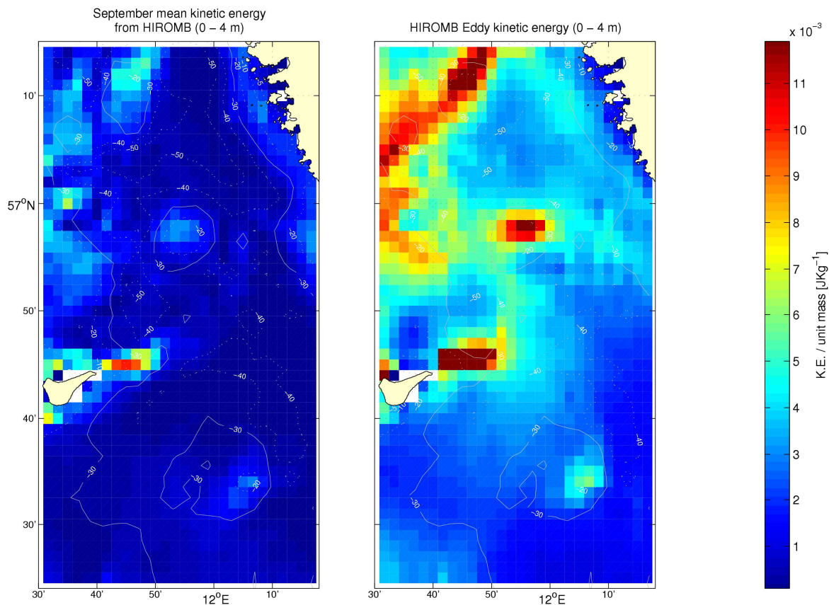
Figure 13 Mean (left) and eddy (right) kinetic energy (per unit mass) from HIROMB surface data, for the Kattegat September 2004. The bathymetry is indicated by the grey contour. Higher kinetic energy is apparent over Stora and Lilla Middelgrund, Fladen, and around Anholt.
