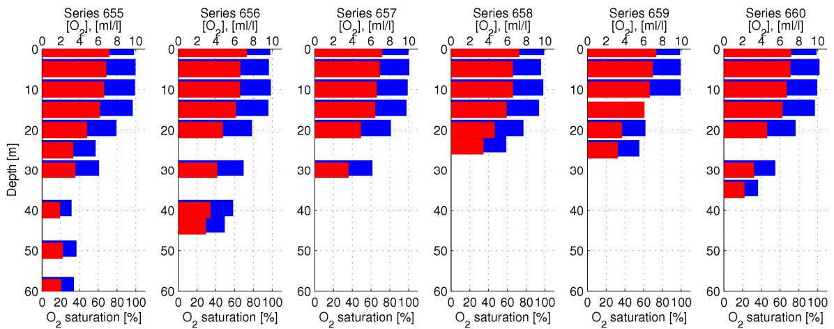
Figure 36 Röde Bank oxygen concentration (red) and saturation(blue)
