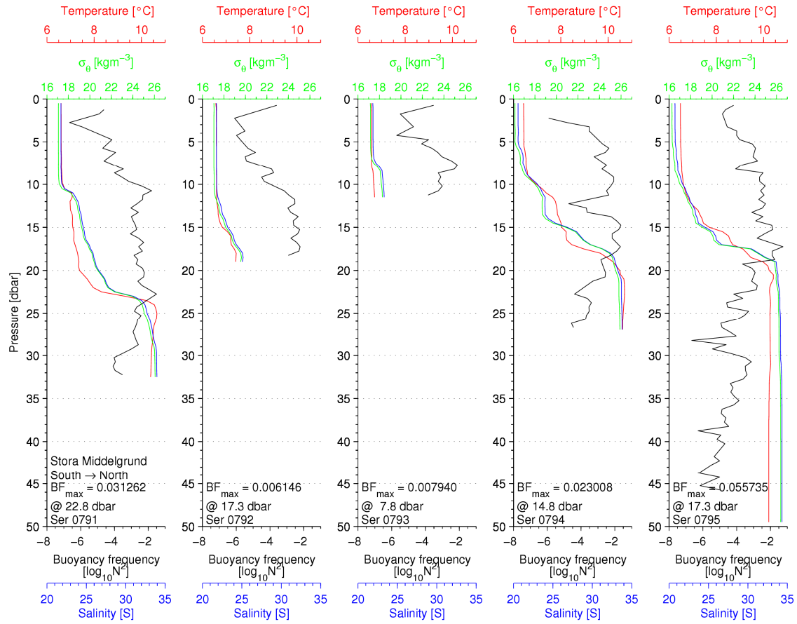
Figure 39 CTD profiles across Stora Middelgrund from south to north
