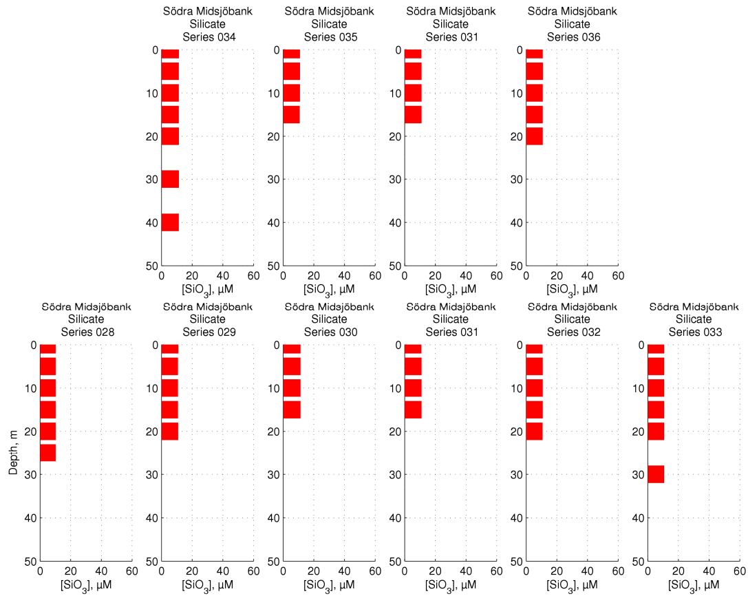
Figure 67 Silicate concentrations over Södra Midsjöbanken
