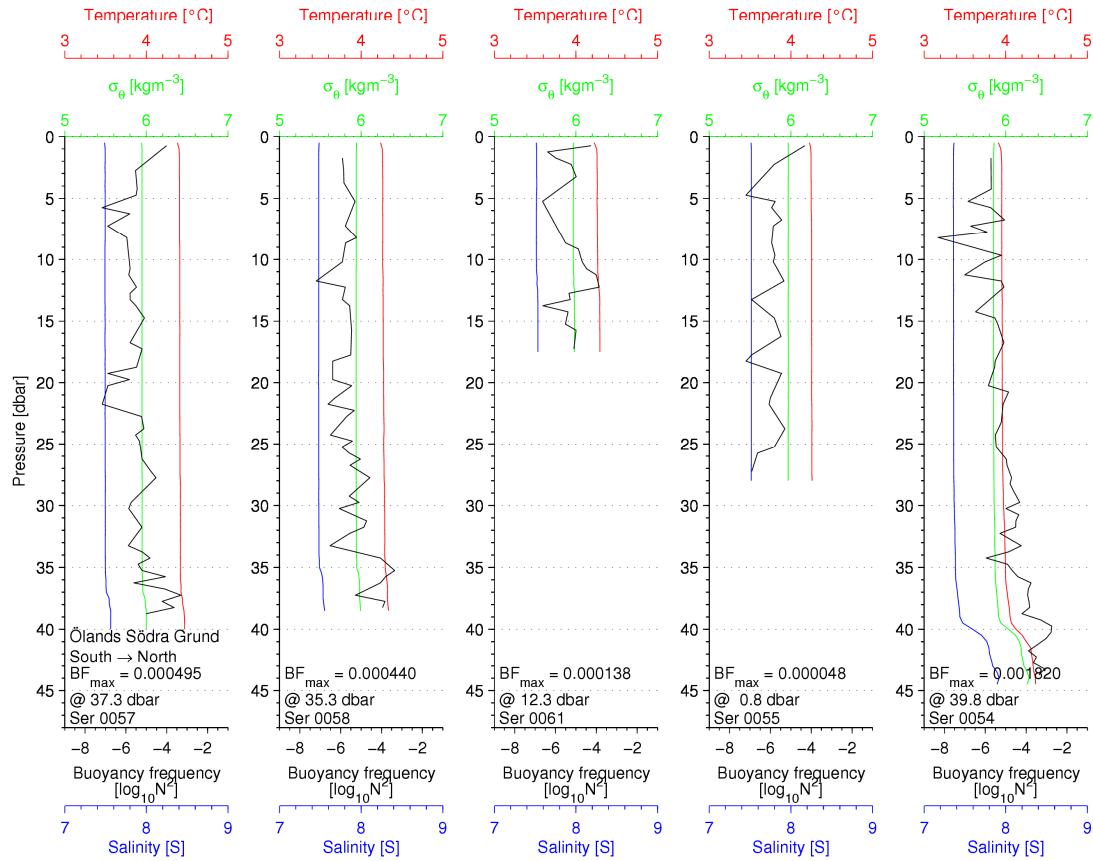
Figure 55 CTD profiles south – north across Ölands Södra Grund
