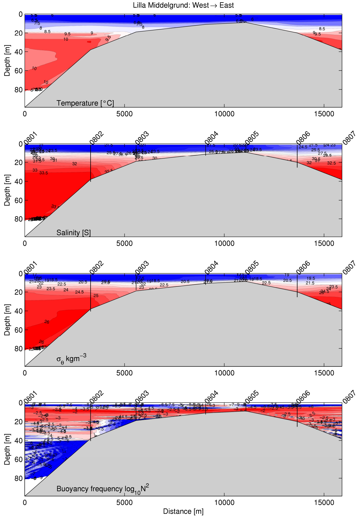
Figure 24 Hydrographic variables gridded over Lilla Middelgrund
