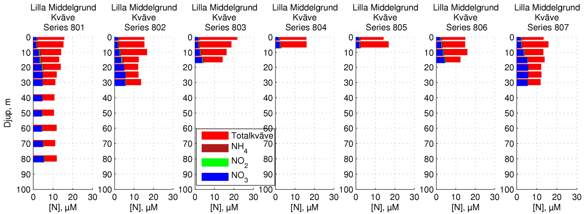
Figure 26 Nitrogen concentrations across Lilla Middelgrund
