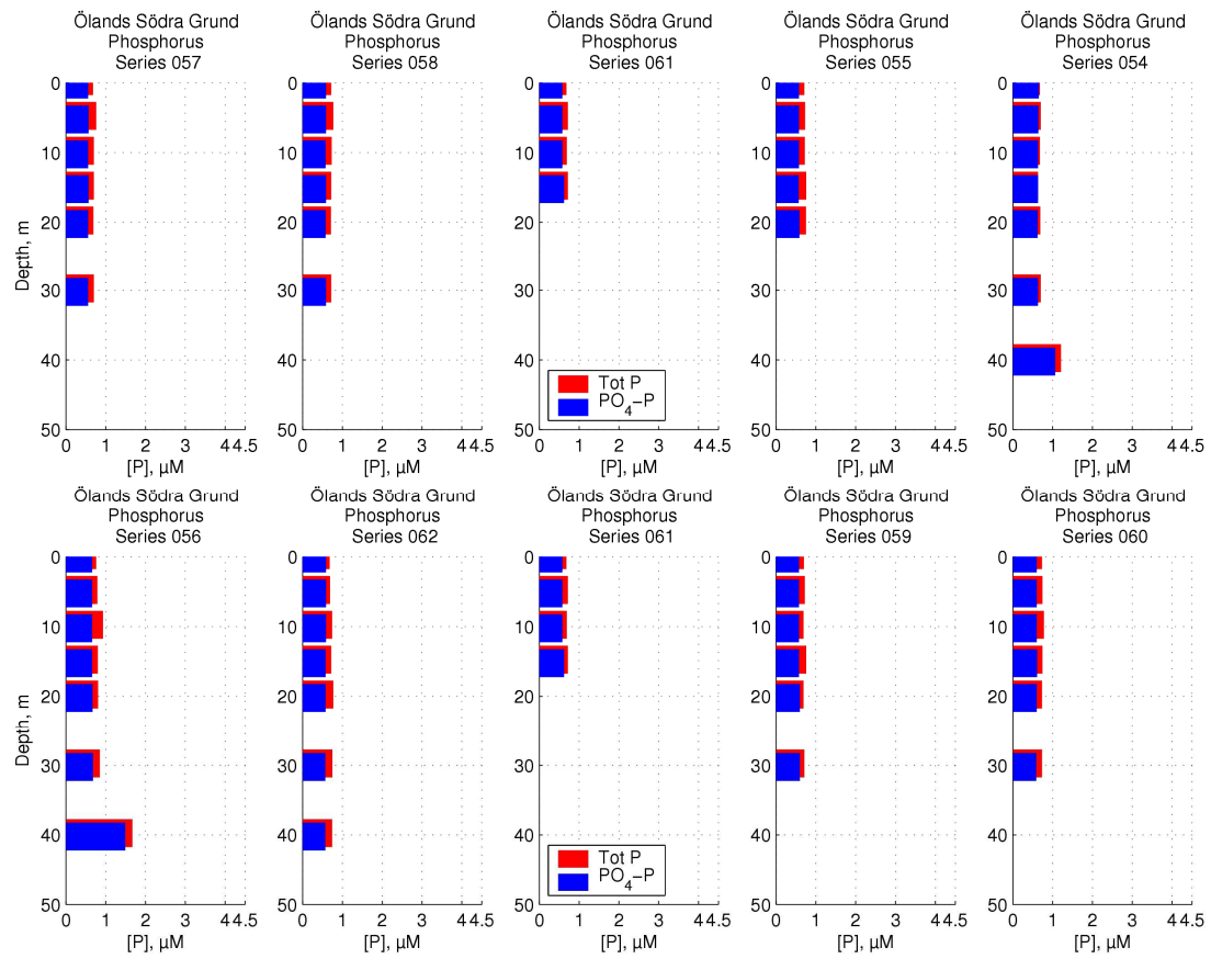
Figure 58 Phosphorus concentrations around Ölands Södra Grund
