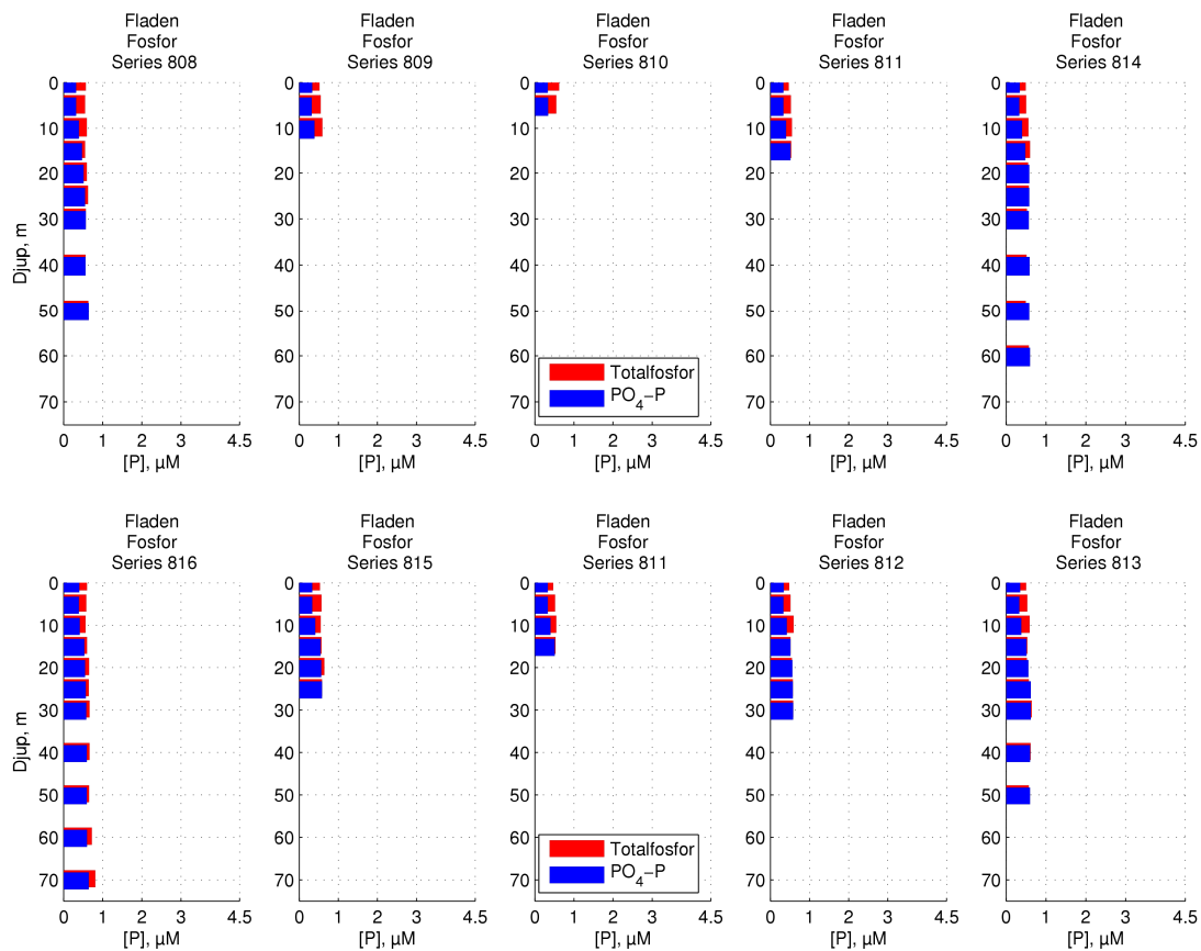
Figure 20 Phosphorus concentrations across Fladen
