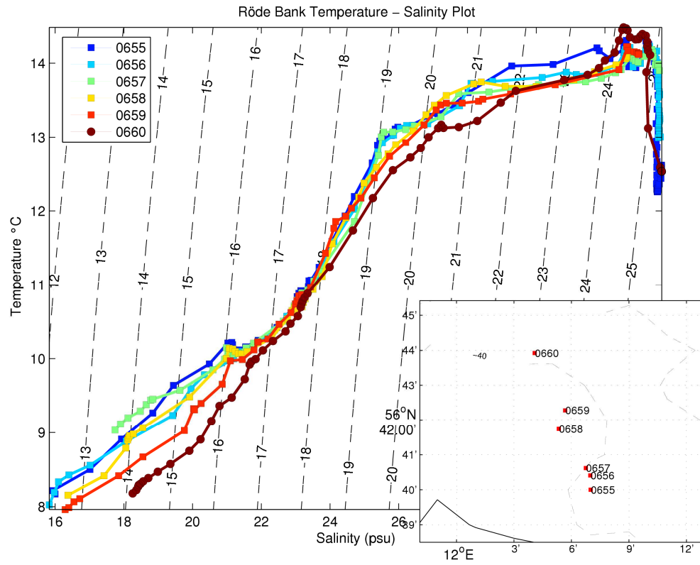
Figure 30 Temperature – Salinity plot over Röde Bank
