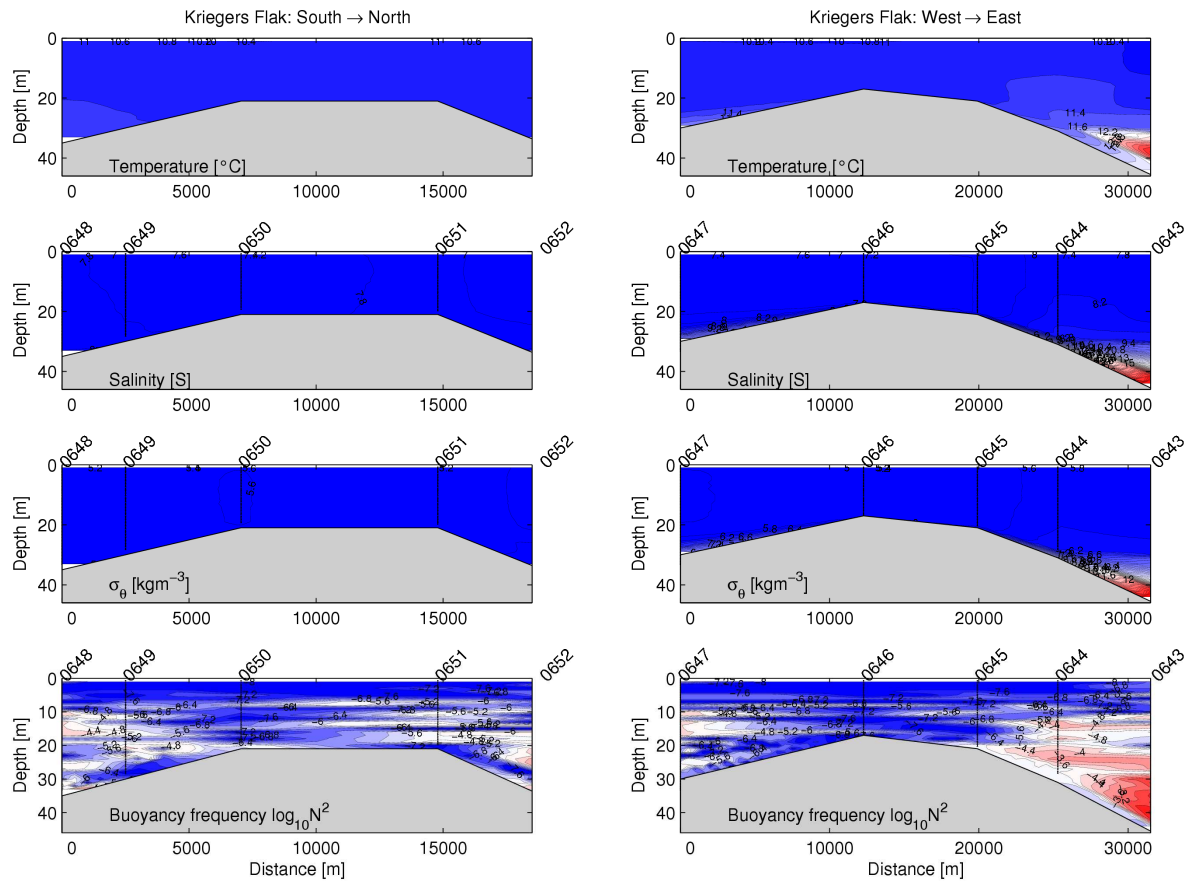
Figure 46 Hydrographic parameters gridded across Kriegers Flak
