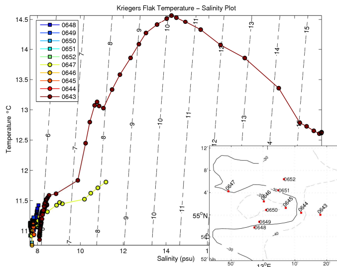
Figure 4 TS-diagram across Kriegers Flak
