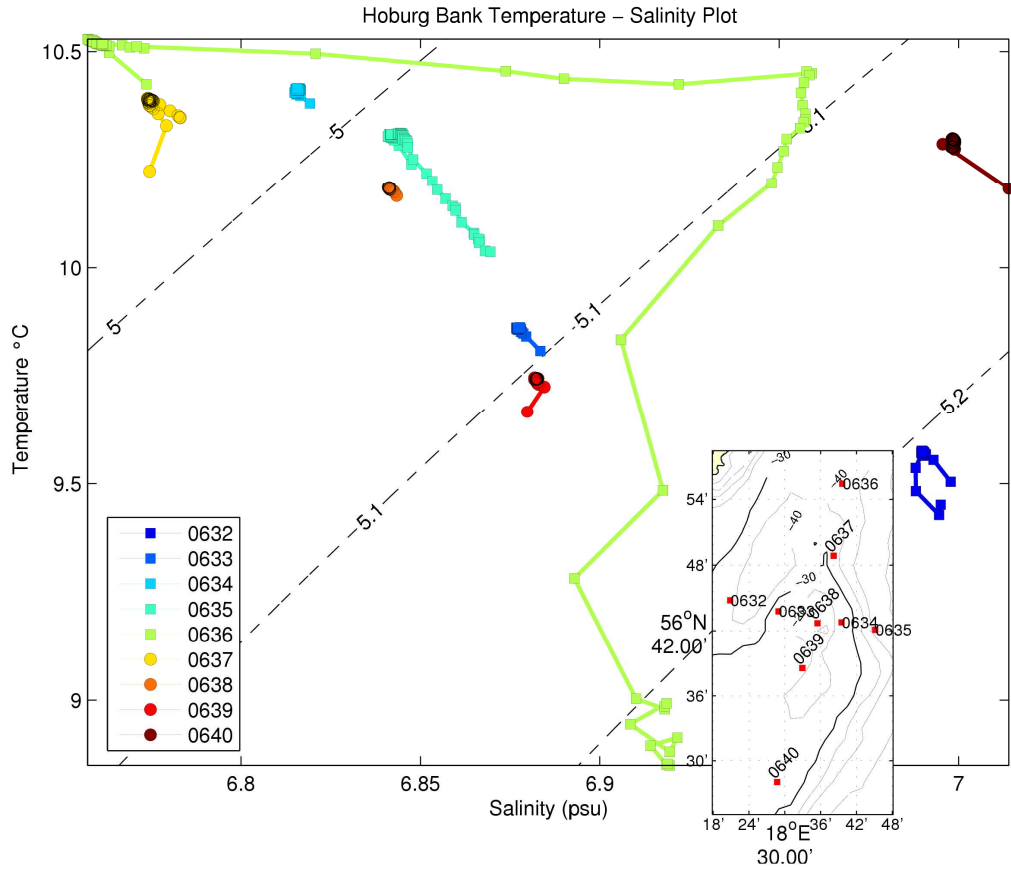
Figure 77 Temperature Salinity data from Hoburg Bank
