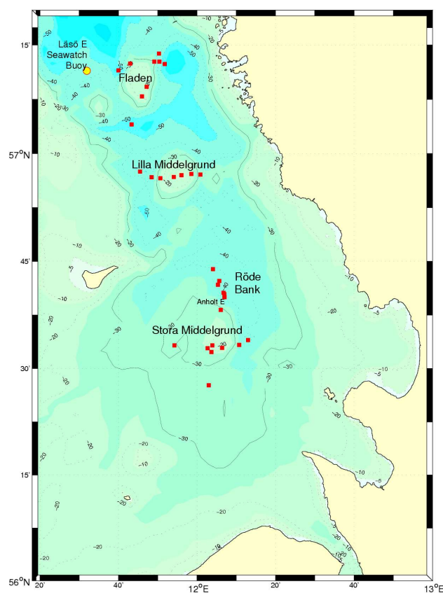
Figure 1 Hydrographic stations taken across the Kattegat Banks, October – December 2003
