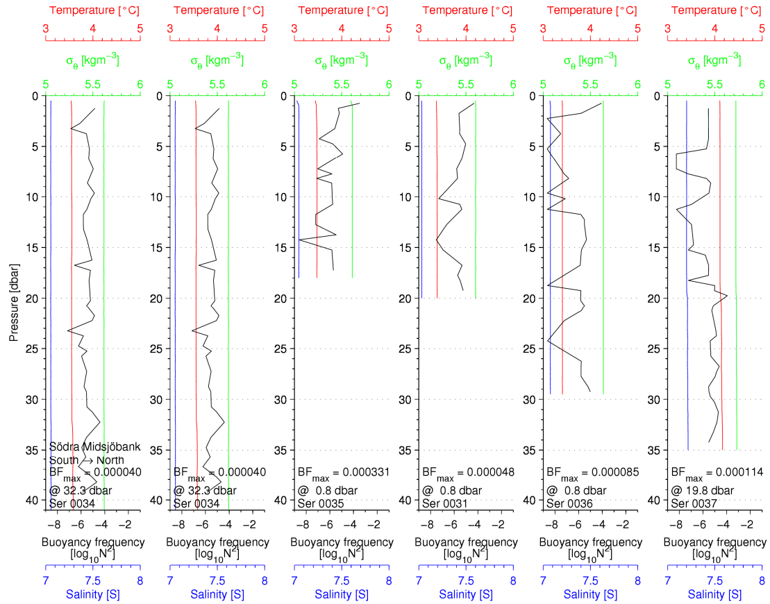
Figure 63 CTD profiles from south – north transect over Södra Midsjöbank
