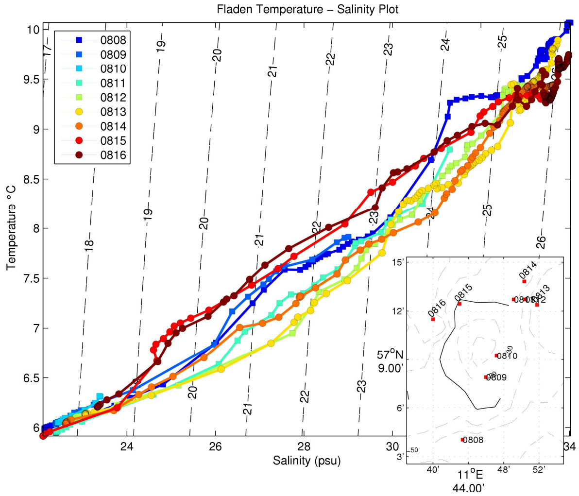
Figure 15 Temperature salinity plot for Fladen
