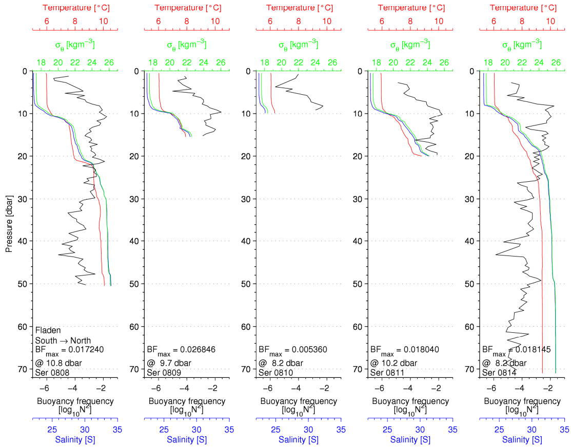
Figure 17 CTD profiles from the south – north transect across Fladen
