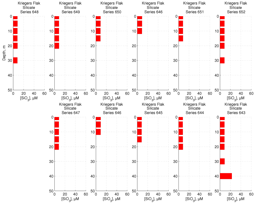
Figure 51 Silicate concentrations in the vicinity of Kriegers Flak
