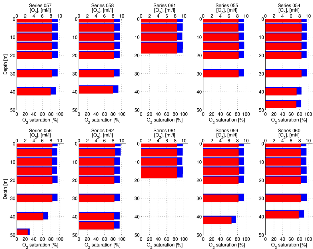
Figure 60 oxygen concentration (red) and saturation (blue) around Ölands Södra Grund
