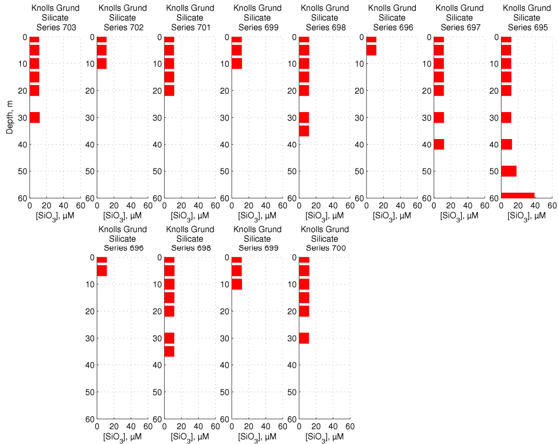
Figure 91 Silicate concentrations over Knolls Grund
