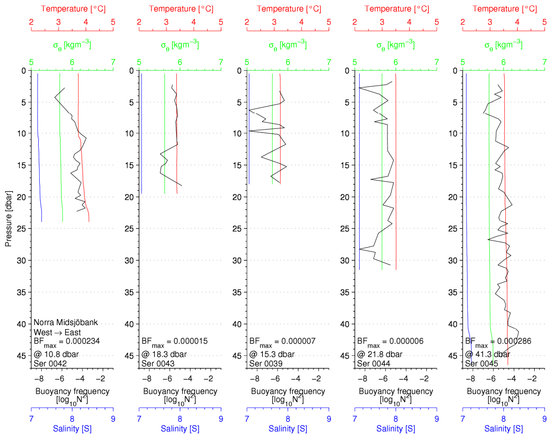
Figure 72 CTD profiles from west to east across Norra Midsjöbank
