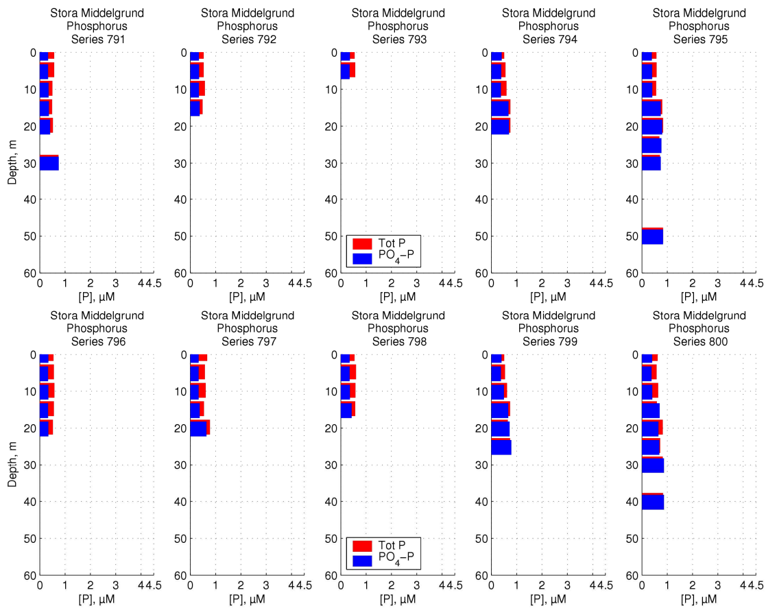
Figure 42 Stora Middelgrund phosphorus concentrations
