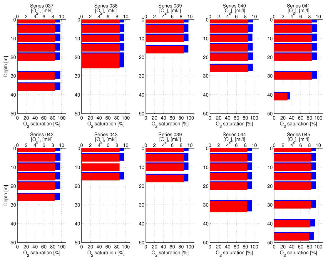
Figure 76 Oxygen concentrations (red) and saturation (blue) over Norra Midsjöbank
