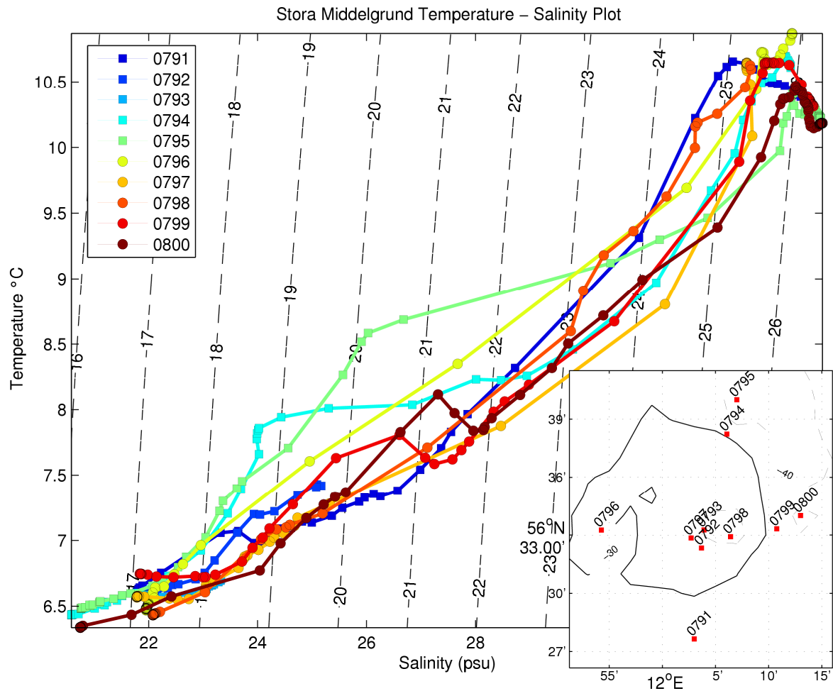
Figure 37 Stora Middelgrund Temperature – salinity plot
