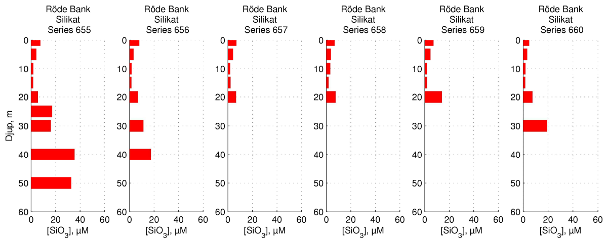
Figure 35 Röde Bank silicate concentrations
