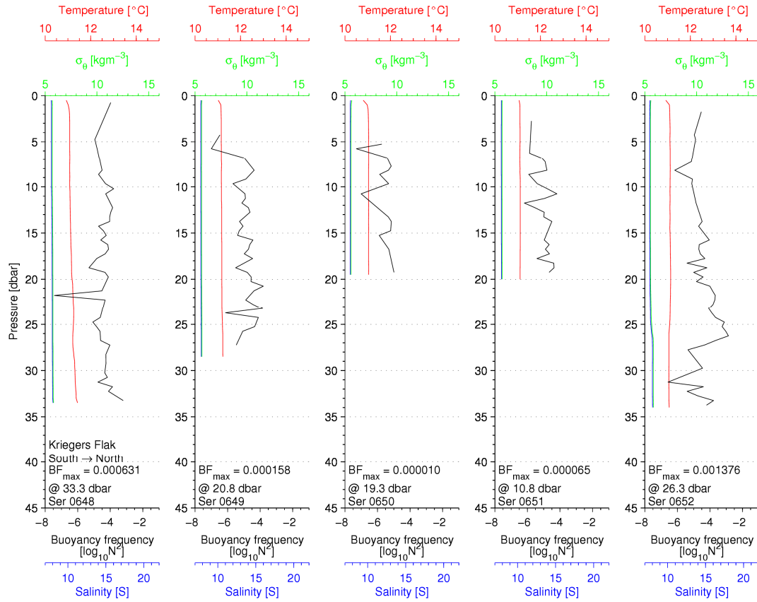
Figure 47 CTD profiles along the south – north transect over Kriegers Flak
