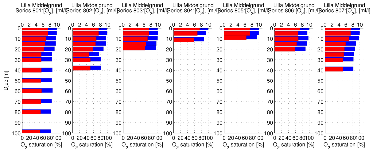
Figure 29 Oxygen concentrations (red) and saturation (blue) across Lilla Middelgrund
