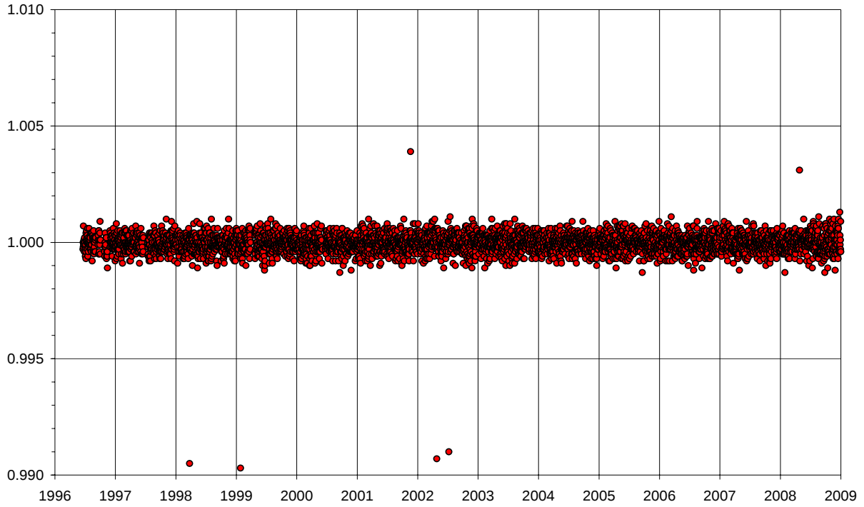
Figure 4.3. Run and stop test for Brewer #128 for the double slit position of the shutter mask for the period 1996-2008.
