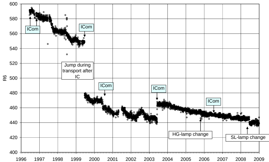
Figure 4.1 Standard lamp test value R_6 for Brewer #128 over the period 1996-2008. The large change after the calibration in 1999 is clearly seen. Times for intercomparisons are noted as well as lamp changes.
