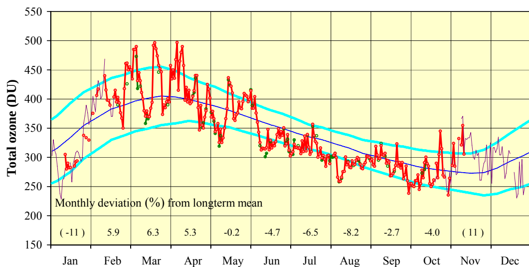
Figure 5.4 Daily 'noon' values of total ozone recorded by Brewer #006 (red) and by Dobson #30 (green) at Vindeln in 2006. Long-term mean and standard deviation are from Uppsala 1951-1966. The values at the bottom are the monthly deviations (percent) from the long term monthly means. All data refer to bass-Paur scale. Missing data are replaced by satellite data (purple line).
