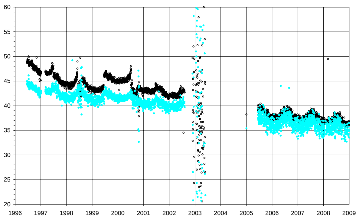
Figure 4.5. Dead-time (ns) for Brewer#006.
