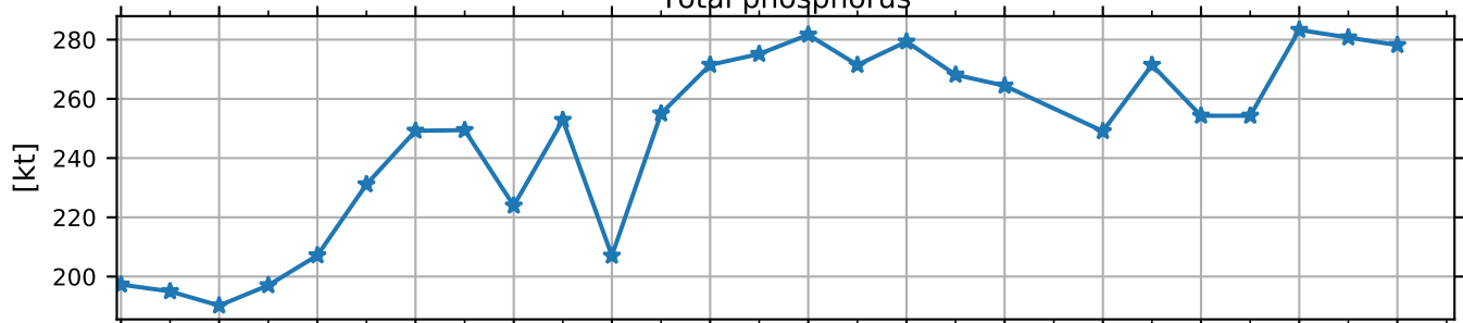
Total phosphorus
