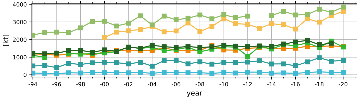
Dissolved Silica
