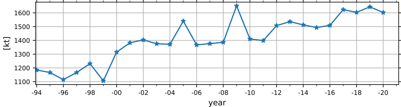
Dissolved Silica
