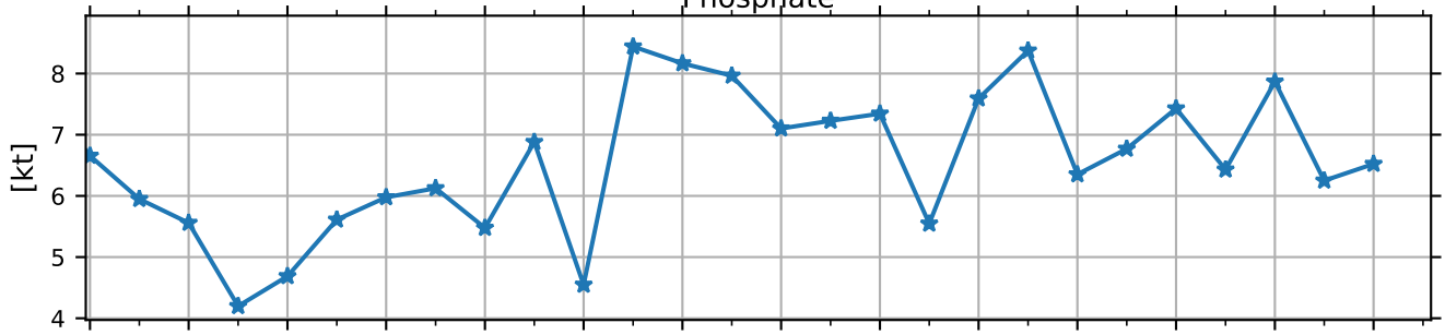
Total phosphorus
