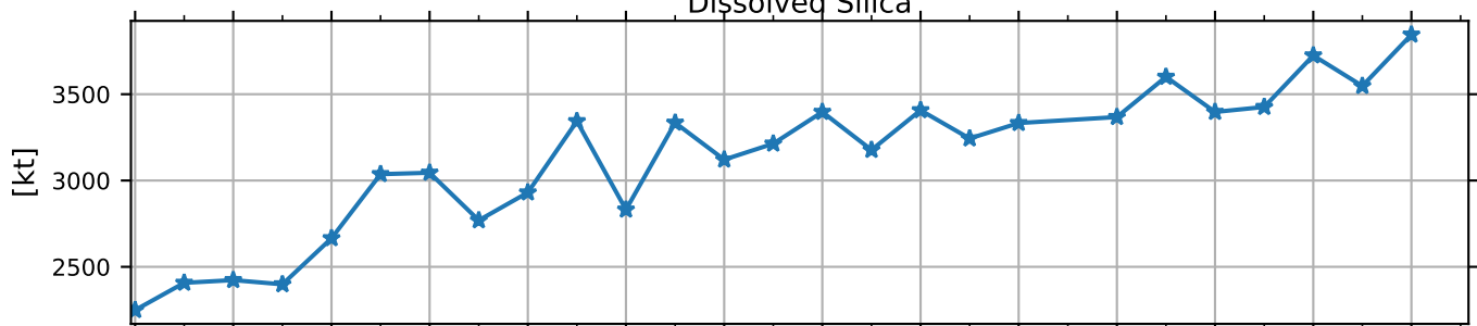
Dissolved Silica
