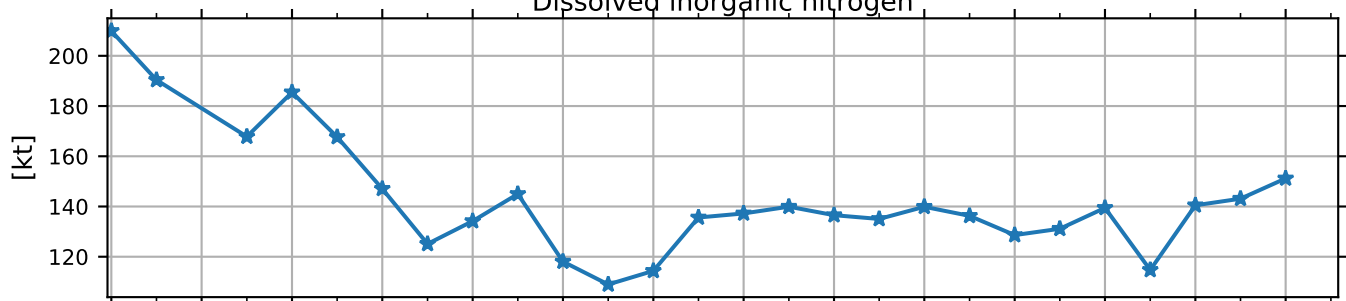
Total Nitrogen
