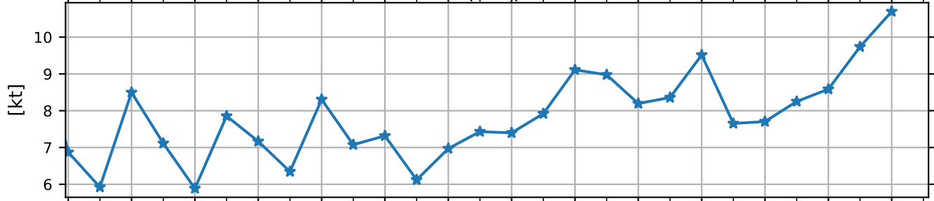
Total phosphorus
