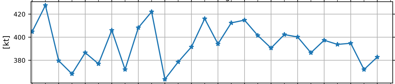
Total Nitrogen
