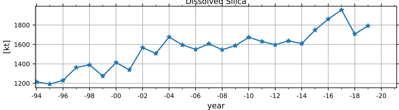
Dissolved Silica
