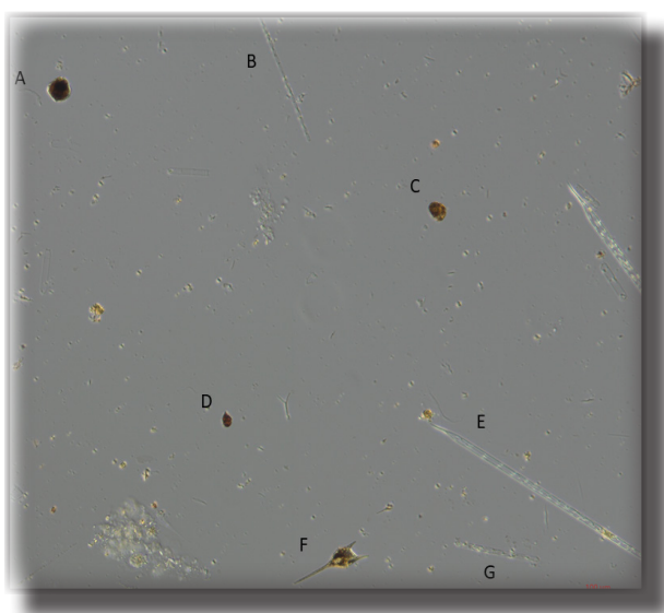
Figure 1. A representation of one of the three stations with high diversity. A. Lingulodinium polyedra *, B. Leptocylindrus minimus , C. Gymnodiniales, D. Scrippsiella CPX, E. Pseudosolenia calcar-avis , F. Triplos lineatus and G. Cerataulina pelagica . Photo: Maria Karlberg.
