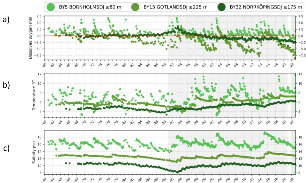
Figure 18. a) Dissolved oxygen, b) temperature and c) salinity in the bottom water at three stations in the Baltic Proper representing the basins Bornholm Basin (BY5), Eastern Gotland Basin (BY15), Western Gotland Basin (BY32). The shadowed grey area highlights the time period that statistics is based on in this report, 1991-2020. The shadowed green area highlights the year 2022.
