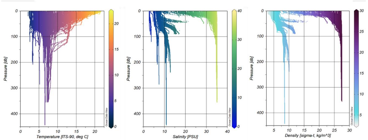
Figure 3. All temperature, salinity and density profiles from the SMHI monitoring cruises during 2022
