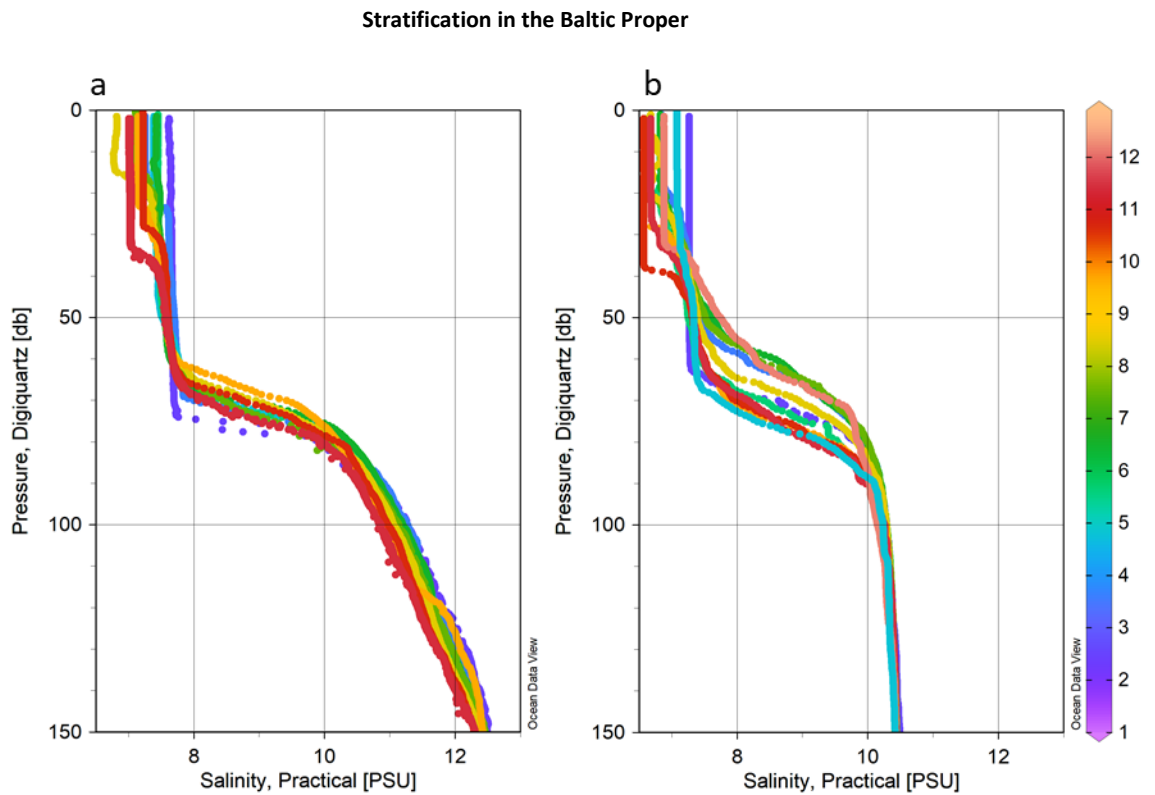
Figure 16 Profiles of salinity at a) BY15 Gotland deep and b) BY32 Norrköping deep from 2022. The figure shows the more variable halocline depth in the Western Gotland Basin (b) compared to the Eastern Gotland Basin (a).
